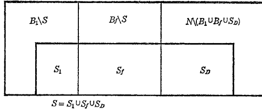
Fig. 3.1. Relation of a Minimal Cover S to x^* .
