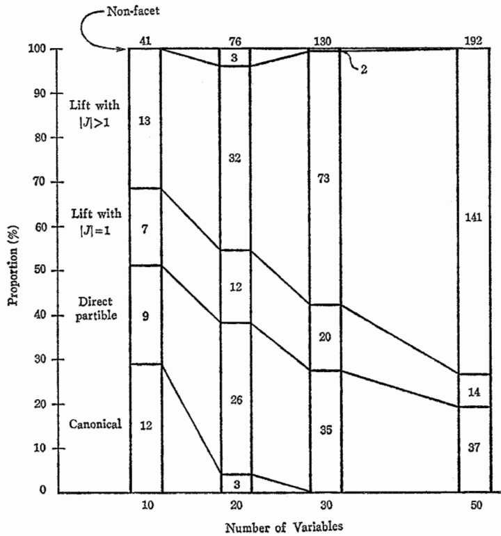
Fig. 5.4. Proportion of Various Facets.
