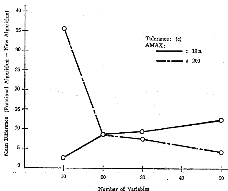
Fig. 5.2. Mean Difference of Objective Function Values at Termination.
