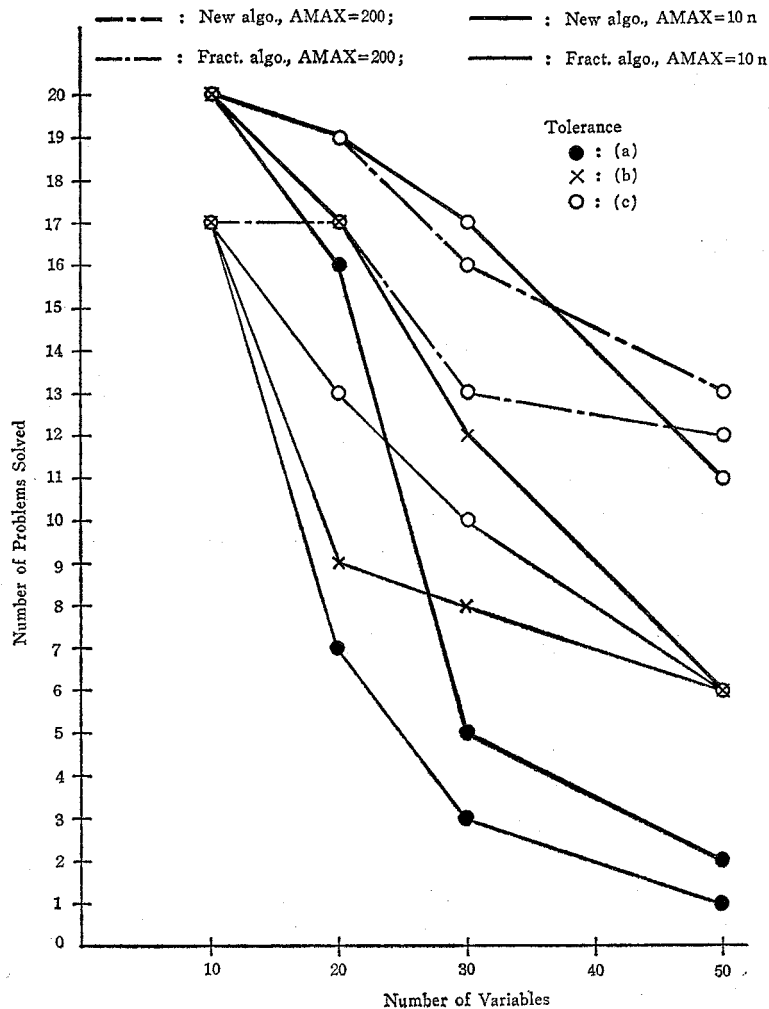
Fig. 5.1. Number of Solved Problems.
