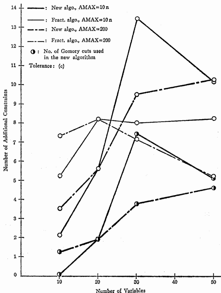
Fig. 5.3. Number of Additional Constraints.
