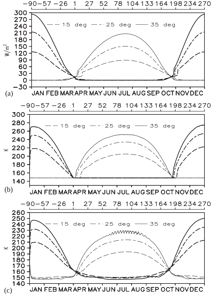
Figure 4: (a) Annual cycle of net incoming radiation (see text for definition), (b) surface temperature, and (c) atmospheric temperature at 1 km height. Shown are curves for 80°N (thin) and 80°S (bold) for obliquity angles of 15° (dashed), 25.2° (dot-dashed) and 35° (solid). The upper x -axis gives solar longitude ( L_s ) in deg, the lower x -axis label are the month of the year.
