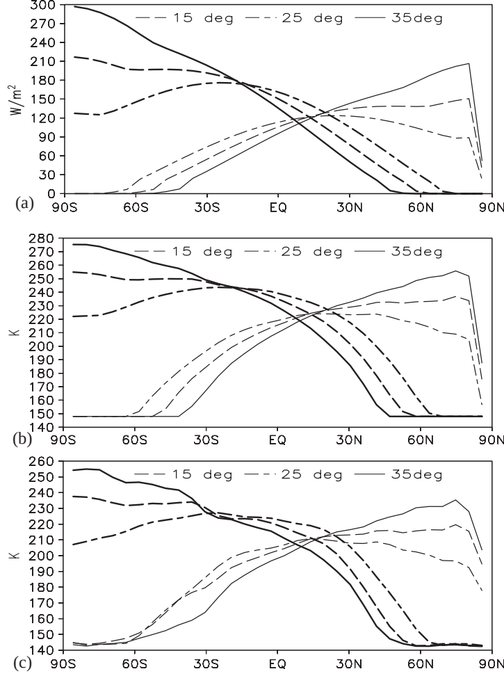
Figure 5: Zonal mean of (a) net incoming radiation, (b) surface temperature, and (c) atmospheric temperature at 1 km height in southern summer ( L_s = 270^\circ , bold) and northern summer ( L_s = 90^\circ , thin) for different obliquity angles: 15^\circ (dashed), 25.2^\circ (dot-dashed) and 35^\circ (solid).
