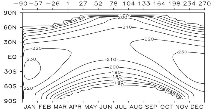
Figure 3: Seasonal cycle of ground temperature (K) for an obliquity angle of 15^\circ . Shown are daily and zonally averaged means. The contour interval is 10 K. The upper x -axis gives solar longitude ( L_s ) in deg, the lower x -axis label are the month of the year. The step-like features of the 150 K contour line are the result of the coarse model resolution and the albedo parameterization.
