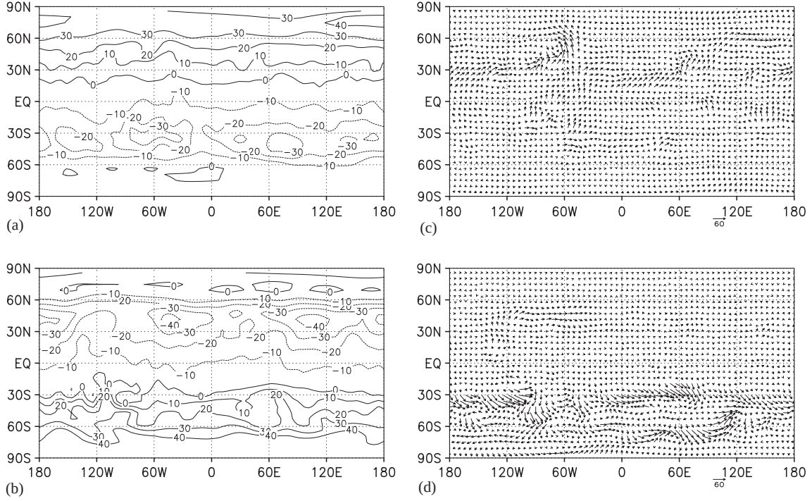
Figure 8: Difference of atmospheric temperature in K (a,b) and wind field in \text{m s}^{-1} (c,d) at 1 km height for \phi = 35^\circ minus \phi = 15^\circ for (a,c) northern summer ( L_s = 90^\circ ) and (b,d) southern summer ( L_s = 270^\circ ). The scale arrow corresponds to 60 \text{ m s}^{-1} .
