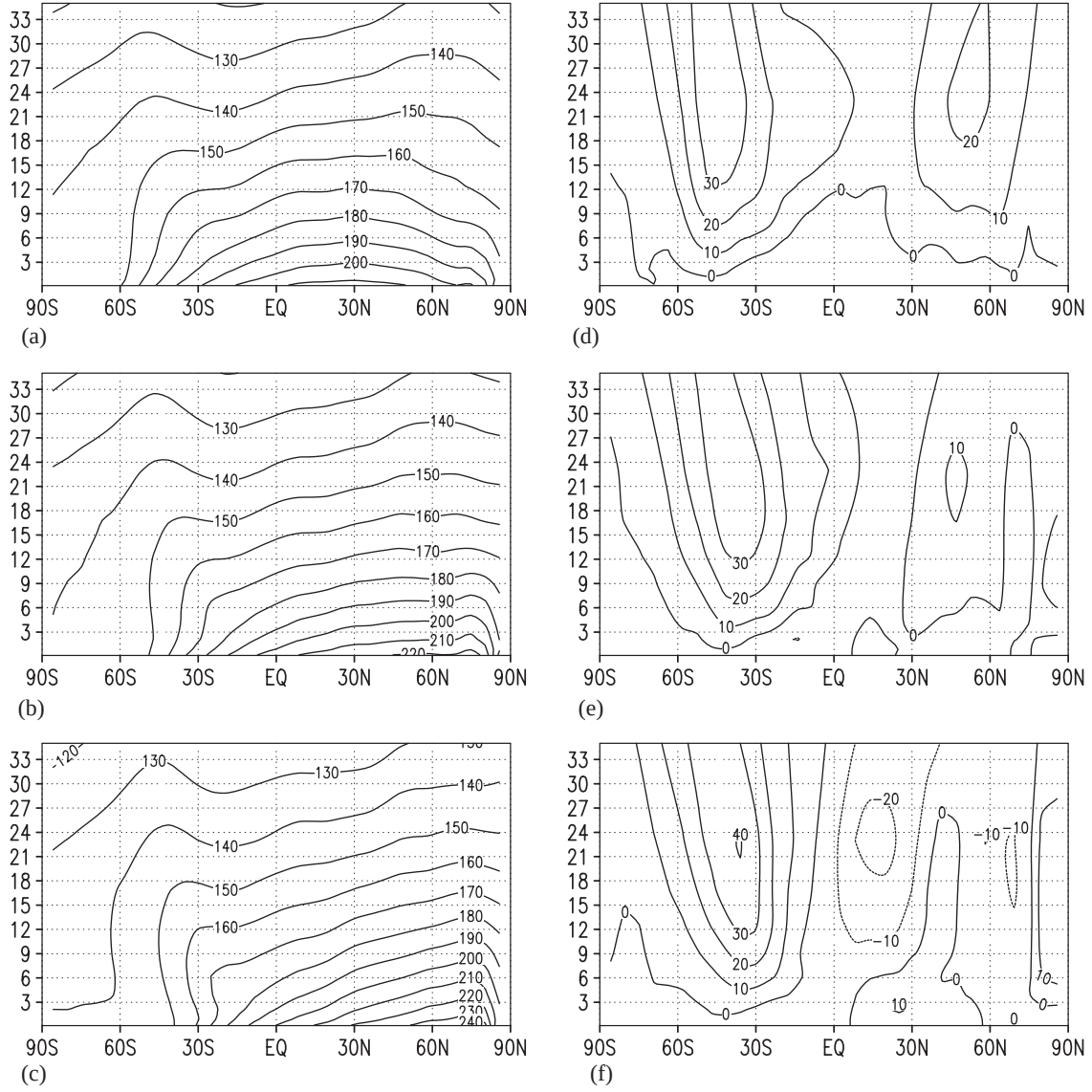
Figure 9: Vertical sections of zonal means of atmospheric temperature in K (a–c, contour interval 10 K) and zonal velocity in \text{m s}^{-1} (d–f, contour interval 10 \text{ m s}^{-1} , negative, i.e. westward values are stippled) for northern summer ( L_s = 90^\circ ) for an obliquity of (a,d) 15^\circ , (b,e) 25.2^\circ , and (c,f) 35^\circ . The height is given in km.
