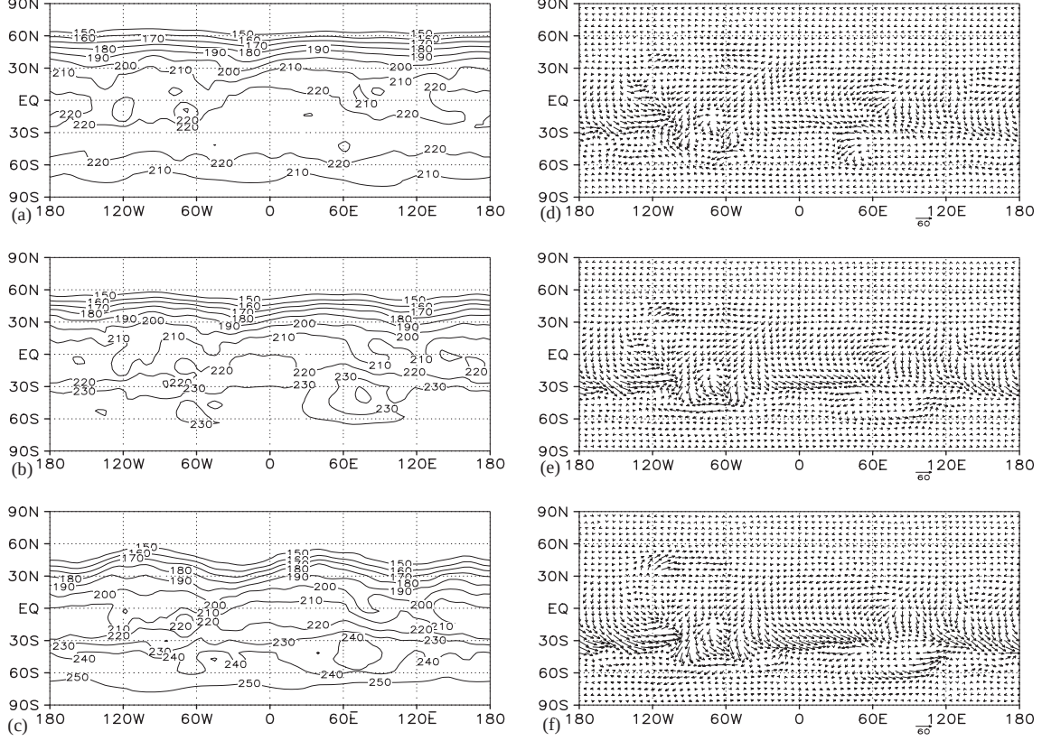
Figure 7: Atmospheric temperature in K (a–c) and wind field in \text{m s}^{-1} (d–f) at a height of 1 km for southern summer ( L_s = 270^\circ ) for an obliquity of (a,d) 15^\circ , (b,e) 25.2^\circ , and (c,f) 35^\circ . The scale arrow corresponds to 60 \text{ m s}^{-1} .
