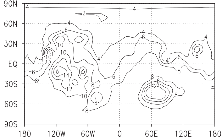
Figure 1: MOLA topography on the model grid in km, normalized to positive values.
