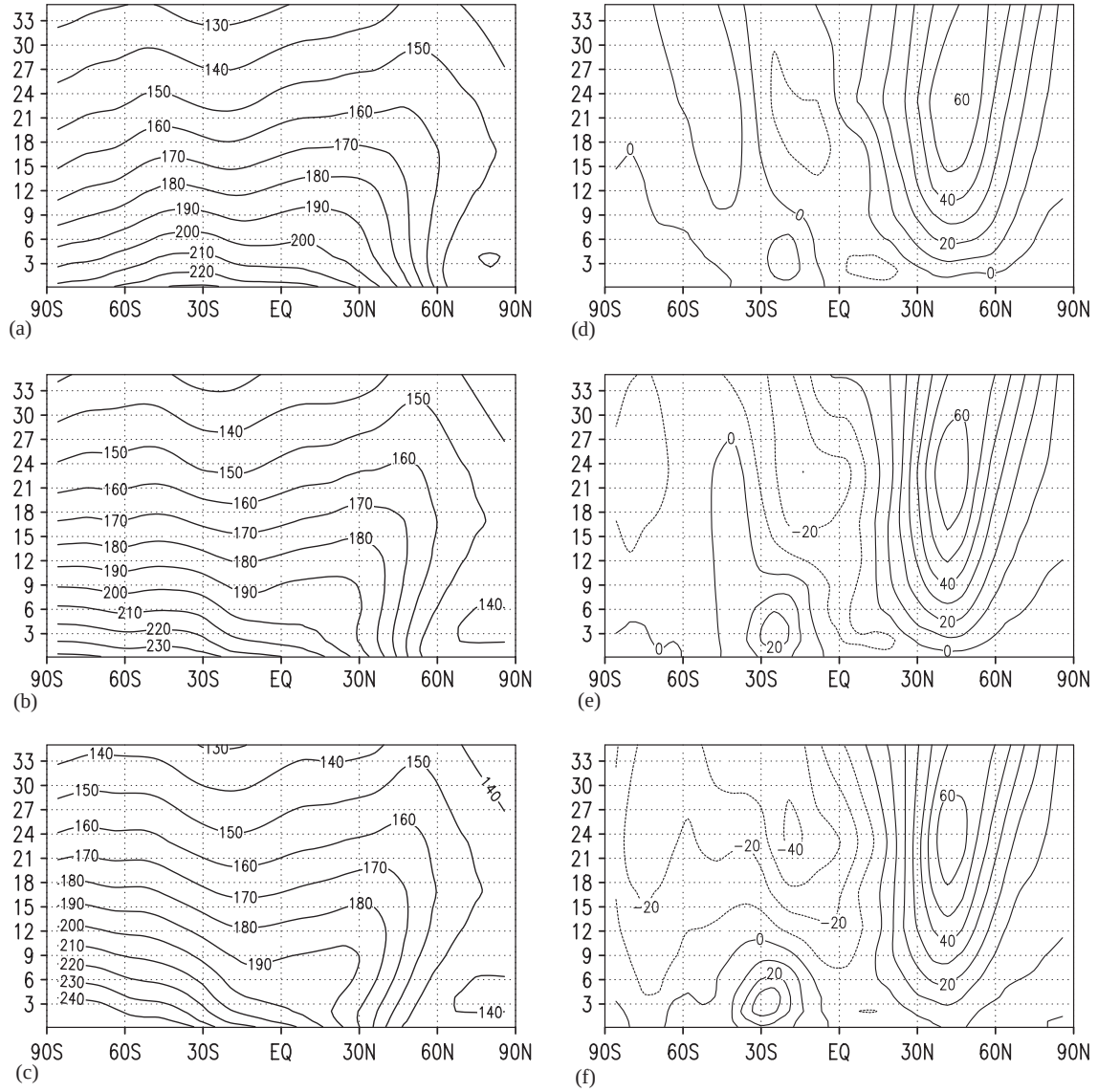
Figure 10: Vertical sections of zonal means of atmospheric temperature in K (a–c) and zonal velocity in \text{m s}^{-1} (d–f, contour interval 10 \text{ m s}^{-1} ) for southern summer ( L_s = 270^\circ ) for an obliquity of (a,d) 15^\circ , (b,e) 25.2^\circ , and (c,f) 35^\circ . The height is given in km.
