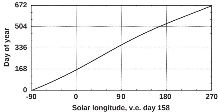
Figure 2: Solar longitude L_s vs. day of the year for \varepsilon = 0.093 , vernal equinox (v.e.) day 158, and longitude of perihelion \lambda_p = 250.87^\circ computed following Berger (1978).
