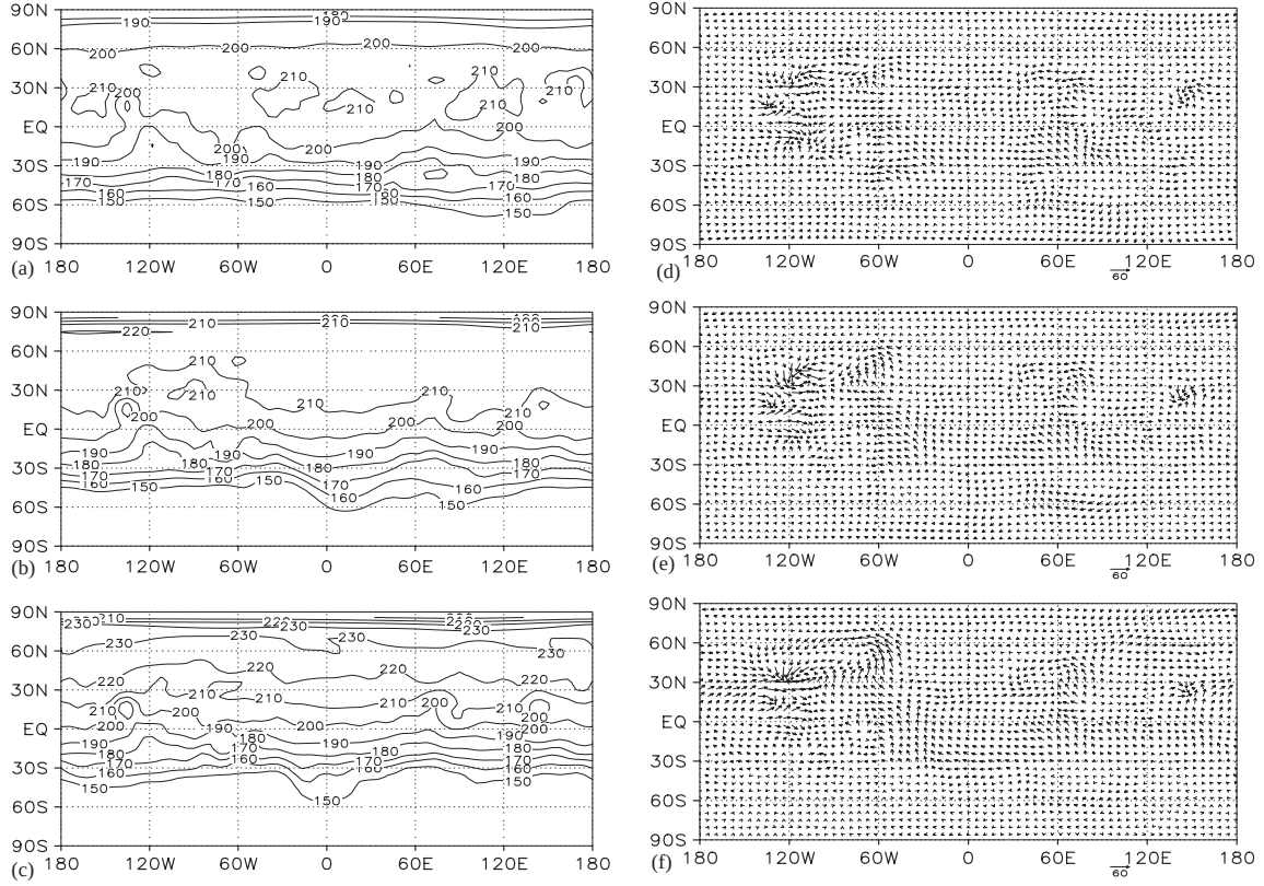
Figure 6: Atmospheric temperature in K (a–c) and wind field in \text{m s}^{-1} (d–f) at a height of 1 km for northern summer ( L_s = 90^\circ ) for an obliquity of (a,d) 15^\circ , (b,e) 25.2^\circ , and (c,f) 35^\circ . The scale arrow corresponds to 60 \text{ m s}^{-1} .
