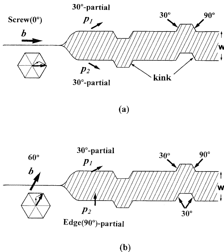
Figure 5: Extended dislocations in ice. The perfect dislocation with the Burgers vector \mathbf{a} dissociates into two partial dislocations with the Burgers vectors \mathbf{p}_1 and \mathbf{p}_2 , where \mathbf{a} = \mathbf{p}_1 + \mathbf{p}_2 , to reduce the total self-energy of the dislocation. (a) screw dislocation and (b) 60°-dislocation lying along the Peierls trough are illustrated. The screw dislocation dissociates into two 30°-partial dislocations, whereas the 60°-dislocation dissociates into edge (90°)- and 30°-partial dislocations. In ice, the width w is very large as shown in Table 3, and therefore the double kink formation on the two partials must not correlate each other.
