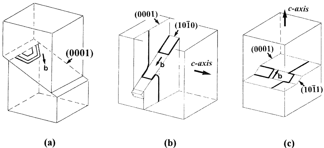
Figure 7: Deformation resulting from dislocation glide in ice. A tensile force is applied in the vertical direction. (a) Deformation by basal dislocations a . Continuous, long slip lines appear on the surface. (b) Deformation by prismatic dislocations a . Glide motion on the pyramidal planes \{10\bar{1}1\} is also possible (see Fig. 3) [9, 12, 41]. Characteristic surface-steps form. Note that successive dislocation generation at the same source is allowed because the basal segments are glissile. (c) Deformation by pyramidal dislocations a+c . A trace of shear appears on the surface, but surface-steps are not expected, and successive generation of the dislocations from the same source are not expected because of the sessile basal segments. Glide motions on the pyramidal planes \{11\bar{2}2\} and on the prism planes \{10\bar{1}0\} are also possible (see Fig. 3). Similar way of deformation is expected for dislocations c .
