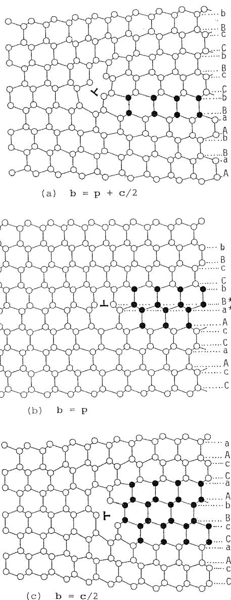
Figure 4: Partial dislocations in ice. These figures illustrate atomic arrangements around three possible partial dislocations, (a) b=p+c/2 , (b) b=p , and (c) b=c/2 . The stacking sequences of the atomic layers indicated by the filled circles are different from the original ones (open circles). The stacking fault has no difference in the nearest neighbors with ice I_h as shown in Fig. 2, but it has second nearest neighbors the same those in the cubic structure I_c . (from Fukuda et al. [1])
