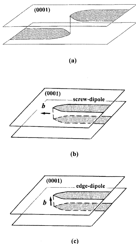
Figure 6: Possible configurations of nonbasal dislocations in ice. (a) A terraced structure of a dislocation in ice [11]. The step height observed by XRT is of the order of 0.1 mm [7, 20, 41]. Basal segments with the Burgers vector \mathbf{a} are glissile, but others with \mathbf{c} or \mathbf{a}+\mathbf{c} are sessile. Nonbasal segments are glissile on the planes given in Fig. 3. (b) Formation of a screw dislocation dipole with the Burgers vector \mathbf{a} led by an edge segment gliding on the nonbasal plane [7, 20]. Basal segments are glissile. (c) Formation of an edge dislocation dipole with the Burgers vector \mathbf{c} or \mathbf{a}+\mathbf{c} led by a screw segment gliding on the nonbasal plane. Basal segments are sessile. See also Fig. 7.
