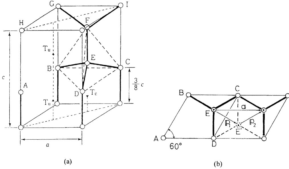
Figure 2: Crystal structure of ice I_h and stacking faults. (a) The unit cell of ice I_h . Water molecules sit on the open circles and are bonded with each other by hydrogen bonds marked by the thick lines. The lattice constants a and c are 4.52Å and 7.36Å, respectively. A tetrahedral bonding is shown by BCDF centered at E. T_u and T_c are the interstitial sites [6, 25]. (b) Stacking faults in ice. When the upper half crystal above E is translated by a vector \mathbf{a} , (1/3)\langle 11\bar{2}0 \rangle , the crystal structure is identical with that before the translation, then the dislocation with this Burgers vector is called a perfect dislocation because it equals a perfect translation vector. In contrast, a different crystal structure is brought by the imperfect translation \mathbf{p}_1 , (1/3)\langle 10\bar{1}0 \rangle because there is no water molecule at E' in the original crystal. However, tetrahedral hydrogen bonding can still form at E' as shown by the dotted lines. The dislocation with the Burgers vector \mathbf{p}_1 is called a partial dislocation. A partial dislocation always has a plane defect brought by the imperfect translation \mathbf{p}_1 . Introduction of this type of plane defect changes the stacking sequence of the atomic layers from the original one; thus, it is called a stacking fault. For hexagonal crystals, this results in the stacking sequence of a cubic structure I_c .
