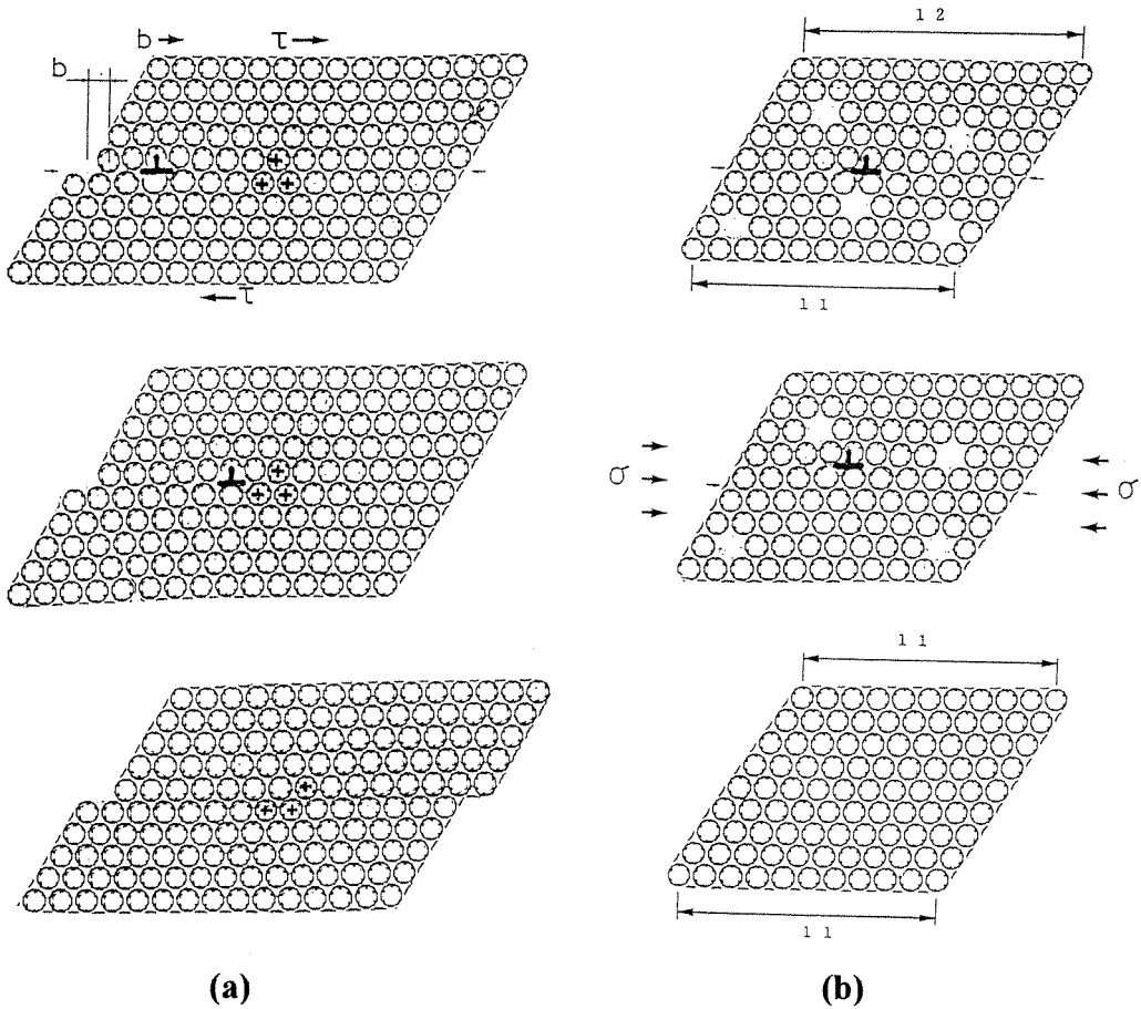
Figure 1: Two types of dislocation motion. (a) Glide motion. An edge dislocation (normal to the page) is passing through the crystal from left to right under a shear stress \tau causing the top half of the crystal to displace by b compared to the bottom half. This slip vector b is called the Burgers vector, and the plane parallel to both b and the dislocation line is called the glide plane. We define the glide motion of a dislocation by its motion on the glide plane. The small displacements of individual atoms during the glide motion are cooperative motions of many atoms required by the glide motion. (b) Climb motion. Dislocation motion in the direction normal to the glide plane is called climb motion. In this figure, the edge dislocation is moving upward by absorbing vacancies under a compression stress \sigma . Then, the top half crystal is compressed by b . For ice, interstitial water molecules are emitted instead of vacancies as described in section 2.6 (from Hondoh [5]).
