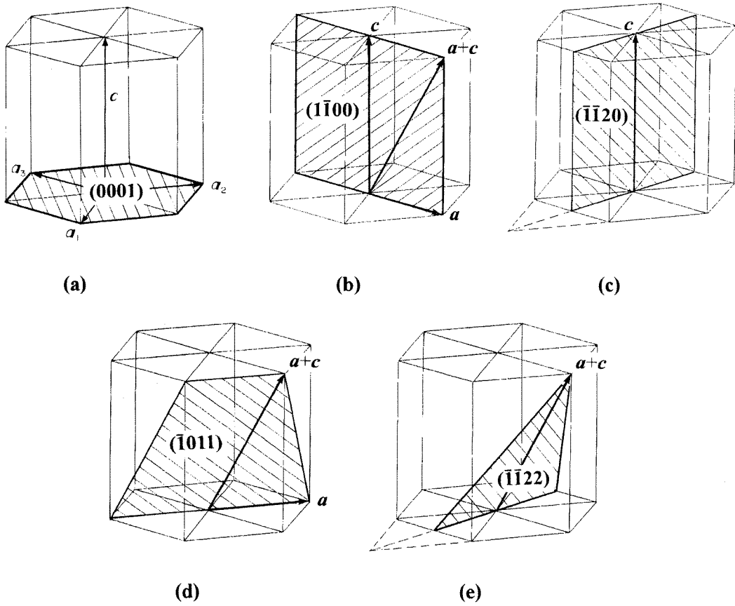
Figure 3: Burgers vectors and glide planes of dislocations in ice. (a) The plane expressed by the notation (0001) is called a basal plane. The primary slip occurs on this plane by the dislocations with the Burgers vector a . (b) The prismatic slip on \{10\bar{1}0\} can be caused by a , c and a+c . (c) The prismatic slip on \{11\bar{2}0\} can be made only by c . (d), (e) The pyramidal slip by a+c takes place on \{10\bar{1}1\} or \{11\bar{2}2\} . For detail see Table 1.
