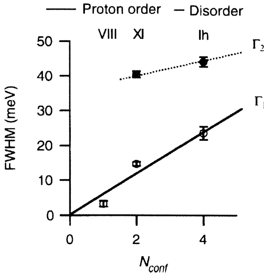
Figure 7: Proton-configuration ( N_{conf} ) dependence of FWHM ( \Gamma_1 and \Gamma_2 ) of ice Ih, XI and VIII [8]. Open and solid circles represent \Gamma_1 and \Gamma_2 , respectively.
