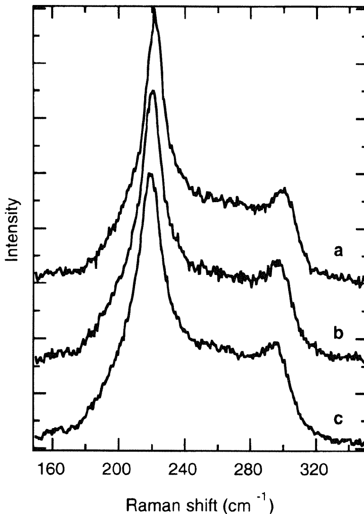
Figure 4: Raman spectra of ice Ih in the region of translational lattice vibrations ( 150\text{--}350\text{ cm}^{-1} ). Measurement temperatures: (a) 220 K, (b) 238 K and (c) 253 K. The polarization plane of the incident beam was parallel to the c-axis of the sample.
