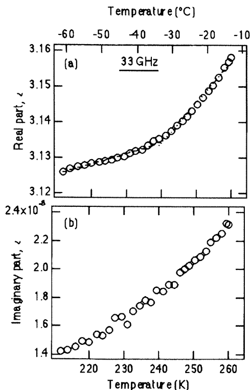
Figure 14: Temperature dependence of permittivities of DF ice core at 33 GHz [55]. (a) real part, \varepsilon' , (b) imaginary part, \varepsilon'' .
