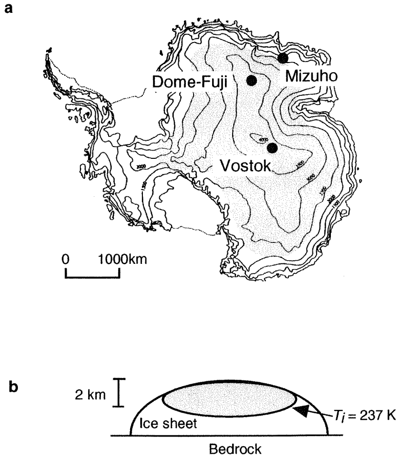
Figure 8: (a) The drilling sites of Dome-Fuji, Mizuho and Vostok ice in Antarctica. The shaded area represents the area where T_i \leq T_c = 237 K on the Antarctic ice sheet surface. (b) Schematic diagram of a cross section of the Antarctic ice sheet. The hatched area shows the area where the ice contains proton-ordered arrangements.
