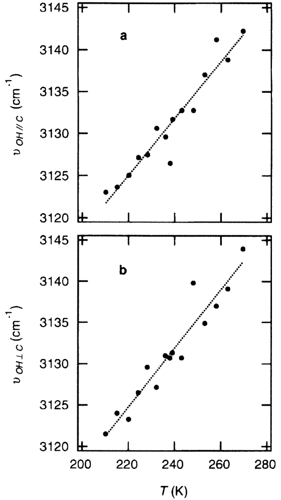
Figure 12: The T dependence of the frequency of the peak of the O-H stretching vibrations, \nu_{OH} , observed by Raman spectroscopy of the c -axis parallel (a) and perpendicular (b) to the polarization plane of the incident beam.
