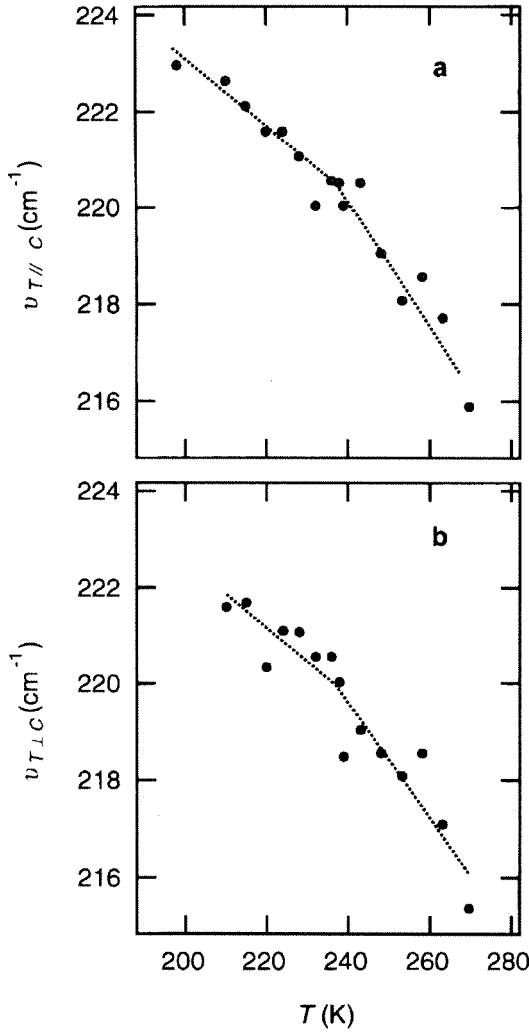
Figure 11: The measurement temperature, T , dependence of the frequency of translational lattice vibrations, \nu_T , observed by Raman spectroscopy of the c -axis parallel (a) and perpendicular (b) to the polarization plane of the incident beam.
