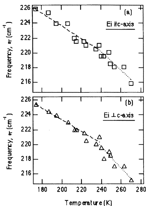
Figure 13: The T dependence of the frequency of translational lattice vibrations in DF ice observed by Raman spectroscopy of the c-axis parallel, (a), and perpendicular, (b), to the electric field [55].
