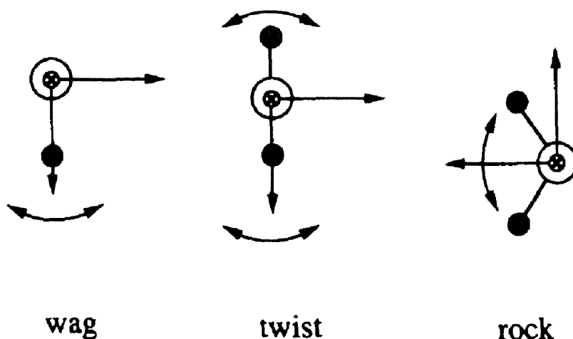
Figure 5: The three librational modes for a water molecules: wag, twist and rock. Oxygen nuclei are represented by open circles and protons by shaded circles [25].
