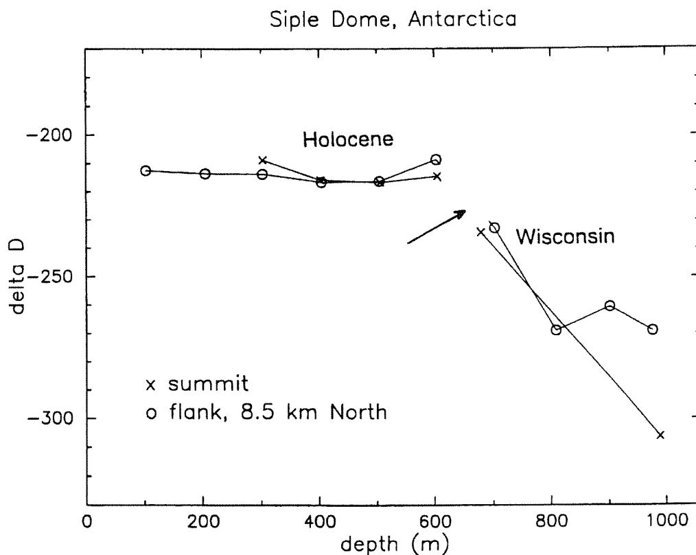
Figure 8: Plot of stable isotope measurements made on cores from the summit and flank of Siple Dome. Analyses were performed by Dr. Jean Jouzel on samples prepared at Siple Dome by Dr. Jean Robert Petit.
