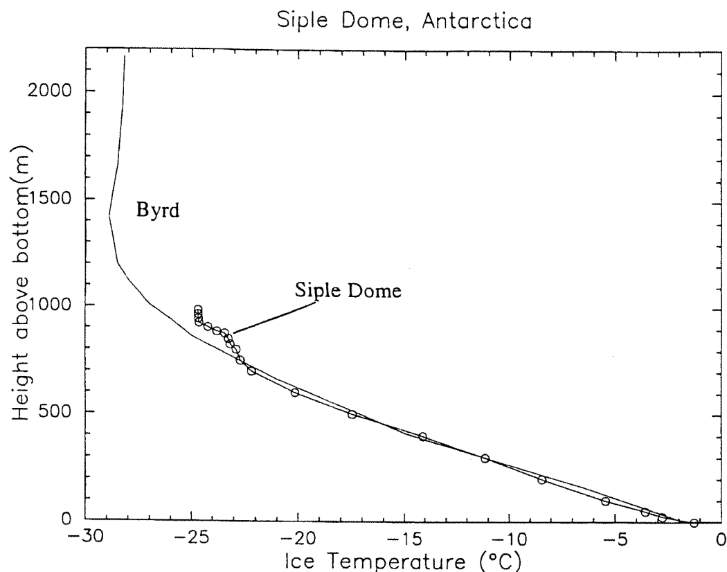
Figure 4: Siple Dome temperature profile superimposed on the Byrd Station profile. Temperature at the bed at Siple Dome measured -1.3^{\circ}\text{C} , \sim 0.5^{\circ}\text{C} below the calculated pressure melting point.
