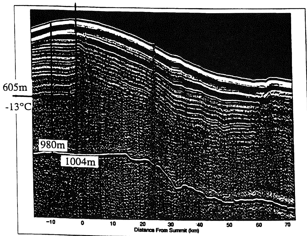
Figure 2: Radar profile across Siple Dome showing surface and bed characteristics and internal reflecting horizons. South is to the right and north is to the left [modified after Raymond et al. 1995]. The 1997/98 hot water drilling and coring sites, and the depth and temperature at which strong internal layering begins to fade are also indicated.
