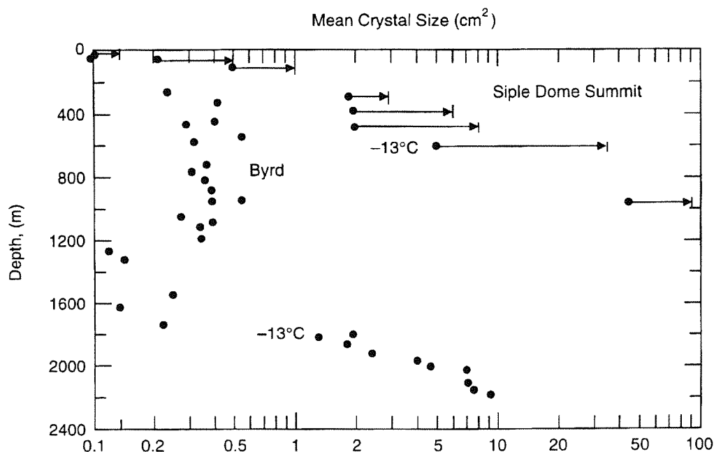
Figure 6: Comparative plots of crystal size versus depth in cores from Siple Dome Summit site and Byrd Station. Note abrupt increase in size of crystals, beginning at \sim 13^{\circ}\text{C} at both locations. Size of largest crystal observed at each depth indicated by arrowhead.
