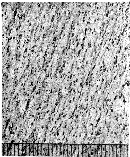
Figure 5 (continue): Air bubble characteristics and fracture patterns in ice cores from Siple Dome. Note bubbles intersected by cracks at 401 m, widespread fracturing at 605 m and cracking parallel to basal glide planes in a single crystal of very coarse-grained ice from 989 m. Scale in millimeters.
