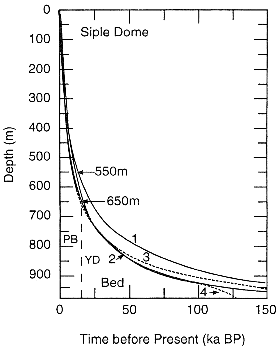
Figure 9: Age estimate modeling of the Siple Dome ice sheet after Nereson et al. [1996]. Depths to the Holocene/Younger Dryas transition (~11,600 yrs) for age-depth variants 1 and 2, derived from finite element modeling, are also indicated.
