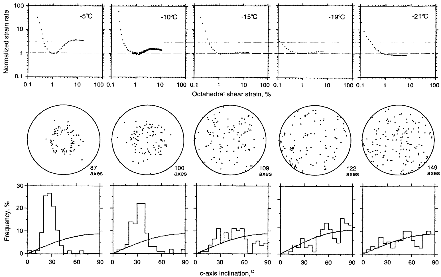
Figure 9: Creep curves (showing a "normalized" strain rate scale for comparison purposes) and fabric data for the series of tests at 0.2 MPa over the temperature range -5.0 to -21.0 °C.
