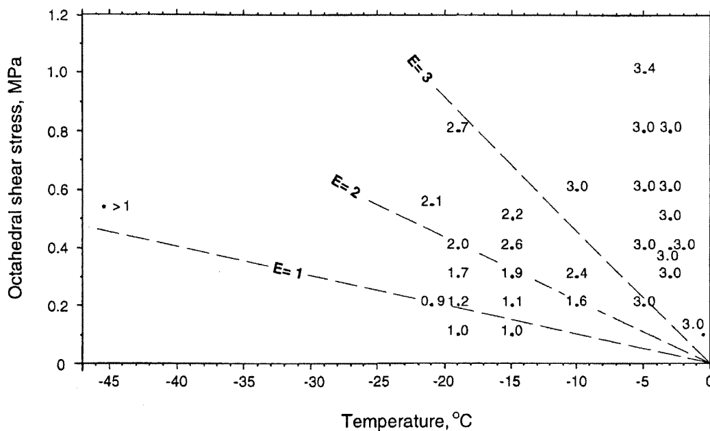
Figure 12: Map of enhancement factor, E plotted as a function of octahedral shear stress and temperature. Dashed lines are contours of E = 1, 2 and 3 . The E = 1 line has been extended to -45^{\circ}\text{C} , where the 0.55 MPa test shows E values >1 . Additional E = 3.0 data have been added from previous studies [1, 2].
