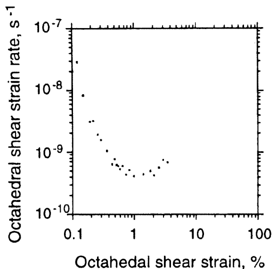
Figure 11: Creep curve for a re-test at 0.55 MPa and -45^{\circ}\text{C} on the same sample as shown in Fig. 10.
