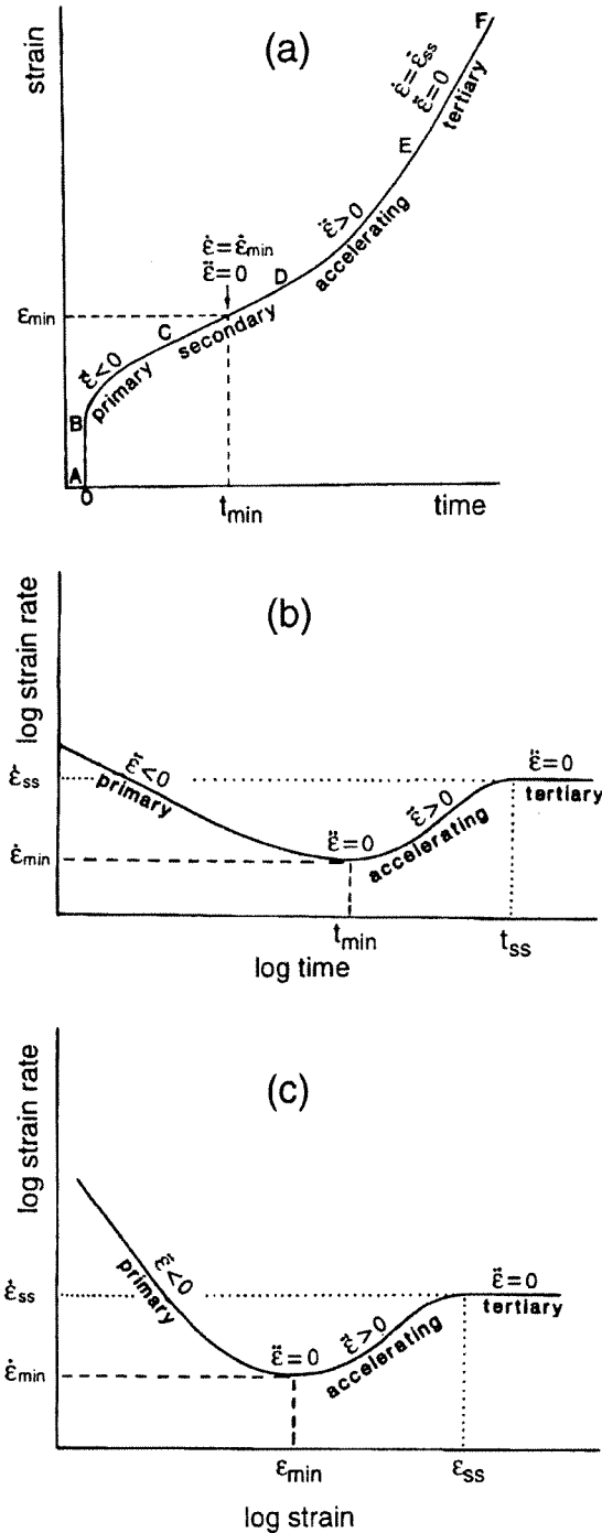
Figure 1: (a) An idealized creep curve for ice shows the various stages of strain, \epsilon versus time, t as follows: A-B: the initial impulsive elastic strain, B-C, C-D, D-E, and E-F the primary, secondary, accelerating and tertiary stages. (b) The corresponding log strain rate versus log time plot is shown indicating the minimum and "steady state" tertiary strain rates. (c) The corresponding log strain rate versus log strain plot shows the same features (after Budd and Jacka [1]).
