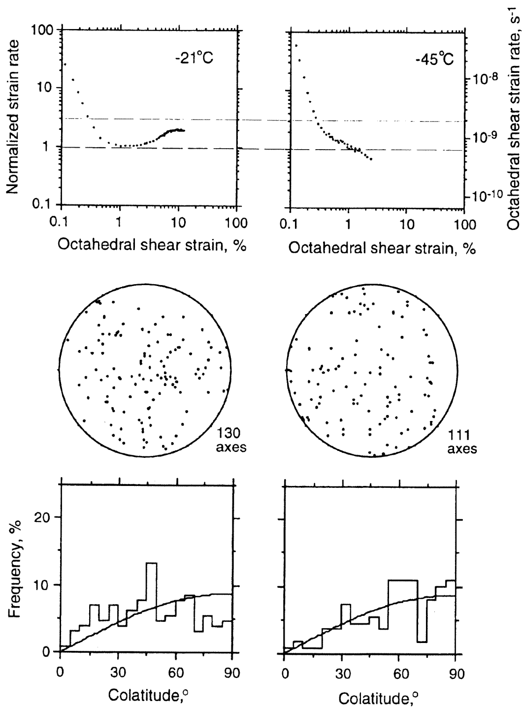
Figure 10: Creep curves and fabric data for tests at 0.55 MPa and temperatures of -21 and -45^{\circ}\text{C} . The strain rate scale on the right hand axis applies to the -45^{\circ}\text{C} test only, and is for comparison with Fig. 11.
