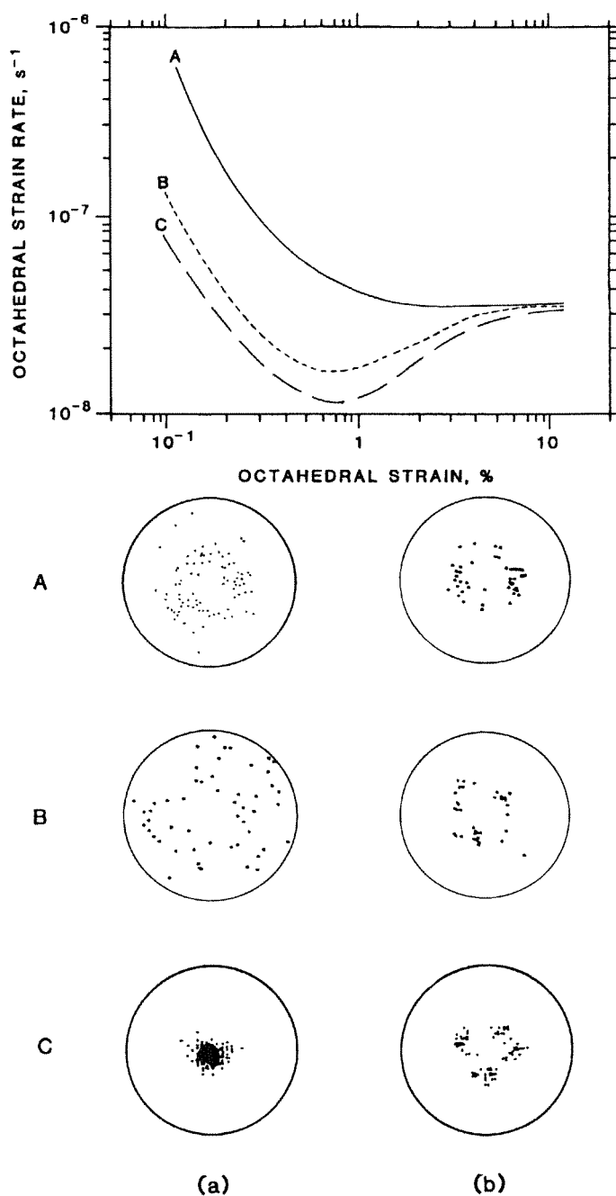
Figure 5: Creep curves for three deformation tests in uniaxial compression at -3.3^{\circ}C and 0.2 MPa. Curve A: initially anisotropic ice exhibiting a small circle girdle orientation fabric; Curve B: initially isotropic ice; and Curve C: initially anisotropic ice exhibiting a single maximum fabric pattern. Curve A illustrates easy glide in compression; Curve C illustrates hard glide (at the minimum strain rate) in compression. Crystal orientation fabrics exhibited (a) prior to testing and (b) at test completion are also shown. Note that in all cases the final (steady state) crystal fabric pattern (at this stress and temperature) was a small circle girdle (after Jacka and Budd [20]).
