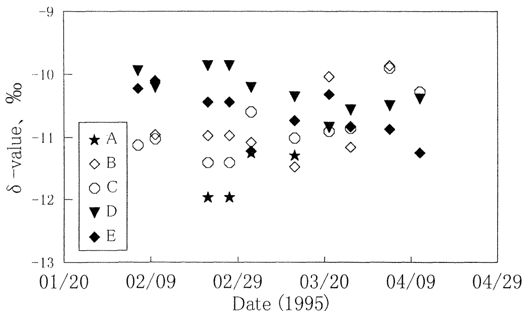
Figure 5: Temporal change of \delta^{18}\text{O} for each snow layer. \delta^{18}\text{O} increases with time in shallow layers (A, B and C) but decreases in deeper layers (D and E).
