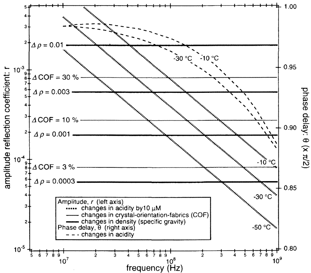
Figure 10: A relation between the complex reflection coefficients ( r^* = r \exp(i\theta) ) and changes in the complex permittivity in the ice sheet. Calculations are carried out for the three major causes: changes in crystal orientation fabrics, changes in acidity, and changes in density. For reflections due to changes in acidity, the phase delay (right axis) is close to \pi/2 . But it decreases with increasing frequency. For changes in the crystal orientation fabrics and changes in density, the phase delay is virtually zero.
