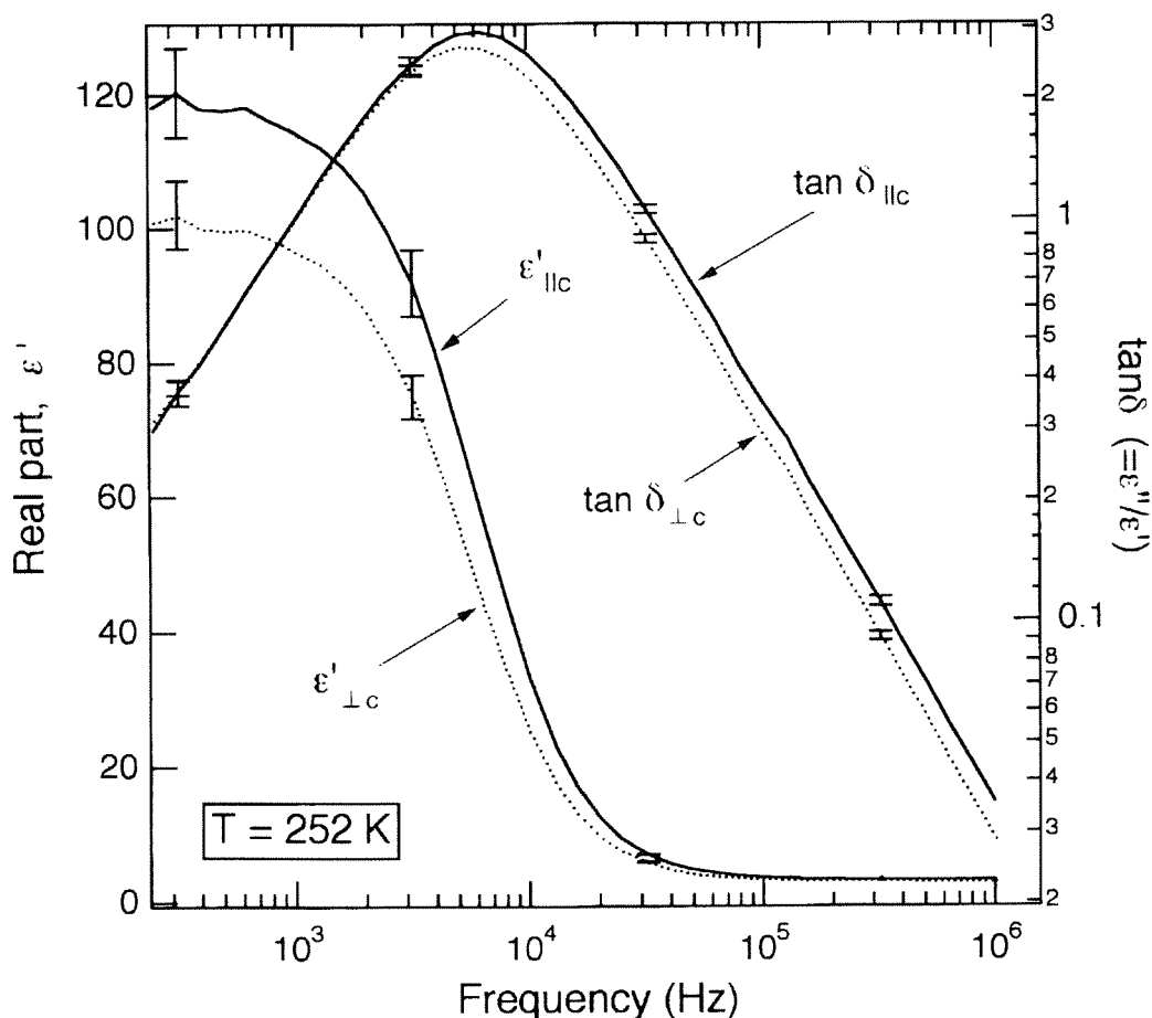
Figure 2: The complex permittivity of a single crystal from Mendenhall Glacier, Alaska. Temperature was 252 K and the frequency range was between 200 Hz and 1 MHz. Two components, the permittivity parallel to the c-axis, \epsilon'_{||c} , and the permittivity perpendicular to the c-axis, \epsilon'_{\perp c} , were independently measured 10 times. Mean values and standard deviations are indicated in the figure. The static permittivity has anisotropy close to 20% ( \epsilon'_{||c} > \epsilon'_{\perp c} ). It decreases with increasing frequency to the high-frequency limit value. For the real part at 10^5 – 10^6 Hz, the figure on an expanded scale is shown in Figure 3. For the loss tangent ( =\epsilon''/\epsilon' ), anisotropy was about 20 % ( \tan \delta_{||c} > \tan \delta_{\perp c} ) in the frequency range well above the Debye dispersion. Note that the data of loss tangent contains a systematic error at frequencies lower than about 2 \cdot 10^4 Hz by a system problem which is not solved yet. Therefore, we cannot assess the relaxation frequencies from the data of loss tangent.
