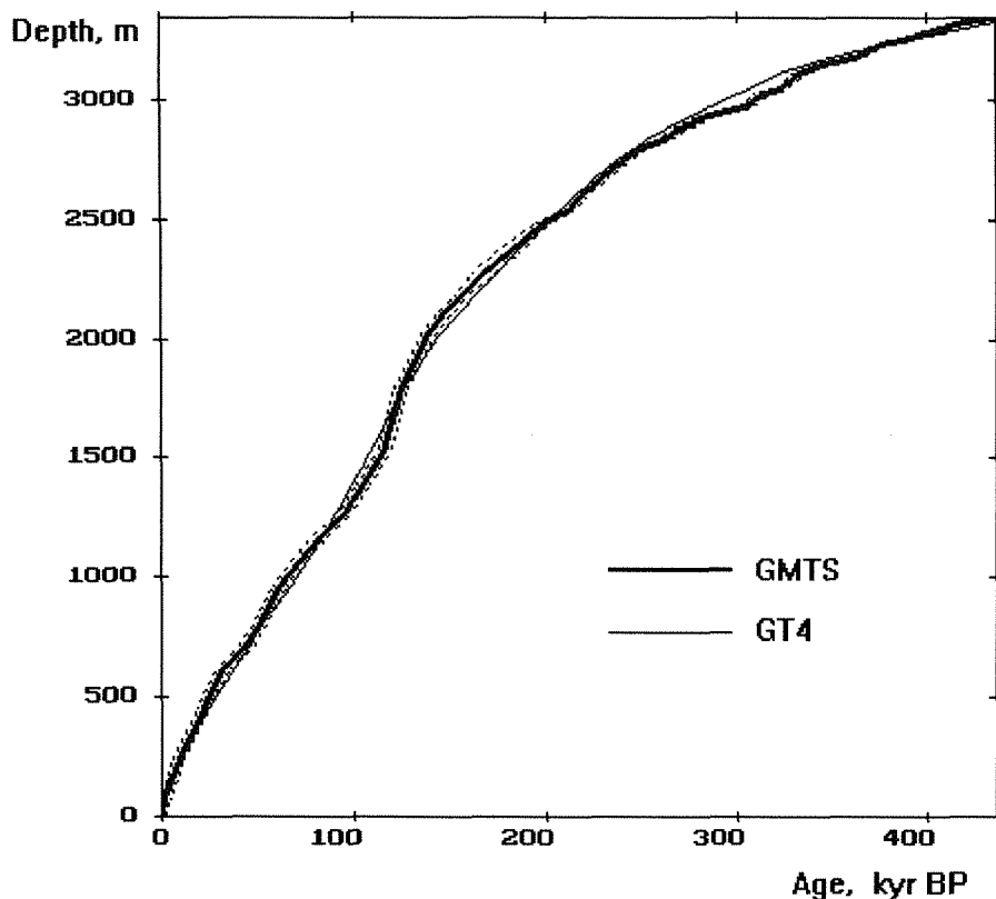
Figure 5: Age-depth relation for the Vostok ice core (GMTS) deduced from the analysis of the borehole temperature profile and its comparison with the glaciological timescale (GT4) developed on the basis of ice sheet flow modelling [59]. The error blanket indicates overall uncertainties of the GMTS chronology.
