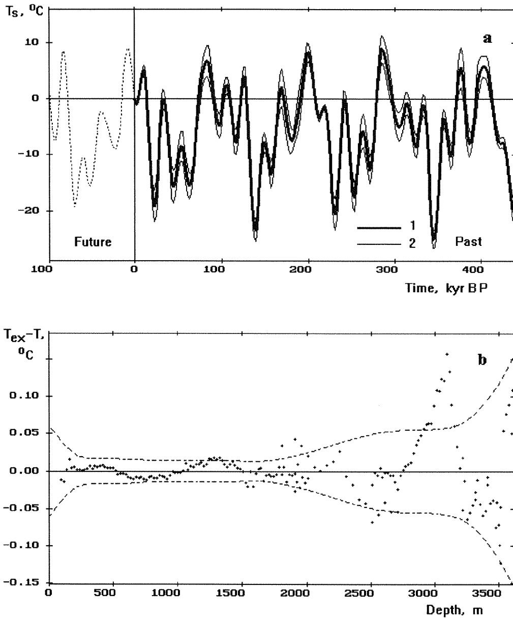
Figure 3: (a) Metronomic signal in the Vostok surface temperature variations (curve 1) inferred from the stacked borehole temperature profile and extrapolated into the future (dotted line) in the case I with the shear deformation and strain heating in the 3540-meter stratum of the ice sheet overlying the immovable ice. Curves 2 show the standard deviations of the reconstruction estimated by Monte Carlo sampling. (b) Mismatch between the observed and computed (best-fit) temperature profiles within the ice-sheet thickness (dots). The dashed curves are the standard deviation bounds of the simulations which correspond to the target norm S \approx 0.014^{\circ}\text{C} .
