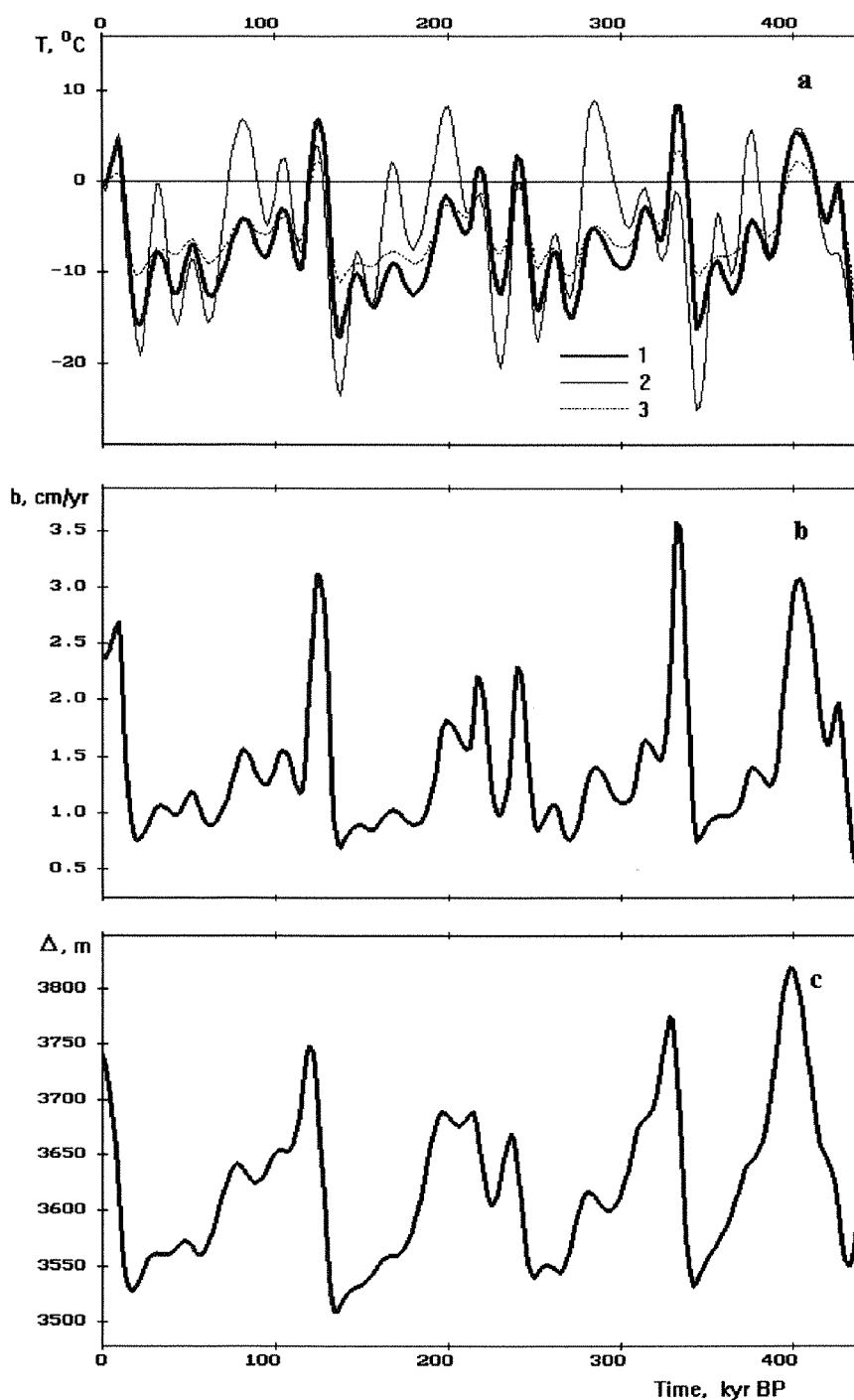
Figure 6: Time series of paleoenvironmental characteristics reconstructed from the smoothed Vostok isotope record for case I with the shear deformation and strain heating in the 3540-meter stratum of the ice sheet overlying the immovable ice. (a) Temperature variations on the ice sheet surface (curve 1) and inversion temperature oscillations (curve 3) counted from their present-day reference levels in comparison with the Milankovich metronomic signal (curve 2). (b) Accumulation rate variations calculated from inversion temperatures. (c) Past changes in the ice-sheet thickness simulated at Vostok.
