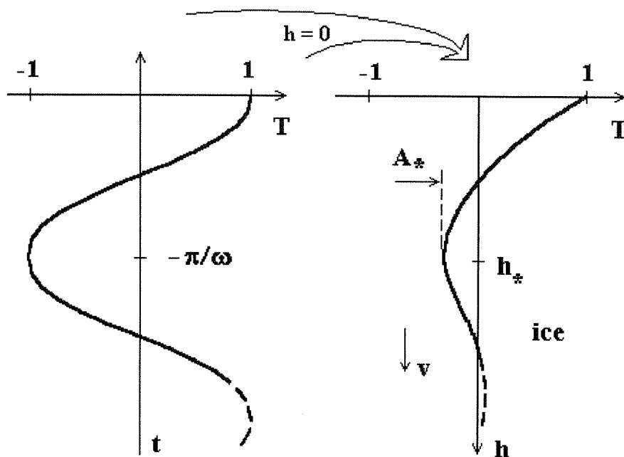
Figure 2: The thermal-wave propagation induced in moving ice by the cosine temperature fluctuations on the ice surface ( h = 0 ). The most recent peak (or trough) in the surface-temperature variations can be distinguished at the present time with the amplitude A_* at depth h_* .
