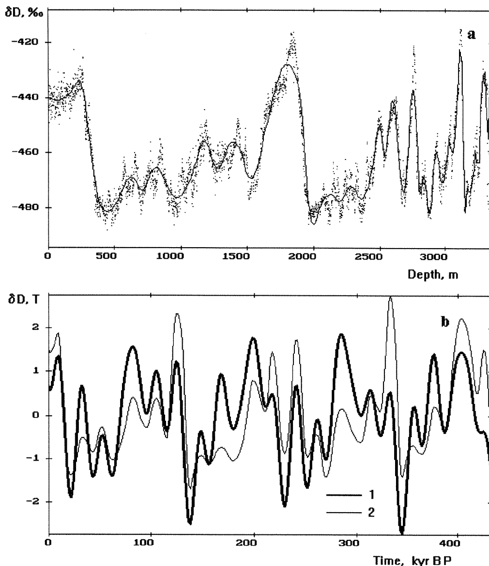
Figure 4: (a) Vostok deuterium ice core record (dots) and its parabolic-spline approximation (solid line) used in the ice-core age dating procedure. (b) The smoothed isotope record (curve 2) correlated with the metronome (curve 1) from Fig. 3a (both curves are normalized).
