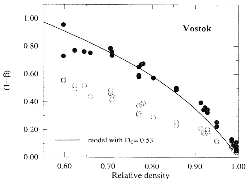
Figure 6: Fraction of free surface area of grain (●) and aggregate (○) versus relative density for Vostok (Bh7). Model curves with D_0 = 0.53 .
