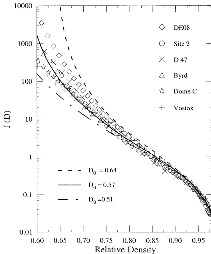
Figure 2: Experimental function f versus relative density for six sites from Greenland and Antarctica (Table 1). The theoretical curves giving the variation of f(D) with density were obtained for three values of D_0 .
