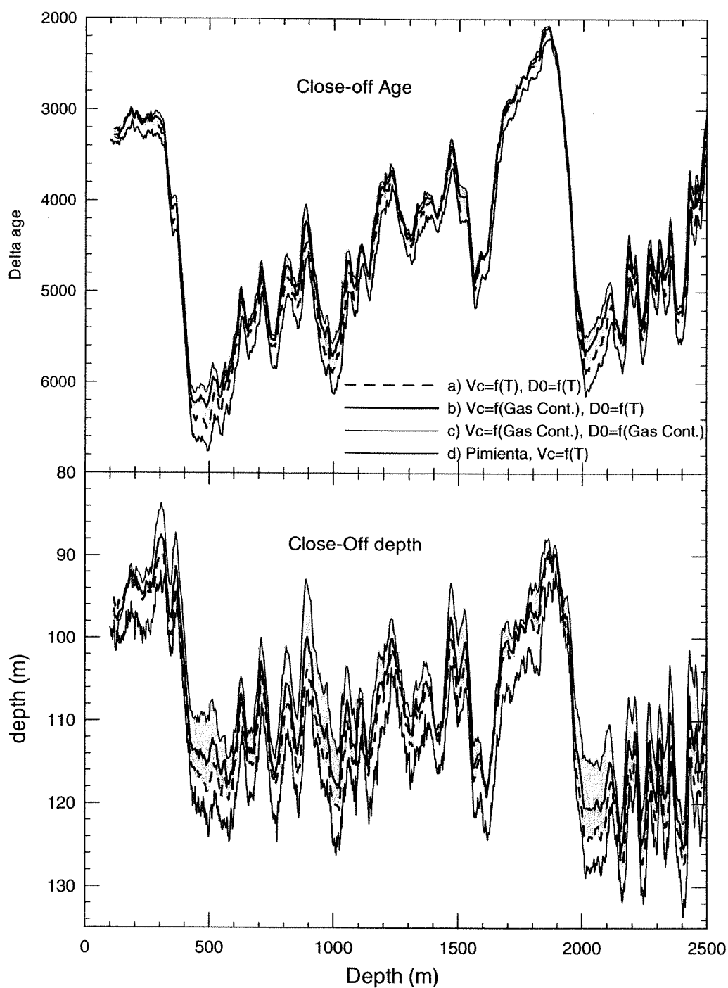
Figure 7: Close-off age (upper panel) and depth (lower panel) reconstructed for the first 2500m of the Vostok core. a, b and c curves correspond to different assumptions in the geometrical model (see text) and d to the Pimienta model. (See color plate 9.)
