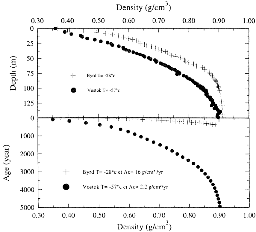
Figure 1: Depth-density (1.a) and time-density (1.b) profiles for two sites: Vostok and Byrd.
