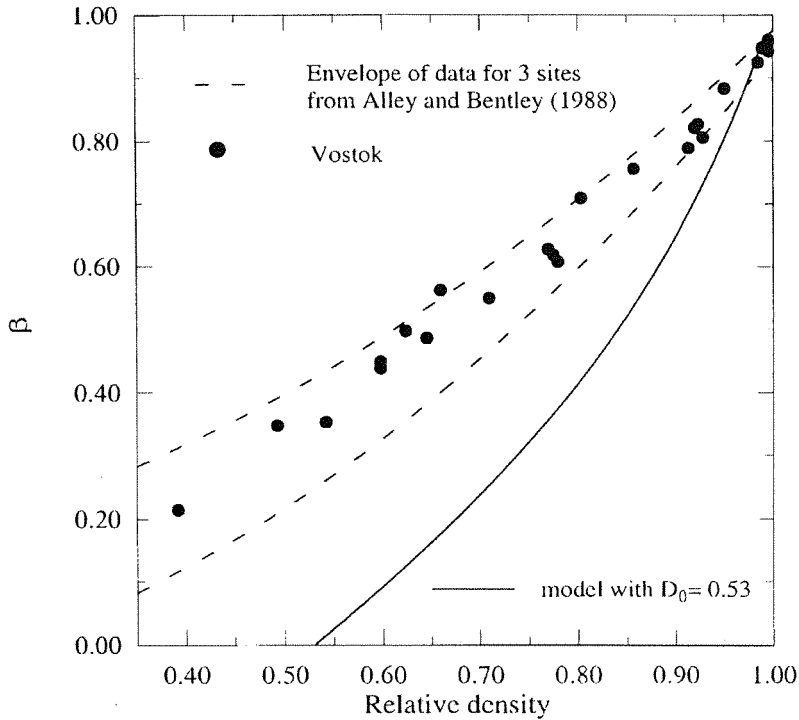
Figure 5: Average fraction of the surface of crystals involved in bonds ( \beta ) for Vostok, and envelopes of the data from three other sites from Alley and Bentley [1988]. Model curves with D_0 = 0.53 .
