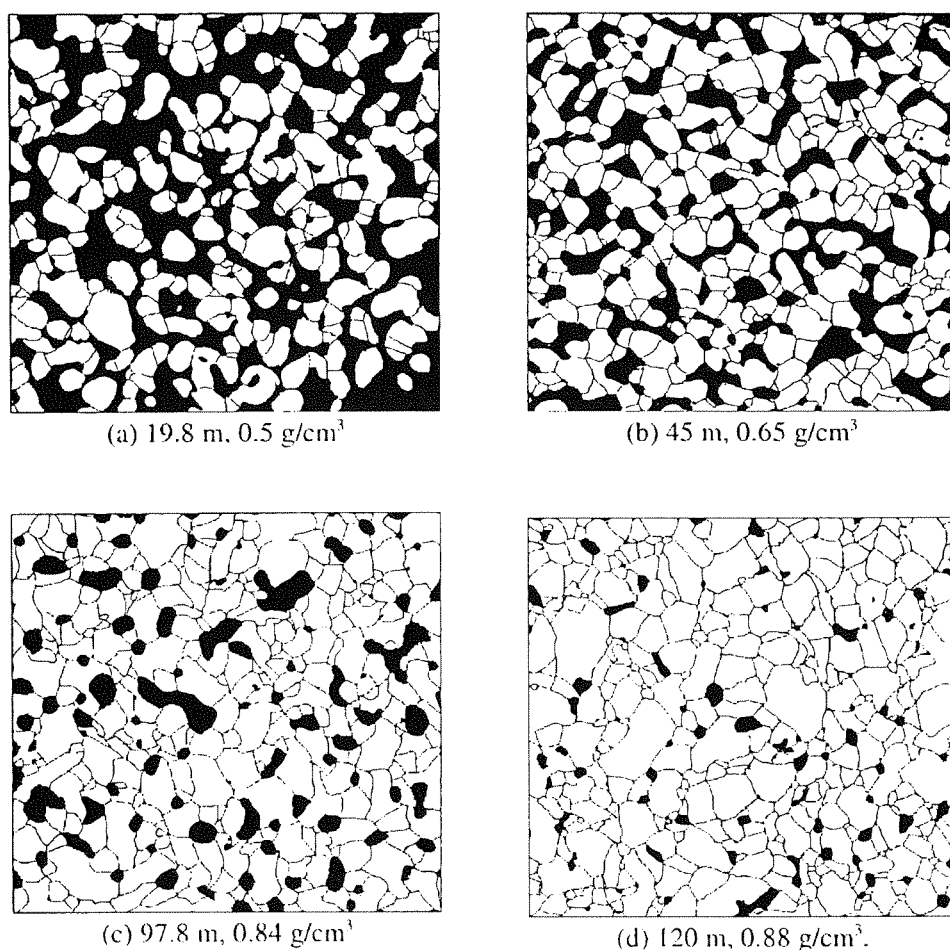
Figure 4: Binary images obtained by image processing of photographs obtained in reflected light from sections of the Vostok core. (a) 19.8 m, 0.5 g/cm 3 ; (b) 45m, 0.65 g/cm 3 ; (c) 97.8 m, 0.84 g/cm 3 ; (d) 120 m 0.88 g/cm 3 .
