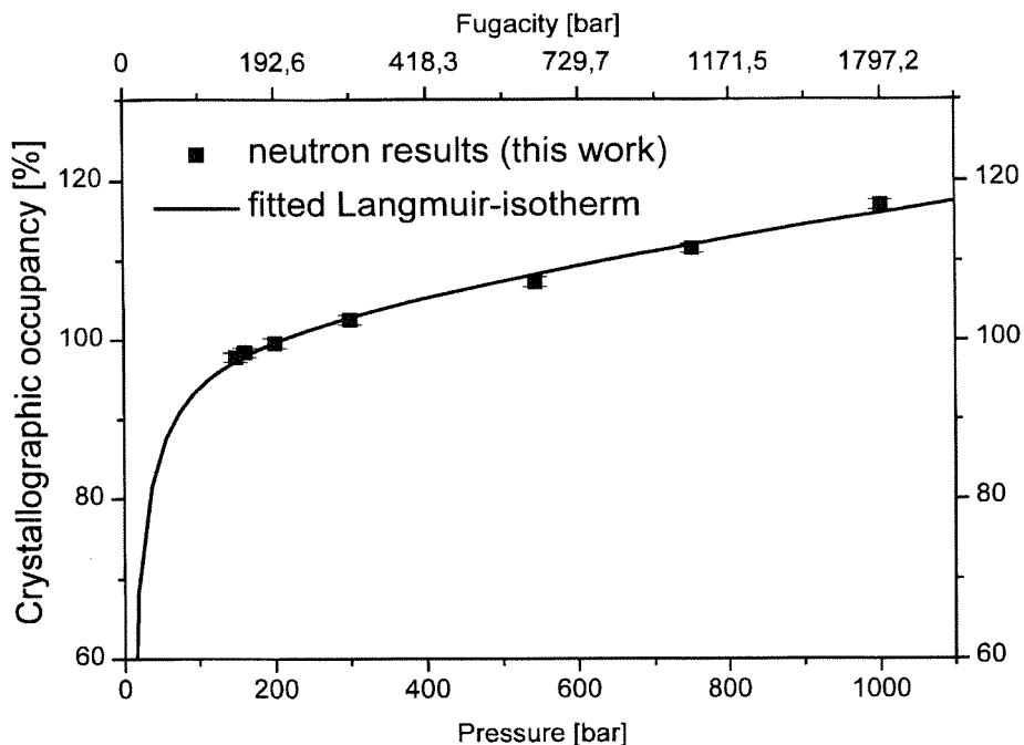
Figure 6: Filling of the large cages of N_2 clathrate vs. fugacity and pressure together with a fitted isotherm using a two constant model [24] with C_{LC,single} = 205(44) \text{ kbar}^{-1} and C_{LC,double} = 0.125(6) \text{ kbar}^{-1} .
