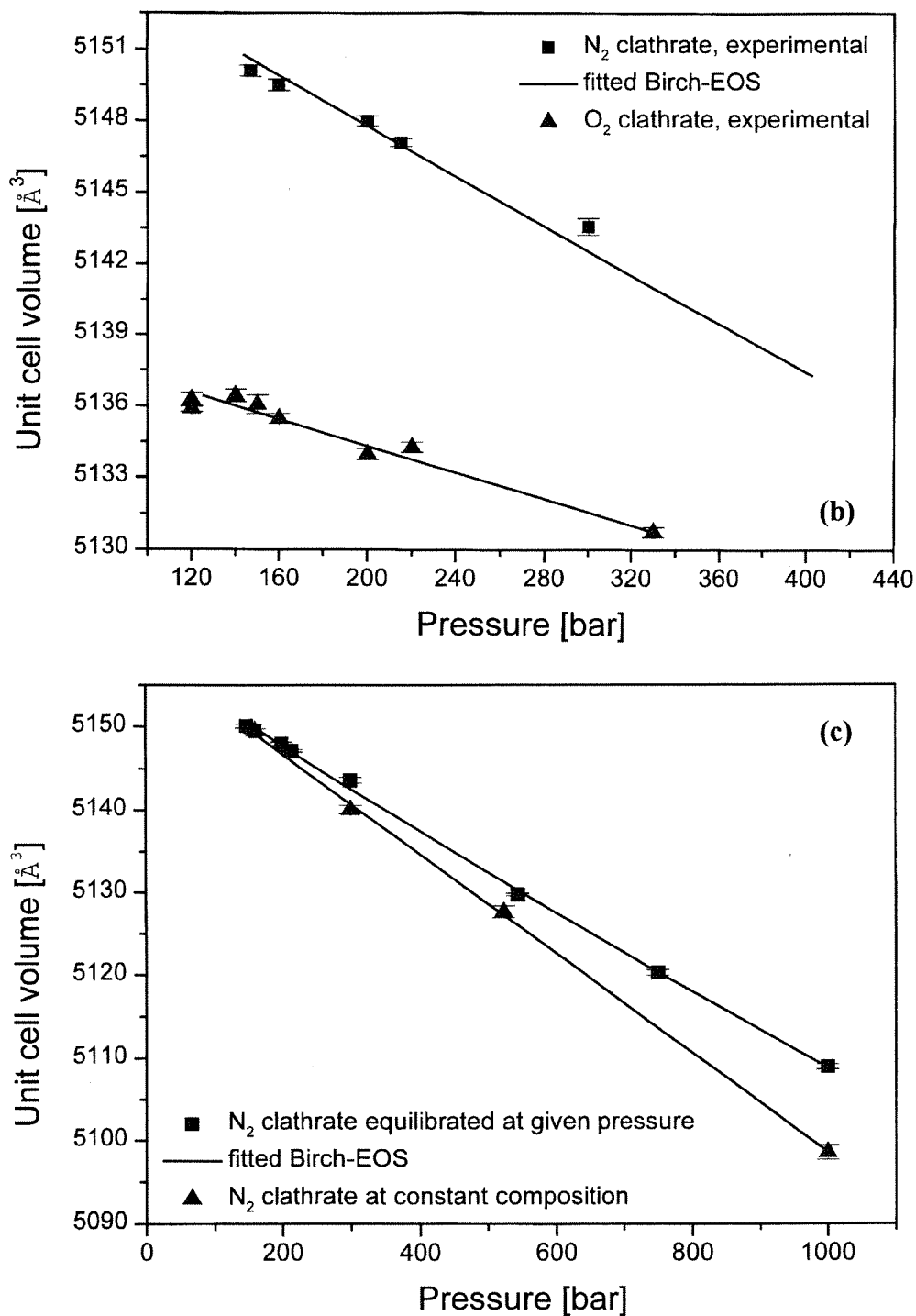
Figure 8: Lattice constants and unit cell volume of \text{N}_2 , \text{O}_2 and air clathrate hydrates vs. pressure. (a) Cubic lattice constants vs. pressure. (b) Unit cell volume and fitted Birch equation-of-state at low pressure. (c) isosteric and isothermal unit cell volumes and fitted equation-of-states. For a discussion see text.
