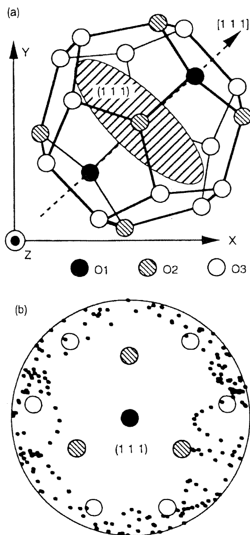
Figure 4: Stereographic projection of nitrogen molecule orientations in a small cage at 50 K. Oxygen atoms of host water molecules, designed O1, O2 and O3, form the 12-hedral small cage. The dashed arrow in Fig. 4a (denoted as [111]) indicates the compressed axis of the small cage, which corresponds to the axis normal to the page and located at the center of Fig. 4b. (From Horikawa et al. [35].)
