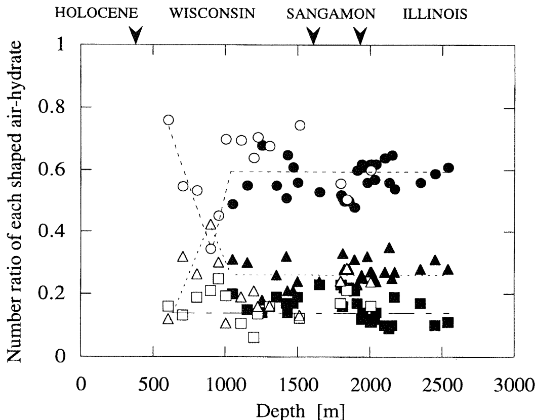
Figure 15: Variations of the stratigraphies of air hydrate crystals in Vostok ice cores. Spherical crystal: N_s/N (circle), irregular: N_i/N (square), and faceted: N_f/N (triangle) for two series of ice cores (open and solid marks). (From Uchida et al. [7].)
