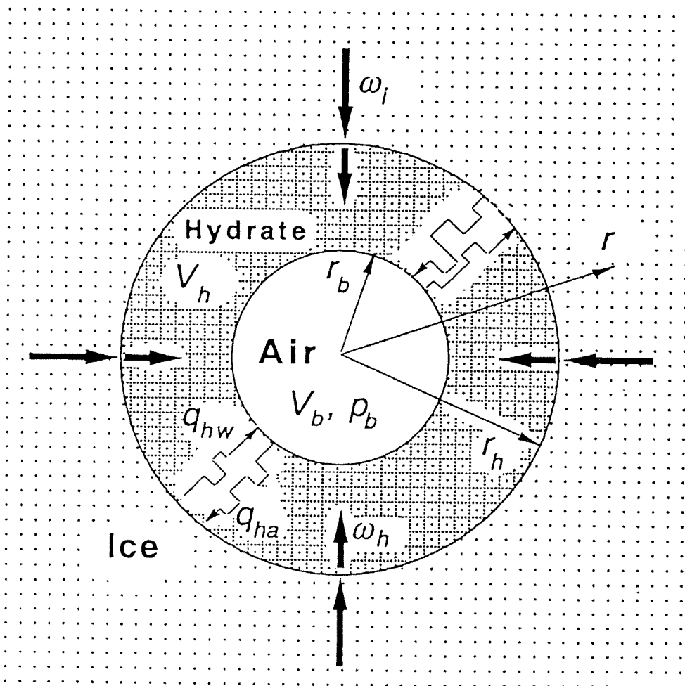
Figure 14: A hydrate growth model that includes molecular diffusion and assumes a spherical bubble with a hydrate shell. Here r_b is the bubble radius, r_h is the external radius of the air hydrate shell. \omega_h and \omega_i denotes the volume deformation rate of the hydrate shell and of the surrounding ice, respectively. q_{ha} and q_{hw} are the mass fluxes through the spherical hydrate shell of air and water, respectively. (From Salamatina et al. [2].)
