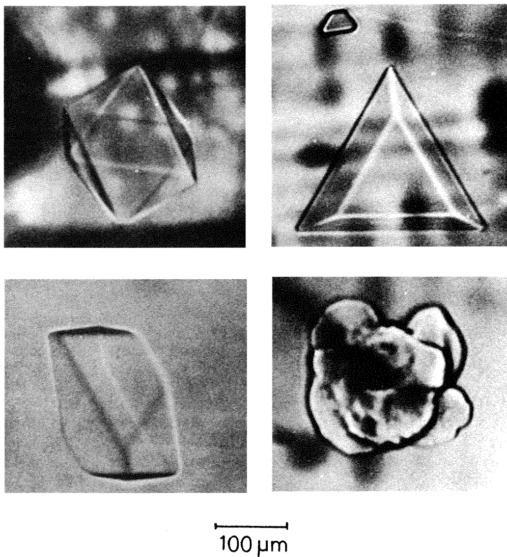
Figure 1: Various air hydrates observed in an ice core from Dye-3, Greenland (From Nakahara et al. [23]).
