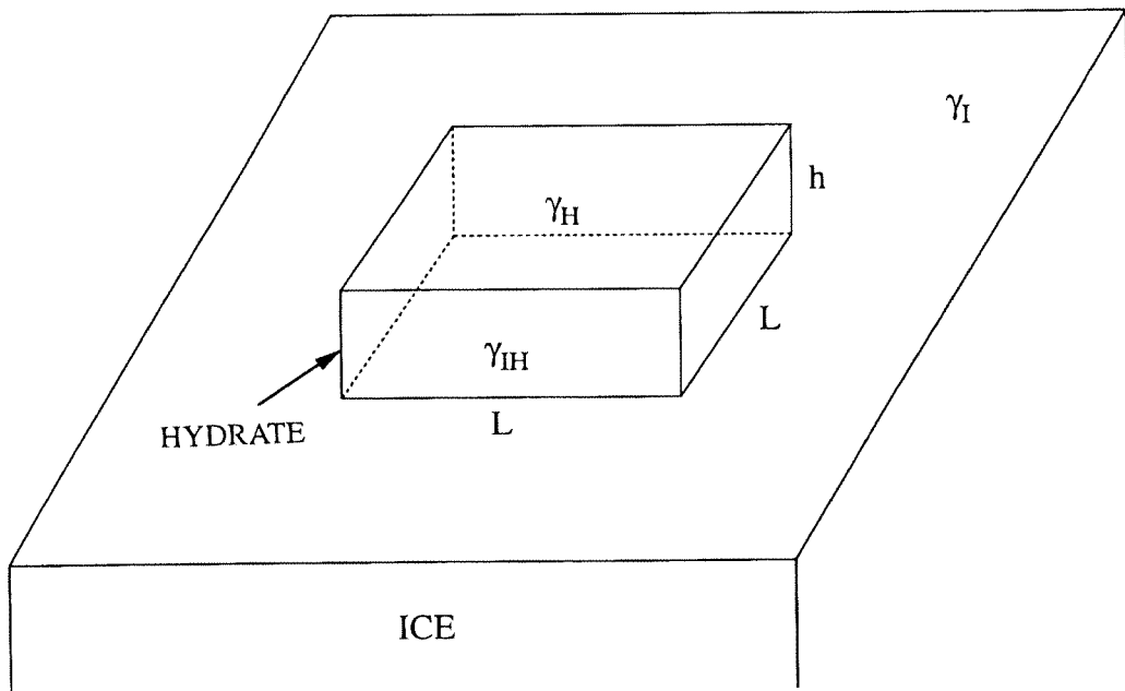
Figure 10: Illustration of the concept of hydrate nucleation on an ice surface [17]. The rectangular nucleus nucleated homogeneously on the smooth ice surface.
