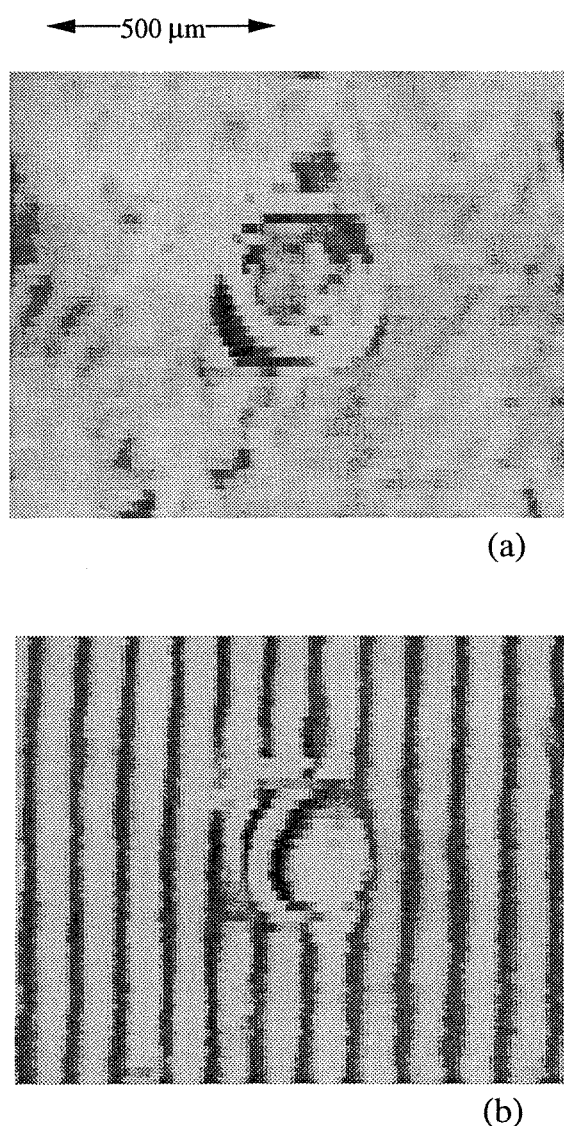
Figure 6: Images of an air-hydrate crystal with (a) schlieren system (sharpen the boundary between ice and hydrate) and (b) Mach-Zehnder interferometer (the relative shift in the fringe is proportional to the difference in refractive indices and crystal thickness). (From Uchida et al. [38].)
