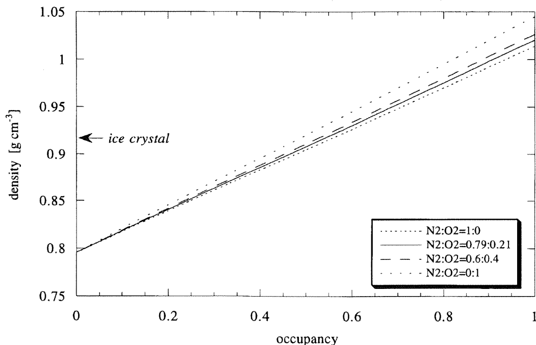
Figure 5: Calculated density of air hydrate crystals. Each line has a different gas composition shown in the legend. The lattice parameter is assumed to be 17.0 Å and the molecular weights of water, nitrogen, and oxygen are 18.025 g, 28.013 g, and 31.999 g, respectively [57].
