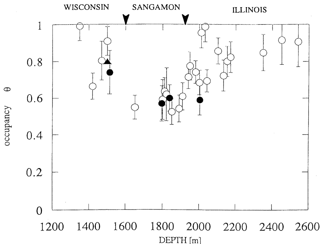
Figure 8: Variation of the cage occupancy \theta with depth in Vostok ice cores as estimated from the volume concentration of air hydrates and the total gas content (modified for ref. 7). Two series of ice cores were used (solid and open circles). The solid triangle denotes the cage occupancy obtained by the refractive index measurements [38].
