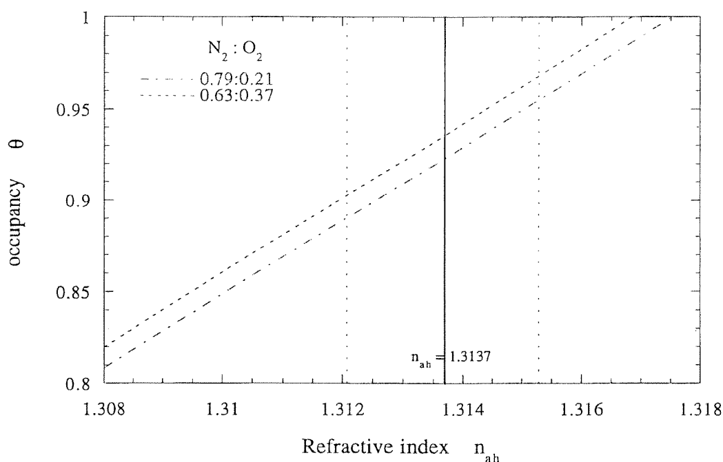
Figure 7: Relation between the cage occupancy and refractive index of air hydrate crystals. Two lines are calculated by the Onsager cavity model with the labeled air compositions. The measured refractive index (thick solid line: n_{\text{ah}} = 1.3137 ) is also shown together with the experimental errors as thin dotted lines. (From Uchida et al. [38].)
