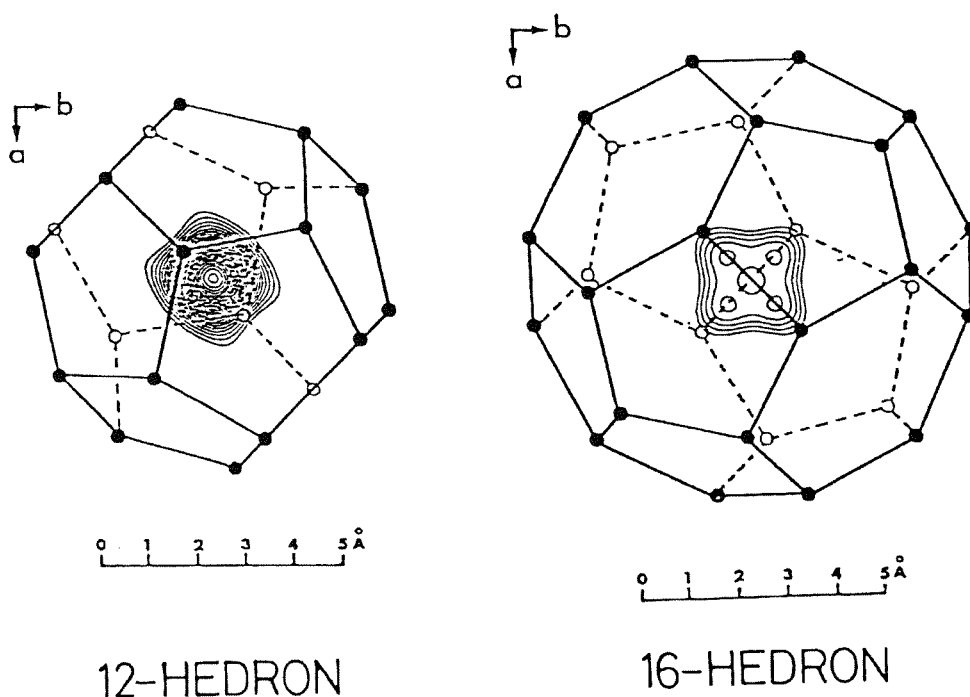
Figure 3: Distribution of air molecules in the cages. Electron density cross-sections through the center of the cages: (a) 12-hedron, (b) 16-hedron. Contours at 0.02 \text{ e} \cdot \text{\AA}^{-3} intervals. This figure shows that air molecules in small cages remain close to the center of the cage, whereas air molecules are too small to remain at the center of the large (16-hedron) cage. (From Hondoh et al. [13].)
