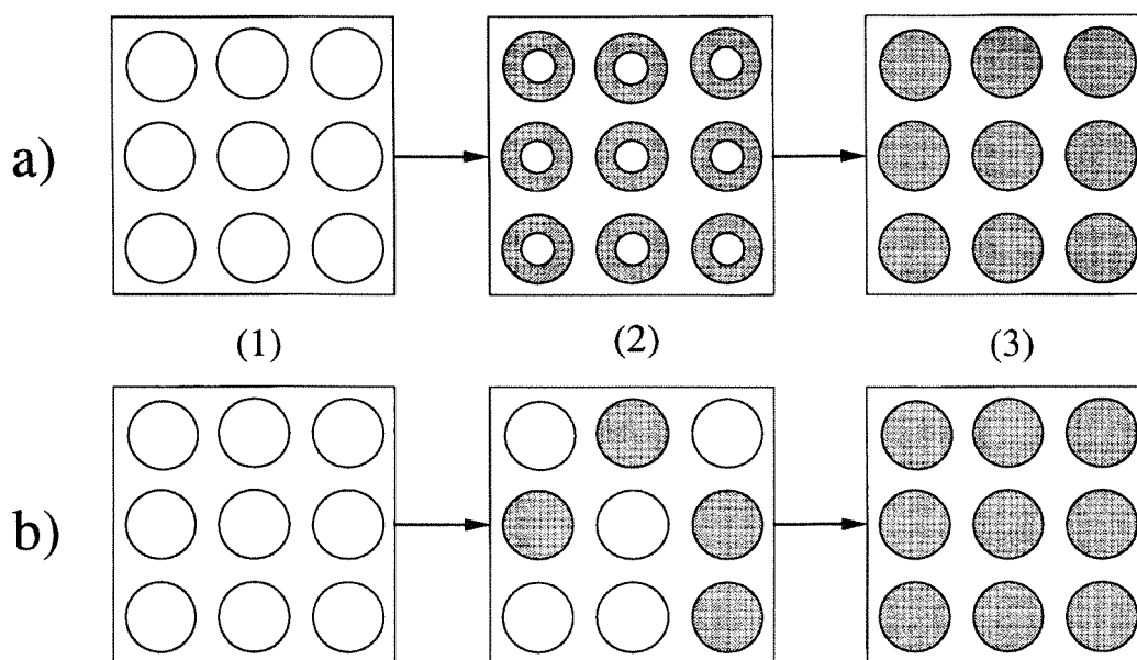
Figure 12: Illustration of the transformation process of air bubbles (open circles) to air hydrates (shaded part): a) the process controlled by water molecule diffusion [5], and b) the process controlled by hydrate nucleation [47].
