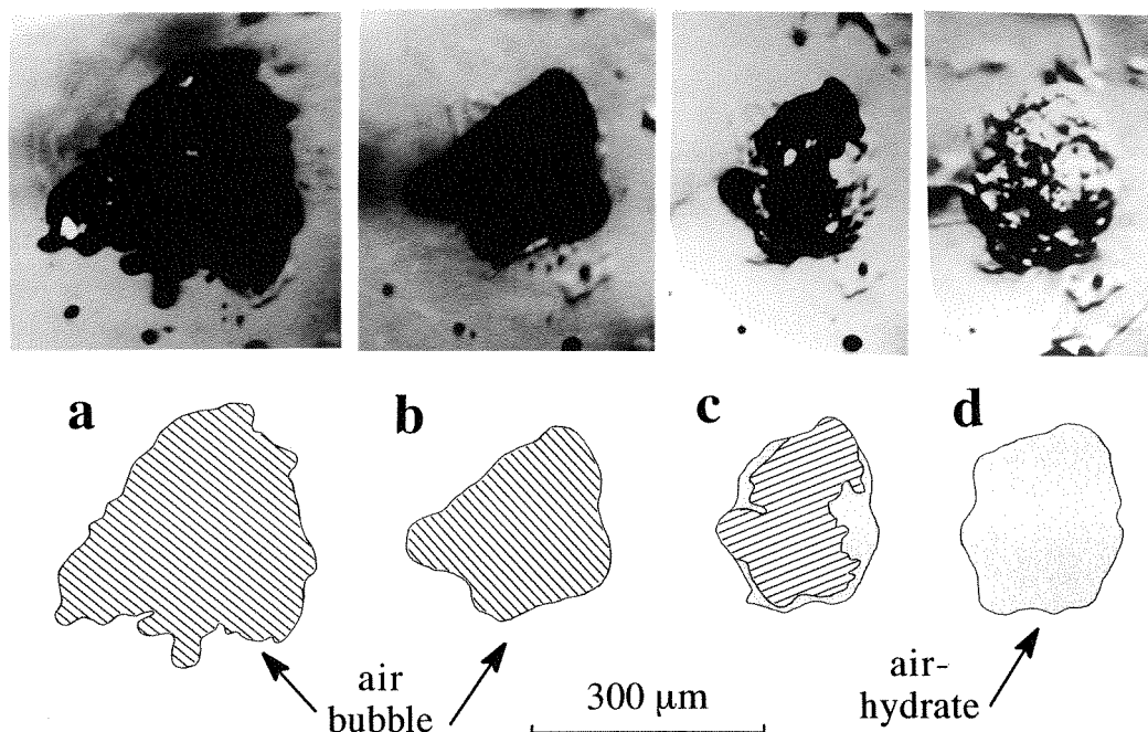
Figure 11: The transformation of an air bubble to hydrate crystal observed under the microscope with sketched outlines [46]. The total elapsed time is 164 hours.
