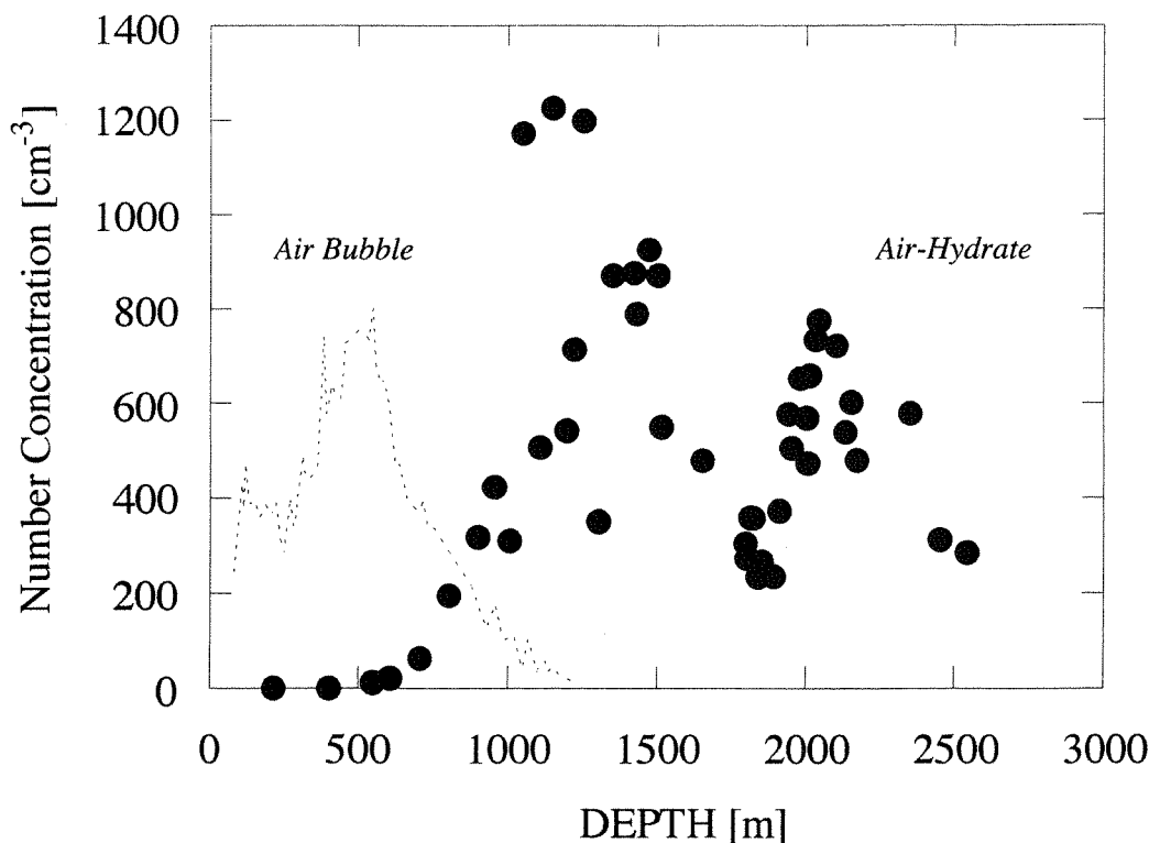
Figure 9: Depth variation of the number concentrations of both air bubbles (dotted line) and air hydrates (solid circles) in Vostok ice cores.
