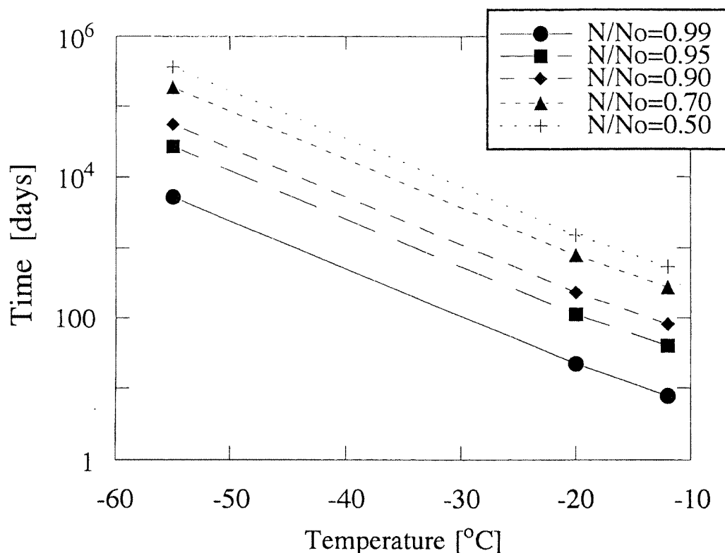
Figure 19: Calculation of the fraction ( N/N_0 ) of hydrates remaining in an ice core as a function of the storage temperature and time period. (From Uchida et al. [56].)
