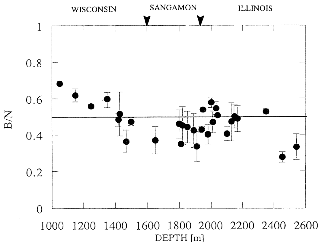
Figure 13: The probability ( B/N ) of a hydrate existing on a grain boundary in a Vostok ice core. (From Uchida et al.[42].)
