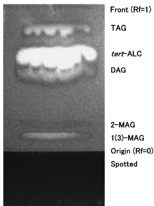
Fig. 1. Boric acid HPTLC profile of the partial hydrolysis products formed from 2 mg of cod liver/mackerel oil TAG.
