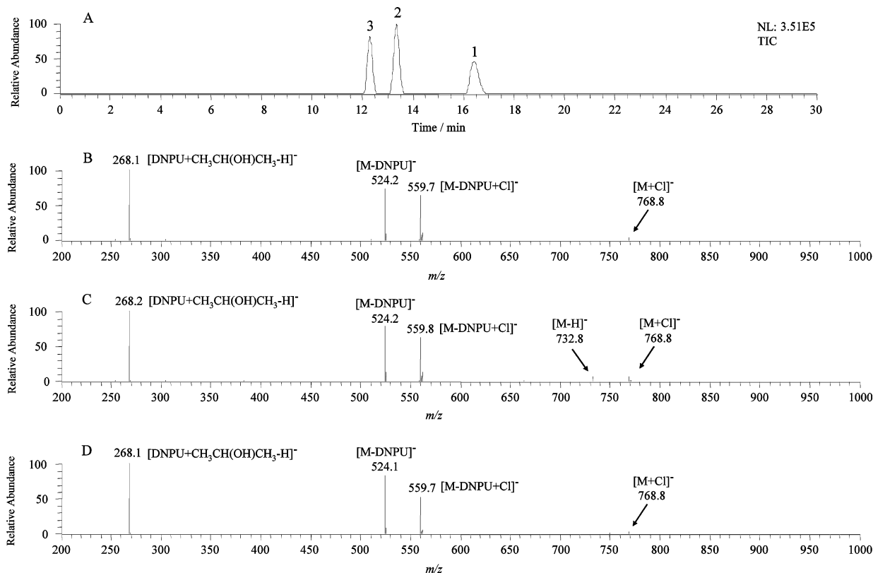
Fig. 3. Chiral-phase HPLC/APCI-MS profiles of the bis(3,5-dinitrophenylurethane) derivatives of enantiomeric and regioisomeric hexadecylglycerols. A, total ion chromatogram (TIC); B, mass spectra averaged over the peak 3 between 12.1 and 12.4 min on the TIC; C, mass spectra averaged over the peak 2 between 13.2 and 13.5 min on the TIC; D, mass spectra averaged over the peak 1 between 16.2 and 16.5 min on the TIC. Post-column solvent addition of 2-propanol was used to assure APCI in the negative mode. Column: OA-4600. Other HPLC conditions as given in text. APCI-MS conditions: capillary temp., 200°C; vaporizer temp., 450°C; source voltage, 6.0 kV; sheath gas ( N_2 ) flow-rate, 70 arb; capillary voltage, -38 V; tube lens offset, -60 V.
