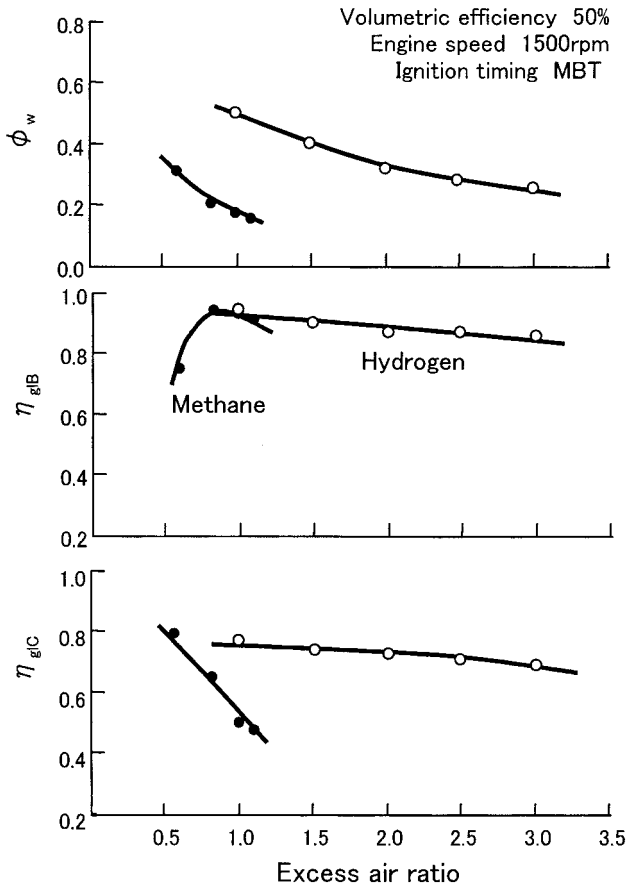
Fig. 11 Influence of the excess air ratio on \phi_w , \eta_{glb} and \eta_{glc} .
