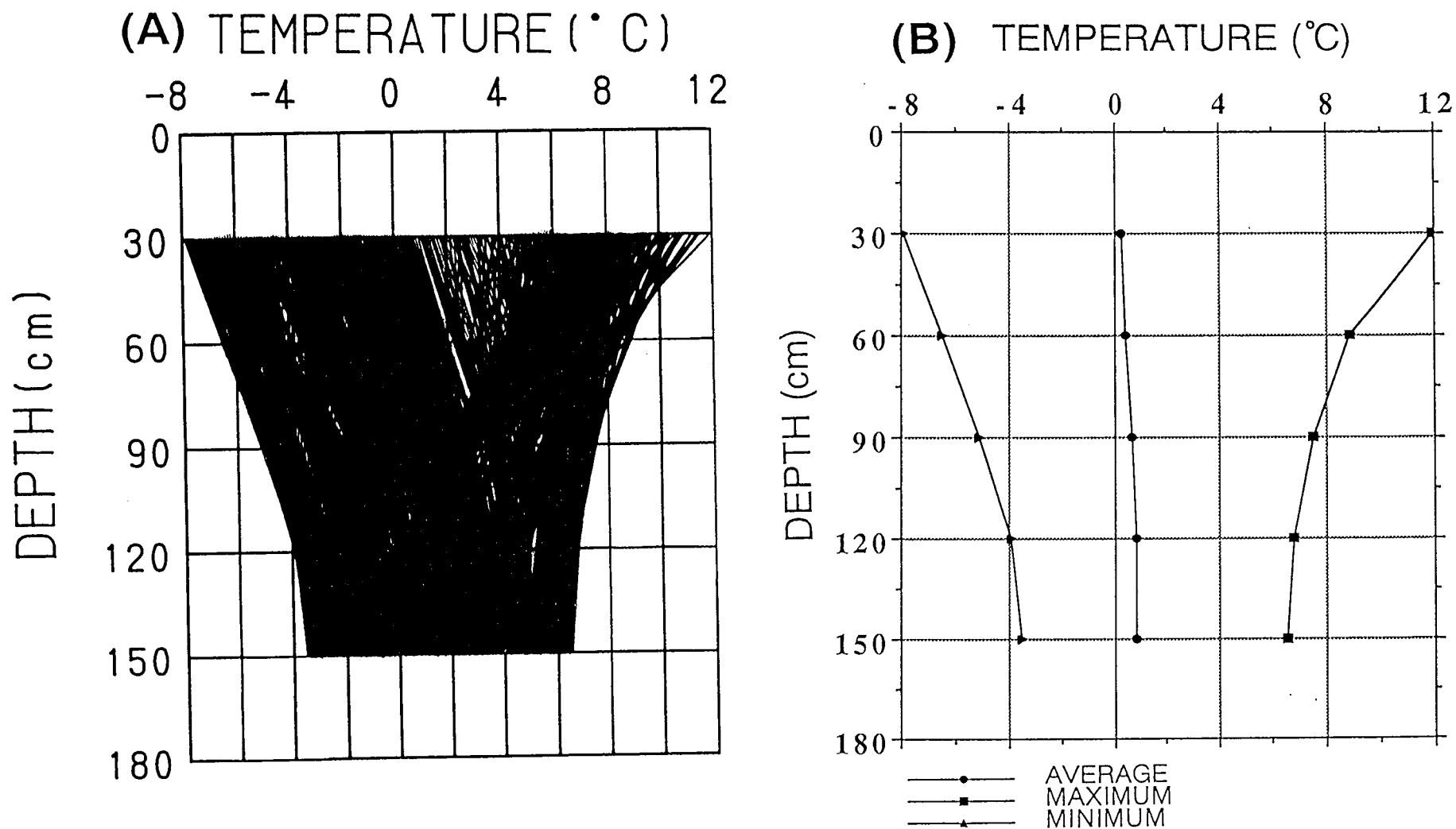
Figure 4.9. (A) The 3-hour ground temperature profiles in the forefields of the Yala Glacier (5090 m) from June 1990 to May 1991. (B) The maximum, minimum and average ground temperatures in the forefields of the Yala Glacier (5090 m) from June 1990 to May 1991.
