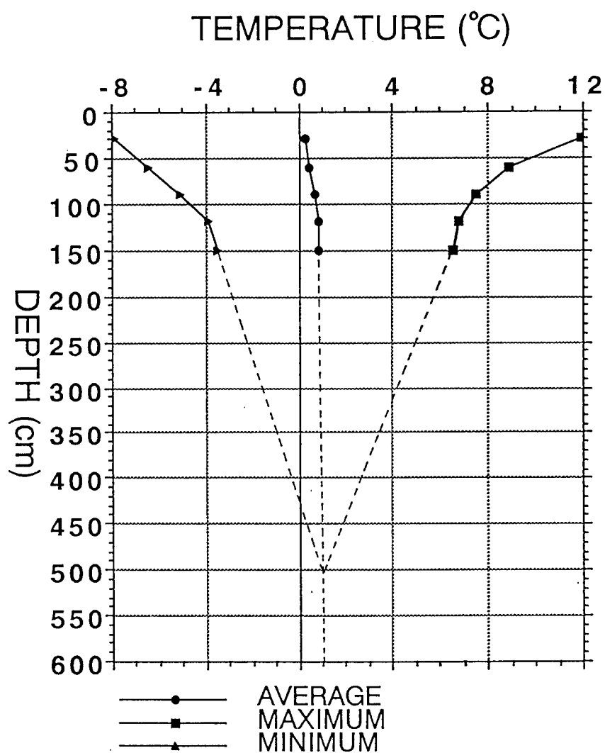
Figure 4.10. Thermal regime in the forefields of the Yala Glacier (5090 m).
