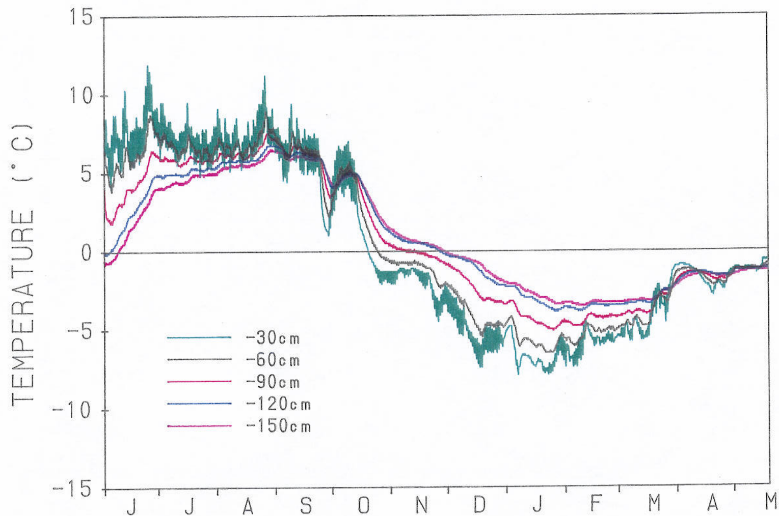
Figure 4.7. Changes in the 3-hour ground temperatures in the forefields of the Yala Glacier (5090 m; GC in Figure 4.2) from June 1990 to May 1991.
