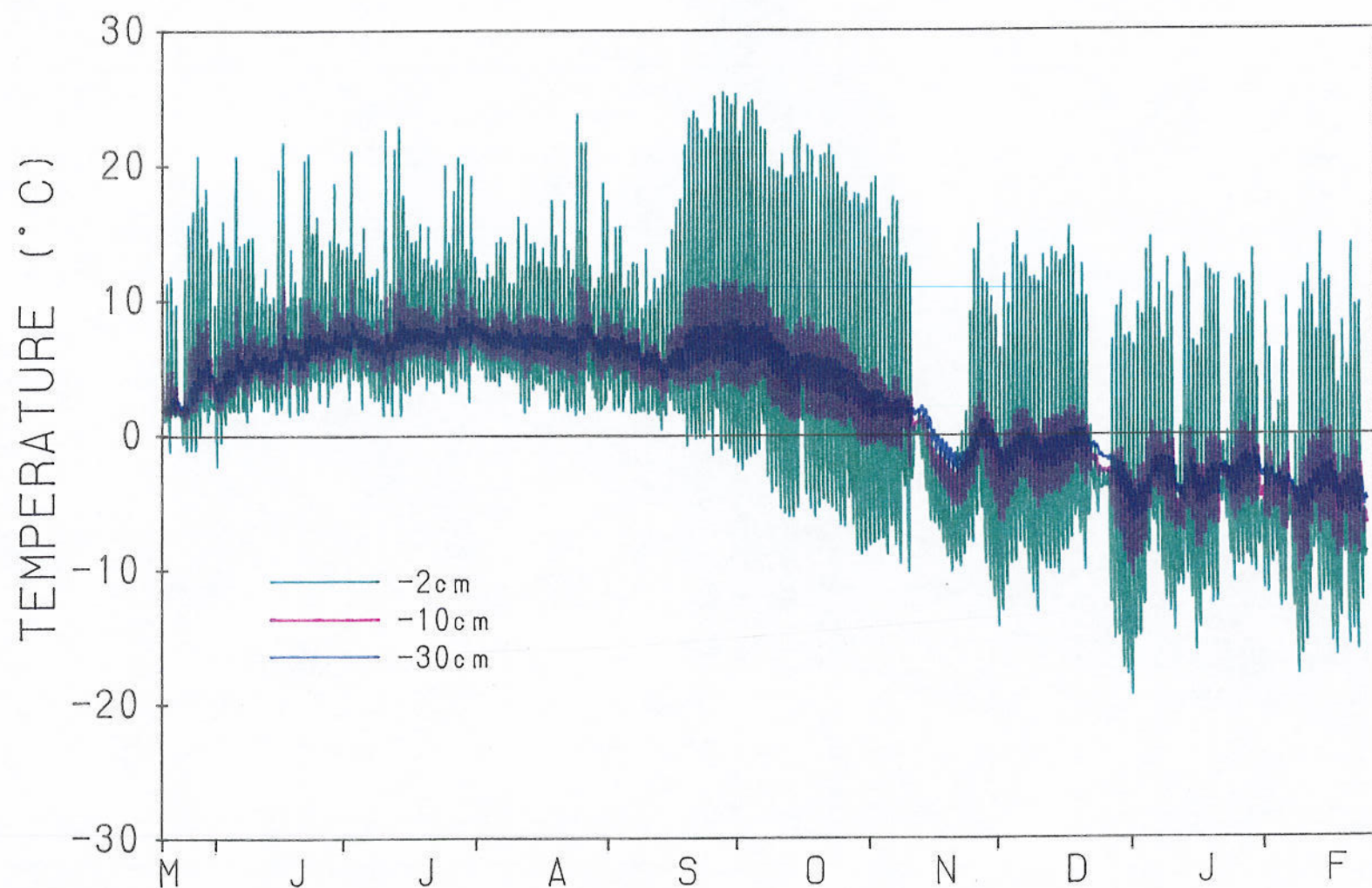
Figure 4.8. Changes in the hourly ground temperatures at Glacier Camp (5090 m) from May 1991 to February 1992.
