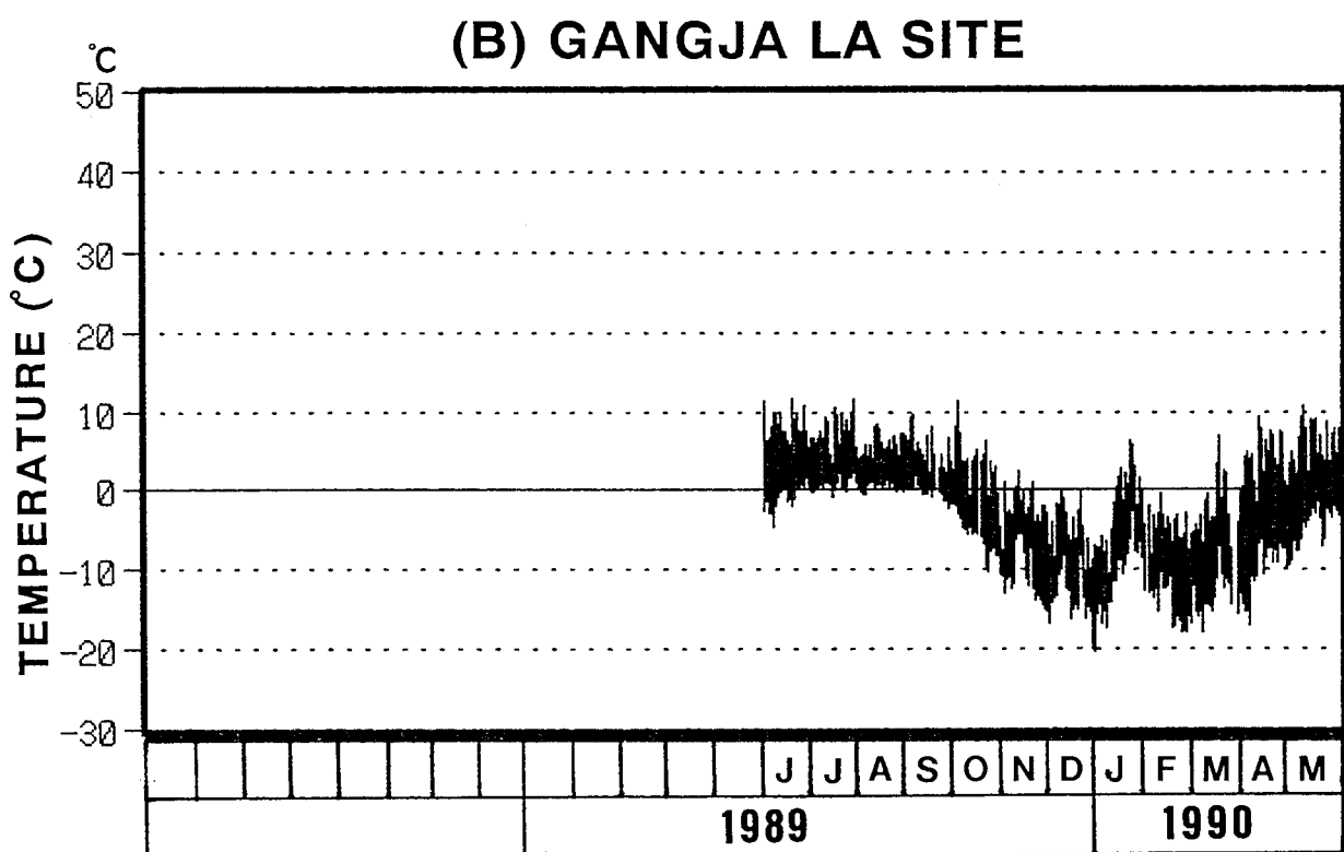
Figure 4.12. Diurnal ranges in air temperature. (A): Glacier Camp (5090 m), and (B): Gangja La (5090 m).
