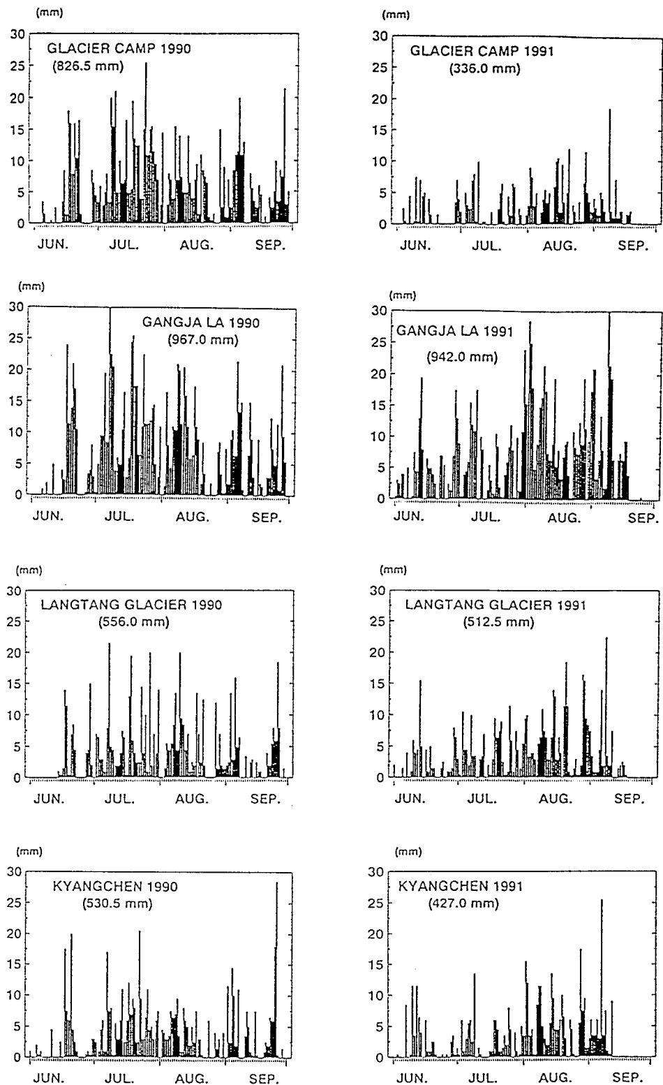
Figure 3.9. Daily precipitation changes at GC, GA, LA and KYN in the monsoon seasons of 1990 and 1991.
