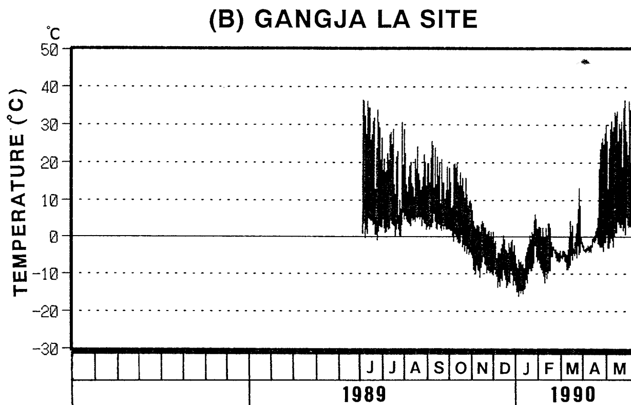
Figure 4.13. Diurnal ranges in rock surface temperature. (A): Glacier Camp (5110 m), and (B): Gangja La (5090 m).
