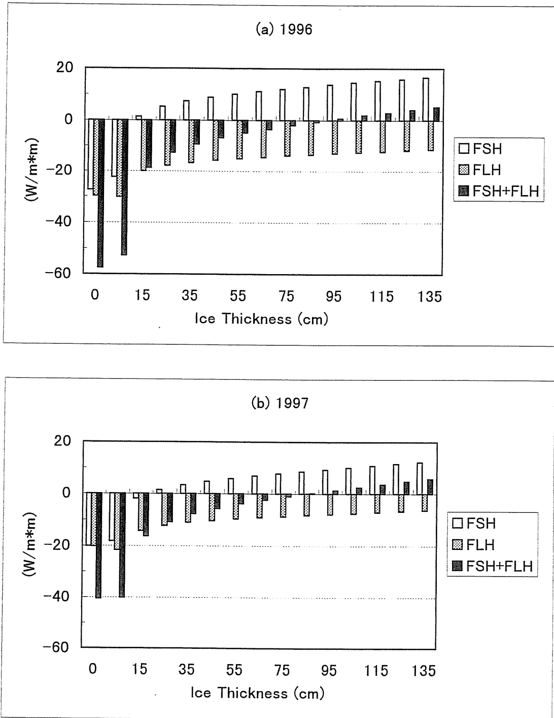
Figure 4.3.2 Turbulent heat flux as a function of ice thickness.
