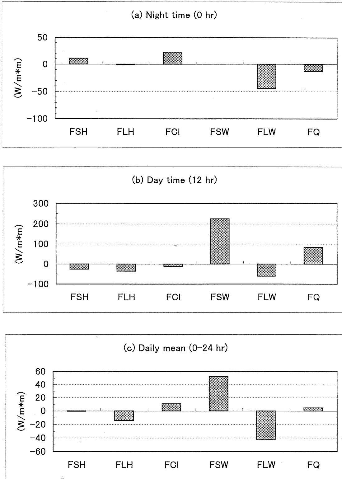
Figure 4.3.7 Diurnal change of heat budget over the entire sea ice area.
