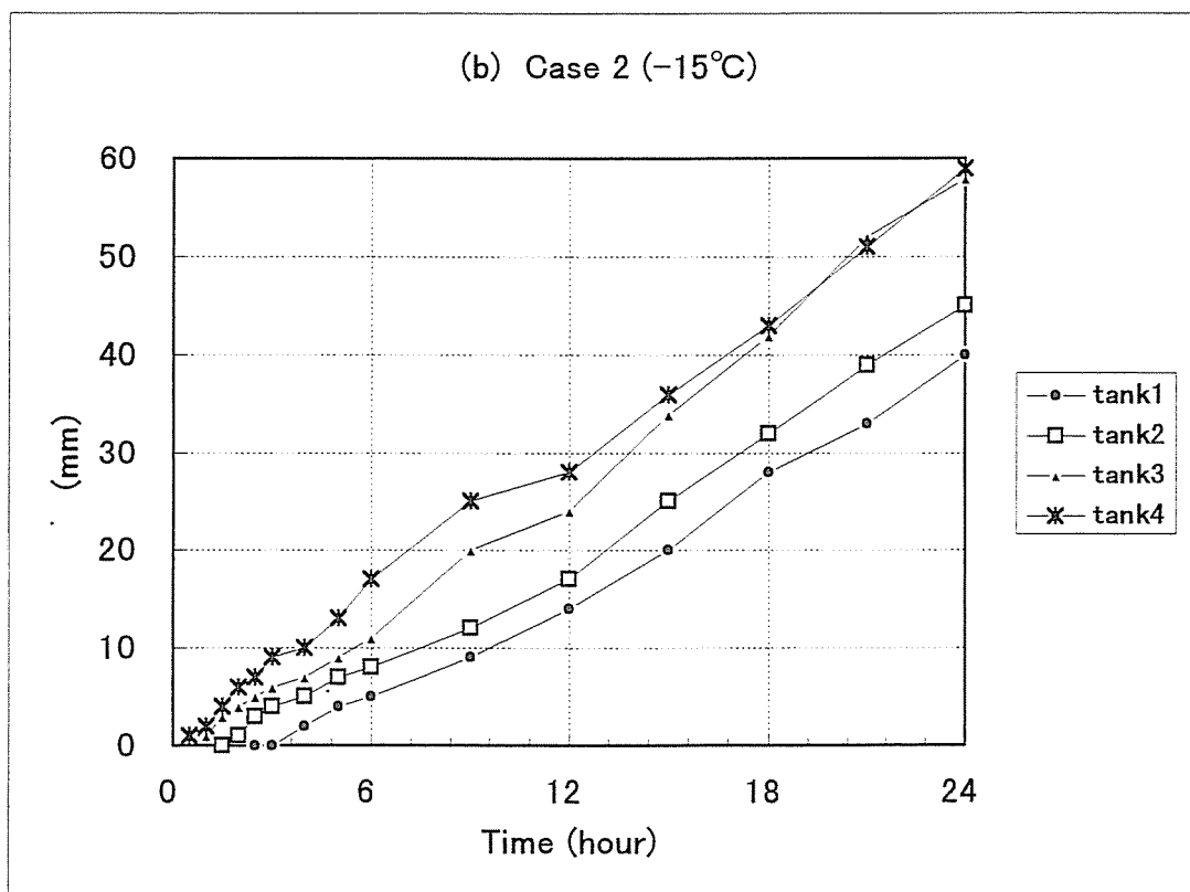
Figure 6.3.2 Growth of ice thickness.
