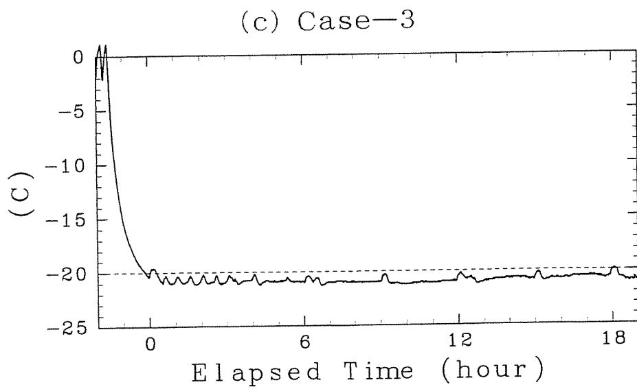
Figure 6.3.1 Time series of the room air temperature.
