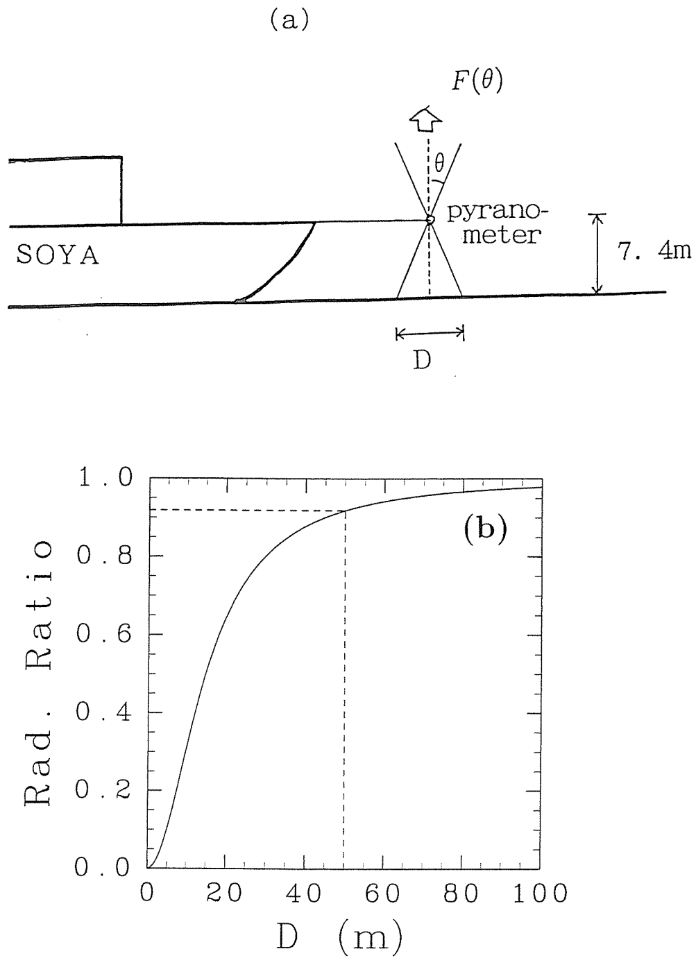
Figure 3.2.2 : Contribution of the radiation emitted from the circle area just below a pyranometer to total upward short wave radiation. (a) Geometric side view. (b) Geometrically calculated contribution as a function of the diameter ( D m).
