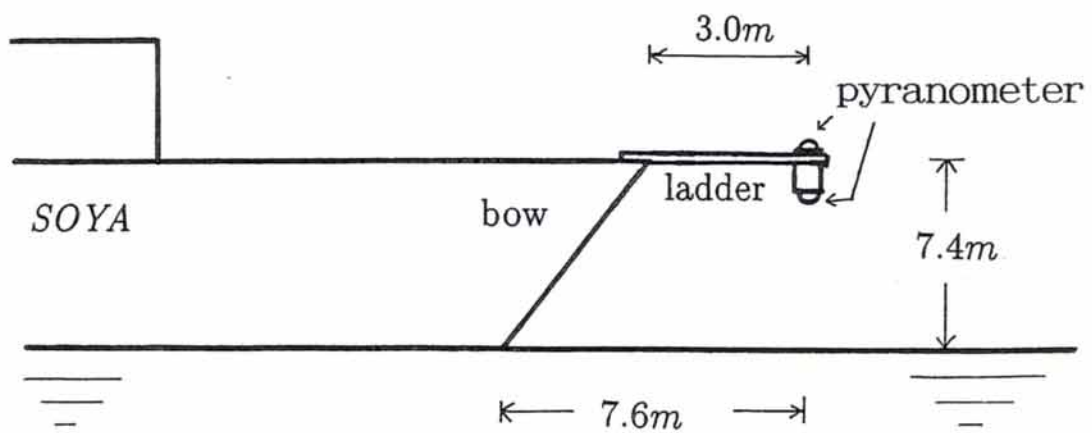
Figure 2.2.1 Measurement of short wave radiation.
