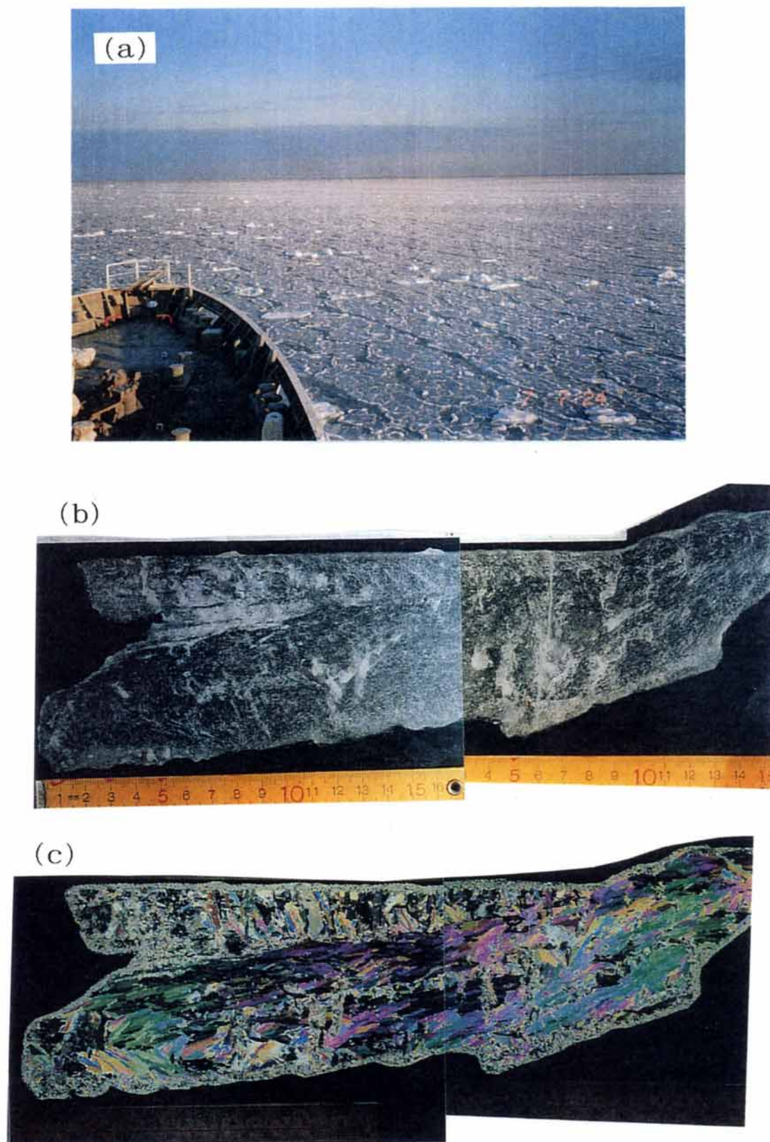
Figure 5.3.12 Vertical structure of pancake ice P3 (1997)
