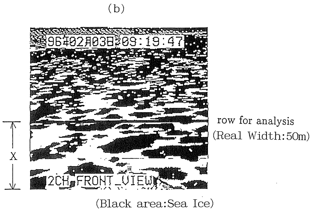
Figure 2.3.1 Ice concentration analysis.
