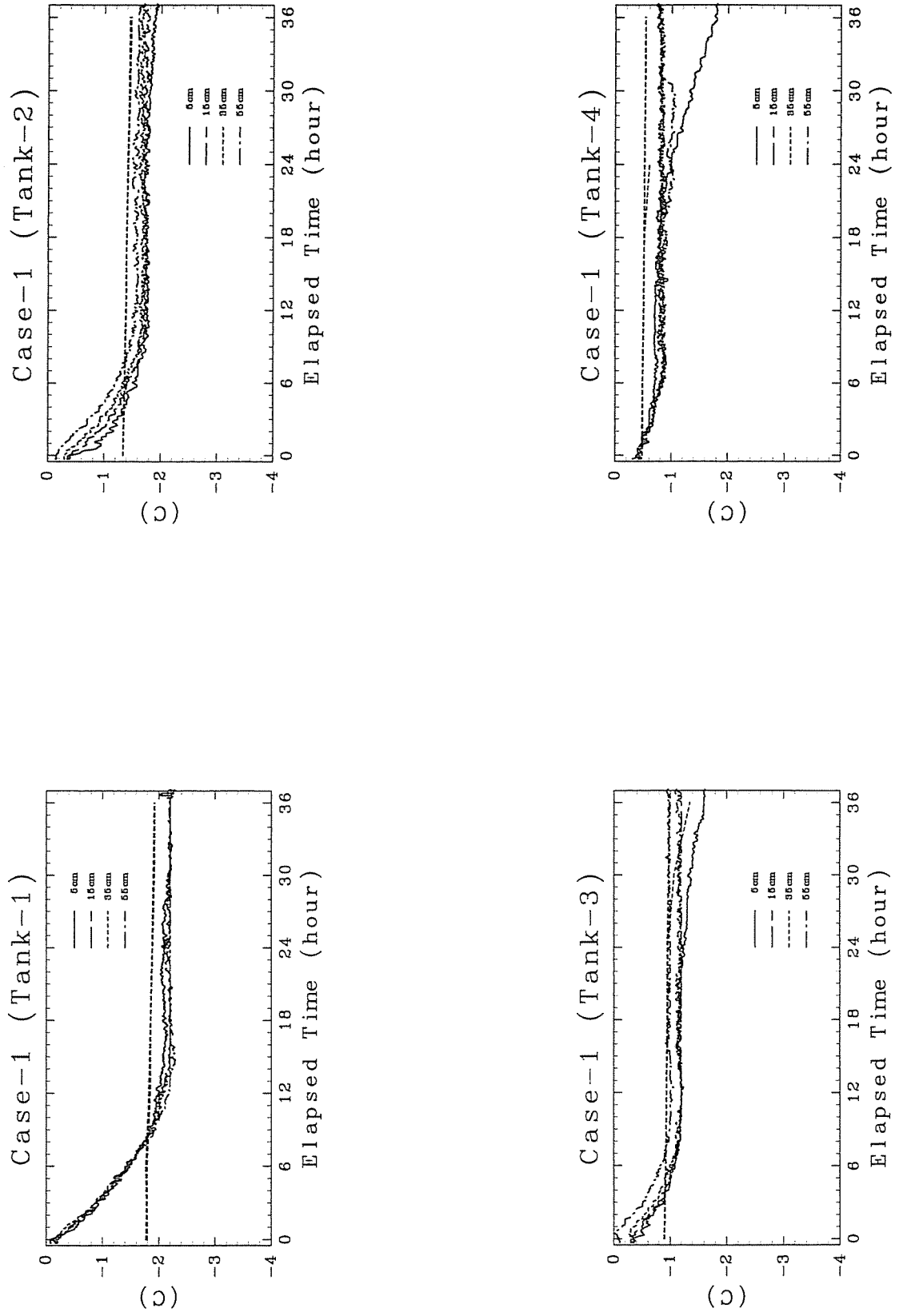
Figure 6.3.3 Time series of water temperature.
