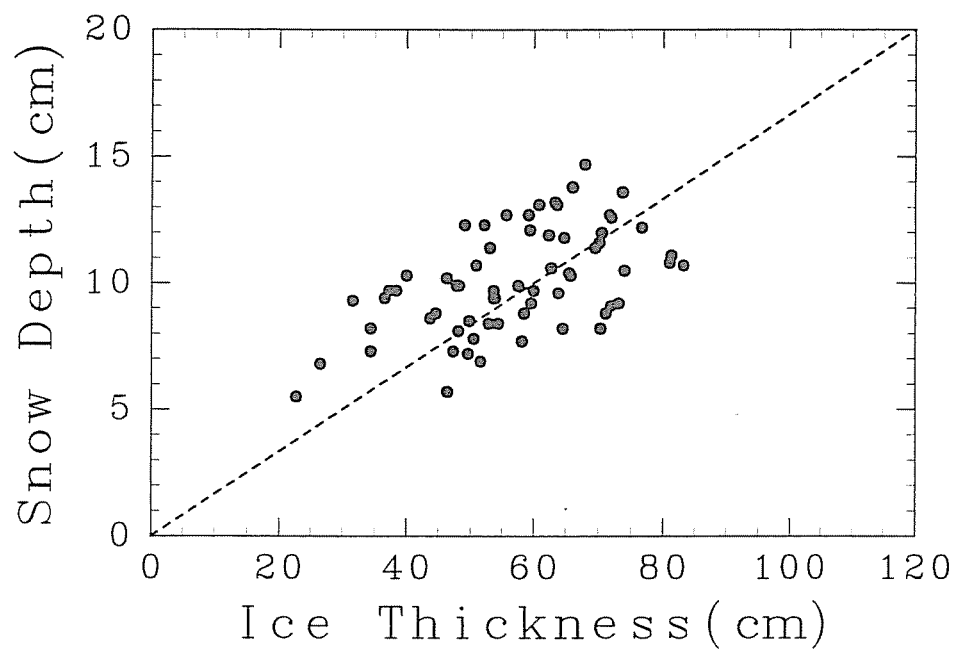
Figure 3.5.1 : Correlation between snow depth and ice thickness.
