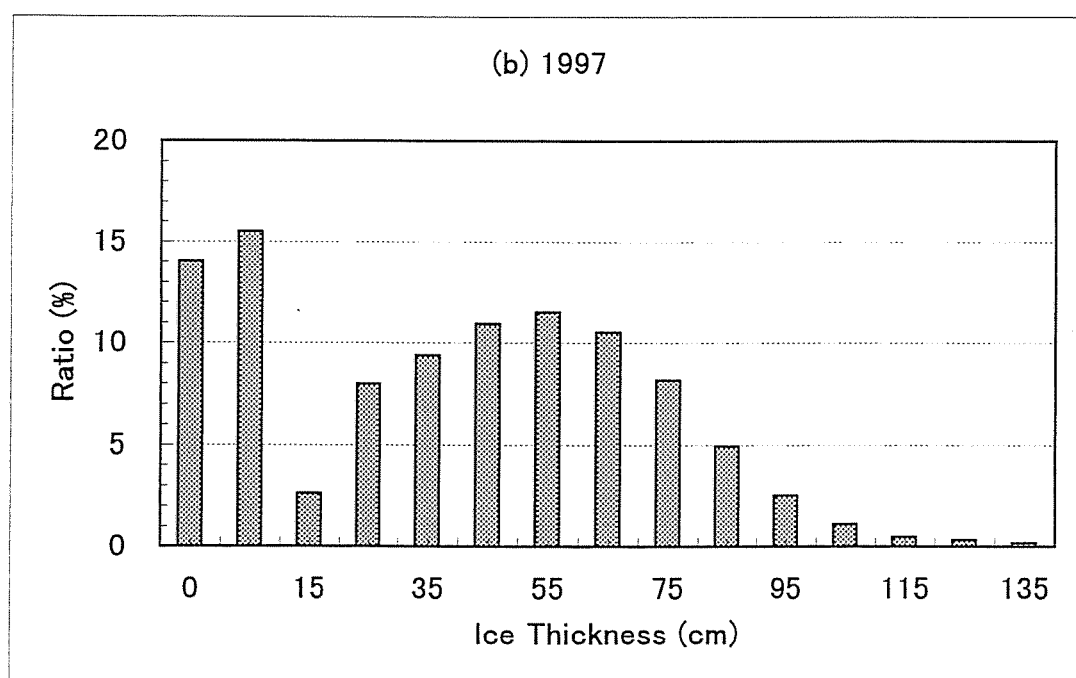
Figure 4.2.2 Areal fraction of ice thickness used for heat budget calculation.
