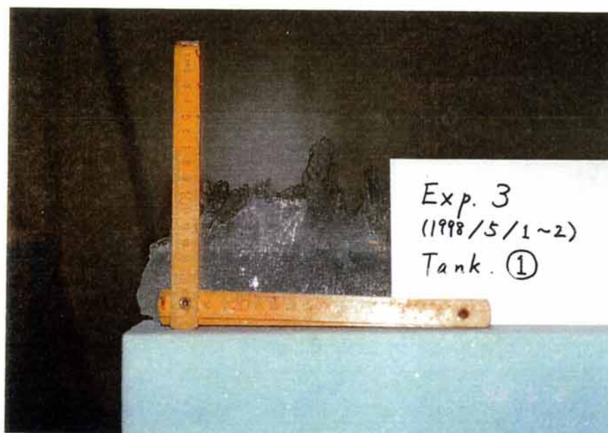
Figure 6.3.5 Photograph of formed ice
