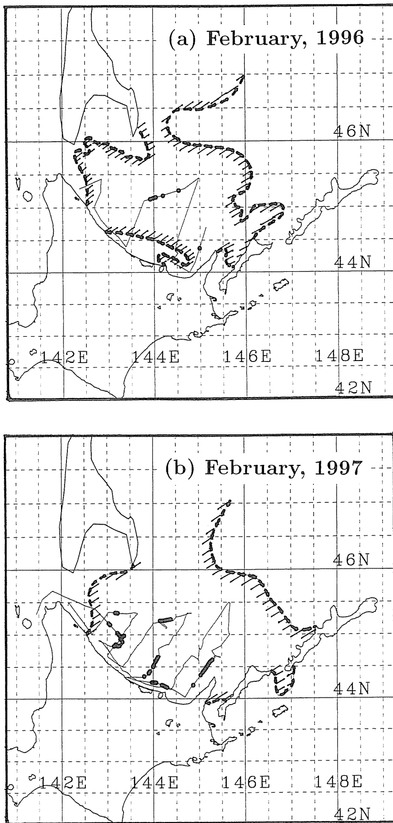
Figure 1.1 Geographical map of the southwestern Okhotsk Sea with the location of the samples used for albedo analysis (black circles) and ship tracks (thin lines).
