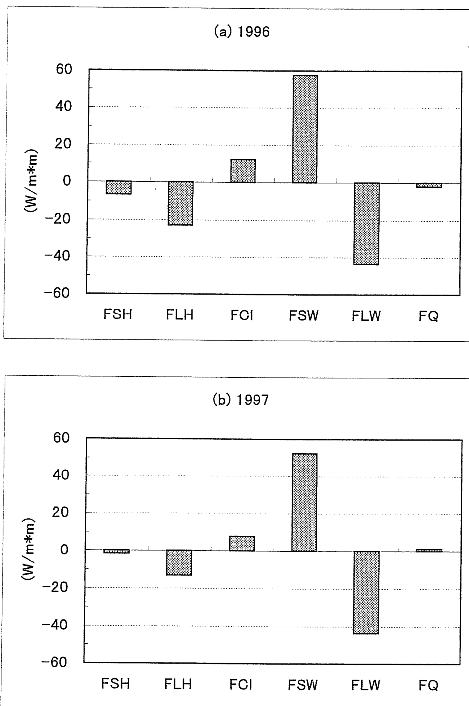
Figure 4.3.1 Heat budgets for daily mean meteorological data.
