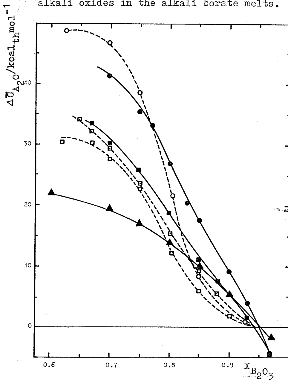
Figure 21. Relative partial molar free energies of alkali oxides in the alkali borate melts.
