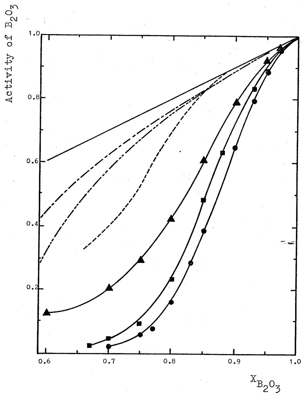
Figure 23. Activities of B_2O_3 in the alkali borate melts.
