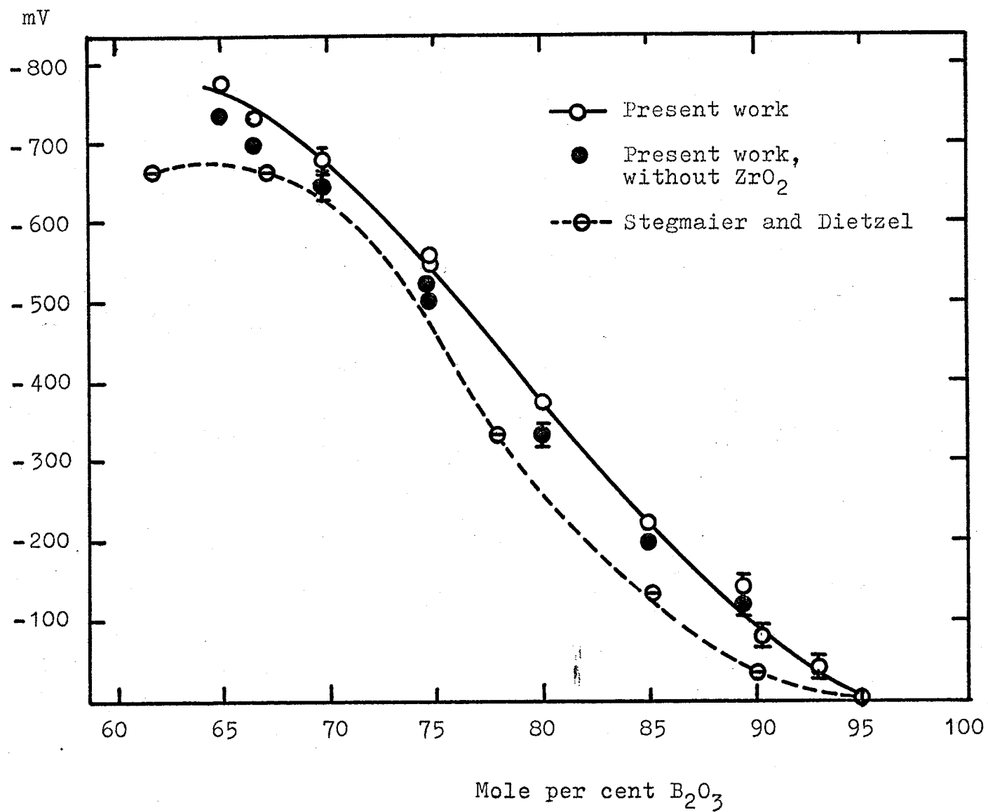
Figure 4. Emf value as functions of composition at 850°C
