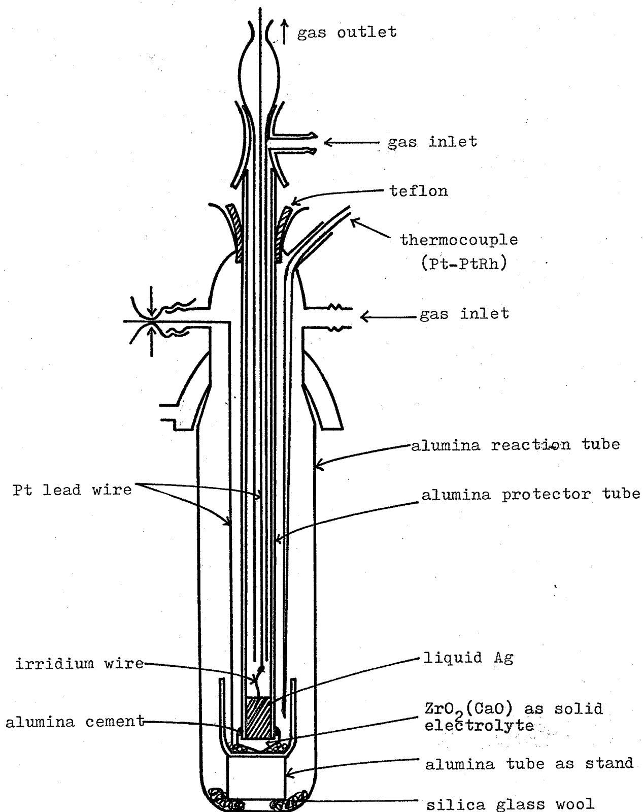
Figure 11. Cell assembly for measurement of diffusion of oxygen in liquid Ag
