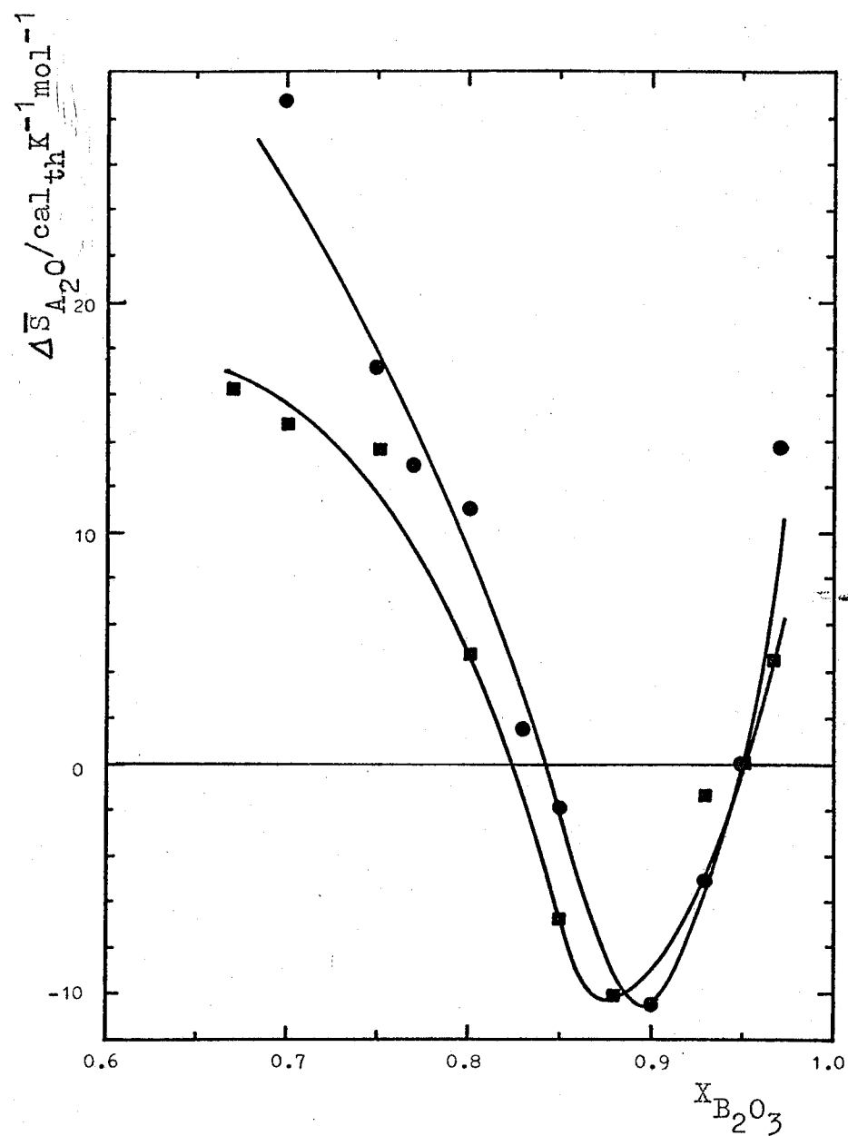
Figure 26. Relative partial molar entropies of alkali oxide in Na_2O-B_2O_3 and K_2O-B_2O_3 melts (reference melt: 95 mol % B_2O_3 solution). ■, Na_2O , at 1137 K; ●, K_2O-B_2O_3 , at 1175 K.
