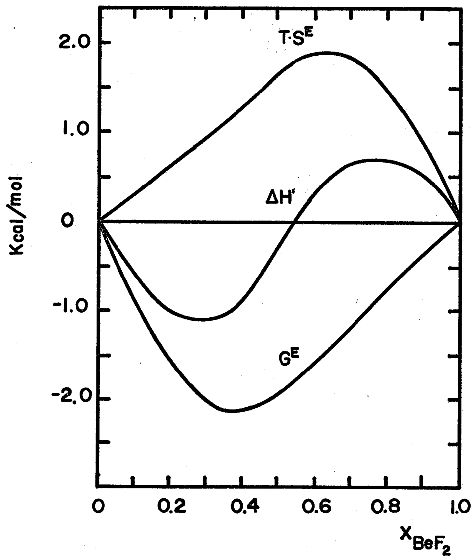
Figure 28. Liquid mixtures of LiF-BeF 2 at 862°C Kleppa et al. Baes et al.
