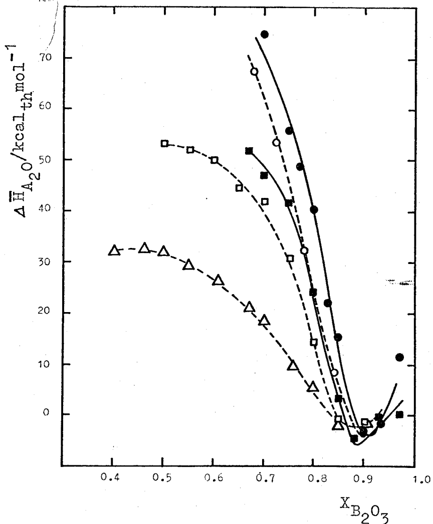
Figure 24. Relative partial molar enthalpies of alkali oxide in the alkali borate melts (reference melts: 5 mol % alkali oxide-95 mol % boron oxide).
