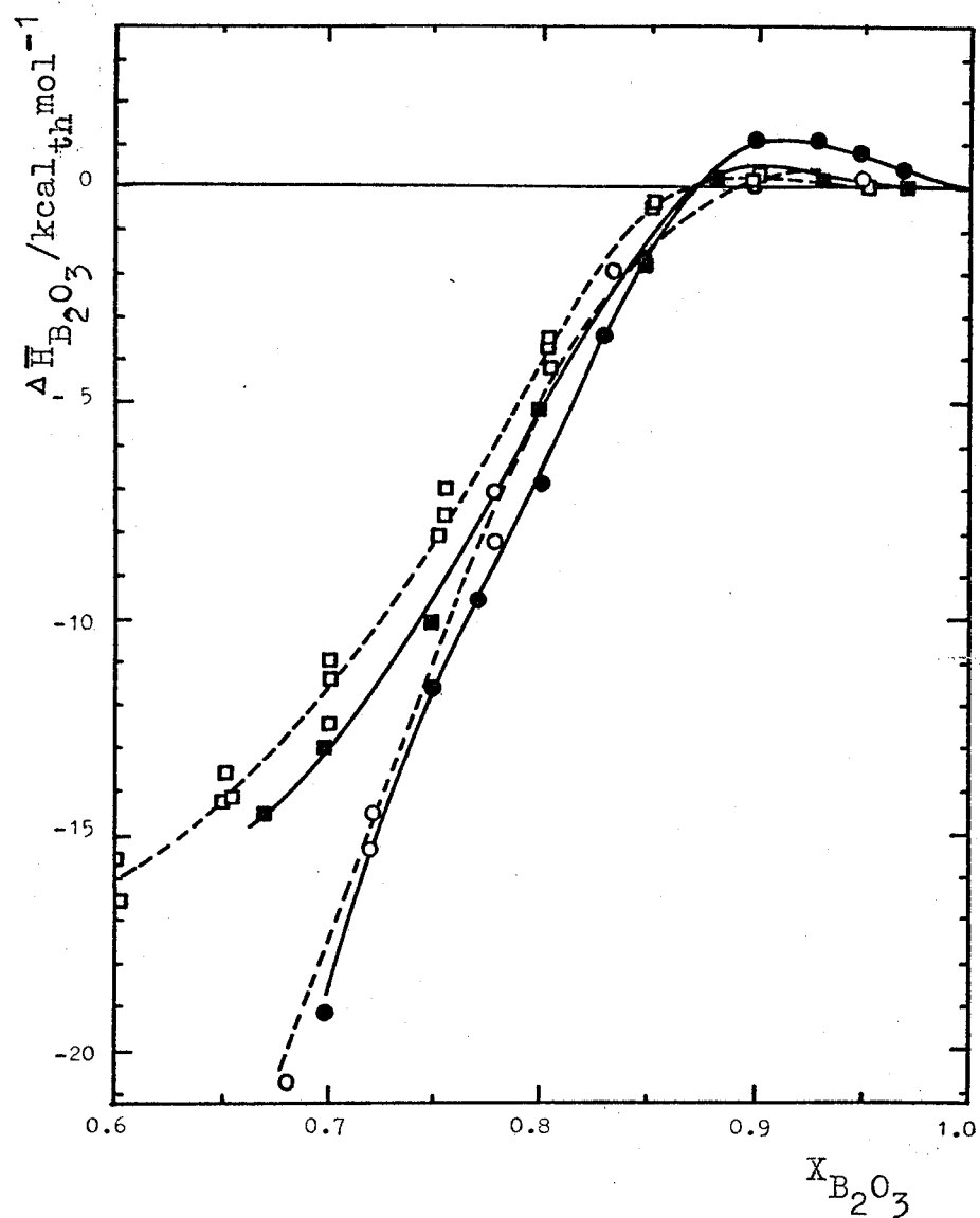
Figure 25. Relative partial molar enthalpies of B_2O_3 in Na_2O-B_2O_3 and K_2O-B_2O_3 melts.
