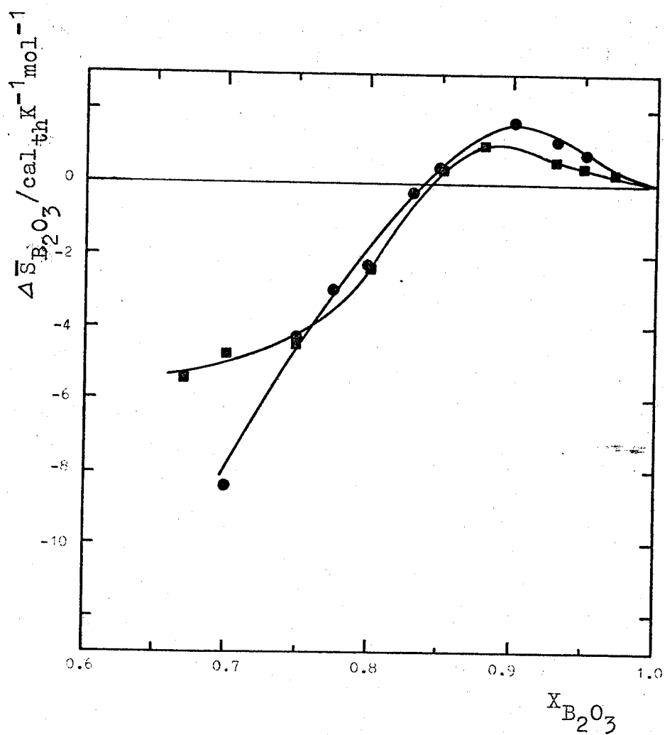
Figure 27. Relative partial molar entropies of B_2O_3 \Delta \bar{S}_{B_2O_3} in Na_2O-B_2O_3 and in K_2O-B_2O_3 melts at 1137 K and 1175 K respectively, \blacksquare , Na_2O-B_2O_3 ; \bullet , K_2O-B_2O_3 .
