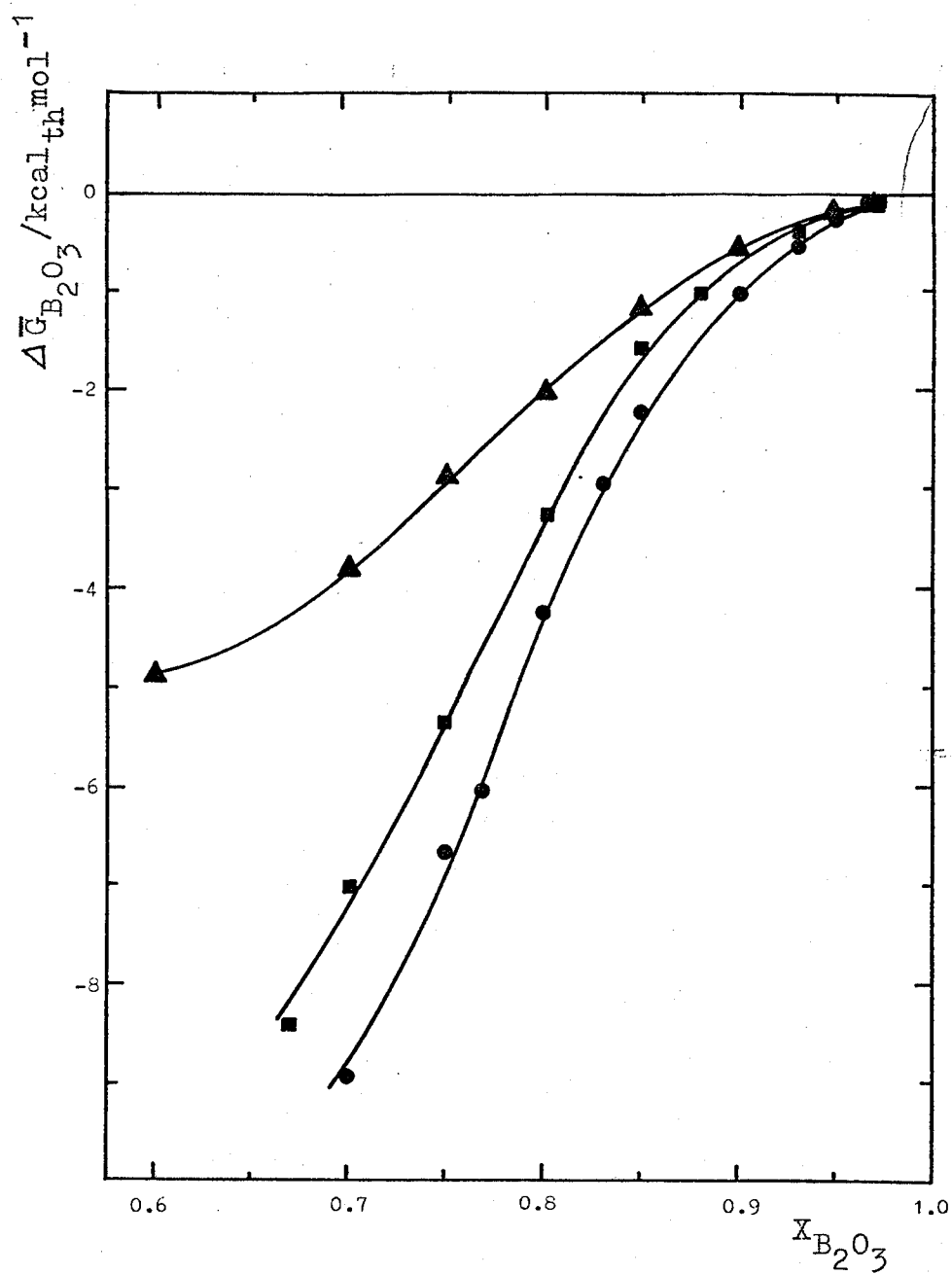
Figure 22. Relative partial molar free energies of B_2O_3 , \Delta \bar{G}_{B_2O_3} , in the alkali borate melts. Li_2O-B_2O_3 : \blacktriangle , at 1198 K. Na_2O-B_2O_3 : \blacksquare , 1137 K. K_2O-B_2O_3 : \bullet , at 1175 K.
