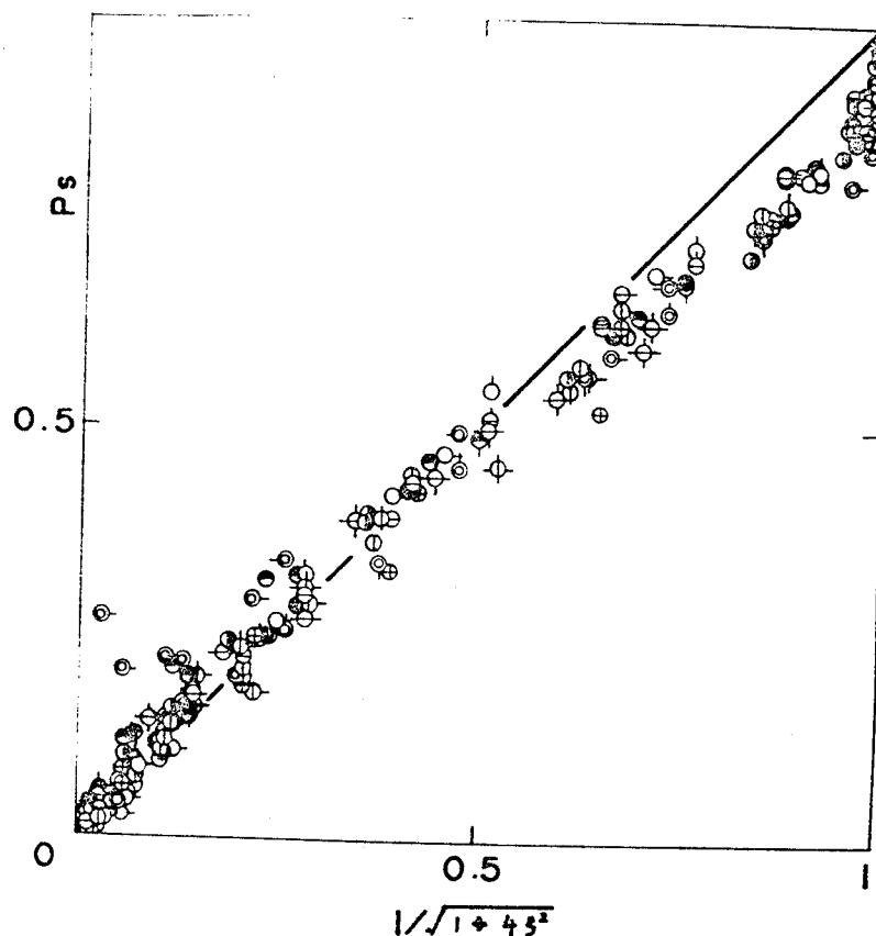
Fig. 5-6. Plots of P_s against 1/(1 + 4\xi^2)^{1/2} for various combinations of membrane and electrolyte.
