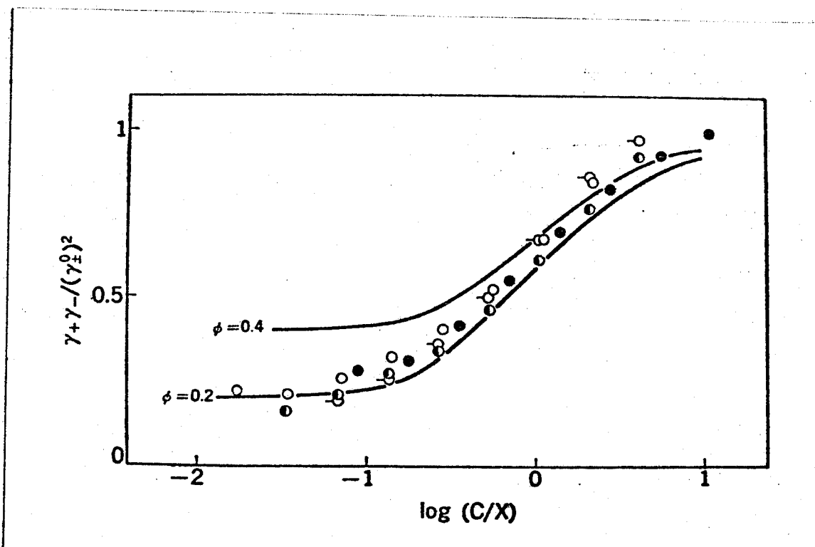
Fig. 3-4. Plots of \gamma_+ \gamma_- / (\gamma_{\pm}^0)^2 against \log(C/X) .
