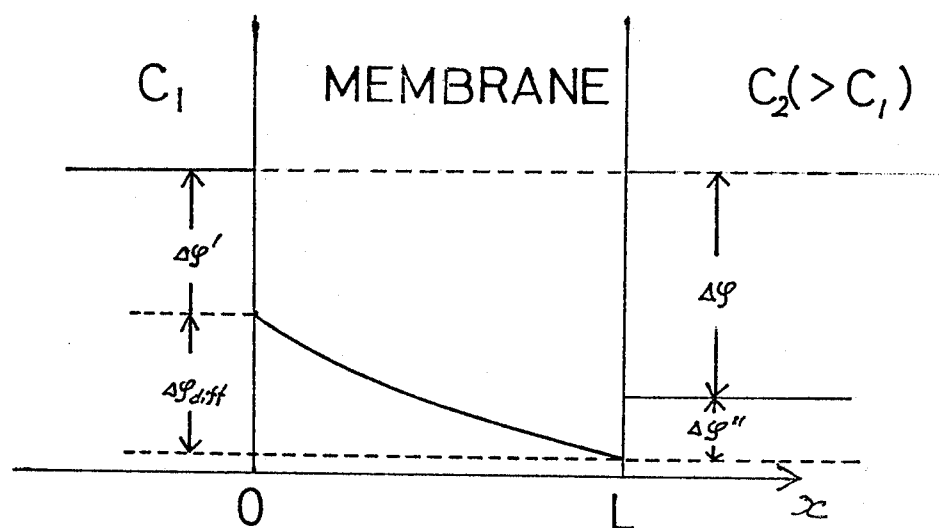
Fig. 3-1. Schematic diagram of potential profile in membranes.
