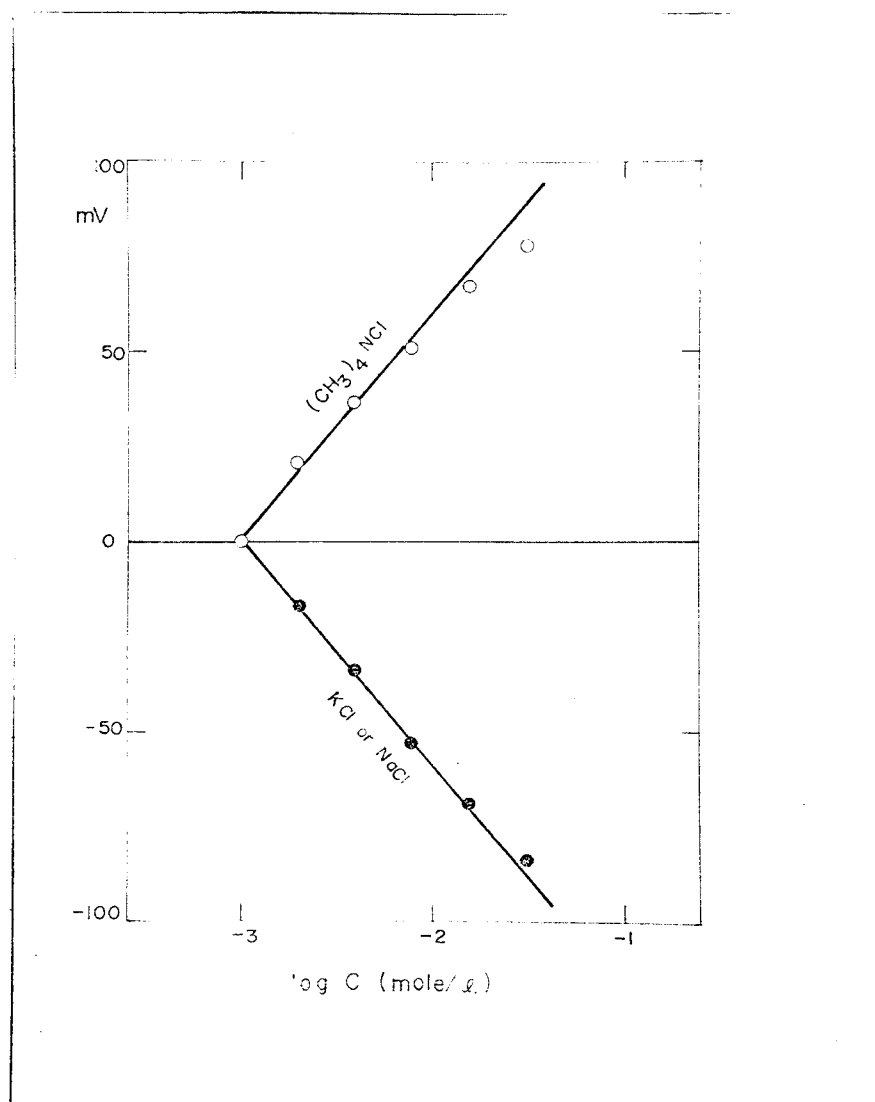
Fig. 10-6. The observed potential difference arisen between two electrolyte solutions separated by a mercury. The concentration of one compartment is kept constant at 1/1024 N and that of another compartment, C is varied. ○, the potential difference arisen between two (\text{CH}_3)_4\text{NCl} solution; ⊙, the potential difference arisen between KCl or NaCl solution.
