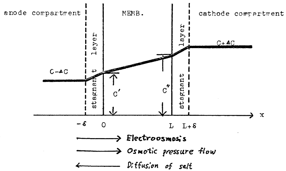
Fig. 8-1. Schematic diagram of the system considered. The symbols are defined in the text.
