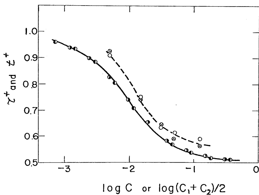
Fig. 7-5. Plots of t^+ and z^+ against \log C for membrane M-2 in KCl solution. Notations are the same as in Fig. 7-4.
