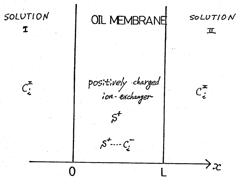
Fig. 9-1. Systems under consideration.
