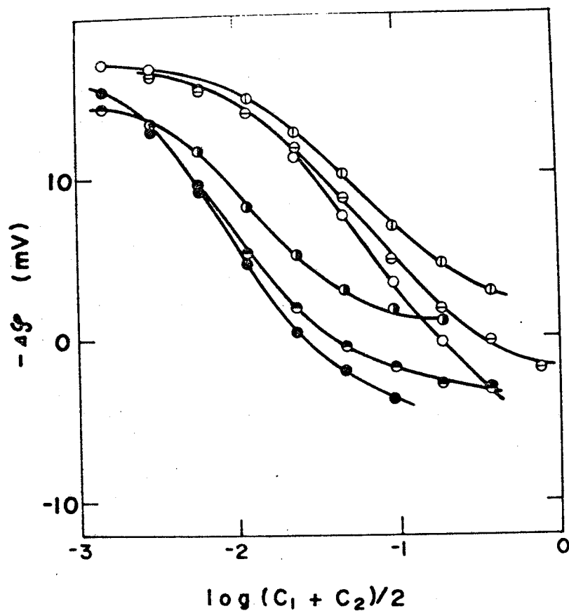
Fig. 5-4. Plots of observed membrane potential, \Delta\phi , against \log (C_1 + C_2)/2 for combinations of PS-1 and PS-3 membranes and LiCl, NaCl, KCl. The concentration ratio of two external solutions is kept constant at 2.
