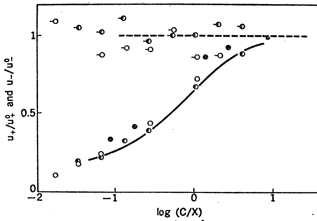
Fig. 3-10. Concentration dependence of u_+/u_+^0 and u_-/u_-^0 in NaCl solution. Results of u_-/u_-^0 , \circ , PS-1; \ominus , PS-2; \oplus , PS-3. Results of u_+/u_+^0 , \circ , PS-1; \bullet , PS-2; \bullet , PS-3. Solid line represents the experimental curve of \gamma_+\gamma_-/(\gamma_{\pm})^2 shown in Fig. 3-4.
