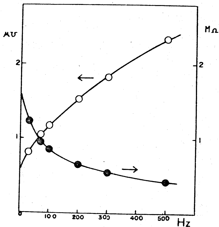
Fig. 10-2. The extrapolation of the observed membrane impedance measured by a dielectric loss bridge to zero frequency for combination of membrane G and 1/1024 N KCl. O, the membrane conductance; ●, the membrane resistance. The dc resistance calculated from these two intercept was agreed within \pm 3\% , and dc resistance was taken as the average of these two values.
