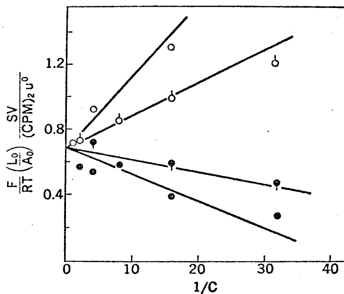
Fig. 3-6. Determination of the tortuosity factor f for systems of two kinds of membranes and ^{22}\text{Na} and ^{36}\text{Cl} . Results of ^{22}\text{Na} , \circ , PS-1; \bigcirc , PS-2. Results of ^{36}\text{Cl} , \bullet , PS-1; \oplus , PS-2.
