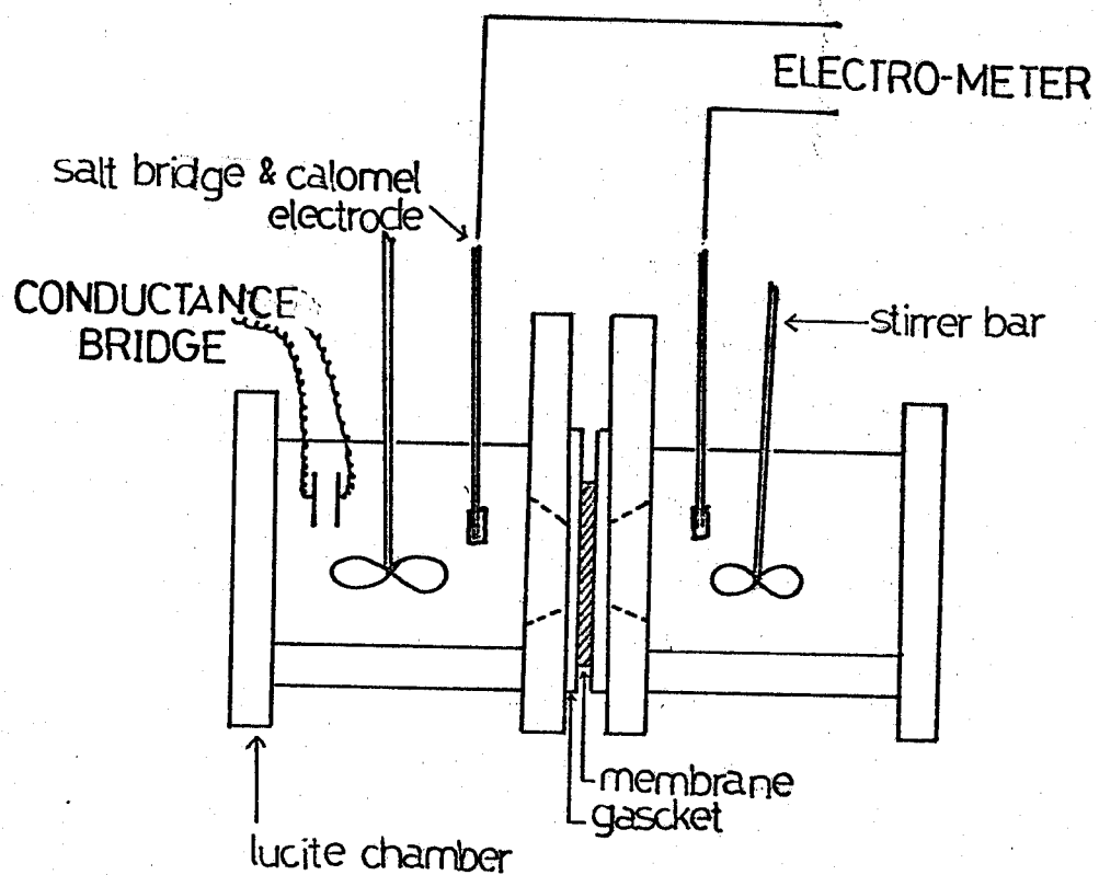
Fig. 3-3. Schematic diagram for a cell and an apparatus of measuring a membrane potential and salt flux.
