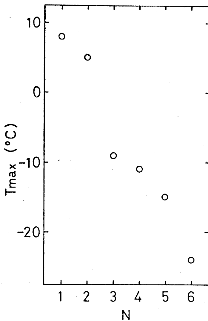
Figure 2.4. The dispersion temperature T_{\text{max}} as a function of the number of carbons in the side-chain alkyl group, N .
