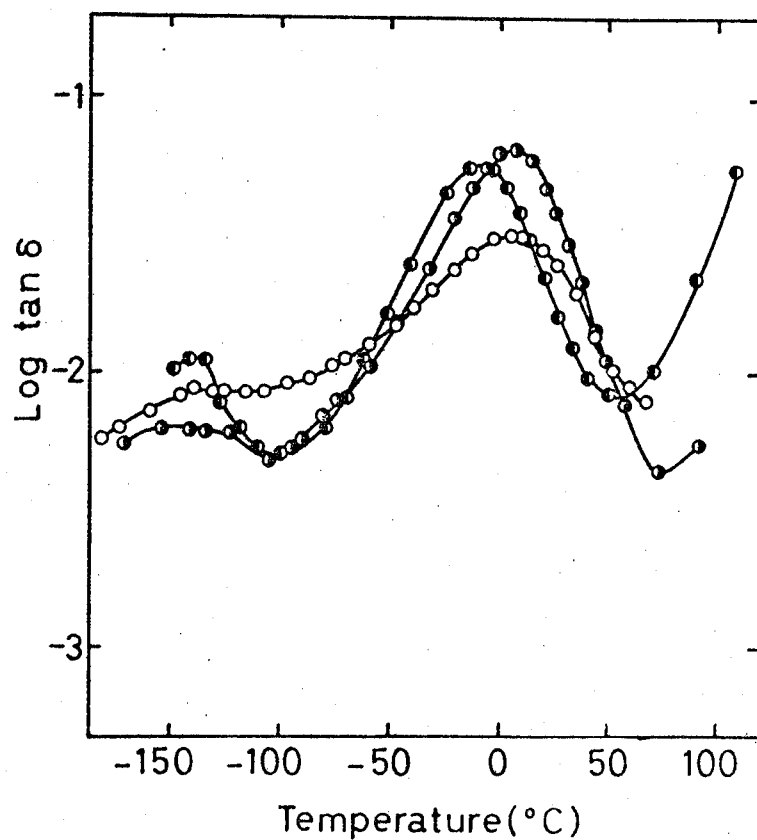
Figure 2.1 (a). Temperature dependence of \tan \delta for PMLG(○), PELG(◐), and PnPLG(●) measured at a frequency of 1kHz.
