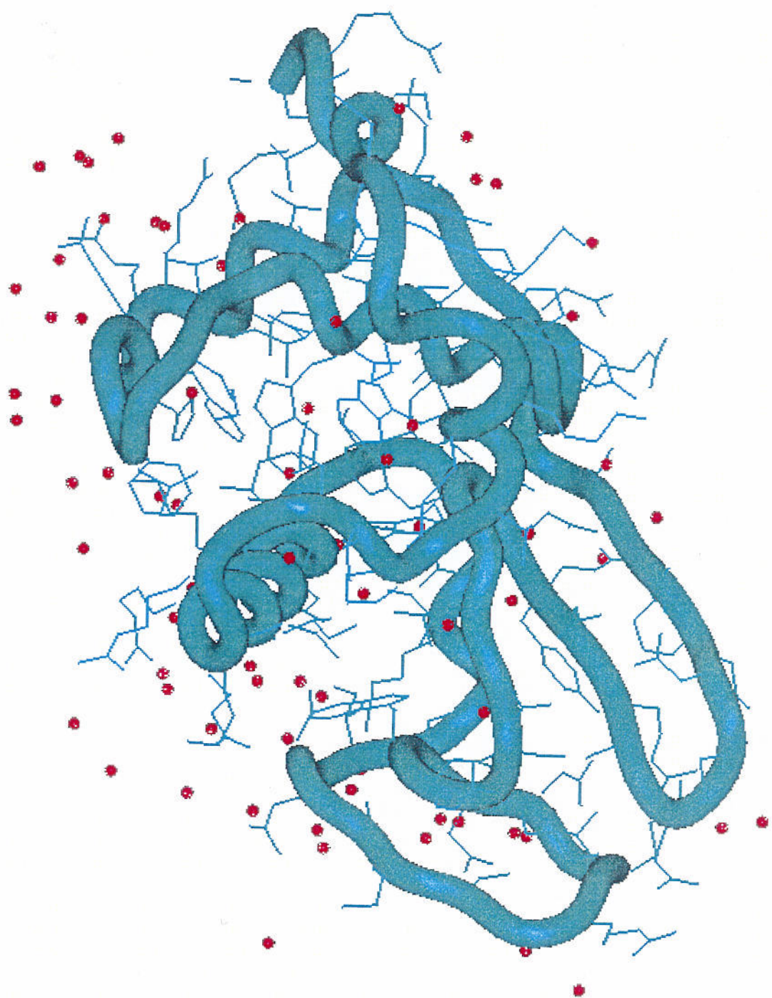
Fig. 4-1.1 The drawing of structure of refined pigeon egg-white lysozyme produced by program MOL-GGRAPH. The red points are 81 water molecules. The main-chain was drawn by blue tube.
