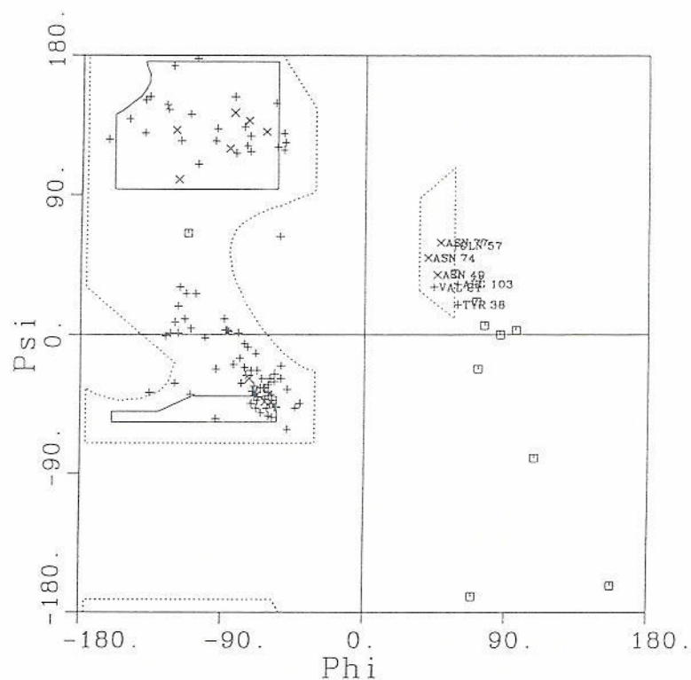
Fig. 4-1.3. Ramachandran plot of main-chain torsion angles for structure of refined pigeon egg-white lysozyme. ( \square ) Glycine; ( \times ) Asparagine; (+) other residues.
