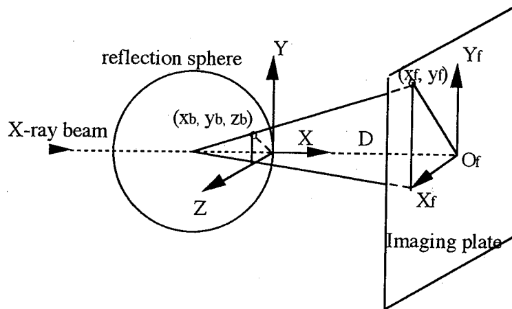
Fig. 3-1-1.2 Relation between reciprocal position vector \mathbf{x}_b(x_b, y_b, z_b) of a reflection and its detector position coordinate \mathbf{x}_f(x_f, y_f) .
