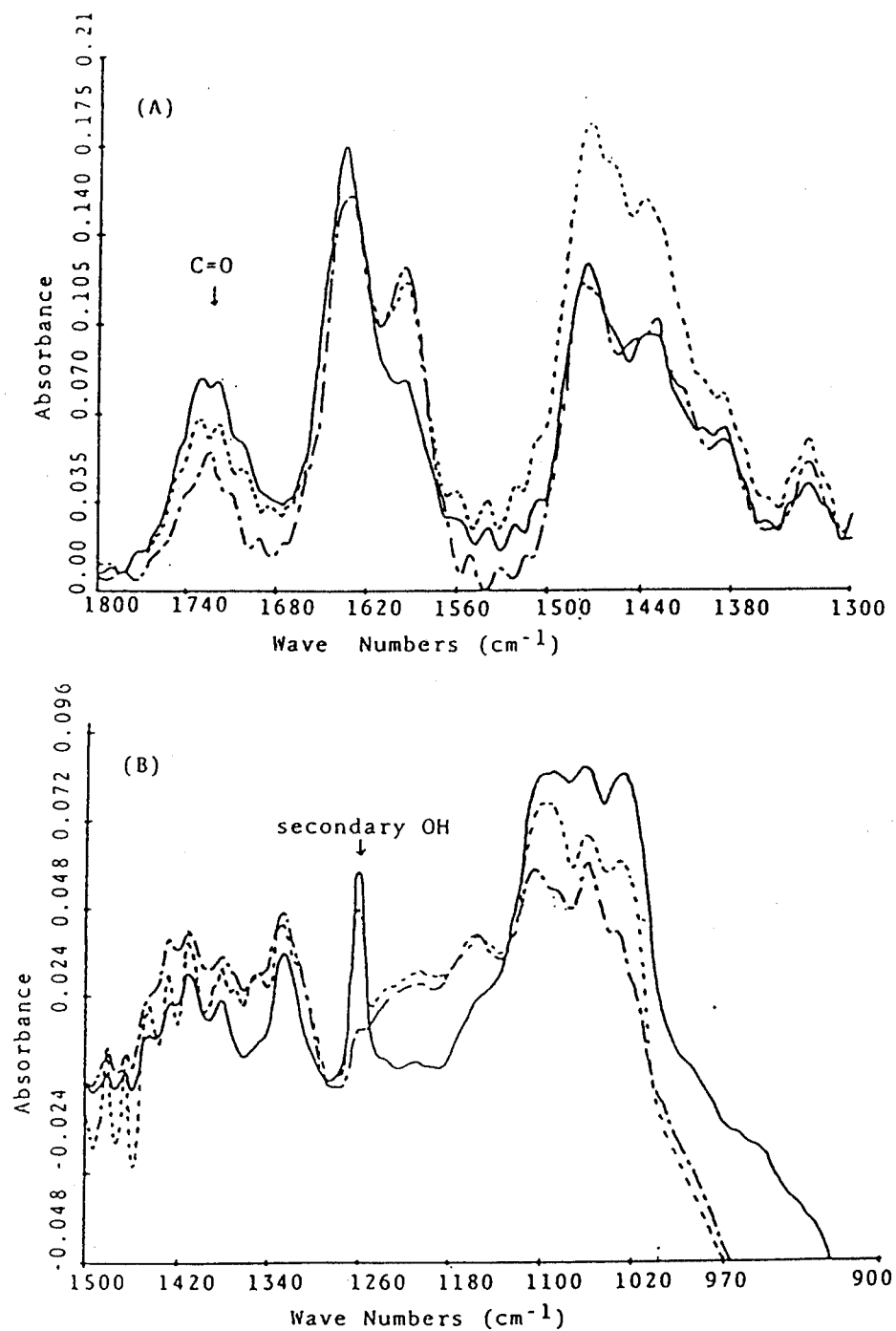
Fig.11 FT-IR absorption spectra of water-soluble CM-chitin(D.S.=0.88) and its metal ion complexes in \text{H}_2\text{O} and \text{D}_2\text{O}
