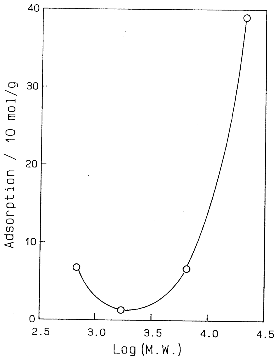
Fig.22 Adsorption capacity of Phenylalanine to Ca-CM-chitin.
