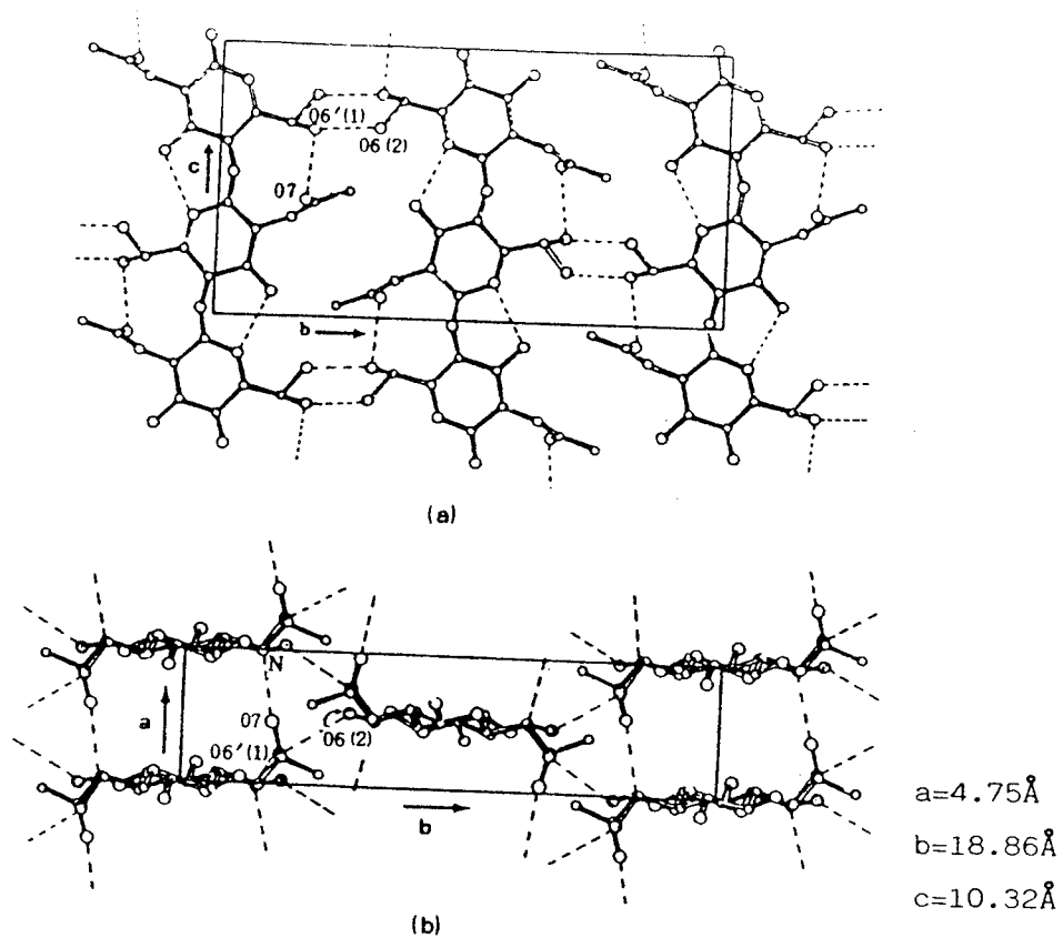
Crystalline structure of \alpha -chitin ; (a) bc-side (b) ab-side
