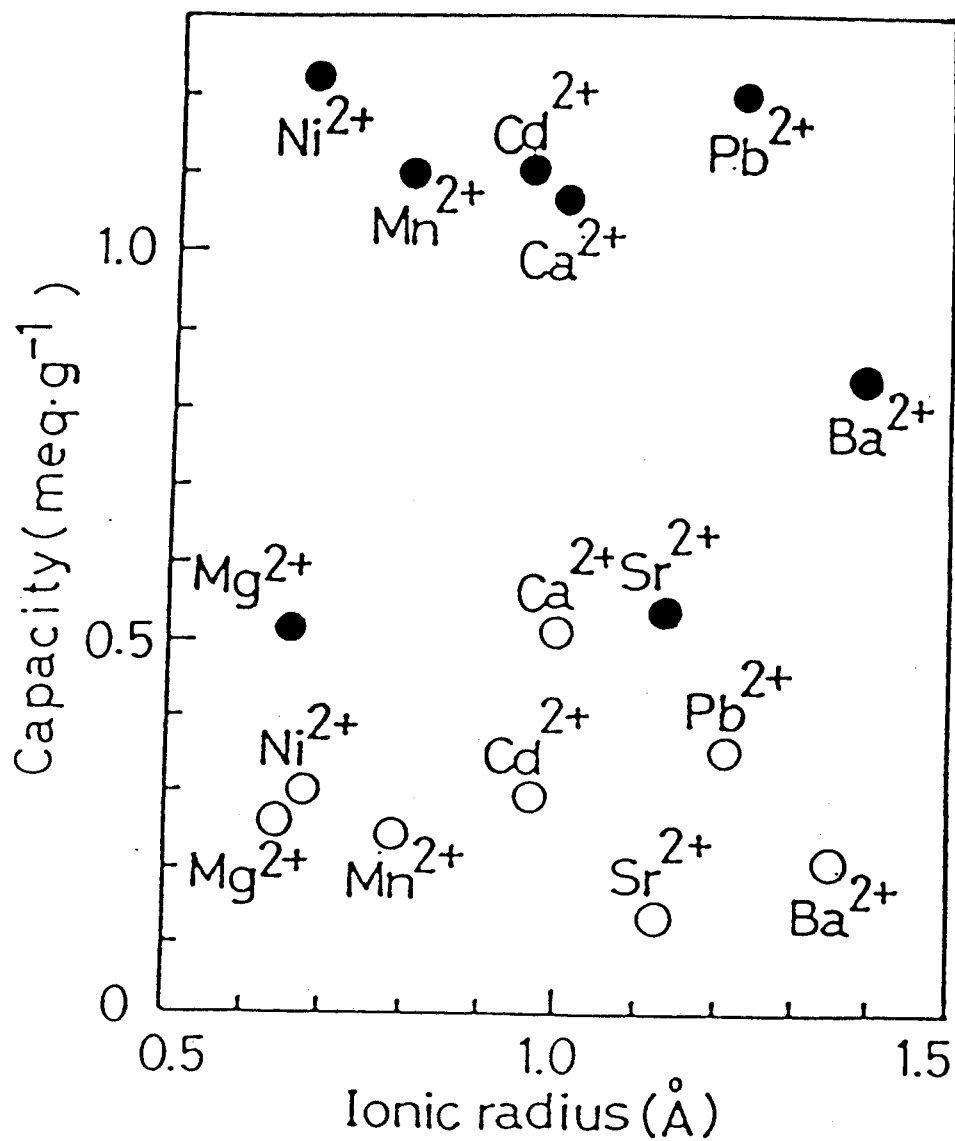
Fig.9 Relationship between ionic radius and adsorption capacities of CM-chitin(D.S.=0.1) for metal ions (○) Poorly substituted CM-chitin(flake) (●) Fibrous CM-chitin
