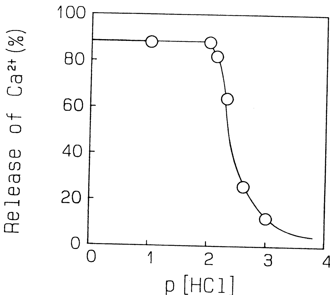
Fig.17 Release of \text{Ca}^{2+} from 6-O-CM-chitin
