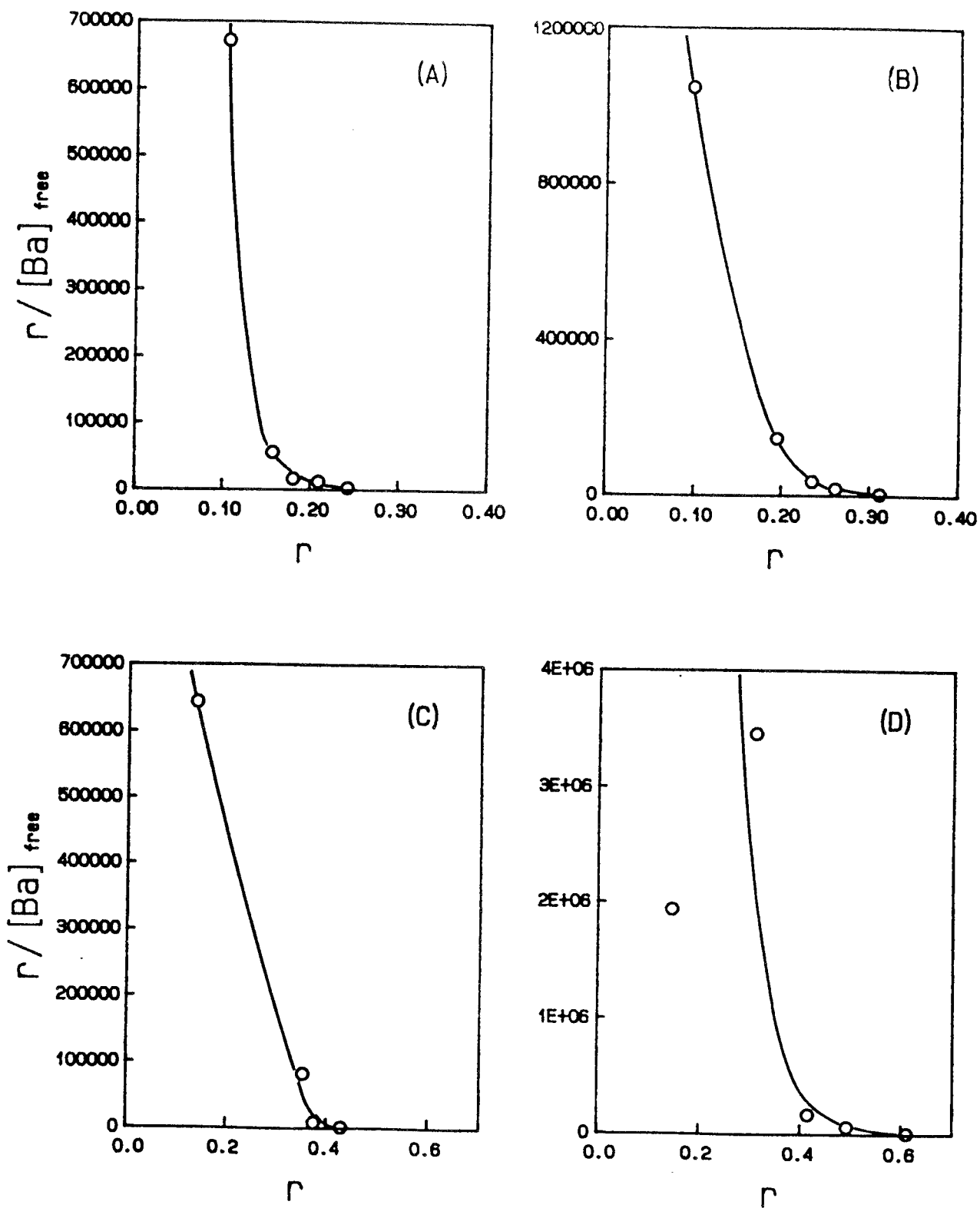
Fig.10-(c) Scatchard plot of \text{Ba}^{2+} v.s. CM-chitins
