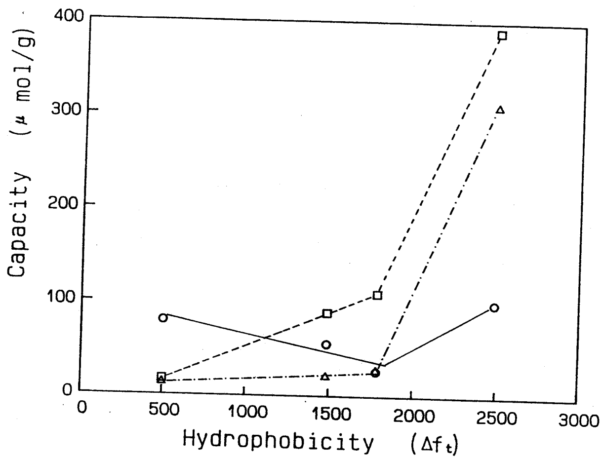
Fig.18 Relationship between adsorption capacities of amino acids for water-soluble 6-O-CM-chitin from -chitin and hydrophobicity of the side chain
