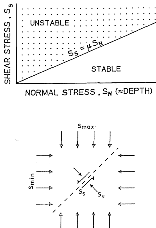
Fig.5.4: Schematic diagram of "Yield Stress Model".
