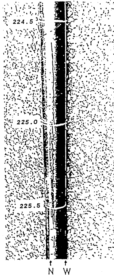
Fig.2.9: Fractures printed on the surface of an impression packer after hydraulic fracturing around the depth of 225 m in the Okabe, [OK], well. N indicates magnetic north.
