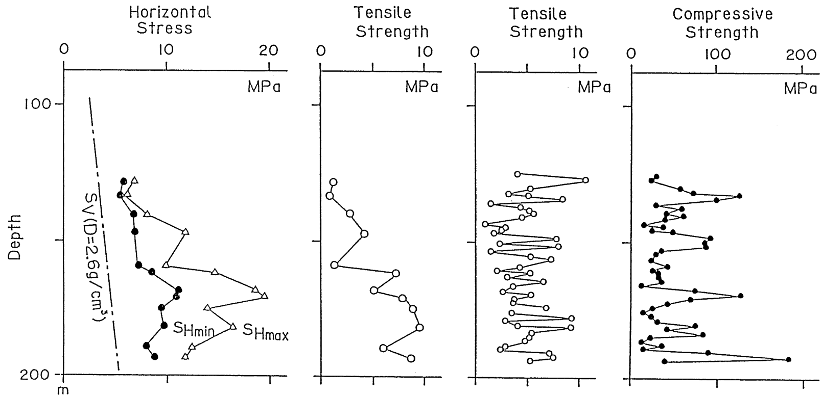
Fig.6.2: Core tensile strength and compressive strength distributions with depth. Horizontal stresses and tensile strength obtained by the hydraulic fracturing stress measurement are also shown for comparison [after SATO et al. (1987)].
