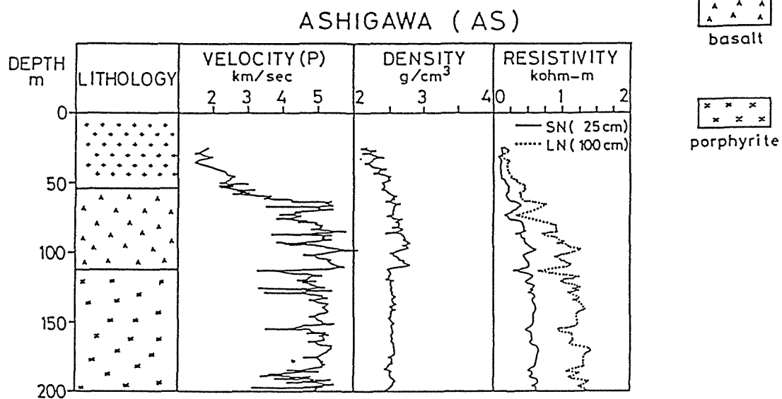
Fig.5.5: Lithological and geophysical logs in the hard rock boreholes.
