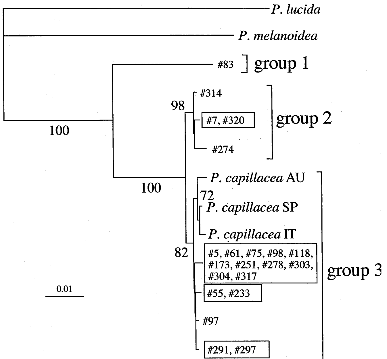
Fig. 19. Phylogenetic tree to elucidate phylogenetic position of Japanese Pterocladia / Pterocladiella complex inferred from rbcL sequences with the neighbor-joining (NJ) method based on Kimura's correction using the Clustal W computer program. The numbers at each node indicate bootstrap values (100 replications) greater than 70. Identical sequences from multiple populations (sample numbers enclosed in boxes) were represented by only one sequence in the analysis. AU, Australia; SP, Spain; IT, Italy. Scale bar = 1% divergence.
