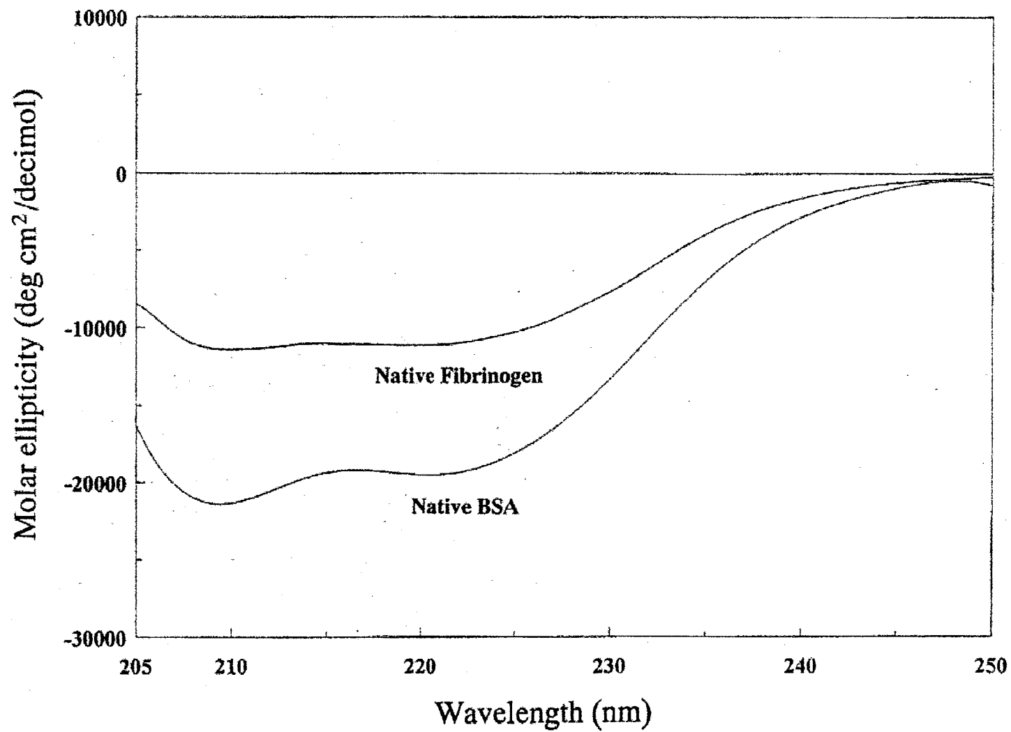
Figure 3-4. CD spectra of native BSA and FNG in PBS (pH 7.4, 37°C).
