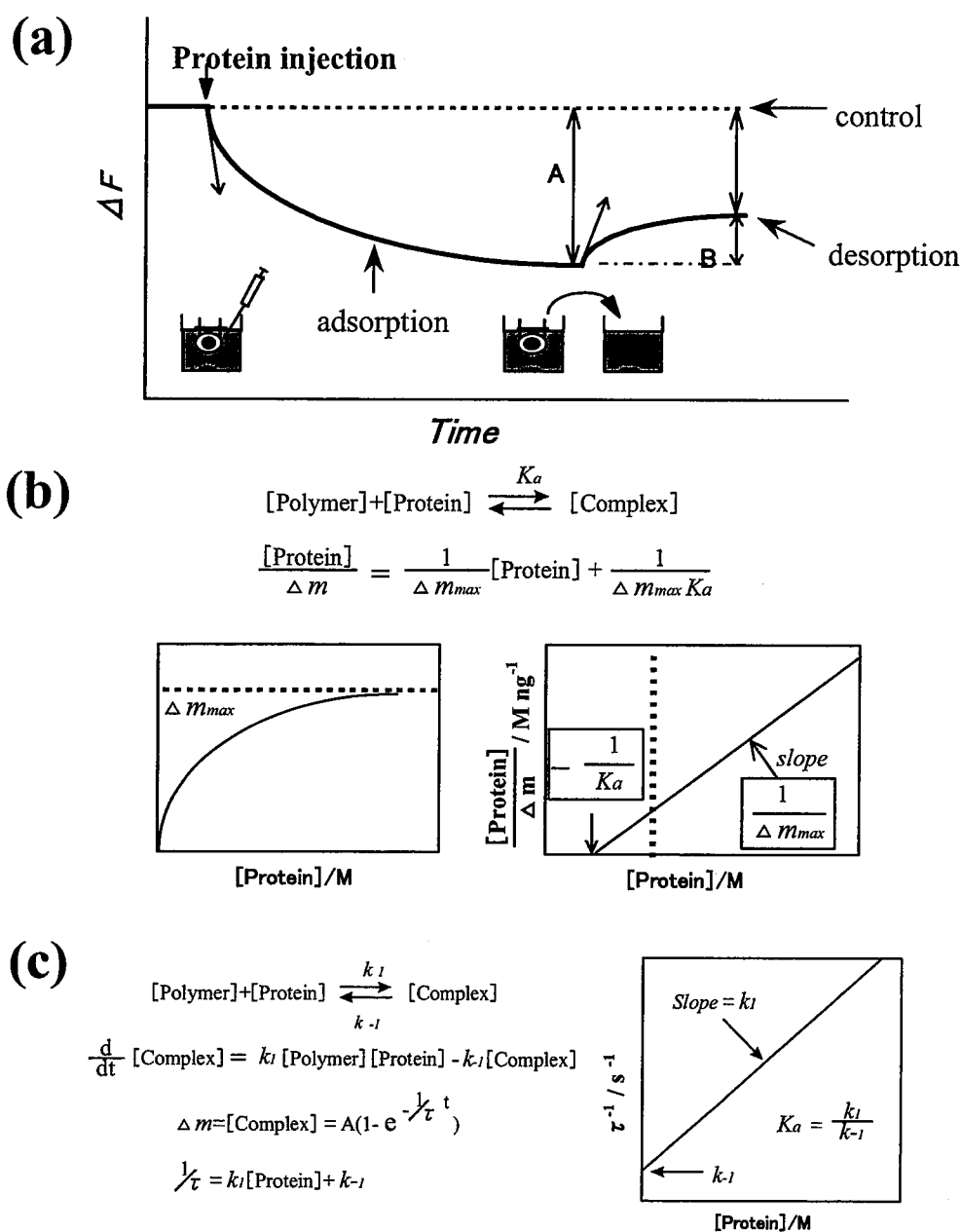
Figure 4-2 (a) Real-time monitoring of protein adsorption to polymer surfaces (37 °C , PBS) A: Amount of adsorbed protein B: Amount of desorbed protein. Kinetic measurements by using a QCM method. Saturation method (b) and Curve fitting method (c)
