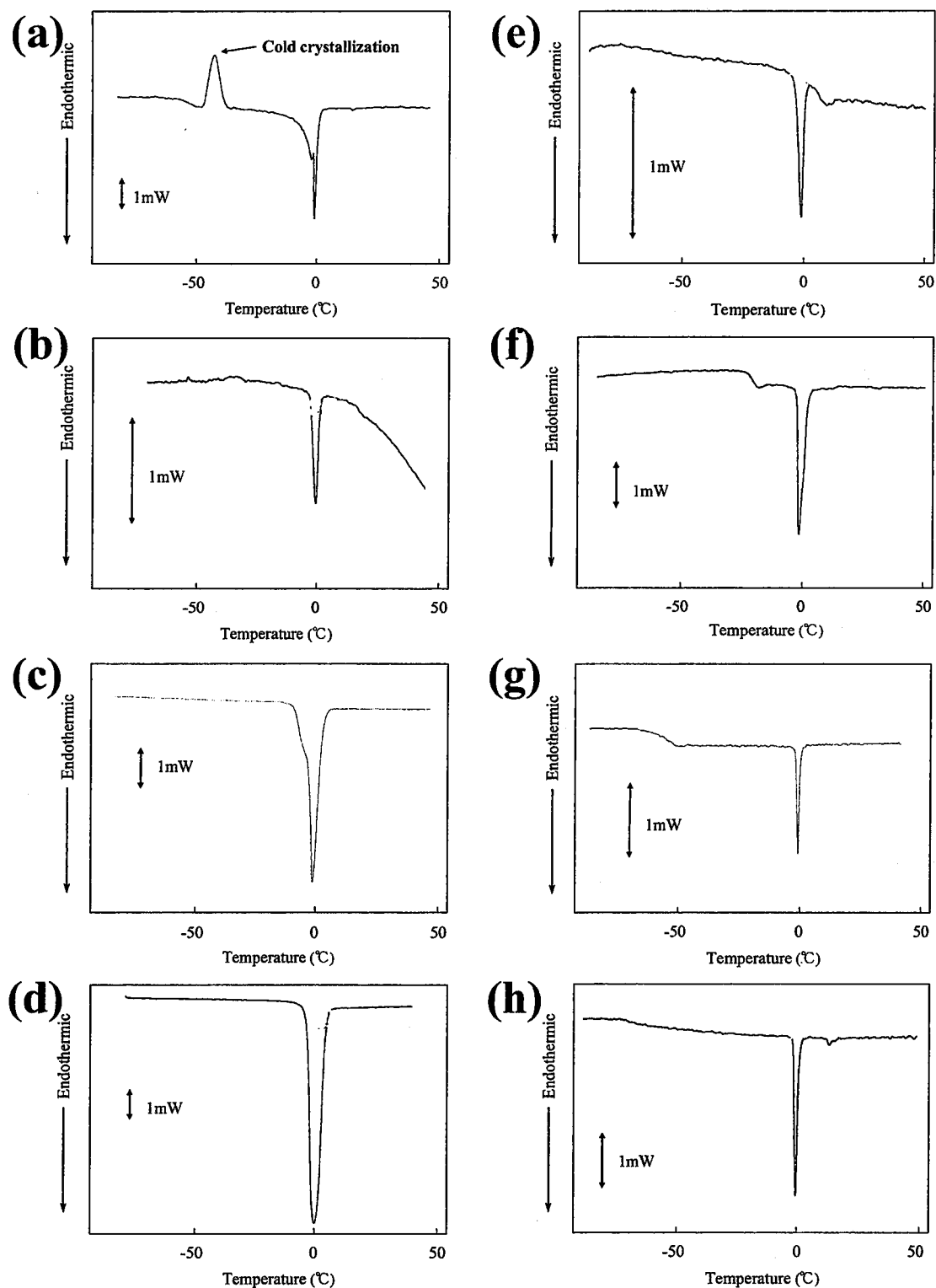
Figure 5-13. DSC thermogram of poly(meth)acrylate with EWC. a)PMEA, b)PMEMA, c)PHEMA, d)PHEA, e)PPEA, f)PEA, g)PBA, h)PEHA heating rate:2.5°C/min.
