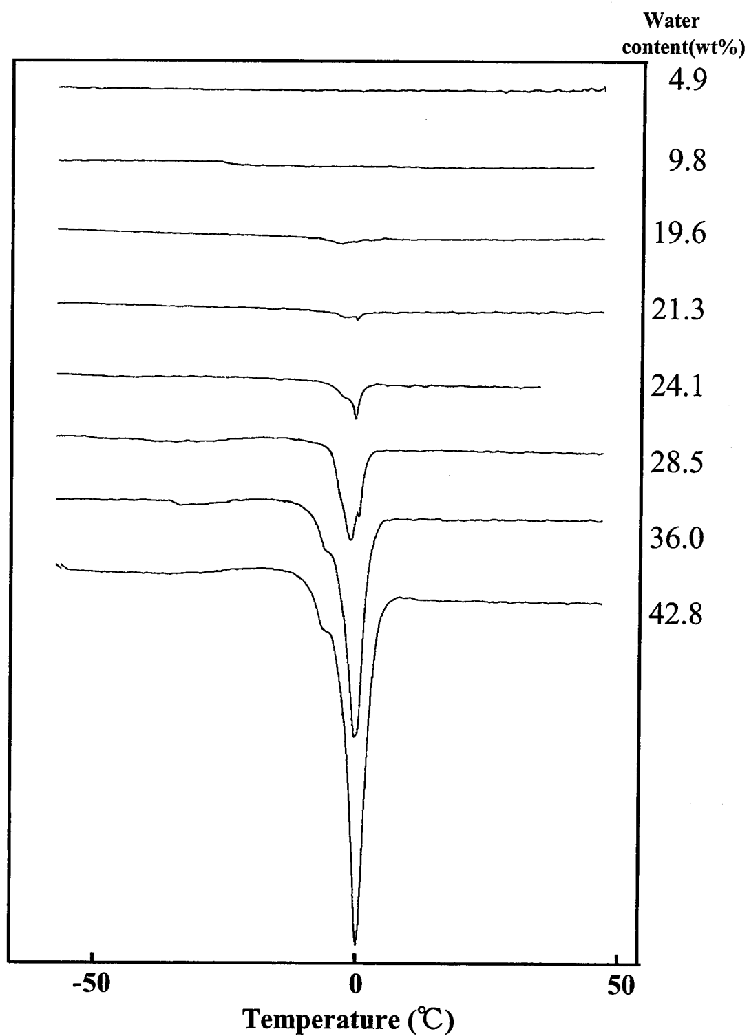
Figure 5-5. DSC curves of the PHEMA-water systems with various water contents; heating rate=2.5 °C / min.
