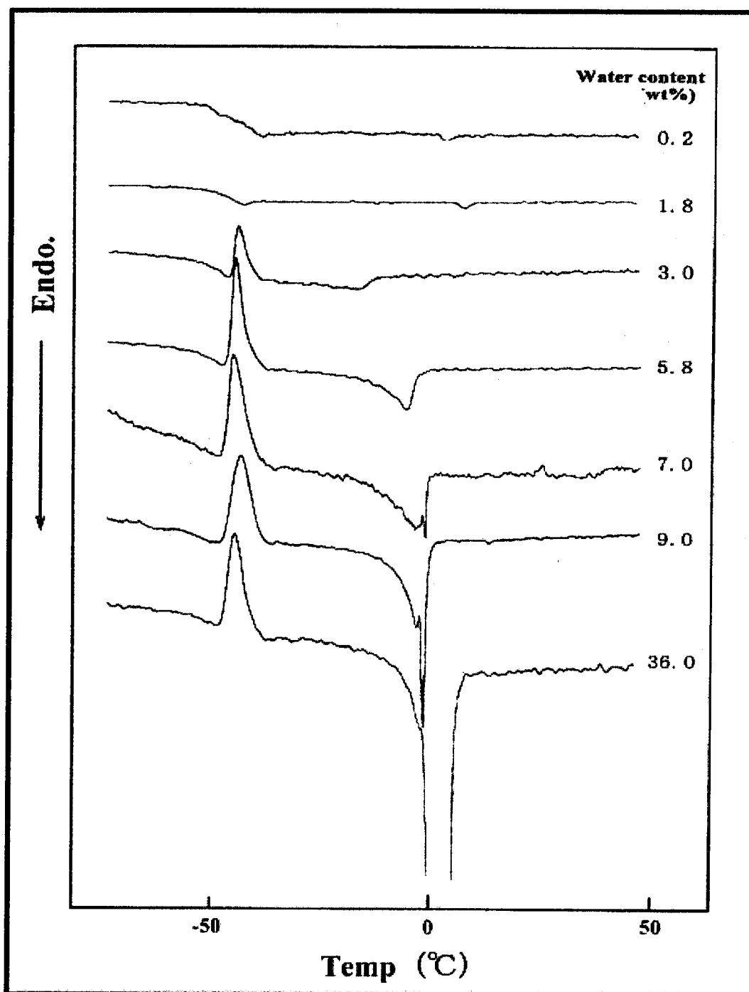
Figure 5-4. DSC heating curves of PMEA-water system : heating rate=2.5 °C / min.
