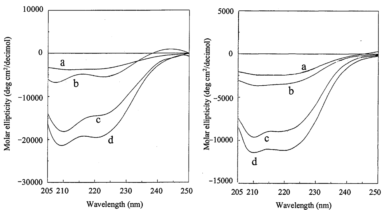
Figure 4-10. CD spectra of proteins adsorbed on polymer surfaces. (a) BSA (b) Fibrinogen, Native protein dissolved in phosphate buffer solution (37°C, pH 7.4). a:PP b:PHEMA c:PMEA d: native protein.
