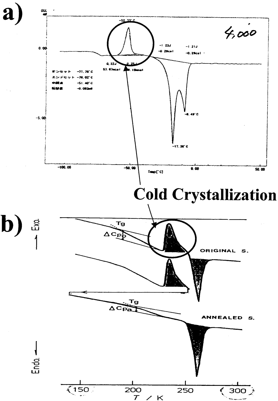
Figure 5-19. DSC heating curves for (a) PEG- and (b) polysaccharide-water systems.
