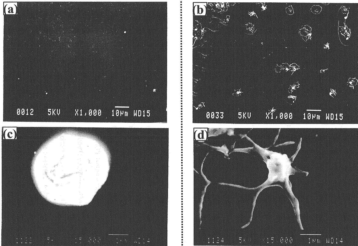
Figure 2-8. Scanning electron micrographs of washed platelets adhered to polymer precoated with FNG or noncoated. (a)PMEA (b)PHEMA (magnification \times 1,000 ) (c)PMEA (d)PHEMA (magnification \times 15,000 )
