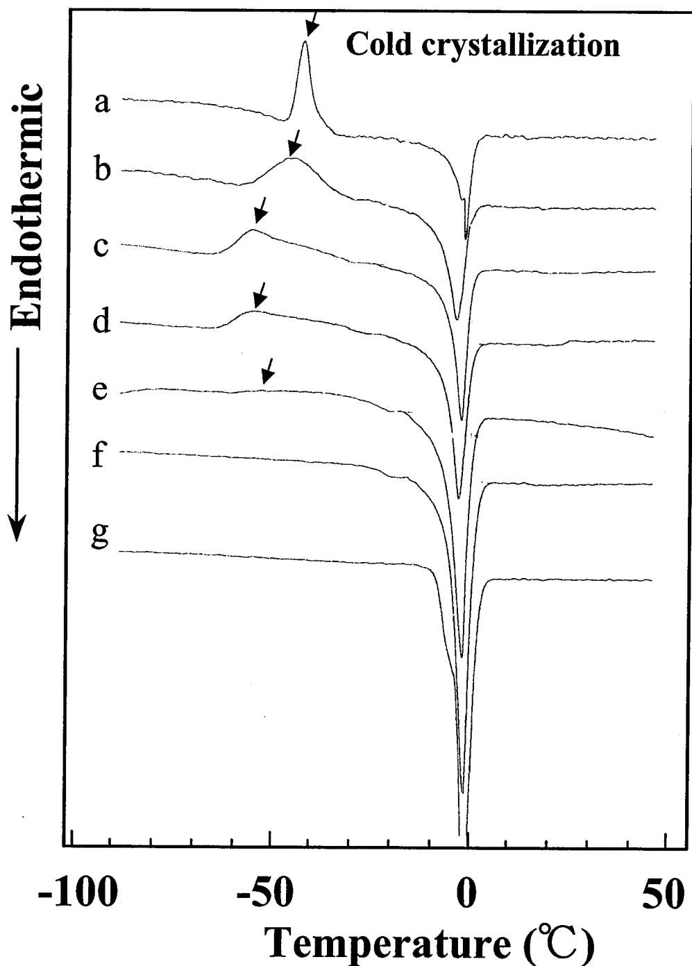
Figure 5-10. DSC heating curves of poly(MEA-co-HEMA) with EWC. heating rate=2.5 °C/min. HEMA content in copolymer (mol%) : (a) 0 (PMEA), (b)10, (c)20, (d)30, (e)40, (f)50, (g)100 (PHEMA).
