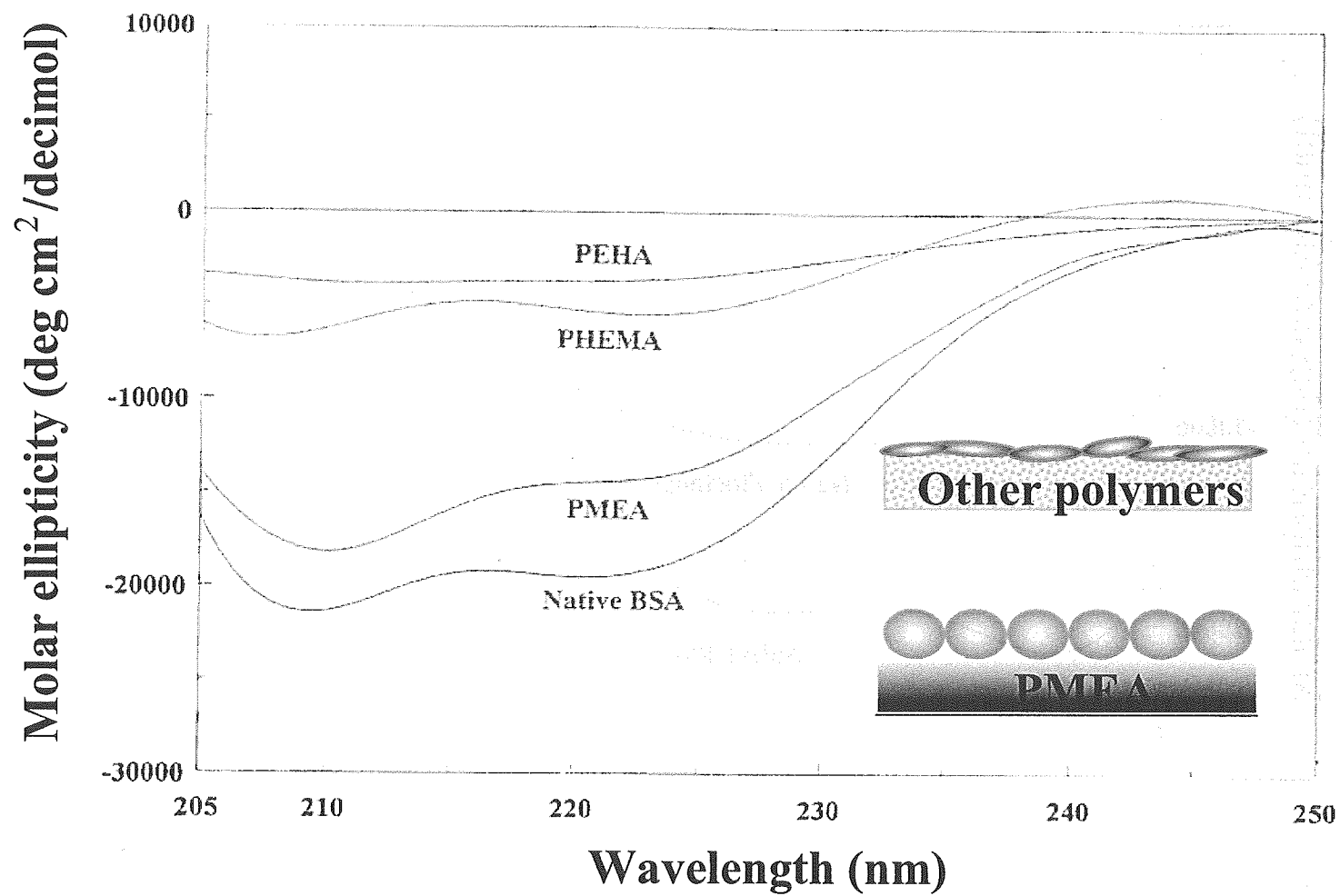
Figure 3-5. CD spectra of BSA adsorbed onto the surface of polymers (pH 7.4, 37 °C)
