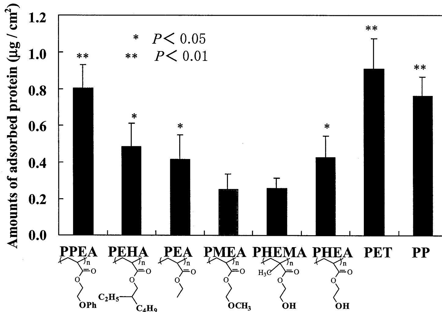
Figure 3-2. Total amount of proteins from human plasma adsorbed onto the surface of polymers. (* P < 0.05 vs PMEA; ** P < 0.01 vs PMEA, Mean \pm standard deviation, n=5 )
