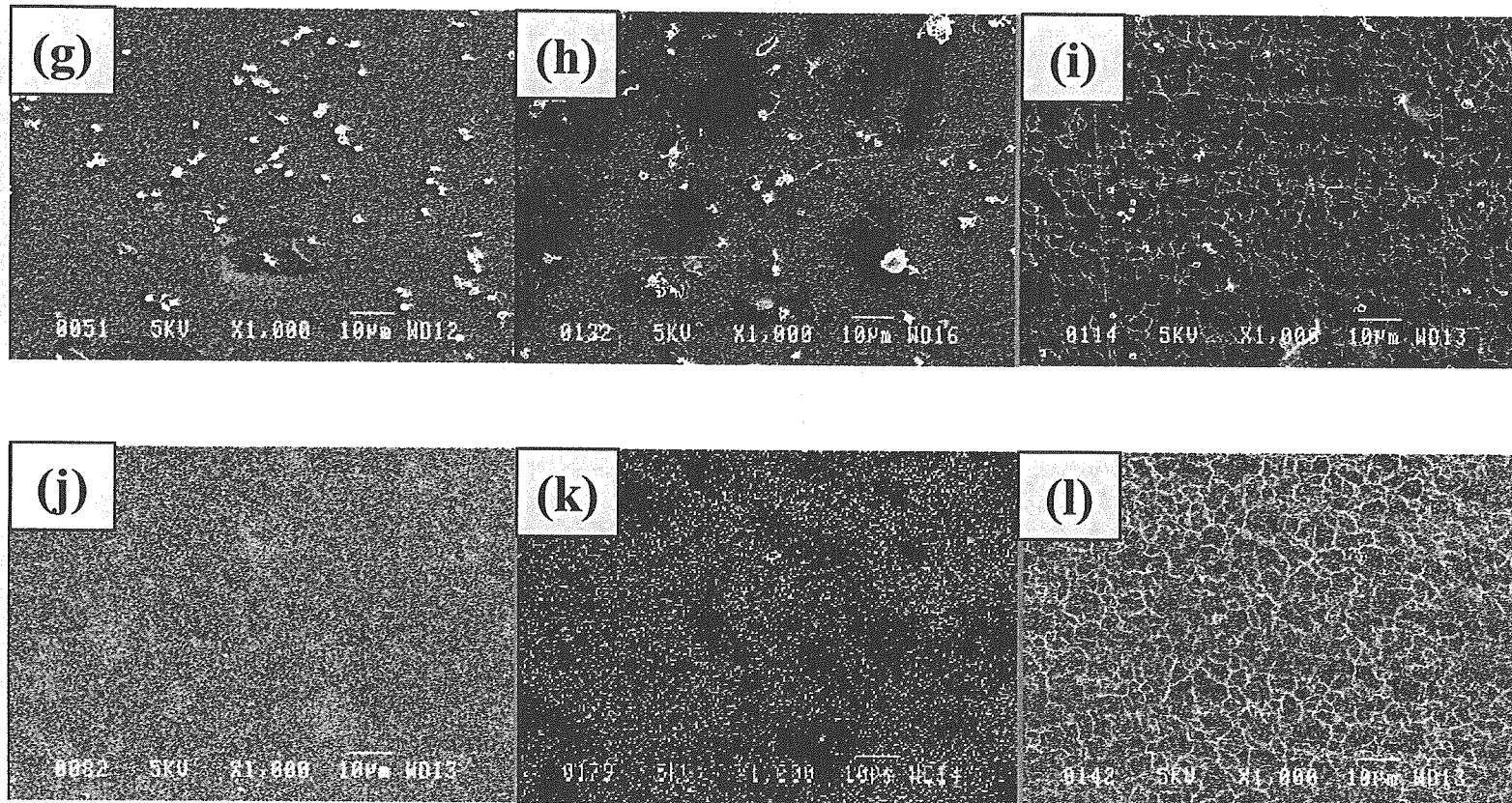
Figure 2-13. (Continued) (g, j) PU(polyurethane), (h, k) PET(polyethyleneterephthalate), (i, l) SUS(stainless steel) (g,h,i) without PME A coating, (j,k,l) with PME A coating
