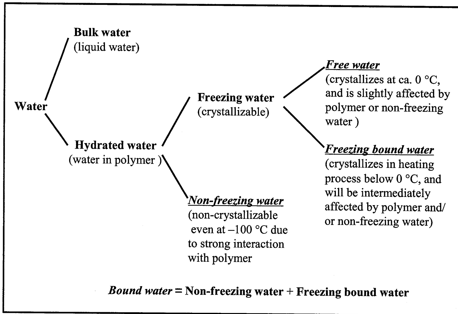
Figure 5-6. Classification of water in hydrated polymer based on DSC analysis.
