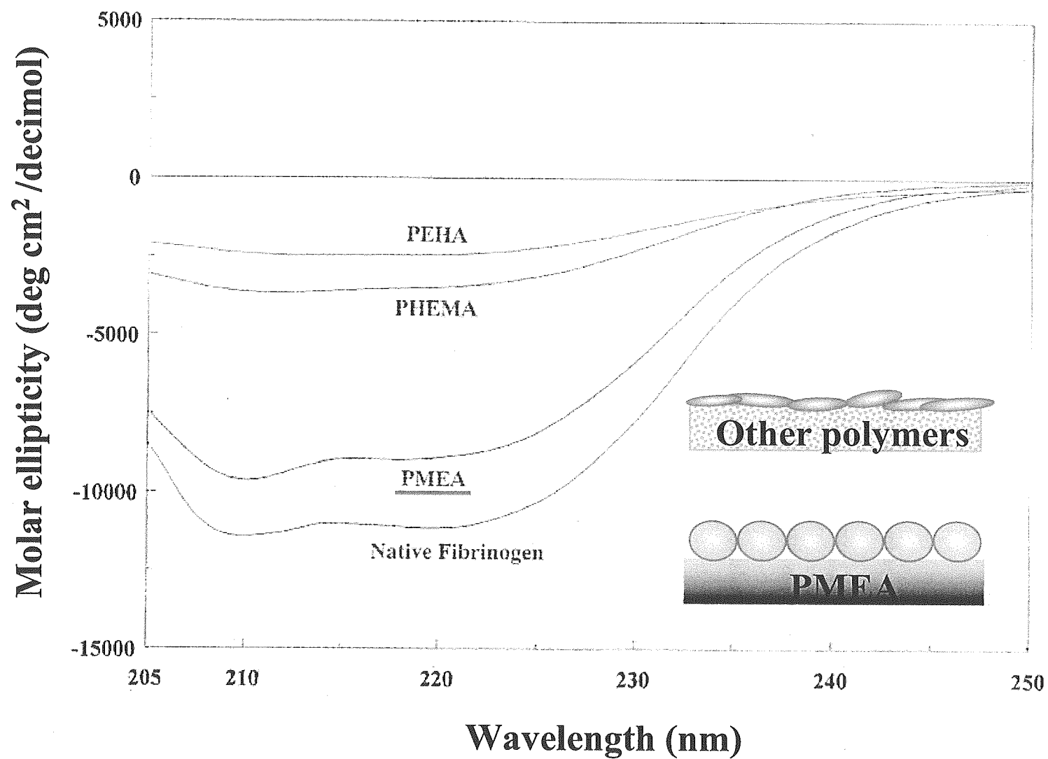
Figure 3-6. CD spectra of FNG adsorbed onto the surface of polymers (pH 7.4, 37 °C ).
