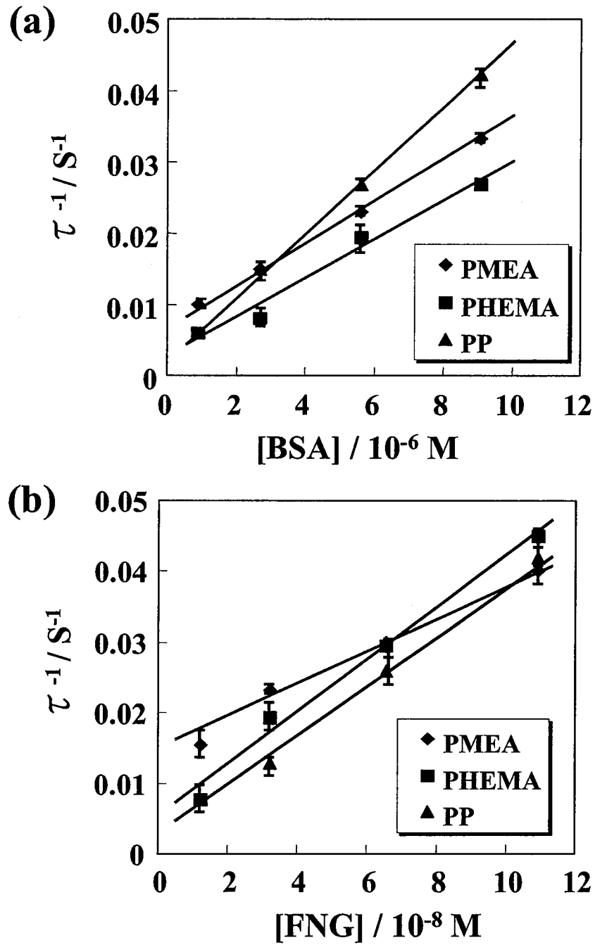
Figure 4-8. Reciprocal plots of relaxation time ( \tau ) against concentrations of protein ( n=4-6 , mean \pm SD). (a) BSA (b) Fibrinogen
