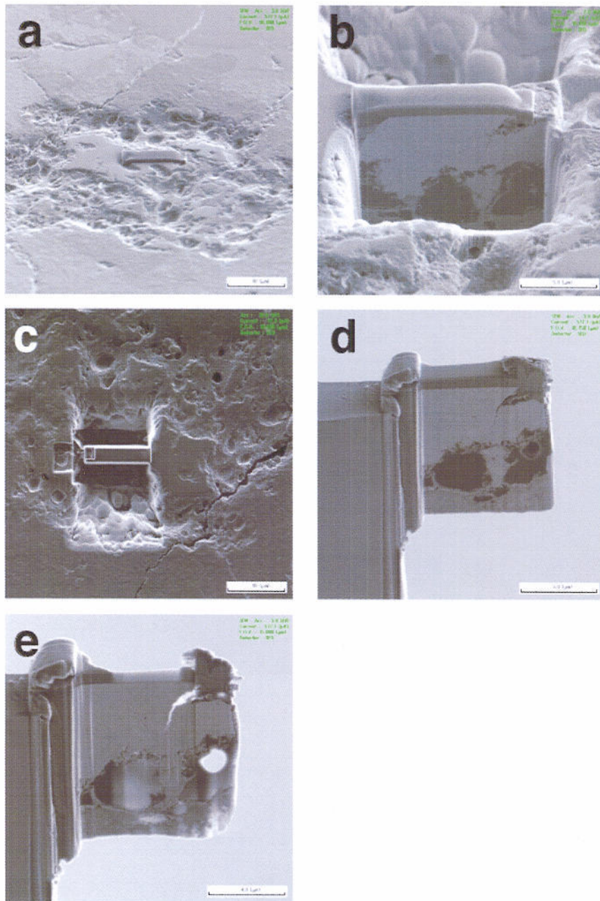
Figure 5 Sample preparation procedure with focused ion beam instrument for the transmission electron microscopy. (a) Target region of grain #17 (see Figure 8) is protected by carbon deposit. (b) (c) Digging surrounded area by Ga ion beam. (d) Lifted up by manipulator from thin section and set to the silicon pillar (right) with carbon deposit. (e) Treated by Ar gas to reduce the damage layer after thinning by Ga ion beam. Finally the sample size become \sim 8 \mu\text{m} \times 8 \mu\text{m} \times 50\text{nm} . FIB sample preparation is assisted by T. Kaito and I. Nakatani.
