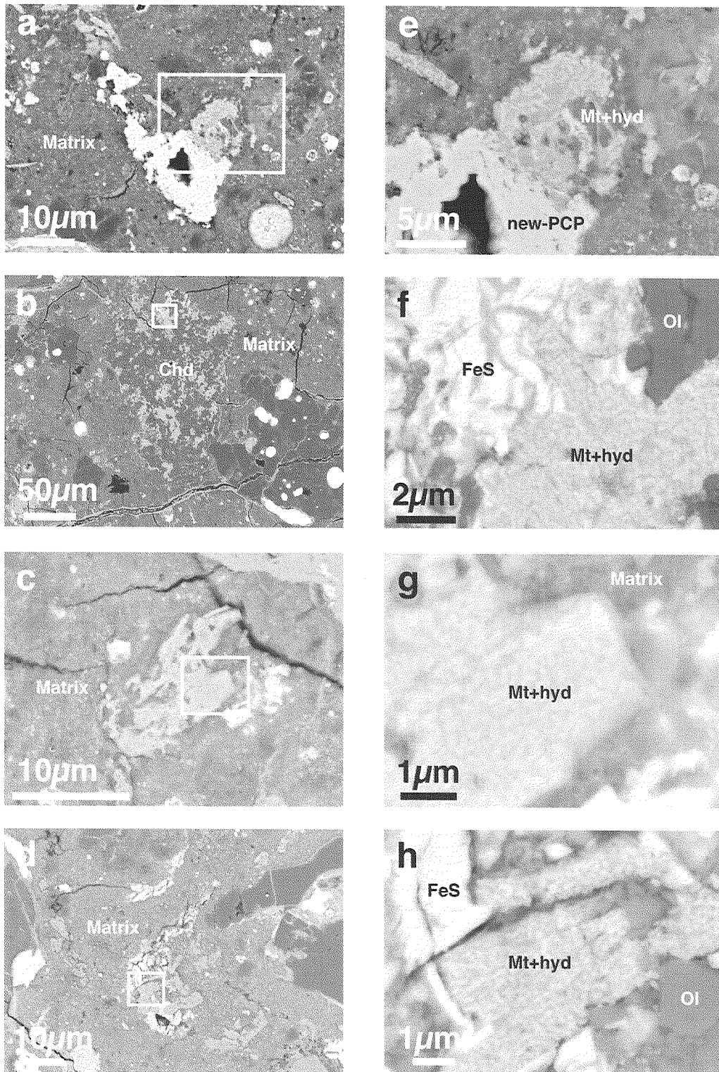
Figure 17 Granular iron oxides/hydroxides in Acfer 094. (e to h) are magnified images of square (a to d) respectively. Ol:olivine, FeS: fractured FeNi-sulfide, hyd: Fe-oxyhydroxide, Mt:sulfur-free iron oxide (magnetite)
