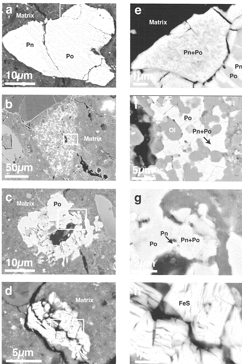
Figure 15. Different types of iron-nickel sulfides in Acfer 094 classified by the appearances. (e to h) are magnified images of square in (a to d) respectively. Pn: pentlandite, Po: pyrrhotite (or troilite), Ol: olivine, FeS: fractured FeNi-sulfide
