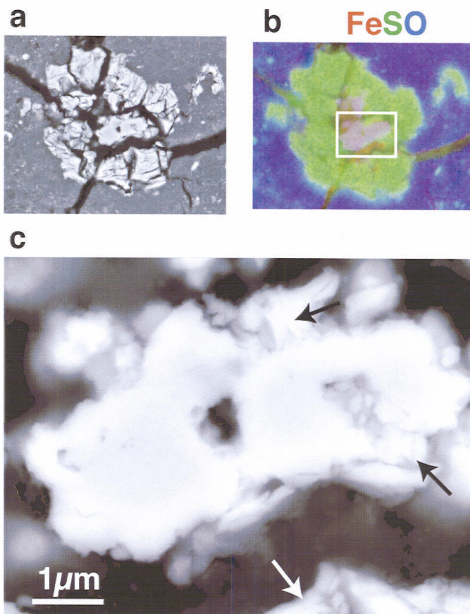
Figure 14. (a) Backscattered electron (b) X-ray Elemental map of new-PCP #21 which Fe is red, S is Green and O is blue. Purple color indicates new-PCP in (b). (c) Close up image of squared area. Arrows indicates FeS.
