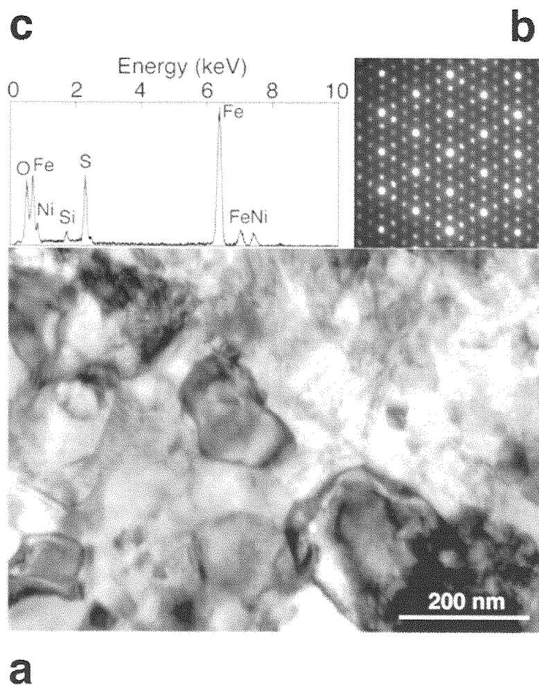
Figure 13 (a) Transmission electron micrograph showing the texture of new-PCP. (b) A diffraction pattern and (c) an X-ray elemental spectrum from a single new-PCP grain. The main spots in the diffraction pattern are similar to those of magnetite (space group Fd3m ); the weak extra spots indicate a 3-fold superstructure. This pattern is viewed along [111] of the Fd3m cell of the main spots. These data are produced by Dr. Seto.
