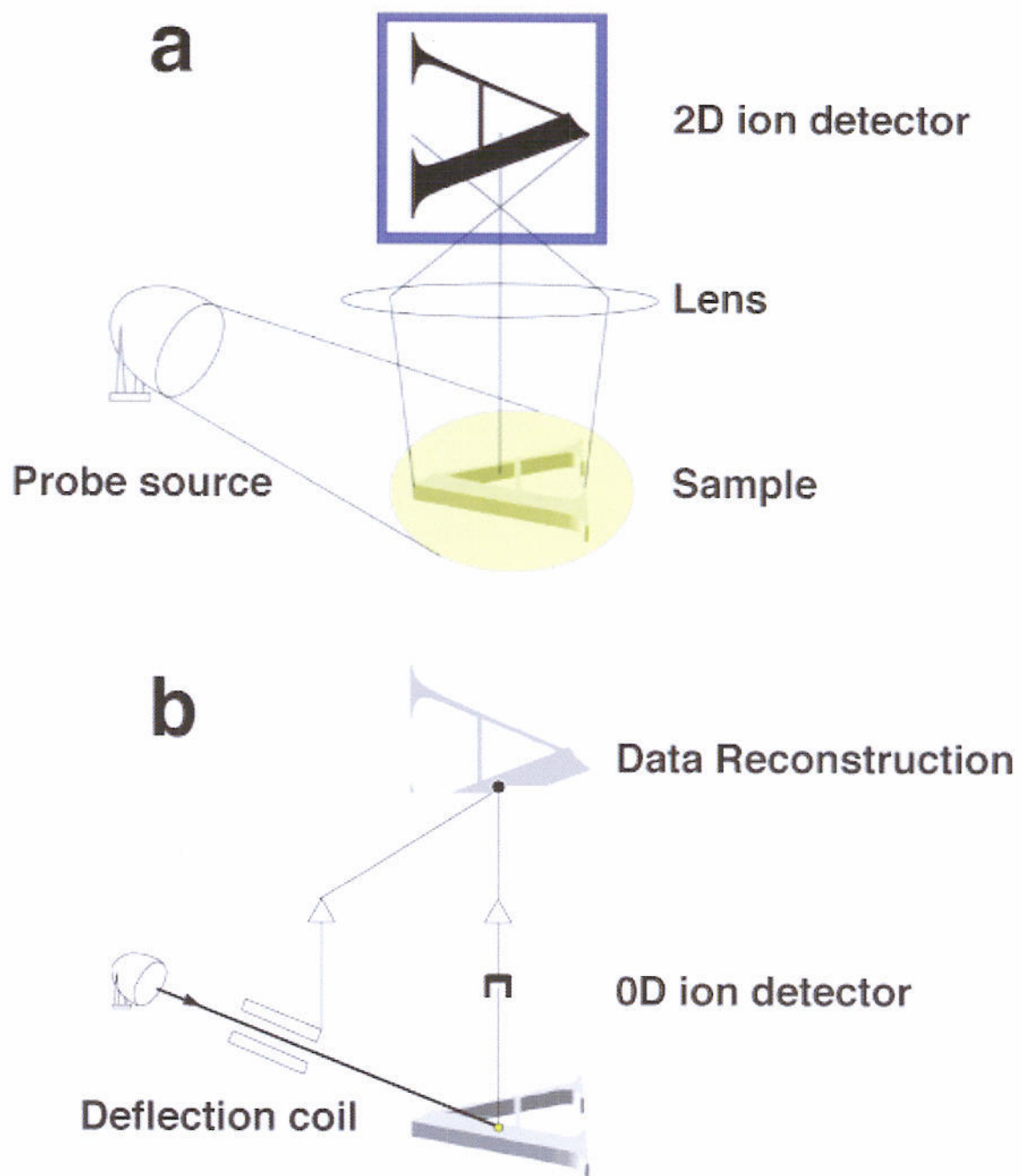
Figure 2 Illustration of isotope imaging methods. (a) Direct-imaging method (b) Scanning method
