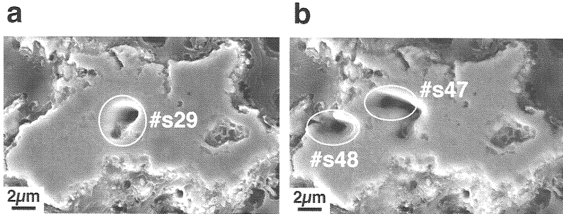
Figure 10. Secondary electron images of new-PCP #17 (Figure 7i) after point SIMS analysis. #s29 in a white circle of (a) and #s47, #s48 in (b) indicates analyzed points and probe shapes. The data of #s48 is not presented in this thesis because the isotope ratio data was unstable during measurement probably caused by the effect of surrounded epoxy.
