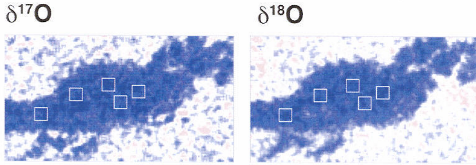
Figure 8. Example of quantification from isotope ratio images (y and z in Figure 7). White squares are selected regions of interests (ROI). The pixels of ROIs without moving averaged data are averaged to estimate the quantitative value. Color scale is same as Figure 7.
