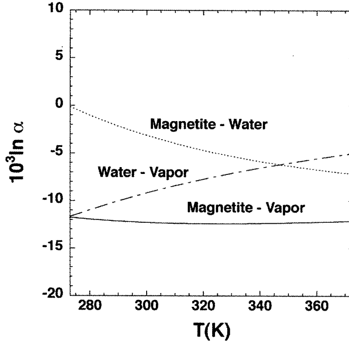
Figure 24. Isotopic fractionation factors ( ^{18}\text{O}/^{16}\text{O} ) between magnetite and water liquid or vapor. \alpha is ^{18}\text{O}/^{16}\text{O} ratios fractionation between phases.
