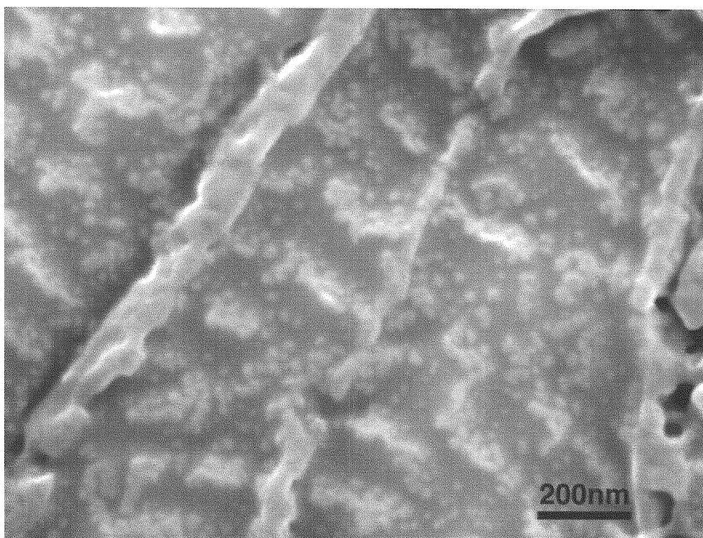
Figure 22. Secondary electron image of PCP grain #38 after spattered by \text{Cs}^+ ions
