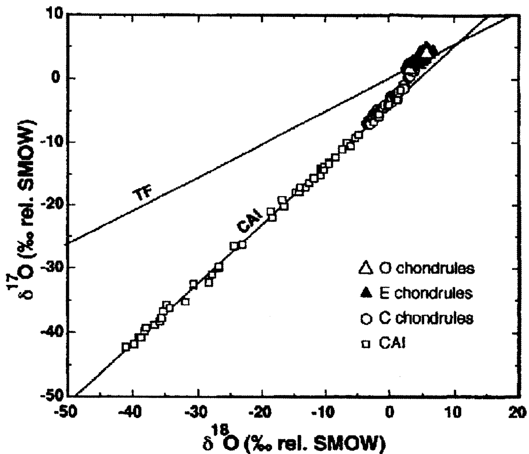
Figure 1 Mass independent fractionation of oxygen isotopes in meteorites (Clayton, 1993).
