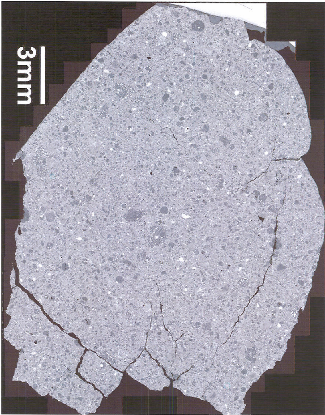
Figure 4 Backscattered electron image of Acfer 094 polished thin section.
