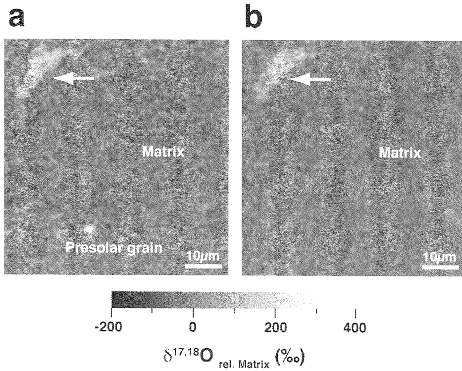
Figure 6. Spatial distribution of ^{17}\text{O}/^{16}\text{O} (a) and ^{18}\text{O}/^{16}\text{O} (b) in matrix of the ungrouped carbonaceous chondrite Acfer 094 measured using isotopography. An isotopically anomalous 10 \mu\text{m} -sized region and a spot are surrounded by the matrix materials. The spot corresponds to a presolar silicate grain. Arrows indicate the existence of ^{17,18}\text{O} -rich material.
