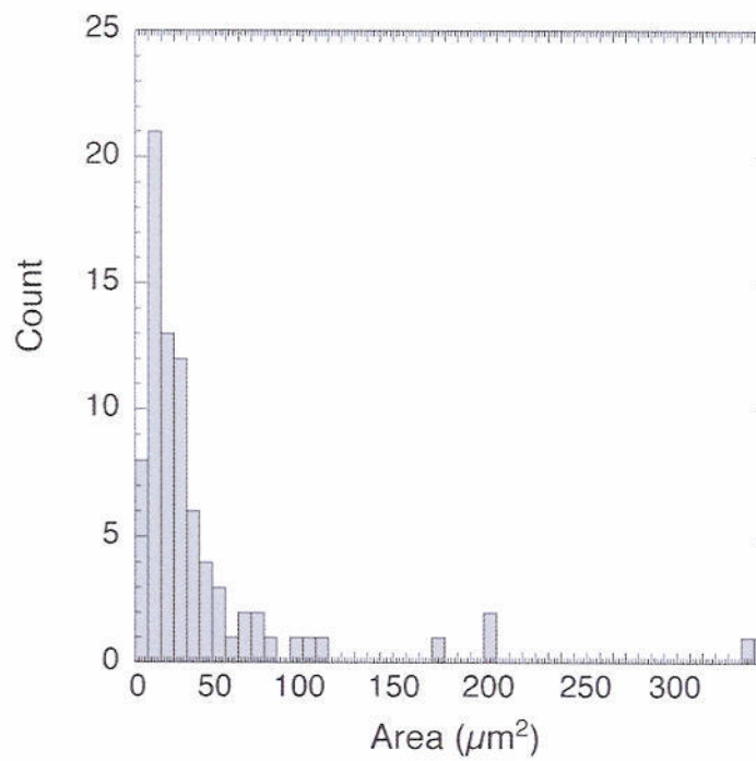
Figure 19 Size distribution of new-PCP. The bin size of this histogram is 7\mu\text{m}^2 .
