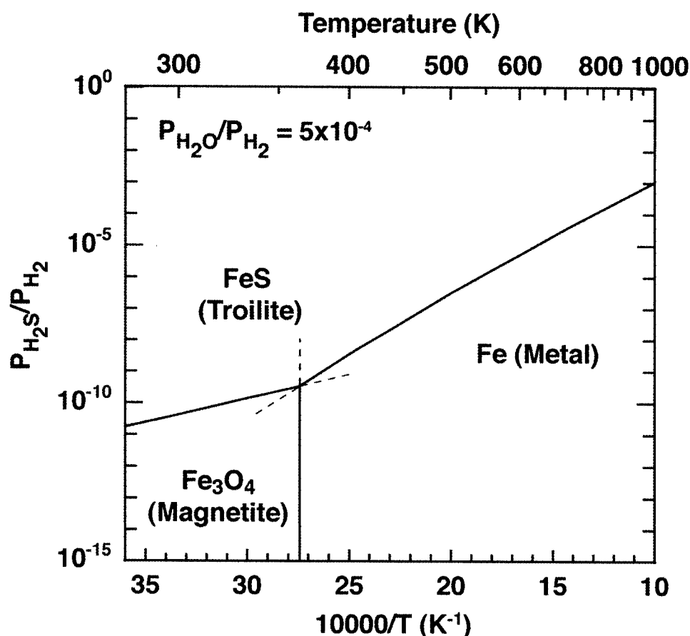
Figure 23. Calculated equilibrium temperatures for Fe-metal, troilite (FeS) and magnetite ( \text{Fe}_3\text{O}_4 ) as a function of P_{\text{H}_2\text{S}}/P_{\text{H}_2} ratio. The magnetite phase boundary is calculated assuming canonical solar nebular \text{H}_2\text{O}/\text{H}_2 ratio of 5 \times 10^{-4} (Krot et al. , 2000). Magnetite is considered as a proxy of a new-PCP. Thermodynamic data from JANAF tables (Chase, 1998) were used for calculations.
