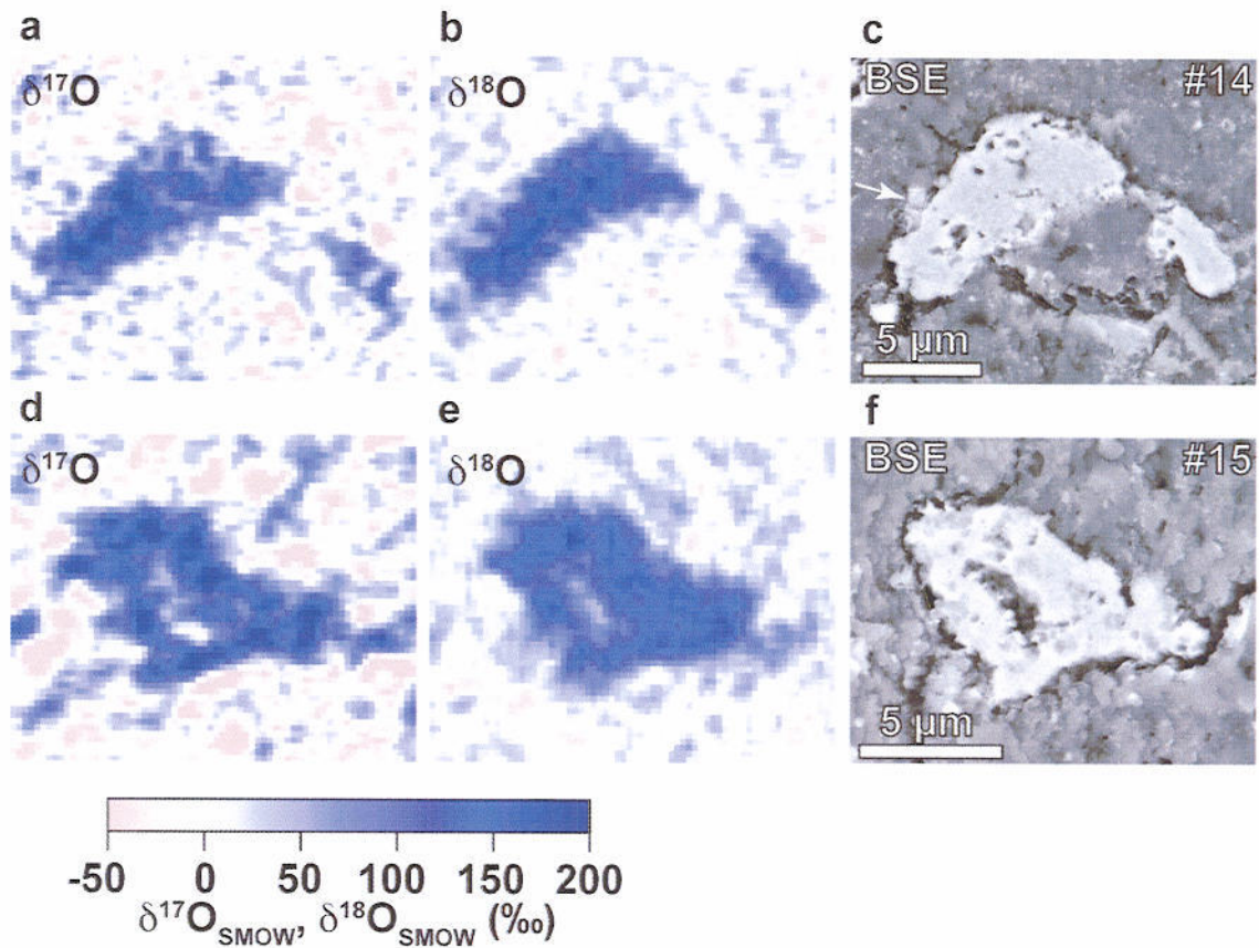
Figure 7. Oxygen isotopic distribution and grain shape for new-PCP embedded in chondrite matrix. \delta^{17}\text{O}_{\text{SMOW}} (a, d, g, j, m, p, s, v, y, B), \delta^{18}\text{O}_{\text{SMOW}} (b, e, h, k, n, q, t, w, z, C) and backscattered electron (c, f, i, l, o, r, u, x, A, D) images 10 for new-PCP #14 (a-c), #15 (d-f), #17 (g-i), #19 (j-l), #20 (m-o), #21 (p-r), #22 (s-u), #24 (v-x), #25 (y-A), and #27 (B-D) in the Acfer 094 matrix. Arrow in (A) indicates small troilite grains attached to the new-PCP #14. The new-PCP #21 is surrounded by troilite. Because troilite contains no oxygen, the troilite area and gaps filled with epoxy in (#17, #21, #22, #24, #25) is masked by black color. The color bar is same in all isotope ratio images. The new-PCPs are highly enriched in ^{17}\text{O} and ^{18}\text{O} isotopes relative to the matrix.
