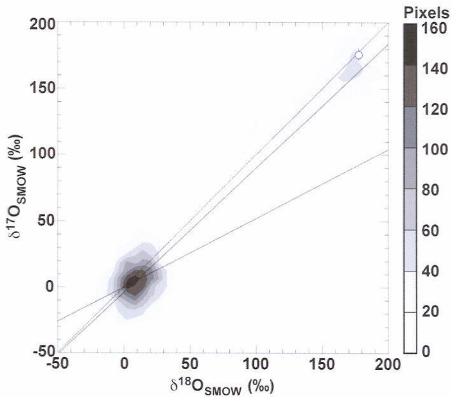
Figure 9. Comparison with two-dimensional histogram of all pixels data in the isotope ratio image from Figure 8 (contour) and average value of selected region of interests (open circle). The colors of contour mean numbers of pixels included in the range of oxygen isotopic compositions from moving averaged data.
