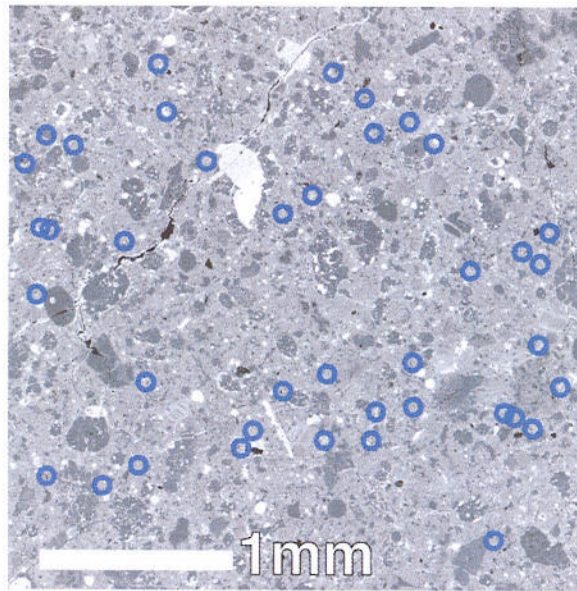
Figure 18. Spatial distributions of new-PCP in the Acfer 094 matrix. Blue circles indicate the position of new-PCP identified by the unique chemical composition.
