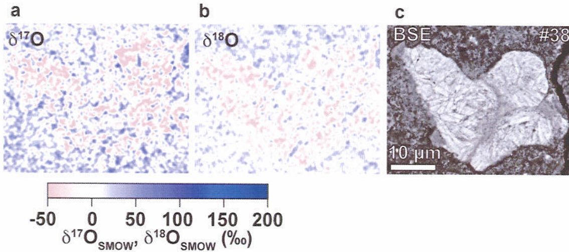
Figure 18 Oxygen isotope ratio images of \delta^{17}\text{O}_{\text{SMOW}} (a), \delta^{18}\text{O}_{\text{SMOW}} (b) and backscattered electron image (c) of Poorly Characterized Phase (PCP) in Murchison meteorite.
