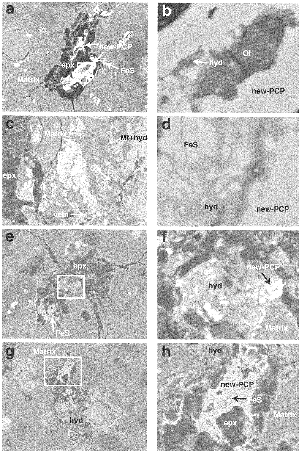
Figure 16 Morphologies of new-PCP. (b, d, f, h) are magnified images of square in (a, c, e, g) respectively. Pn: pentlandite, Po: pyrrhotite (or troilite), Ol: olivine, FeS: fractured FeNi-sulfide, hyd: Fe-oxyhydroxide, ep: epoxy
