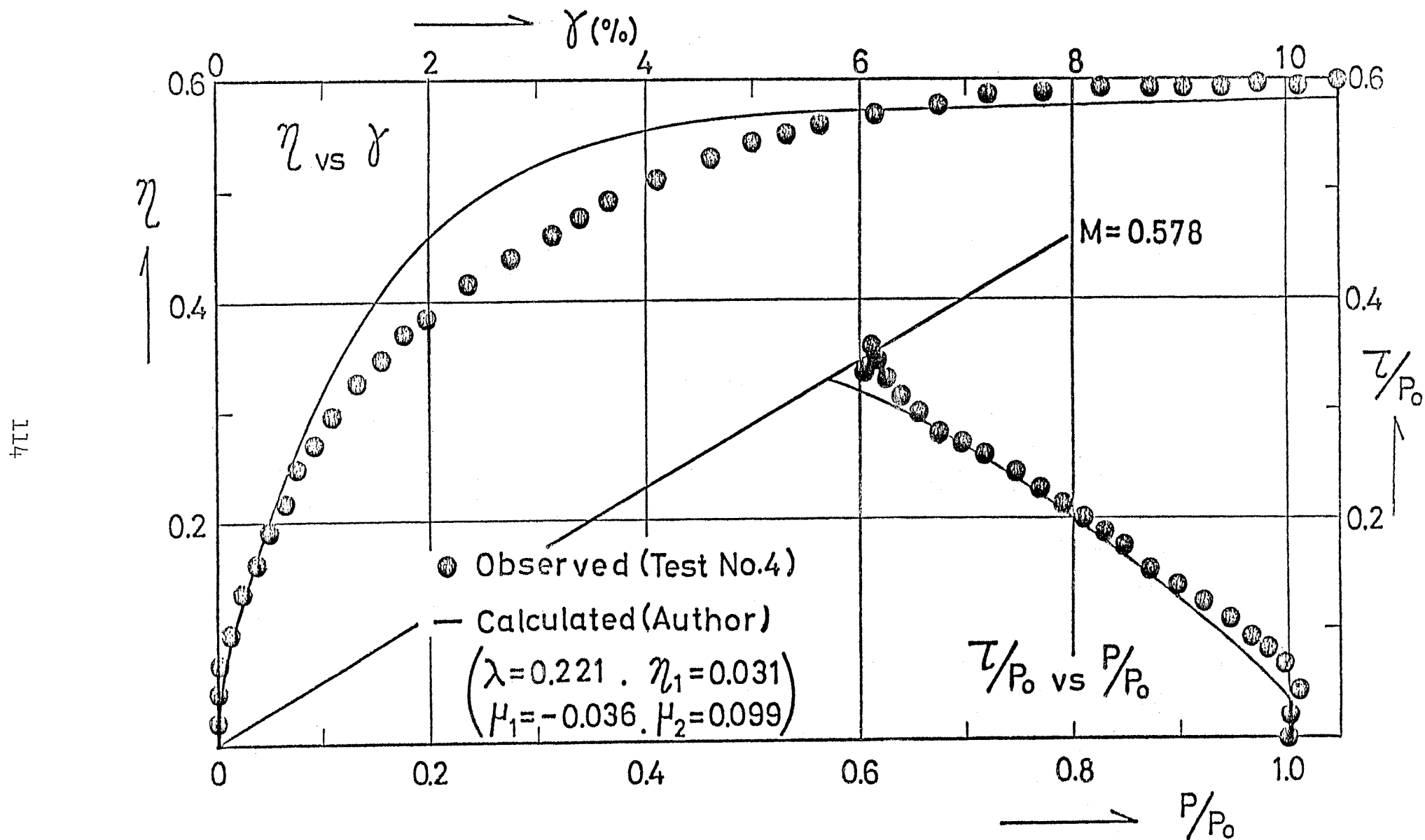
Fig.3-12 Observed and predicted stress-strain relationship by the present author
