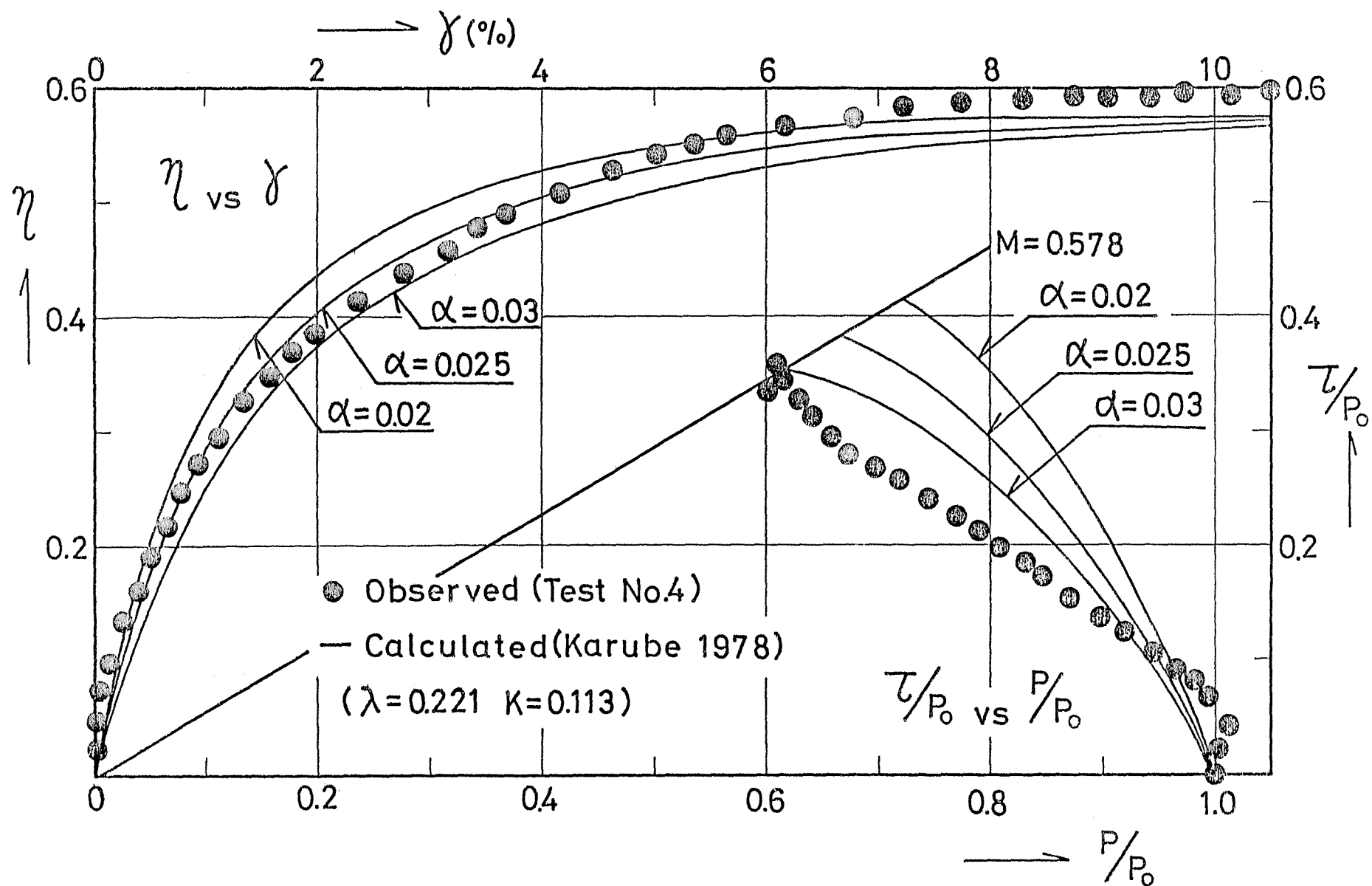
Fig.3-5 Observed and predicted stress-strain relationship by equations of Karube
