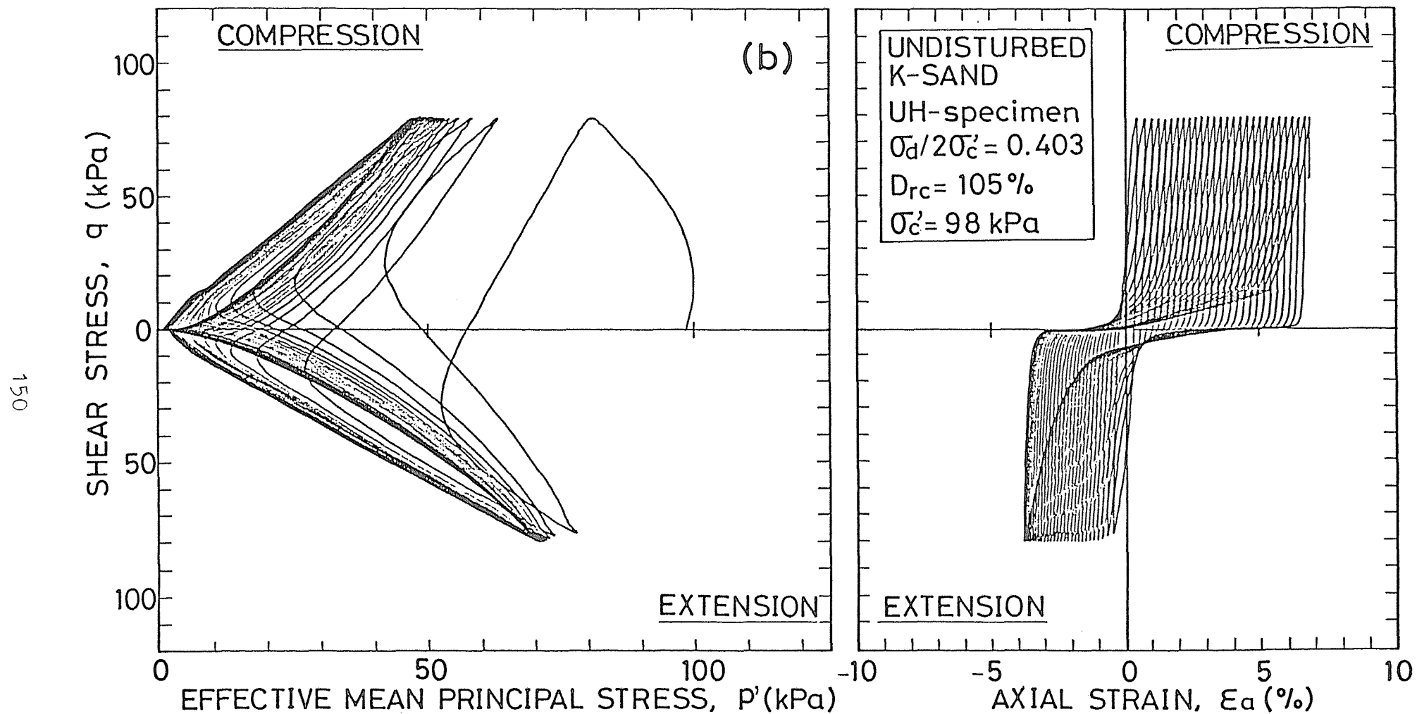
Fig.4-19(b) Time histories of undrained effective stress path and stress-strain relationship for UH-specimen of undisturbed K-sand
