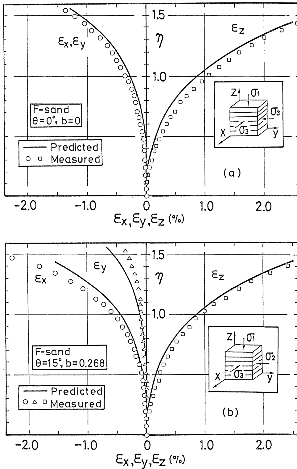
Fig.5-14 Comparisons of measured and predicted relationships between stress ratio and principal strains for F-sand in the stress paths with \theta = 0^\circ (a) and \theta = 15^\circ (b)
