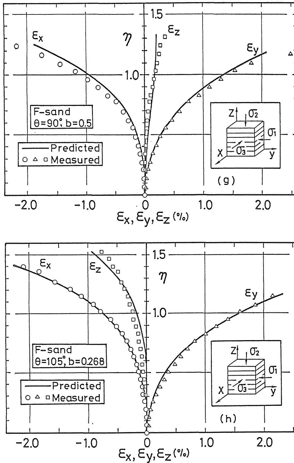
Fig.5-14 Comparisons of measured and predicted relationships between stress ratio and principal strains for F-sand in the stress paths with \theta = 90^\circ (g) and \theta = 105^\circ (h)
