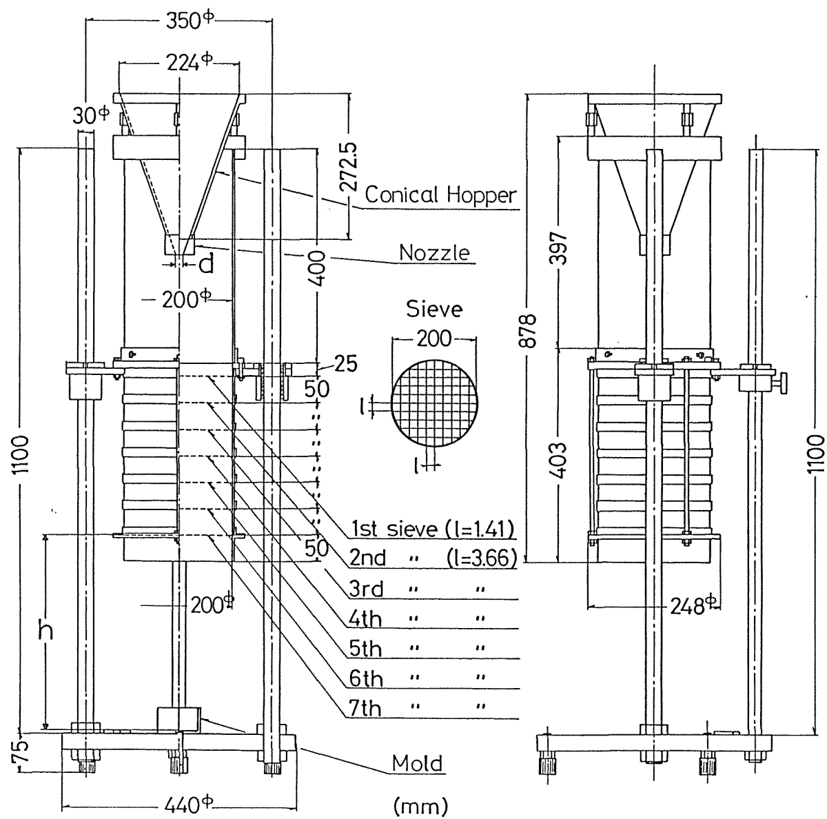
Fig.2-1 General view of multiple sieve pluviation apparatus
