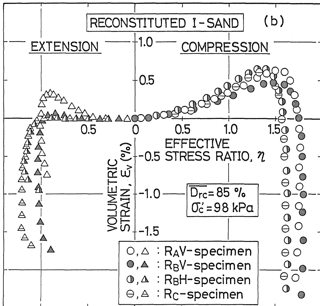
Fig.4-15(b) Variation in drained stress-strain-dilatancy relationship of reconstituted I-sand due to the effect of difference in sample preparation method ( \eta vs. \epsilon_v )
