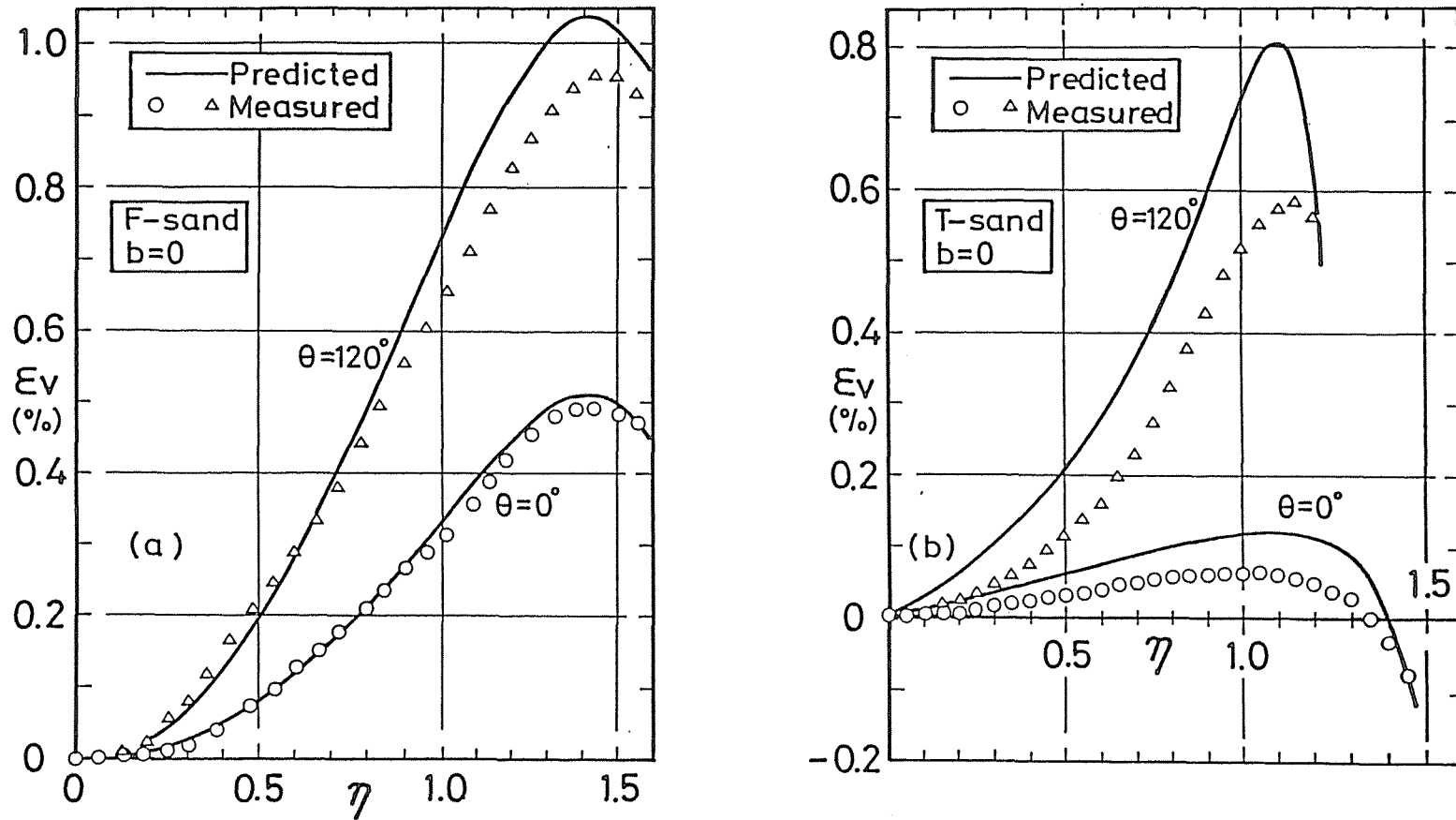
Fig.5-17 Comparisons of measured and predicted stress ratio-volumetric strain relationships in the test with the same b -value of 0 performed on; (a) F-sand (After data of Yamada and Ishihara (1979)), (b) T-sand
