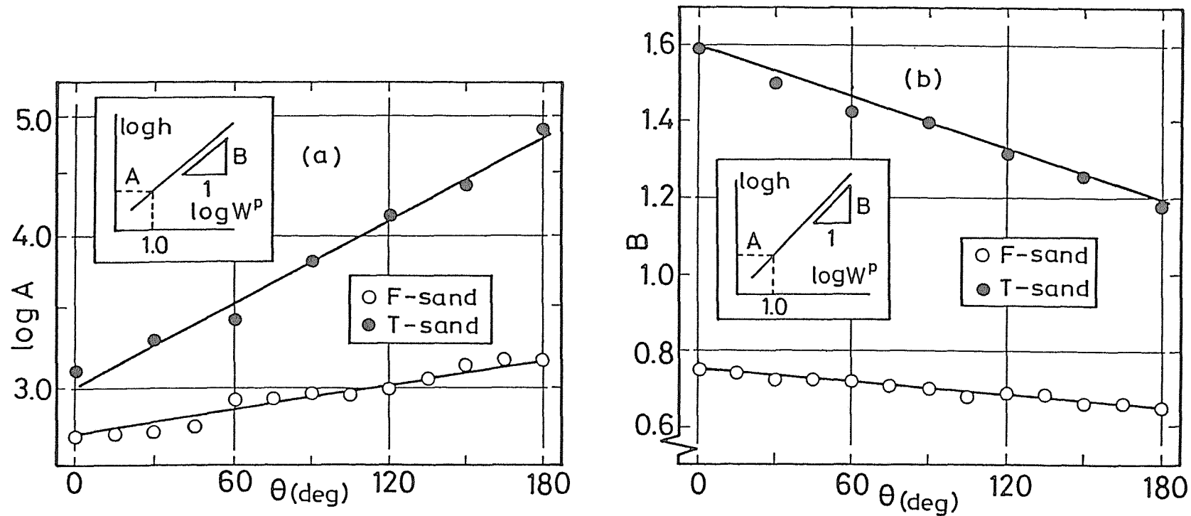
Fig.5-12 Changes in parameters A and B due to difference of stress system; (a) A vs. \theta , (b) B vs. \theta (Test data of F-sand from Yamada and Ishihara (1979))
