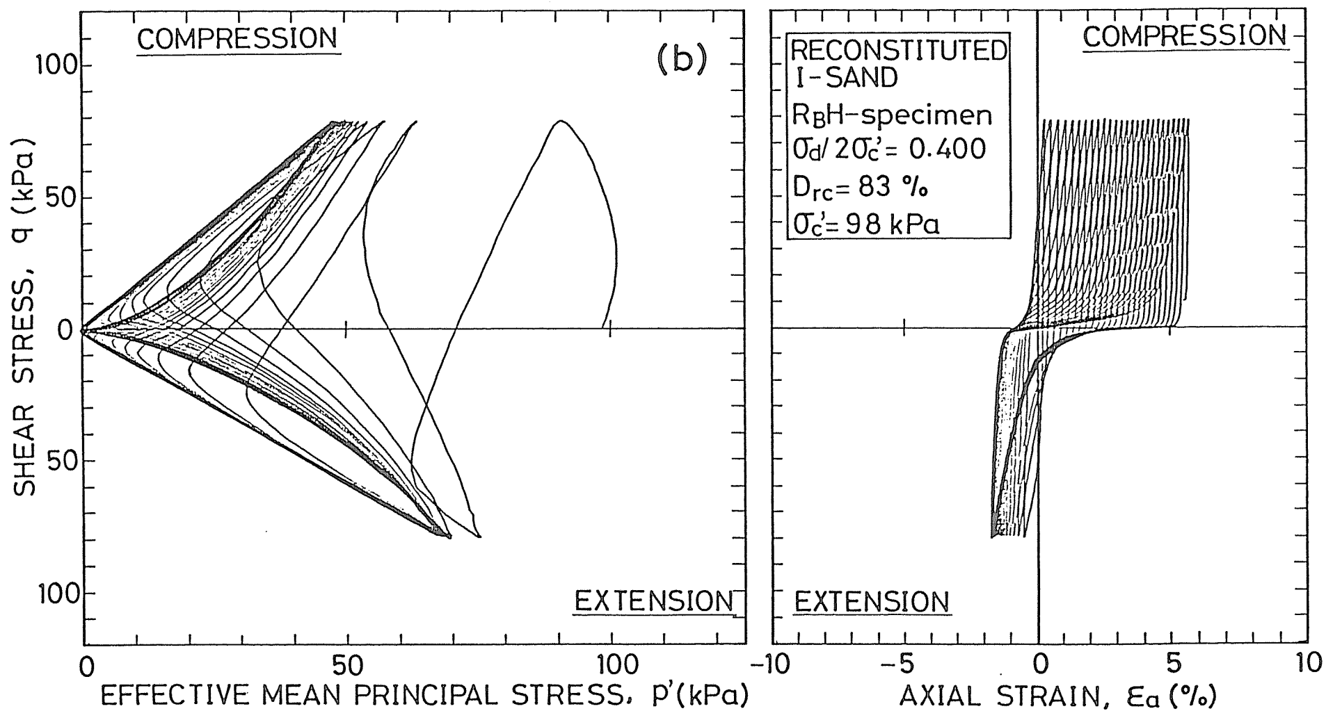
Fig.4-27(b) Time histories of undrained effective stress path and stress-strain relationship for R_B H-specimen of I-sand reconstituted by R_B method (MSP method)
