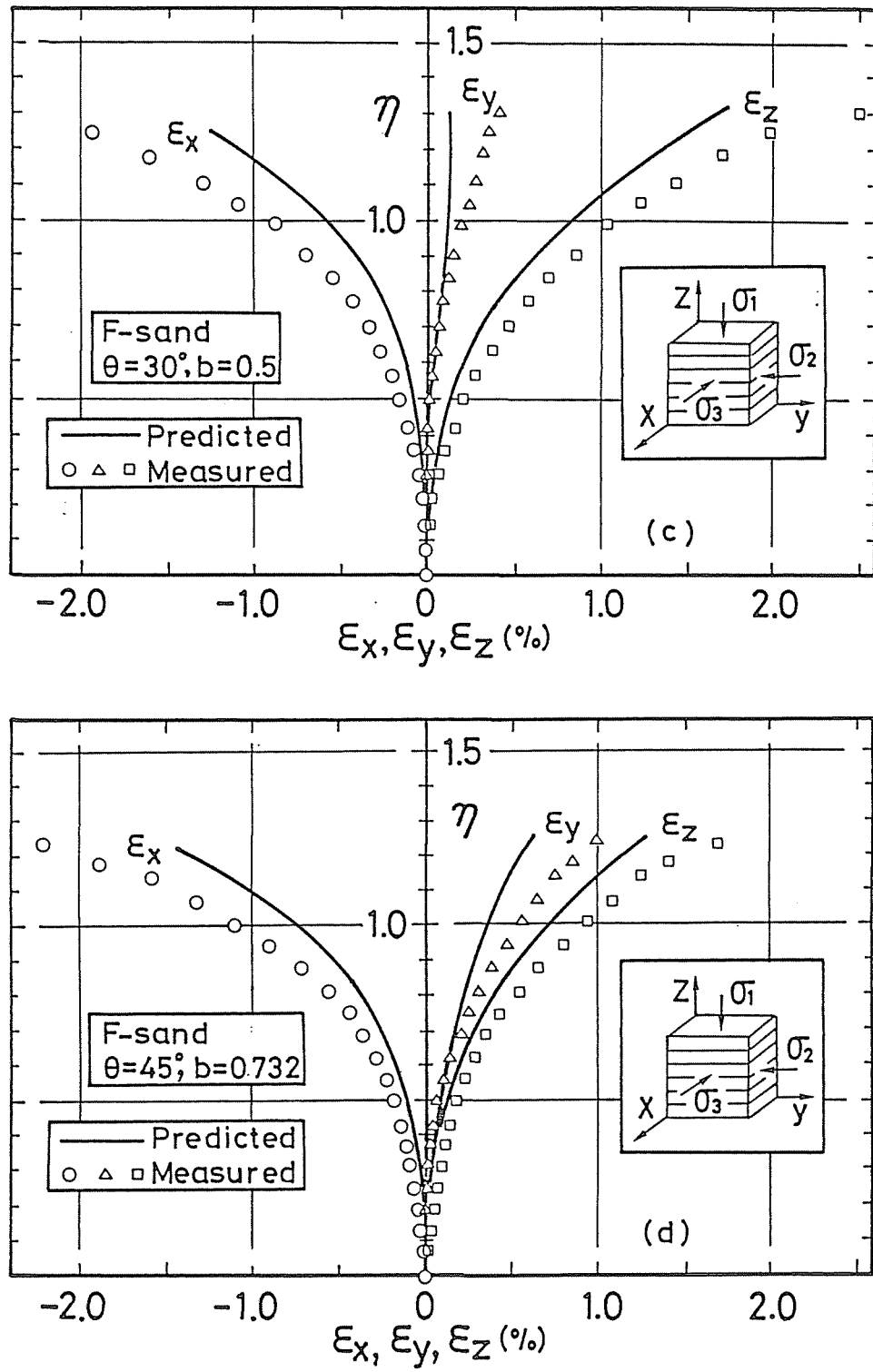
Fig.5-14 Comparisons of measured and predicted relationships between stress ratio and principal strains for F-sand in the stress paths with \theta = 30^\circ (c) and \theta = 45^\circ (d)
