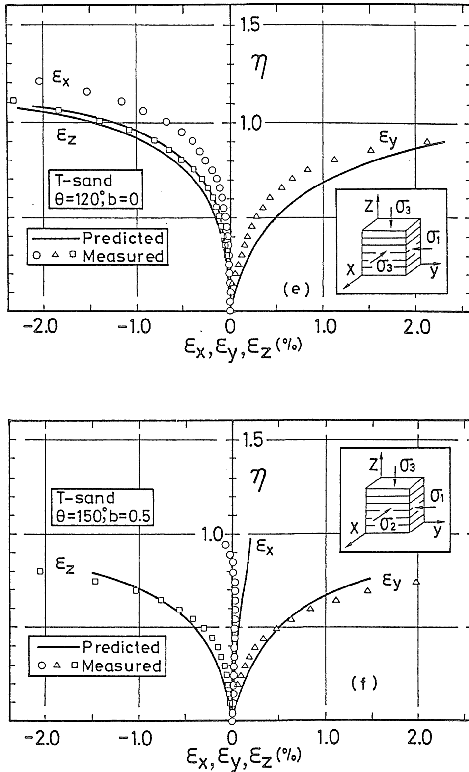
Fig.5-15 Comparisons of measured and predicted relationships between stress ratio and principal strains for T-sand in the stress paths with \theta = 120^\circ (e) and \theta = 150^\circ (f)
