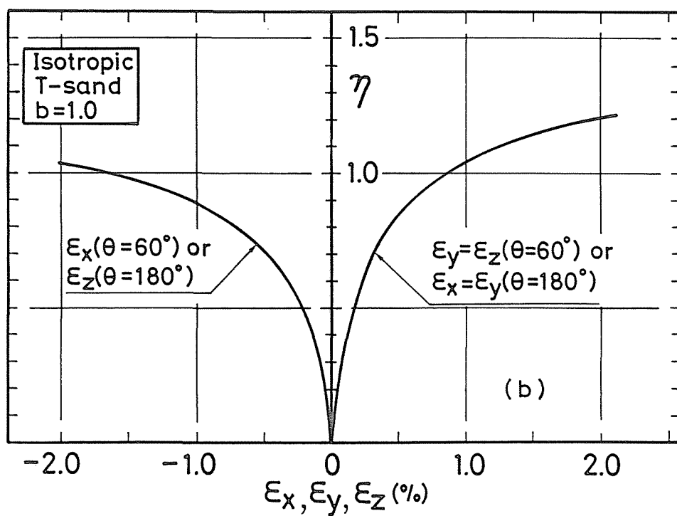
Fig.5-22 Predicted stress ratio vs. principal strains relationships for sand with isotropic fabric; (a) F-sand, (b) T-sand
