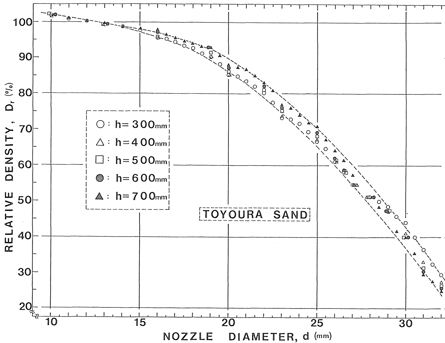
Fig.2-3 Variation of relative density of Toyoura sand with nozzle diameter
