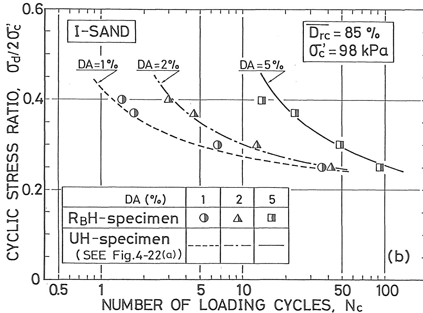
Fig.4-28(b) Comparison of cyclic stress ratio vs. number of loading cycles to 1%, 2% and 5% double amplitude axial strains relationships for reconstituted and undisturbed I-sand specimens between R B H- and UH-specimens
