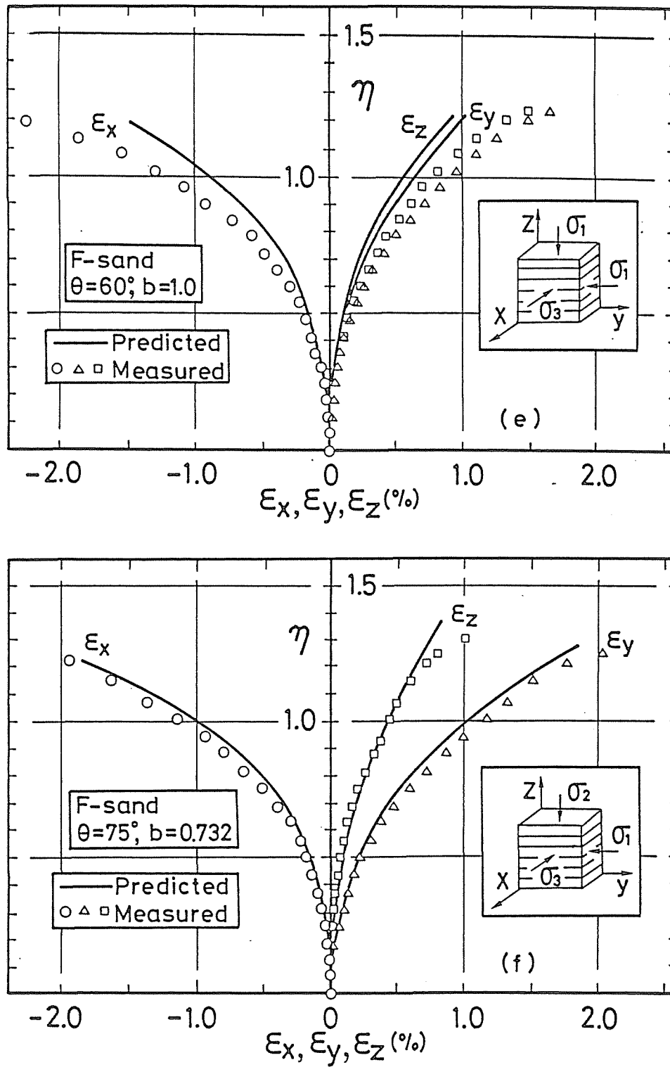
Fig.5-14 Comparisons of measured and predicted relationships between stress ratio and principal strains for F-sand in the stress paths with \theta = 60^\circ (e) and \theta = 75^\circ (f)
