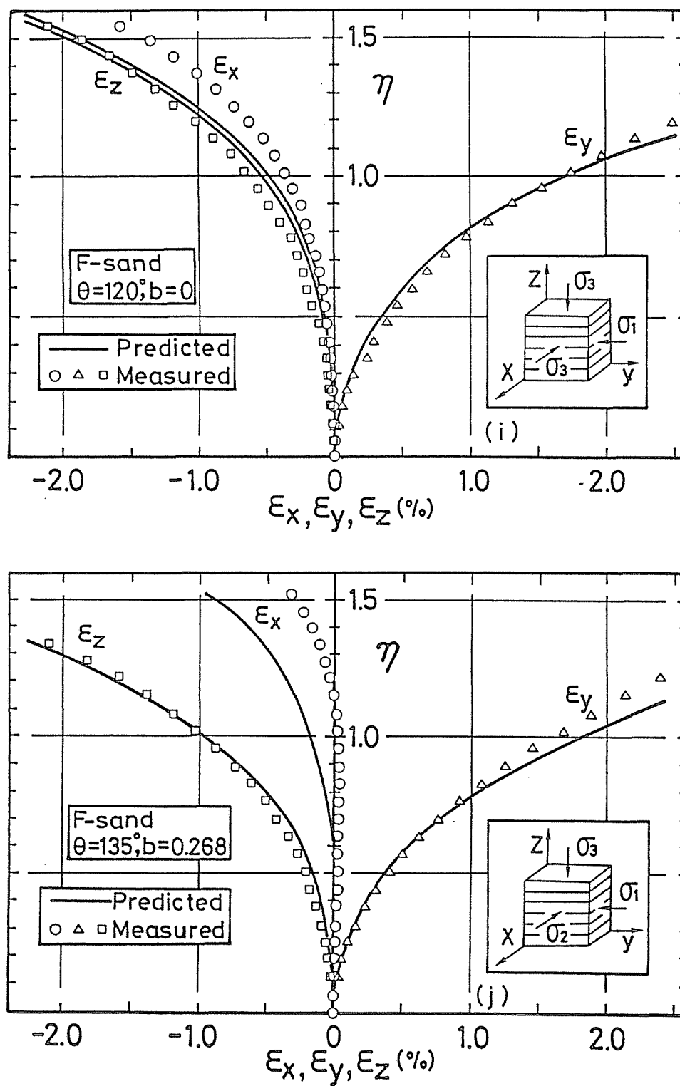
Fig.5-14 Comparisons of measured and predicted relationships between stress ratio and principal strains for F-sand in the stress paths with \theta = 120^\circ (i) and \theta = 135^\circ (j)
