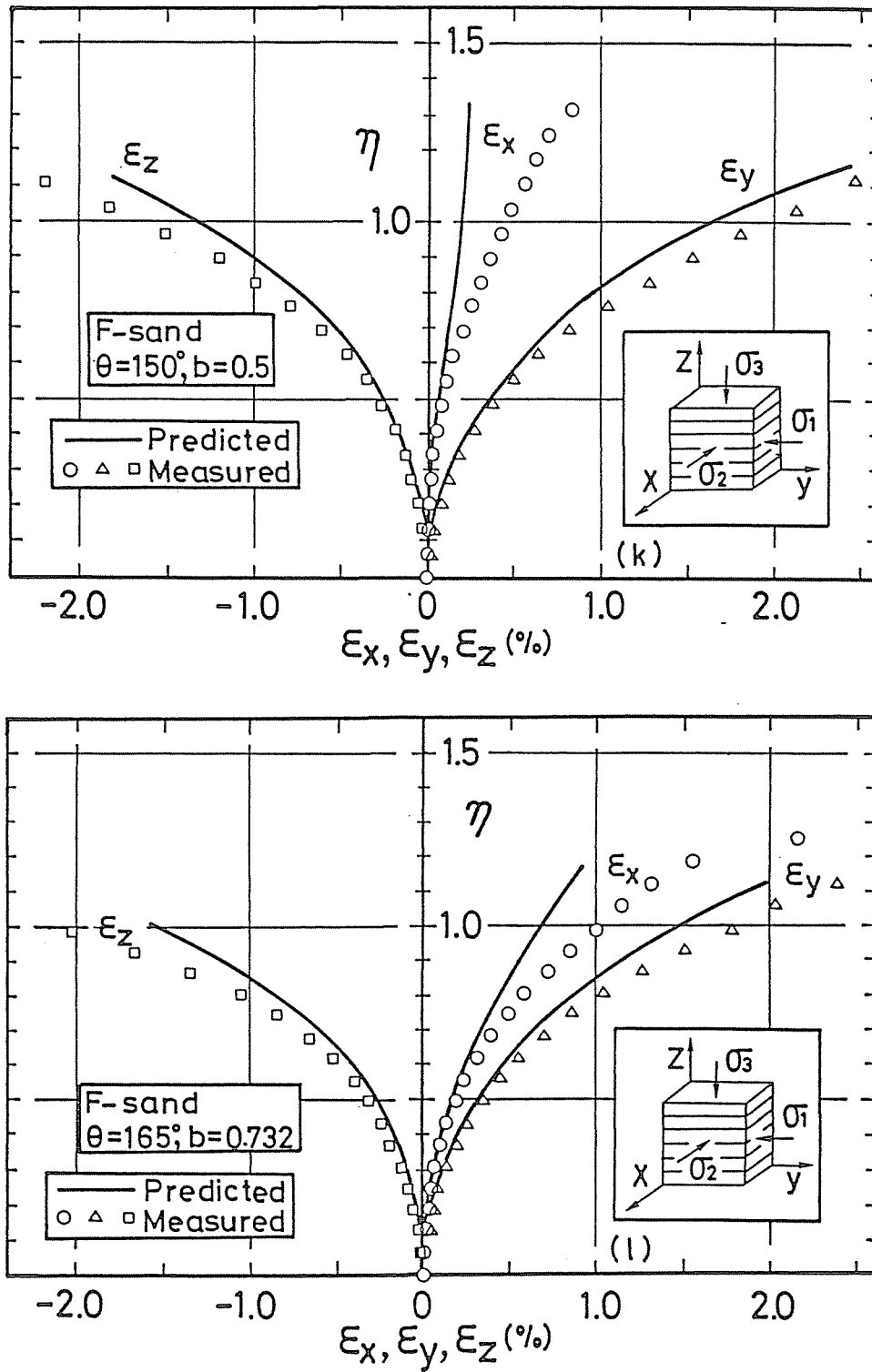
Fig.5-14 Comparisons of measured and predicted relationships between stress ratio and principal strains for F-sand in the stress paths with \theta = 150^\circ (k) and \theta = 165^\circ (l)
