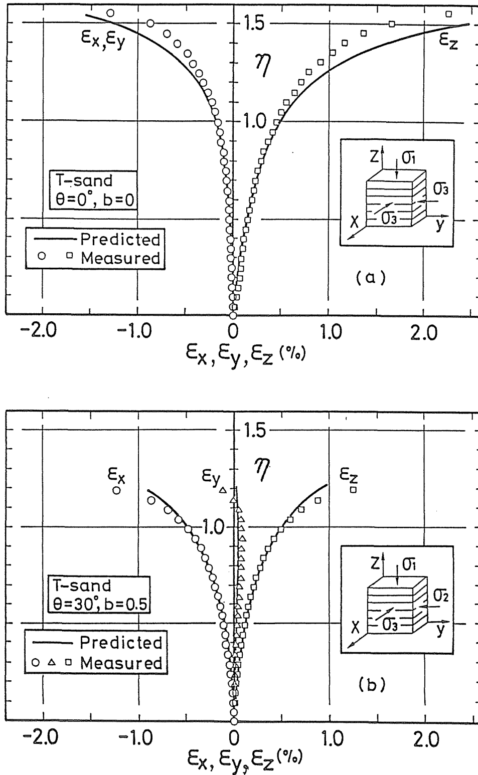
Fig.5-15 Comparisons of measured and predicted relationships between stress ratio and principal strains for T-sand in the stress paths with \theta = 0^\circ (a) and \theta = 30^\circ (b)
