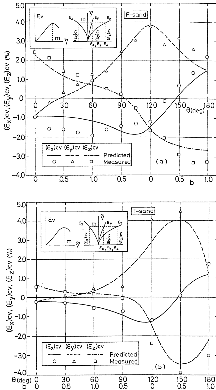
Fig.5-18 Comparisons of measured and predicted principal strains at maximum volume contraction during shear process vs. \theta ; (a) F-sand (After data of Yamada and Ishihara (1979)), (b) T-sand
