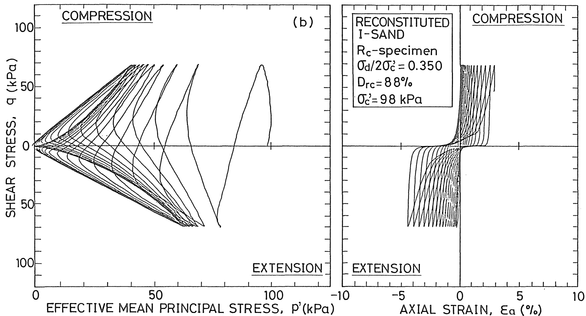
Fig.4-30(b) Time histories of undrained effective stress path and stress-strain relationship for I-sand specimen reconstituted by R_c method (rodding method)
