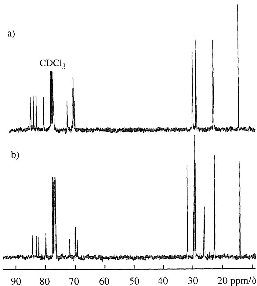
Figure 3.4. ^{13}\text{C} NMR spectra of the polymers prepared from (a) 1,2:5,6-dianhydro-3,4-di- O -pentyl-D-mannitol ( 4 ) and (b) 1,2:5,6-dianhydro-3,4-di- O -decyl-D-mannitol ( 5 ) using t -BuOK.
