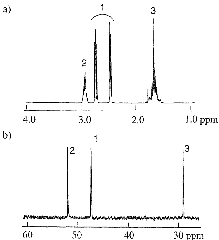
Figure 4.1. 1 H and 13 C NMR spectra of (2 S ,5 S )-1,2:5,6-diepoxyhexane ( ( 2 S ,5 S )- 31 )
