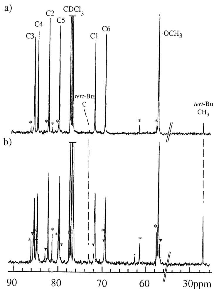
Figure 3.2. ^{13}\text{C} NMR spectra of the polymers prepared from 1,2:5,6-dianhydro-3,4-di- O -methyl-D-mannitol ( 1 ) using t -BuOK in toluene. (a): [ 1 ]/[ t -BuOK] = 20; time, 48 hours; M_n = 6410 ; M_w/M_n = 1.53 , (b): [ 1 ]/[ t -BuOK] = 5; time, 48 hours; M_n = 1590 ; M_w/M_n = 1.27 . Signals marked with asterisks and solid triangles correspond to the carbons for terminal end unit and initiating end unit, respectively.
