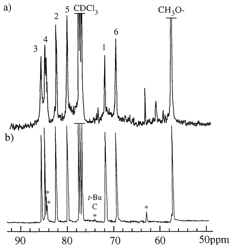
Figure 5.3. ^{13}\text{C} NMR spectra of the polymers obtained from 40 using (a) \text{BF}_3 \cdot \text{OEt}_2 and (b) t\text{-BuOK} .
