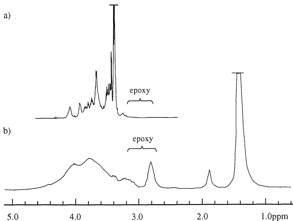
Figure 2.2. ^1\text{H} NMR spectra of the polymers obtained from (a) 1,2:5,6-dianhydro-3,4-di- O -methyl-D-mannitol ( 1 ) and (b) 1,2:5,6-dianhydro-3,4- O -isopropylidene-D-mannitol ( 3 ) using \text{BF}_3 \cdot \text{OEt}_2 .
