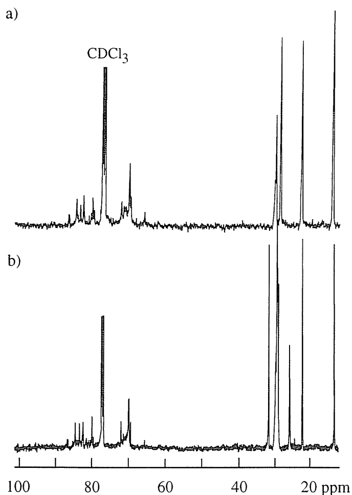
Figure 2.5. ^{13}\text{C} NMR spectra of the polymers prepared from (a) 1,2:5,6-dianhydro-3,4-di- O -pentyl-D-mannitol ( 4 ) and (b) 1,2:5,6-dianhydro-3,4-di- O -decyl-D-mannitol ( 5 ) using \text{BF}_3 \cdot \text{OEt}_2 .
