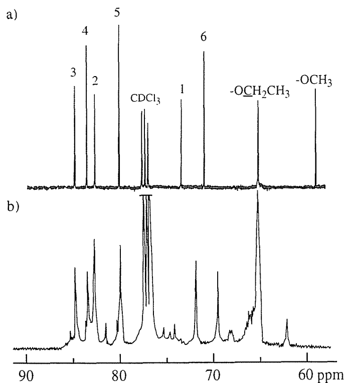
Figure 2.4. ^{13}\text{C} NMR spectra of (a) 2,5-anhydro-3,4-di- O -ethyl-1,6-di- O -methyl-D-glucitol ( 15 ) and (b) the polymer obtained from 1,2:5,6-dianhydro-3,4-di- O -ethyl-D-mannitol ( 2 ) using \text{BF}_3 \cdot \text{OEt}_2 .
