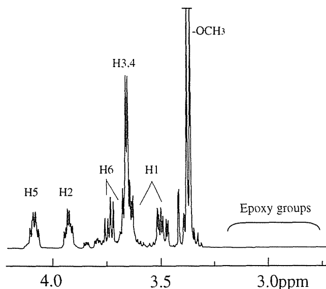
Figure 3.1. 1 H NMR spectrum of the polymer prepared from 1,2:5,6-dianhydro-3,4-di- O -methyl-D-mannitol ( 1 ) using t -BuOK in toluene.
