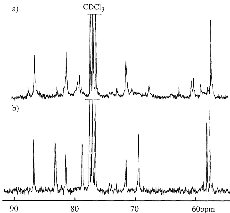
Figure 6.3. ^{13}\text{C} NMR spectra of the polymers prepared from 1,2:5,6-dianhydro-3,4-di- O -methyl-D-glucitol ( 47 ) using (a) \text{BF}_3 \cdot \text{OEt}_2 in dichloromethane and (b) t -BuOK in toluene.
