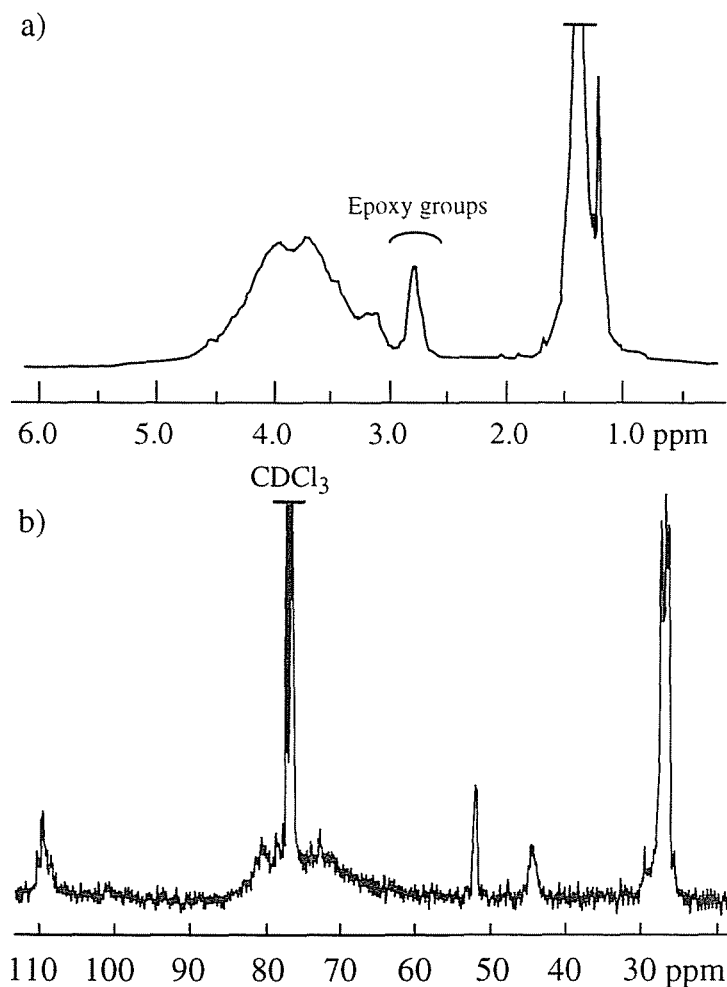
Figure 3.3. ^1\text{H} (a) and ^{13}\text{C} (b) NMR spectra of the polymer prepared from 1,2:5,6-dianhydro-3,4- O -isopropylidene-D-mannitol ( 3 ) using t -BuOK in THF: [ 3 ]/[ t -BuOK] = 20; time, 3 hours; M_n = 8210 ; M_w/M_n = 2.62 .
