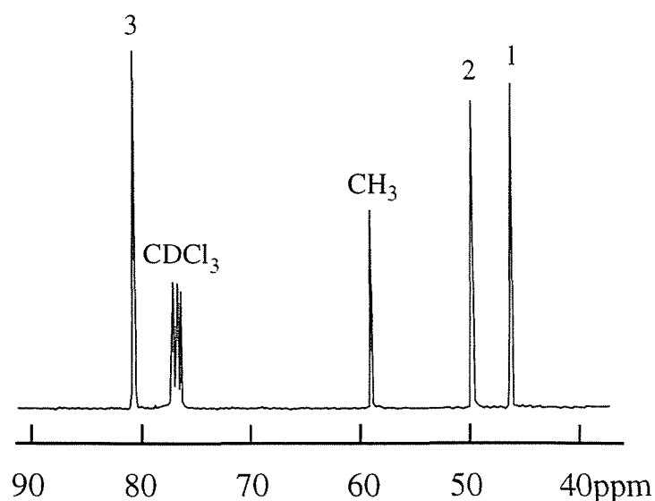
Figure 2.1. ^{13}\text{C} NMR spectrum of 1,2:5,6-Dianhydro-3,4-di- O -methyl-D-mannitol ( 1 ).
