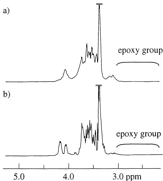
Figure 6.2. ^1\text{H} NMR spectra of polymers prepared from 1,2:5,6-dianhydro-3,4-di- O -methyl-D-glucitol ( 47 ) using (a) \text{BF}_3\cdot\text{OEt}_2 in dichloromethane and (b) t -BuOK in toluene.
