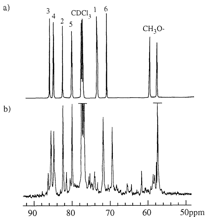
Figure 2.3. ^{13}\text{C} NMR spectra of (a) 2,5-anhydro-1,3,4,6-tetra- O -methyl-D-glucitol ( 14 ) and (b) the polymer prepared from 1,2:5,6-dianhydro-3,4-di- O -methyl-D-mannitol ( 1 ) using \text{BF}_3 \cdot \text{OEt}_2 .
