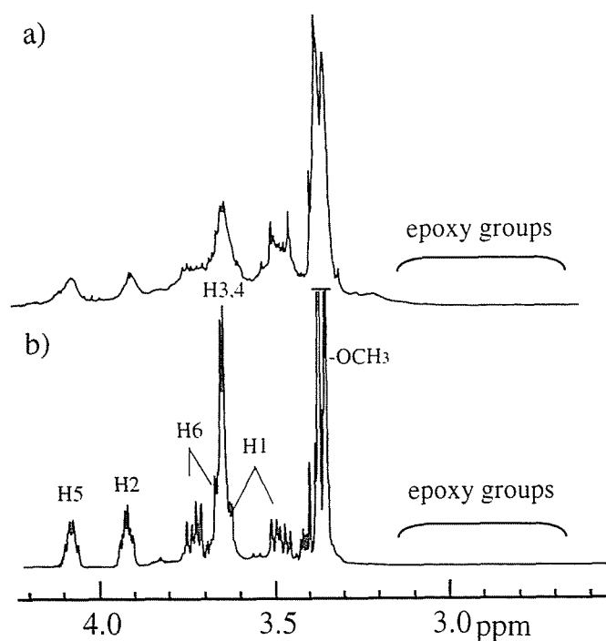
Figure 5.2. ^1\text{H} NMR spectra of the polymers obtained from 40 using (a) \text{BF}_3\cdot\text{OEt}_2 and (b) t\text{-BuOK} .
