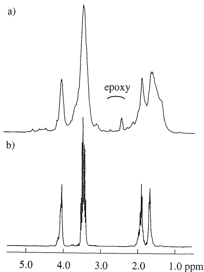
Figure 4.2. ^1\text{H} NMR spectra of the polymers prepared from (2 S ,5 S )-1,2:5,6-diepoxyhexane ((2 S ,5 S )- 31 ) using (a) \text{BF}_3 \cdot \text{OEt}_2 in \text{CH}_2\text{Cl}_2 and (b) t\text{-BuOK} in toluene.
