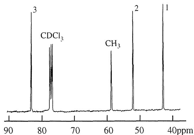
Figure 5.1. ^{13}\text{C} NMR spectrum of 1,2:5,6-Dianhydro-3,4-di- O -methyl-L-iditol ( 40 ).
