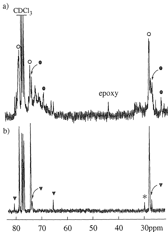
Figure 4.3. ^{13}\text{C} NMR spectra of the polymers prepared from (2 S ,5 S )-1,2:5,6-diepoxyhexane ((2 S ,5 S )- 31 ) using (a) \text{BF}_3\cdot\text{OEt}_2 in \text{CH}_2\text{Cl}_2 and (b) t\text{-BuOK} in toluene.
