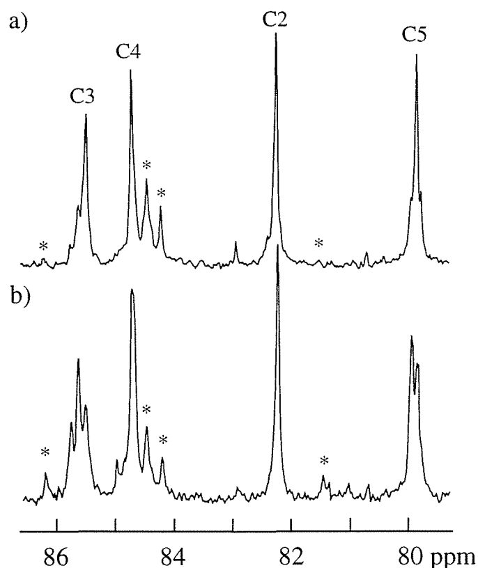
Figure 5.4. ^{13}\text{C} NMR spectra of the copolymers prepared from 1,2:5,6-dianhydro-3,4-di- O -methyl-D-mannitol ( 1 ) ( M_1 ) and 1,2:5,6-dianhydro-3,4-di- O -methyl- L-iditol ( 40 ) ( M_2 ) using t -BuOK in toluene: (a): M_1/M_2 of 0.09 / 0.91 in copolymer, (b): M_1/M_2 of 0.42 / 0.58 in copolymer. The asterisked signals correspond to the carbons of polymer chain-ends.
