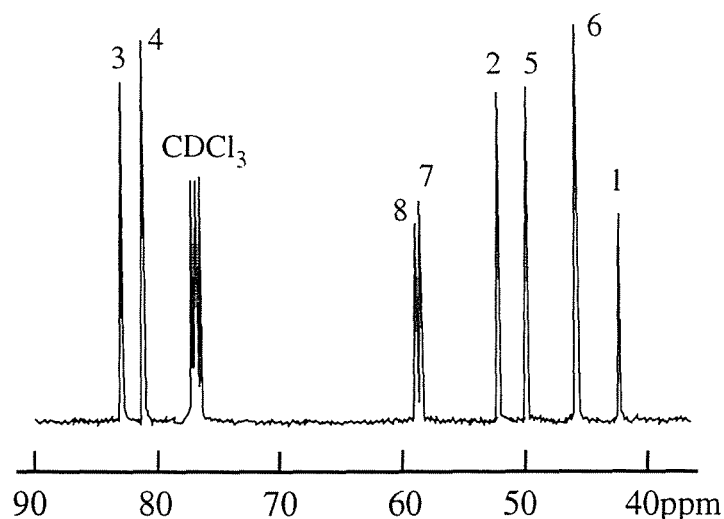
Figure 6.1. ^{13}\text{C} NMR spectrum of 1,2:5,6-Dianhydro-3,4-di- O -methyl-D-glucitol ( 47 ).
