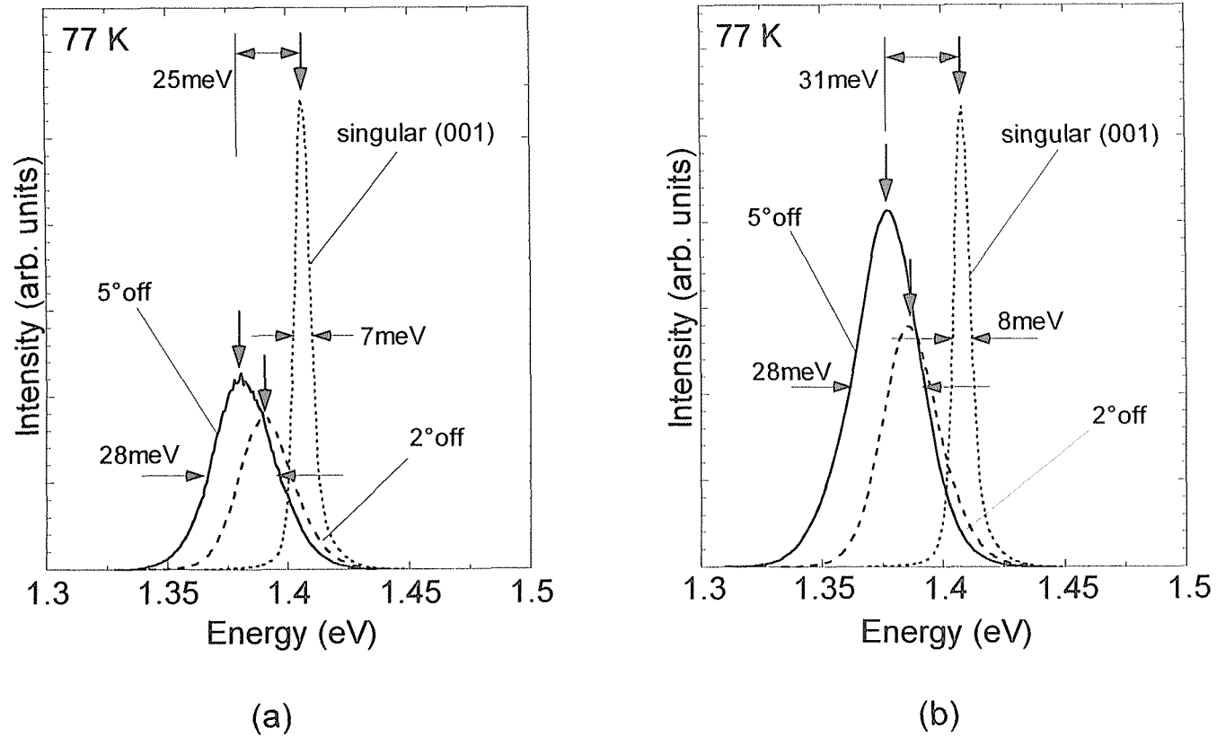
Fig. 5.12 Photoluminescence spectra of InGaAs QWR structures on 5.0°- misoriented substrate (solid line) and 2.0°- misoriented substrate (dashed line), and QWL on the singular (001) substrate (dotted line). (a) \text{In}_{0.1}\text{Ga}_{0.9}\text{As}/\text{GaAs} and (b) \text{In}_{0.15}\text{Ga}_{0.85}\text{As}/\text{GaAs} samples.
