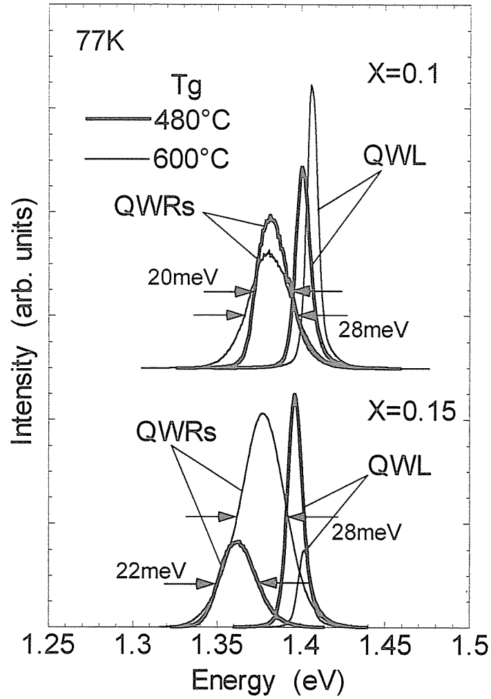
Fig. 5.13 Photoluminescence spectra (thick line) of In 0.1 Ga 0.9 As (upper) and In 0.15 Ga 0.85 As (lower) QWRs on 5.0°-misoriented substrates with 40 nm-thick GaAs upper layers grown at 480 °C, followed by GaAs layers grown at 600 °C, compared to the spectra (thin line) grown at 600 °C. QWL were also grown on singular (001) substrates for a reference.
