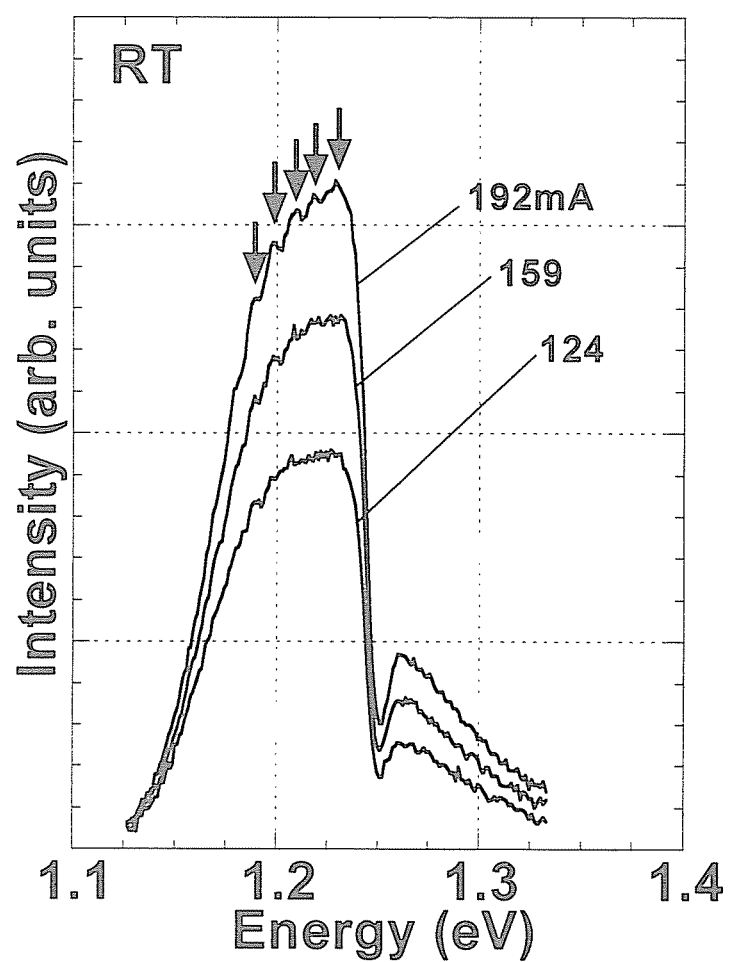
Fig. 6.15 Electroluminescence spectra of QWRs with 0.3 indium content at room temperature. Repetition rate is 12 kHz and duty ratio is 90 %. Cavity direction is parallel to QWRs.
