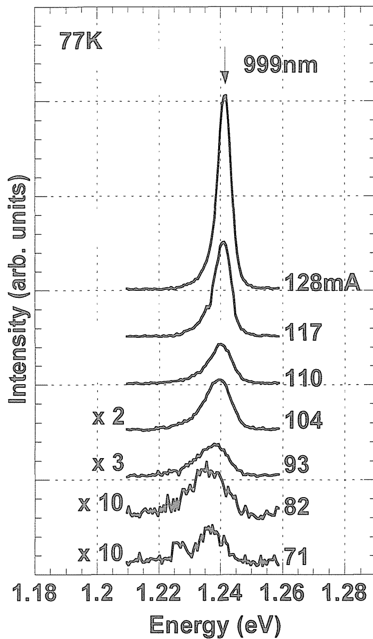
Fig. 6.12 Electroluminescence and lasing spectra of QWRs on 5.0°-misoriented GaAs (001) substrates by pulsed current injections at 77 K. Indium content is 0.3 and cavity direction is parallel to QWRs.
