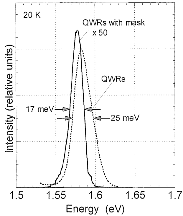
Fig. 4.7 Photoluminescence spectra of QWRs on 5.0°-misoriented substrate at 20K. Solid line is PL spectrum through the 2 \mu m-width and 800 \mu m-long line patterned mask, which corresponds to the luminescence of about thirty QWRs, and dotted line is that without the mask.
