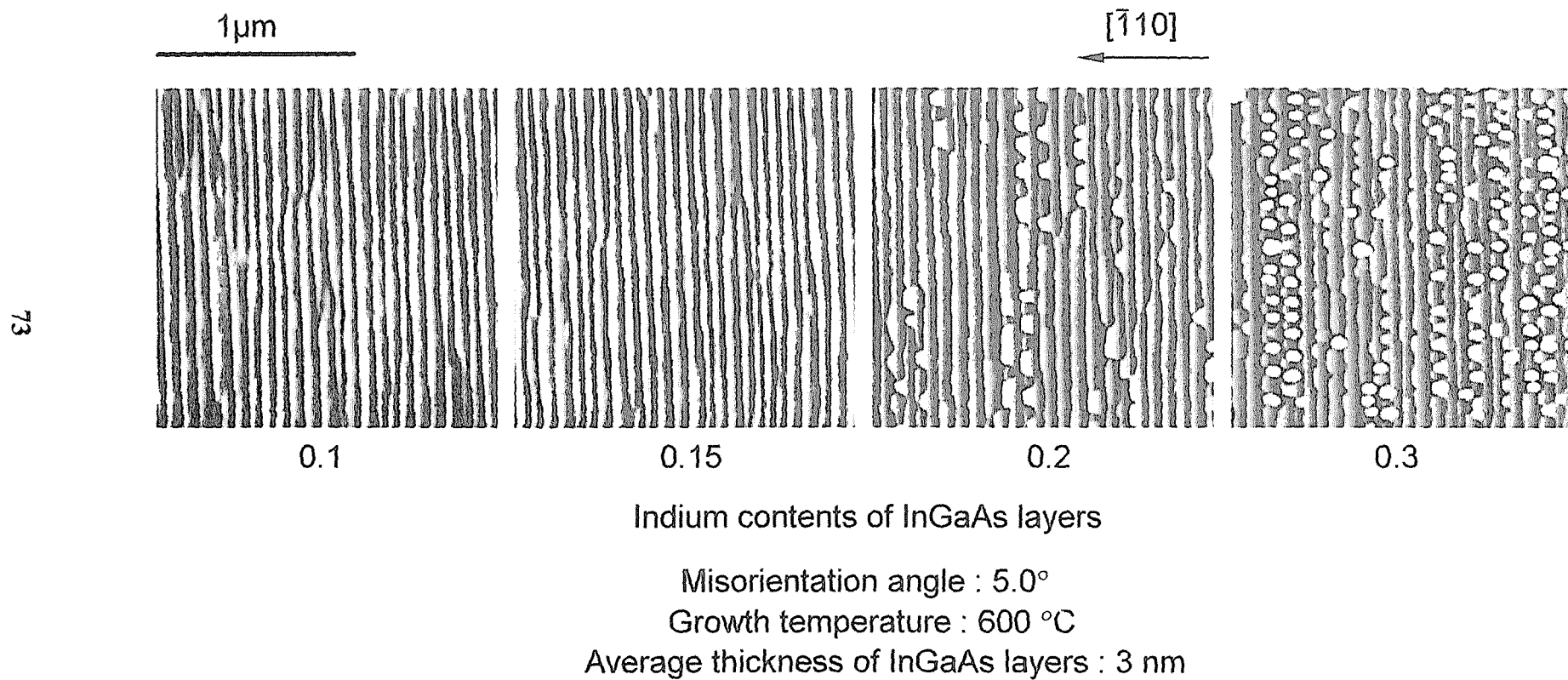
Fig. 5.3 Indium content dependence of InGaAs surface morphologies grown on vicinal GaAs (001) substrates.
