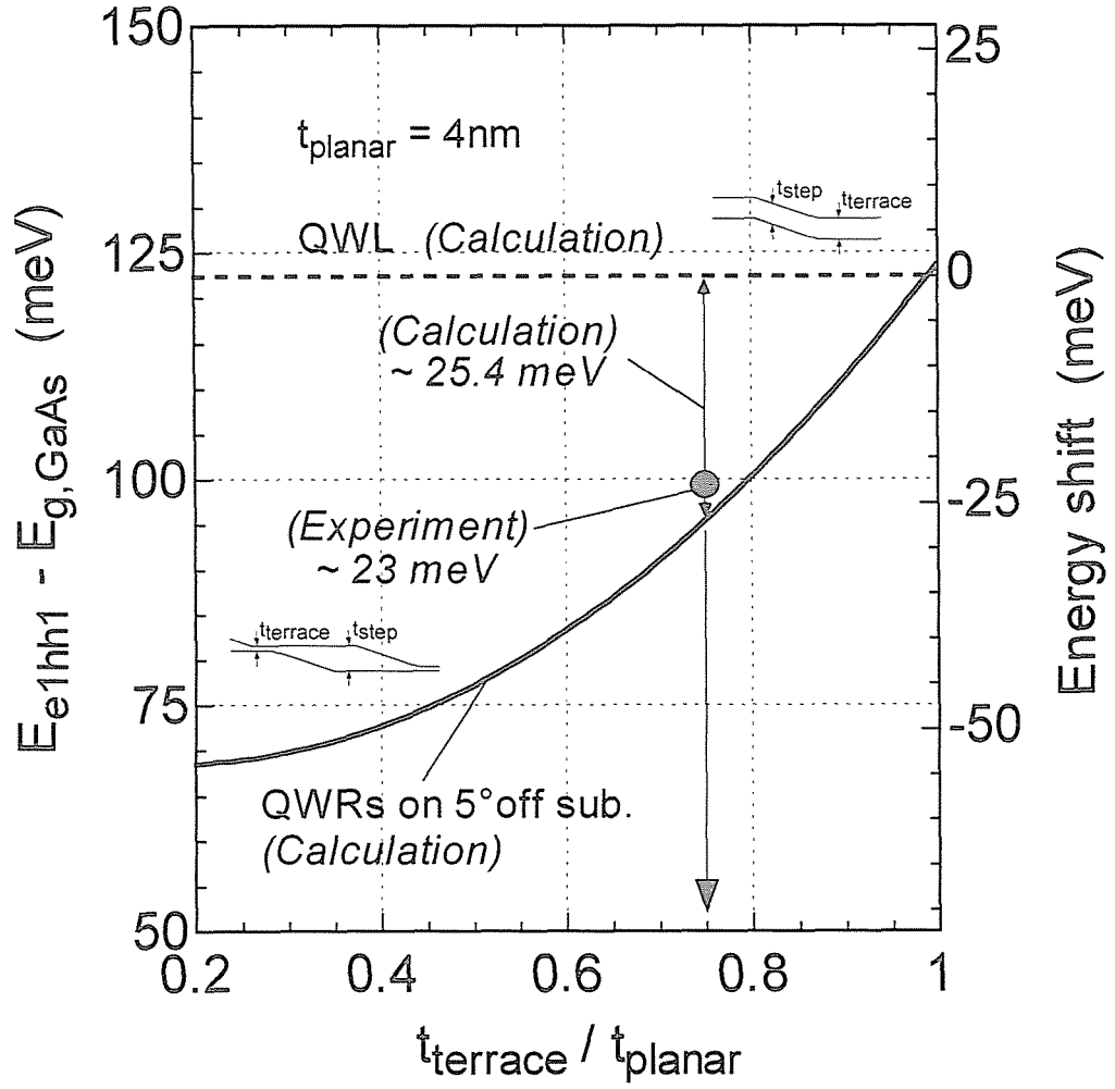
Fig. 3.6 Photoluminescence peak energy as a function of thickness variation of GaAs layer, t_{\text{terrace}}/t_{\text{planar}} : (solid line) QWR structures on 5.0°- misoriented substrate; (dashed line) QWL on the singular (001) substrate. Well thickness on the singular (001) substrate( t_{\text{planar}} ) is fixed at 4 nm in this calculation.
