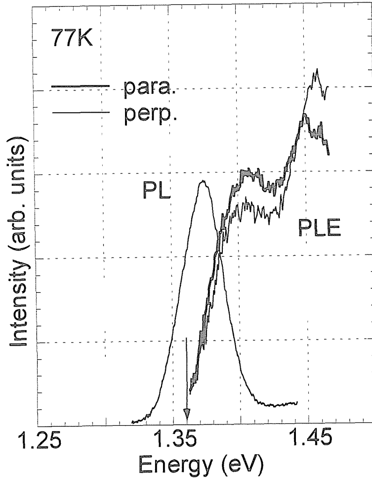
Fig. 5.15 PL and PLE spectra of In 0.15 Ga 0.85 As QWRs on 5.0°- misoriented substrates at 77 K. An arrow shows detection energy (1.359 eV) in PLE measurements.
