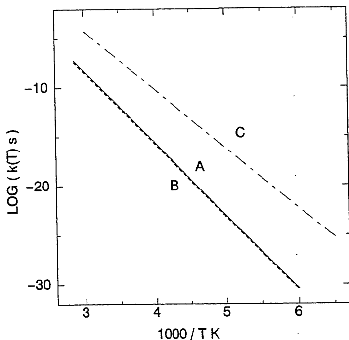
Figure VII-9. Arrhenius plots of the \text{CH}_3\text{O}\cdot/\text{CH}_2\text{OH} isomerization reaction. (A) reaction rate constant in the methanol cluster, (B) in vacuo, (C) in a water cluster.
