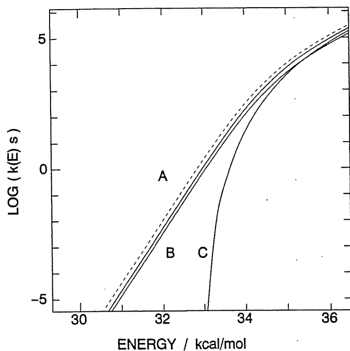
Figure VII-8. Microcanonical rate constants of the \text{CH}_3\text{O}\cdot/\text{CH}_2\text{OH} isomerization reaction as a function of the total energy. (A) Rate constant in the methanol cluster calculated based on the VC model, (B) rate constant in vacuo, (C) Classical rate constant (i.e., the rate does not take into account the tunnel effect) in the model cluster calculated based on the VC effect. Dashed line indicates the reaction rate calculated based on the VC model plus the continuum model.
