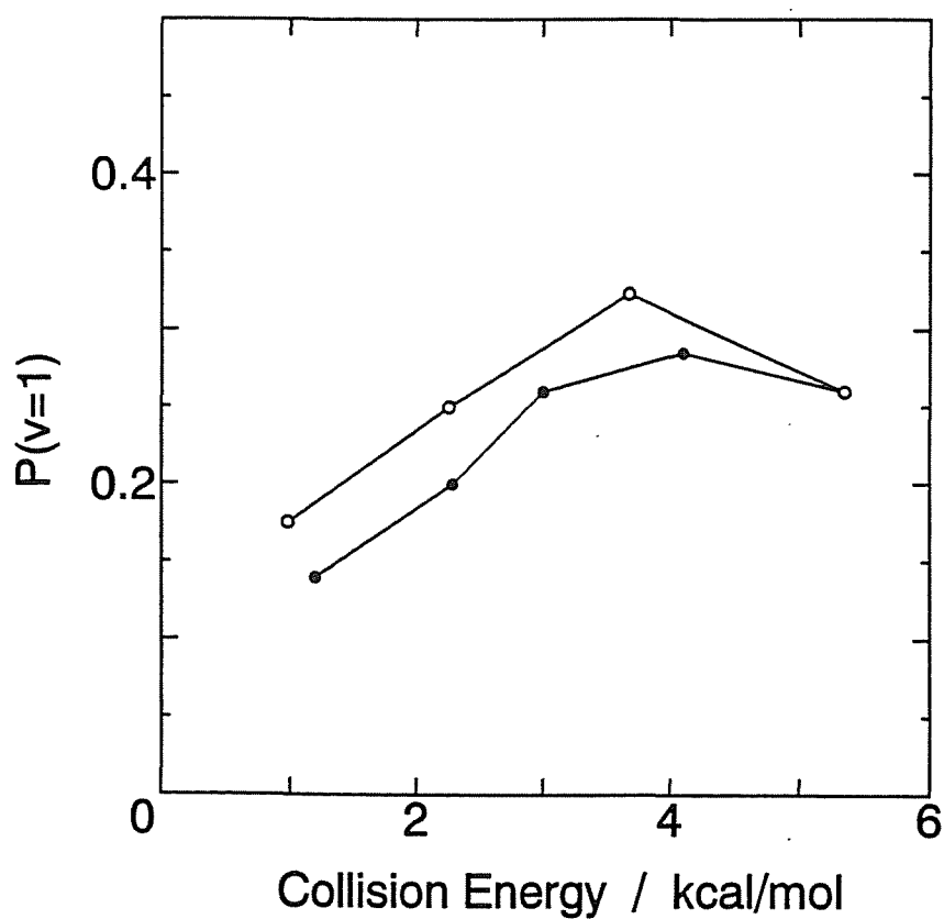
Figure IV-6. The theoretical fraction of total OH population in v=1 , P(v=1) , vs. center-of-mass collision energy of the reagents (●). The experimental data (O) are cited from Ref. 7.
