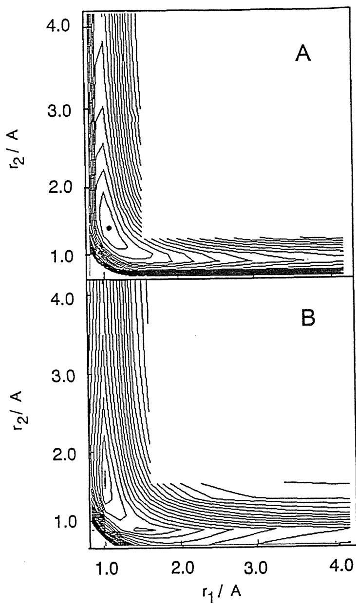
Figure IV-2. Potential energy surfaces of the \text{O}^- + \text{HF} \rightarrow \text{OH} + \text{F}^- reaction calculated at the HF/6-31++G** level. (A) Collinear collision ( \theta = 180^\circ ), (B) Coplanar collision ( \theta = 135^\circ ). Contours are drawn for each 5 kcal/mol.
