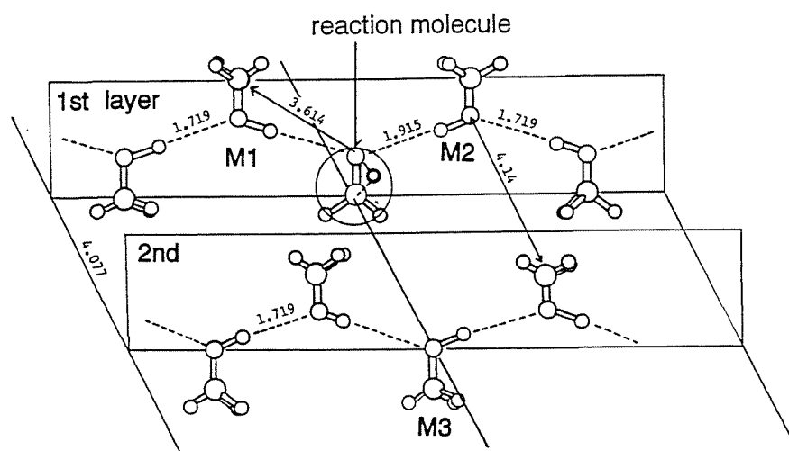
Figure VII-6. Geometry of the methanol molecules around the reaction molecule. Eight methanol molecules on the first and second layers are sketched. The M 1 , M 2 and M 3 mean the methanol molecules considered in the vibrational coupling with the reactant molecule. The position of oxygen atom of the reaction molecule is fixed during the reaction.
