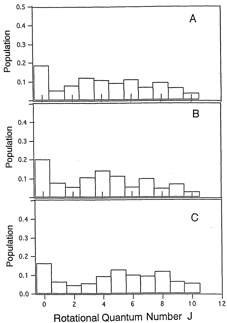
Figure IV-4. Rotational state populations of the OH radical formed by the \text{O}^- + \text{HF} \rightarrow \text{OH} + \text{F}^- reaction. The collision energies are (A) 1.198 kcal/mol, (B) 3.00 kcal/mol, and (C) 5.31 kcal/mol.
