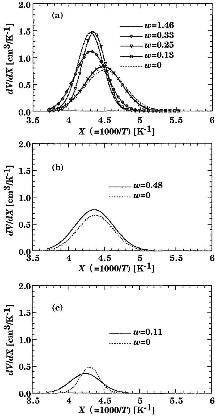
Figure 4.6. Freezing point distribution of freezable pore water for YL (a), BZ (b), and IL (c) coals.
