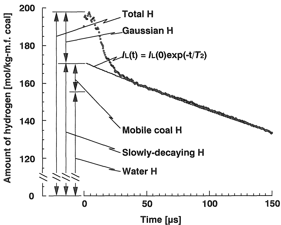
Figure 5.6. ^1\text{H} NMR transverse relaxation signal of as-received YL at 298 K. The solid line represents the fit of the data points for the slowly decaying components using an exponential function.
