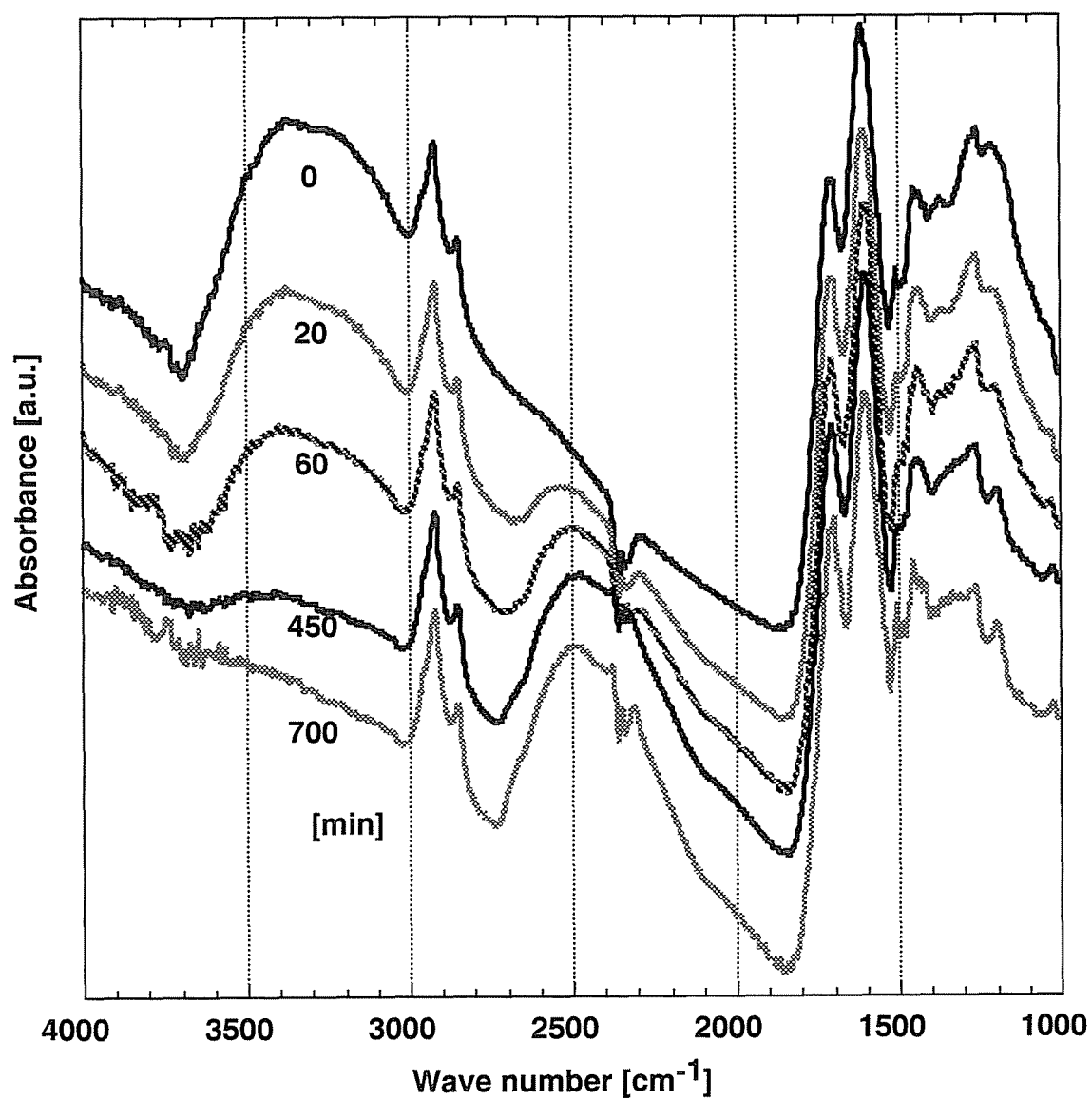
Figure 5.8. Changes in the IR spectra of deuterated YL with time period of exposure to D 2 O vapor.
