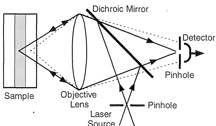
図2-3. 顕微共焦点蛍光分光法の光学系 (from Masuhara and Sasaki, 1995)
