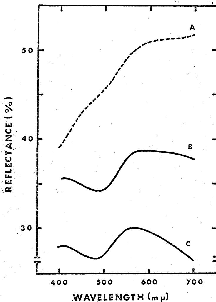
Fig. V-1. Reflectance spectra of the normal meat(A), slightly coloured blue meat(B) and strongly coloured blue meat(C) in canned king crab.
