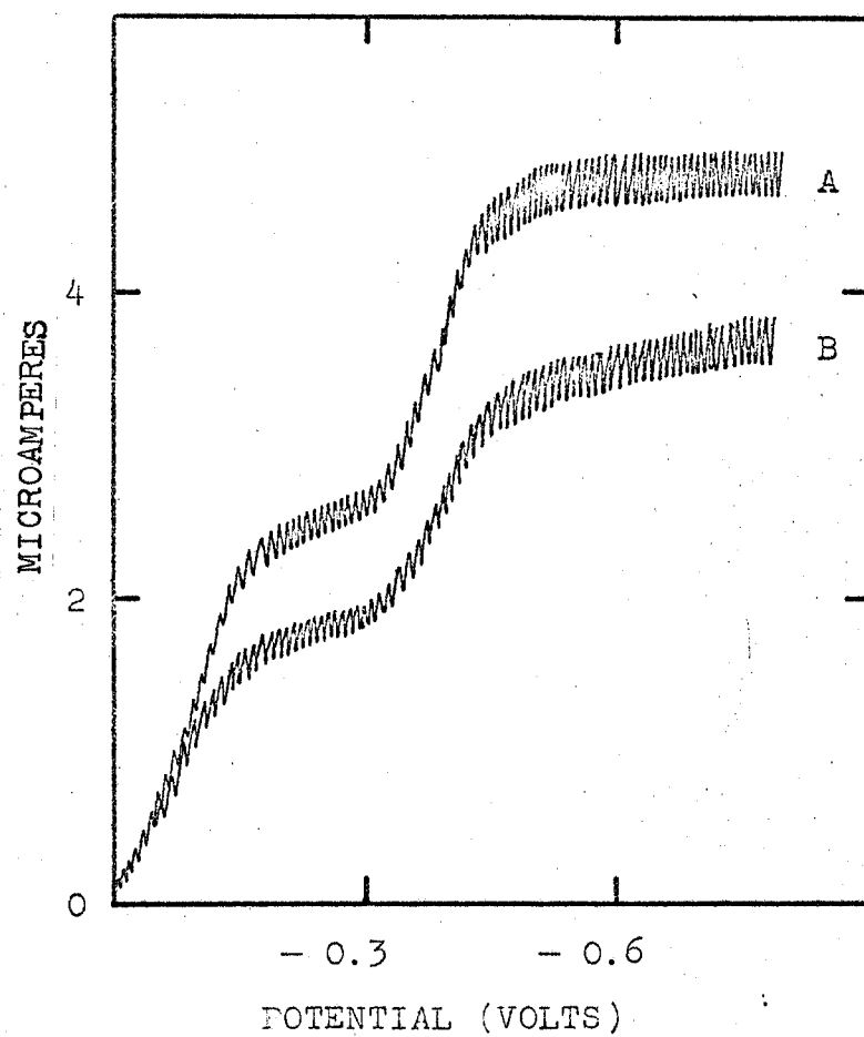
Fig. IV-3. Polarograms of Cu(II)(A) and metal ion of haemocyanin(B) in aqueous solution.
