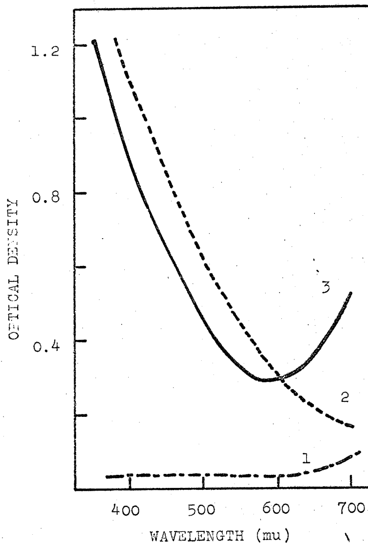
Fig. IV-4. Absorption spectra of Cu(II) solution, Cu(II) treated with hydrogen sulphide and its heat treated solution.
