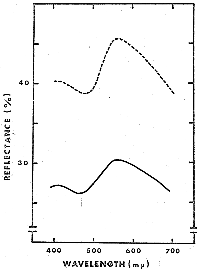
Fig. V-4. Reflectance spectra of blue meat and haemocyanin-sulphide complex with red pigment of epidermis. Dashed line ---- haemocyanin-sulphide complex with red pigment in epidermis; full line — blue meat.
