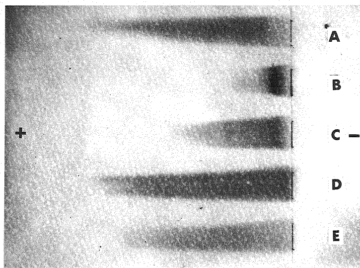
Fig. VI-2. Paper electrophoresis of fractions extracted by 1N sodium hydroxide from the blue meat Veronal buffer(pH 8.6, \mu = 0.05), Current at 5 mA for 4 hours, Stained with Amido black 10B
