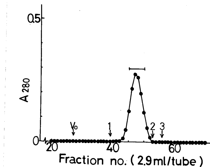
Fig. 38. Elution diagram of a partially purified preparation of chum salmon FS. The fraction containing FS isolated from hydroxylapatite column was applied to a column of Sepharose 6B (2.2×59) equilibrated with 0.02 M Tris-HCl buffer, pH 8.0 containing 2% NaCl. The fractions marked with a bar which was eluted at a position of molecular weight of approximately 600,000 were collected for further analysis. Marker proteins: 1. human IgM, 2. horse spleen apoferritin, 3. human albumin, V 0 : void volume, A 280 : absorbance at 280 nm.
