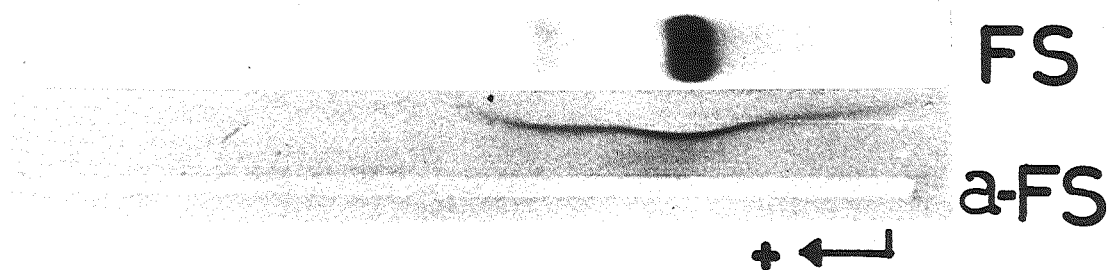
Fig. 42. Disc immunoelectrophoresis of purified chum salmon FS. The sample was subjected first to disc electrophoresis in 5% polyacrylamide gel which was subsequently implanted in 1.2% agarose gel, putting anti-salmon FSSP into the trough. The protein (FS) in polyacrylamide gel diffused into agarose gel and formed precipitin line. FS: purified FS, a-FS: anti-salmon FSSP.
