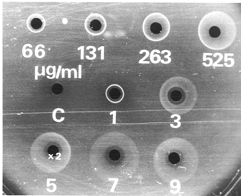
Fig. 23. Typical immunodiffusion plate (unstained). The agarose contained anti-trout FSSP. The antigen wells were filled with varying amounts of purified FS from rainbow trout used as standard and serum samples (C,1,3,5 and 7).
