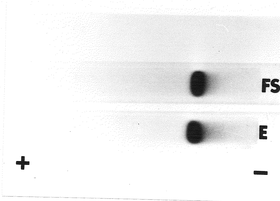
Fig. 51. Disc electrophoresis in 5% polyacrylamide gel of purified FS and its related egg yolk protein of Japanese eel. FS, E: same as in Fig. 50.
