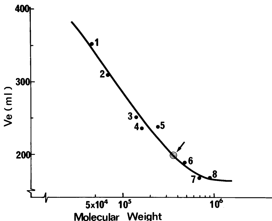
Fig. 53. Estimation of molecular weight by Sephadex G-200 gel filtration. Both FS and its related egg yolk protein of Japanese eel are eluted at the position of open circle (arrow). The samples used for calibration are indicated by dark circles. 1: ovalbumin, 2: bovine serum albumin, 3: alcohol dehydrogenase, 4: human IgG, 5: bovine liver catalase, 6: apoferritin, 7: bovine thyroglobulin, 8: human IgM, Ve: elution volume.
