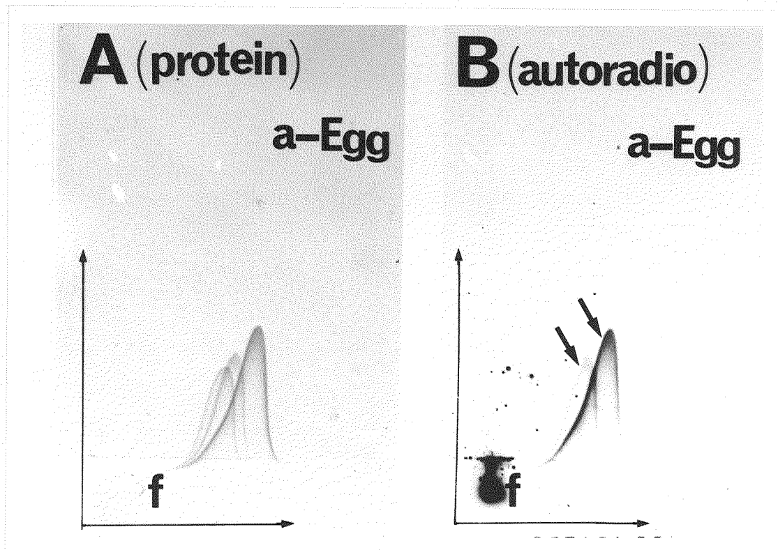
Fig. 57. Crossed immunoelectrophoresis (A) and its autoradiography (B). Antigen: female serum of medaka in breeding season mixed with ^{59}\text{FeCl}_3 . Antibody: anti-medaka eggs. After staining and dried, the plate was exposed to X-ray films.
