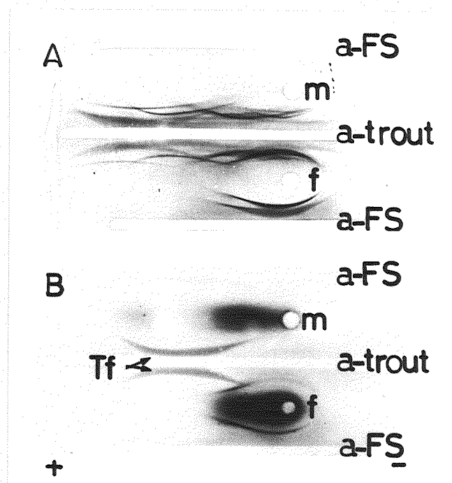
Fig. 4. Immunoelectrophoresis of ripe rainbow trout sera. A: protein staining, B: autoradiography with ^{59}\text{Fe} , a-trout: anti-trout serum, a-FS: a-trout FSSP, m,f,: male or female serum.
