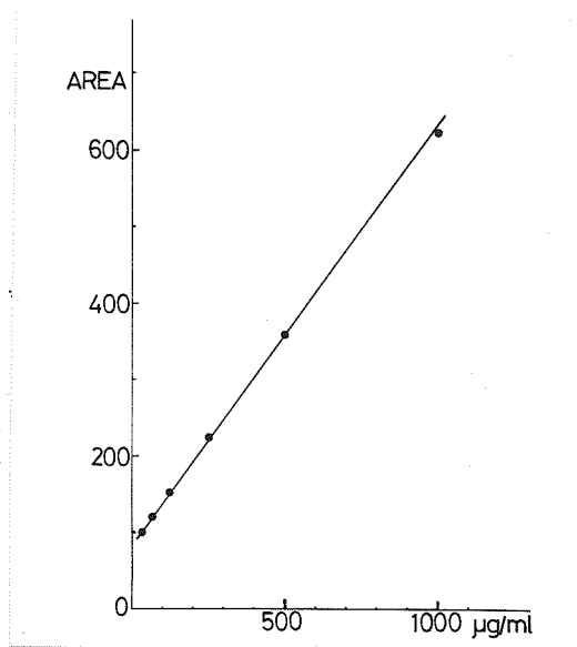
Fig. 24. The standard curve determined by a typical single radial immunodiffusion (see Fig. 23). Horizontal line indicates the concentration of trout FS.
