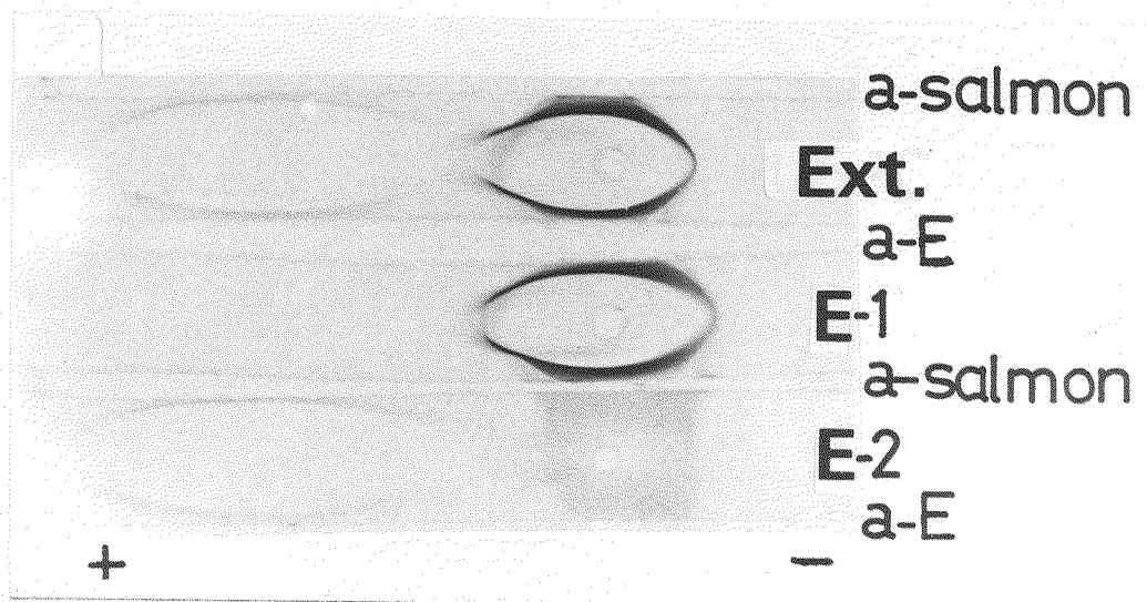
Fig. 44. Immunoelectrophoresis of 0.9% NaCl extracts (Ext.), E1 (E-1) and E2 (E-2) of chum salmon egg. The antisera used were anti-salmon serum (a-salmon) and anti-salmon eggs (a-E).
