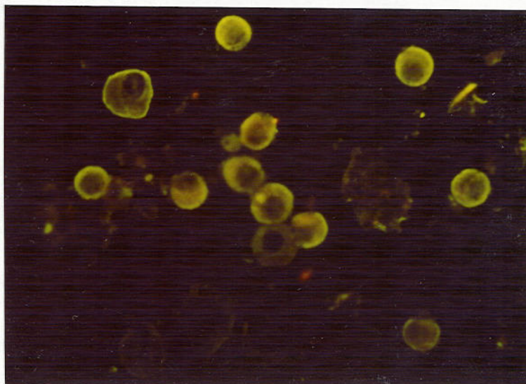
Fig. 32. Localization of female-specific serum protein(s) in fixed rainbow trout liver cells as revealed by immunofluorescence. The cytoplasm is homogeneously stained.
