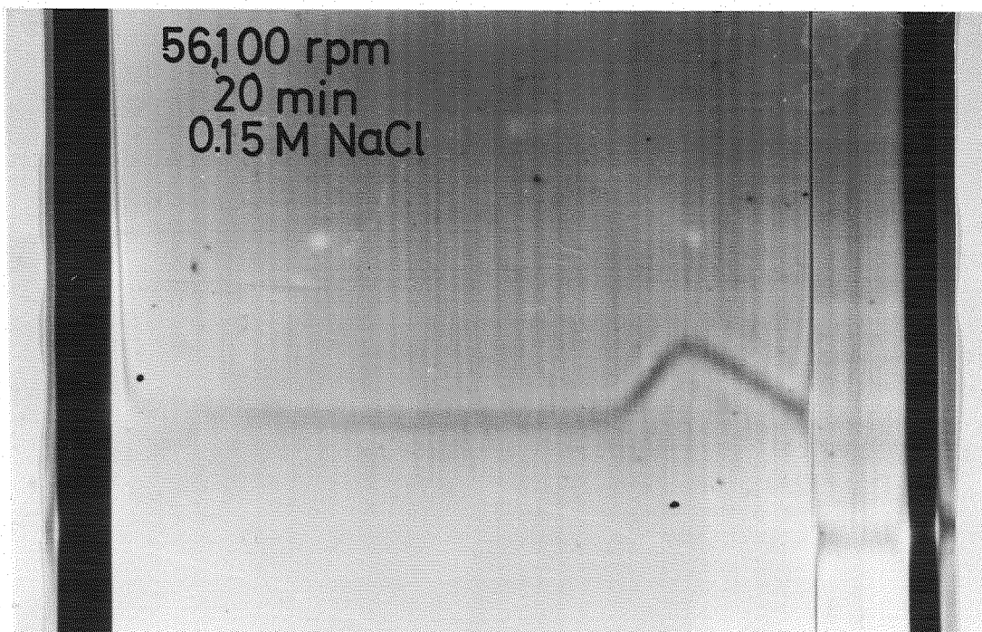
Fig. 21. Ultracentrifugal pattern of purified trout E2 from egg yolk proteins.
