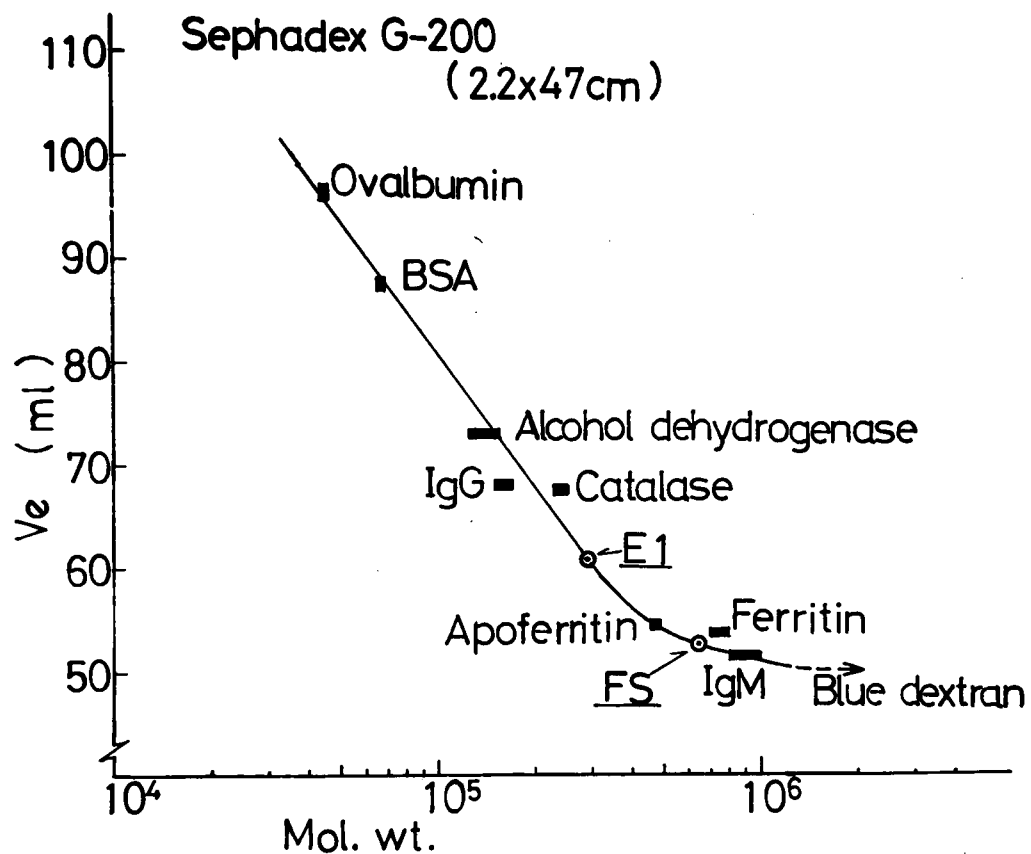
Fig. 9. Estimation of molecular weight from the exclusion volume on Sephadex G-200. Calibration curve of Sephadex G-200 (2.2x47cm). The samples used for calibration are indicated by dark bars. The open circles correspond to the elution volume of trout female-specific iron-binding serum protein (FS) and egg protein (E1) passed through the Sephadex G-200 column.
