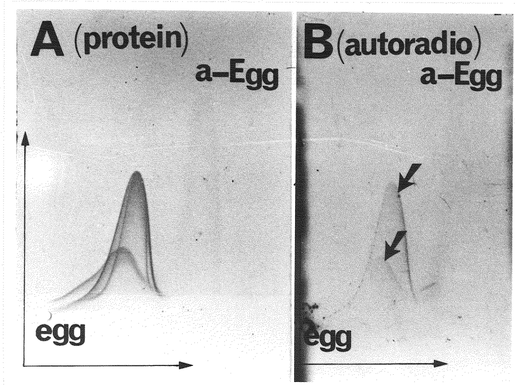
Fig. 55. Crossed immunoelectrophoresis (A) and its autoradiography (B). Antigen: egg yolk proteins of medaka mixed with ^{59}\text{FeCl}_3 . Antibody: anti-medaka eggs. The arrows show the radioactive precipitin lines.
