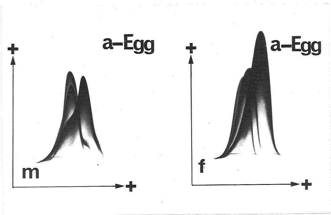
Fig. 69. Crossed immunoelectrophoresis of sera from male and female medaka after administration of ethinylestradiol. Samples were collected at 10 days after hormone treatment.
