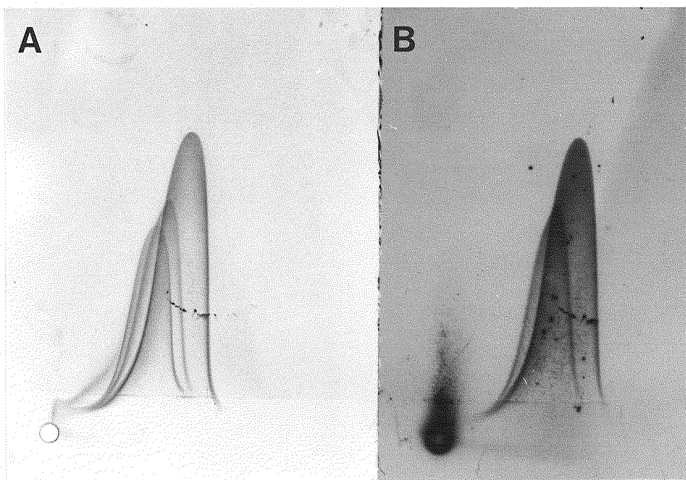
Fig. 70. Crossed immunoelectrophoresis (A) and its autoradiography (B). Antigen: male medaka serum after administration of estradiol-17 \beta mixed with ^{59}\text{FeCl}_3 .
