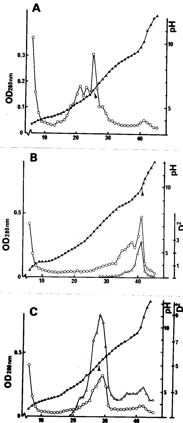
Fig. 22. Patterns of isoelectrofocussing of purified proteins of FS(A), E1(B) and E2(C) isolated from rainbow trout. Ampholite: pH 3-10, voltage 700 V for 72 hr. Sample: 1.0 ml. The pH (▲) was measured with pH meter at 0°C and each protein was determined with a single radial immunodiffusion (Δ) and/or absorbance at 280 nm (O). Single radial immunodiffusion in agarose gel was performed using anti-trout eggs.
