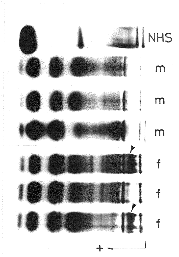
Fig. 33. 7.5% polyacrylamide disc electrophoresis of ripe chum salmon serum. The band indicated by arrow was observed in some females but not in males. NHS: normal human serum, m: male serum, f: female serum.
