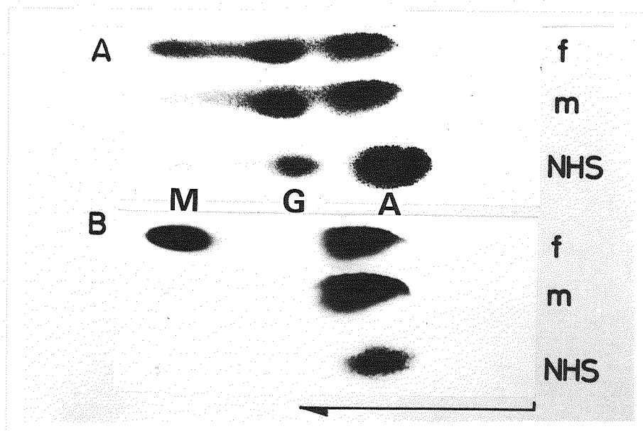
Fig. 35. Thin-layer gel filtration (A) and its autoradiography (B) with ^{59}\text{Fe} on Sephadex G-200, superfine. To 25 \mu\text{l} of the serum was added 10 \mu\text{l} of ^{59}\text{FeCl}_3 solution with an activity of 0.5 \mu\text{Ci} . After being incubated for 1 h, 5 \mu\text{l} of the mixture was subjected to thin-layer chromatography. NHS, m, f: same as in Fig. 33.
