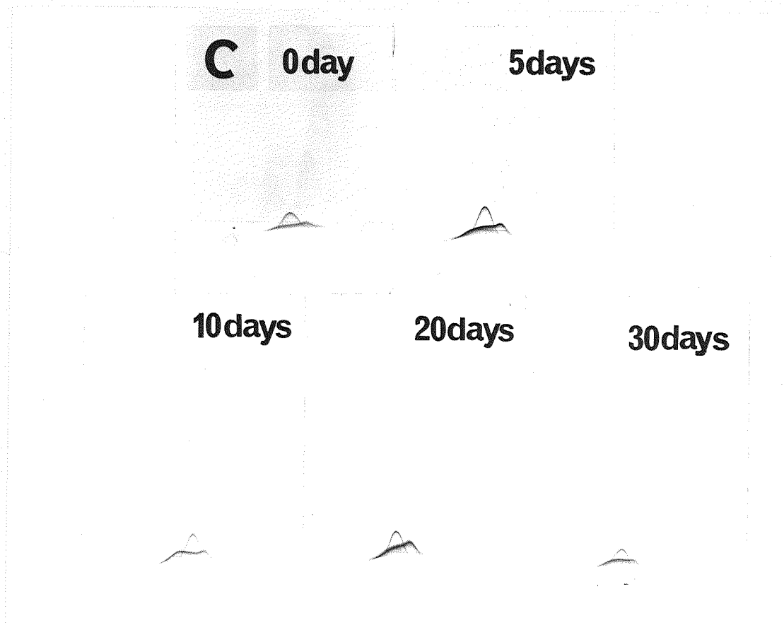
Fig. 64. Crossed immunoelectrophoresis of sera of female medaka of the control group.
