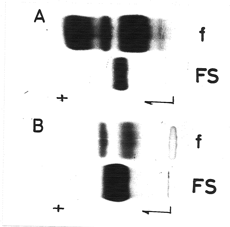
Fig. 40. Electrophoresis of purified FS of chum salmon. A: Cellulose acetate membrane electrophoresis of female salmon serum (f) and the purified FS(FS), B: its autoradiography.
