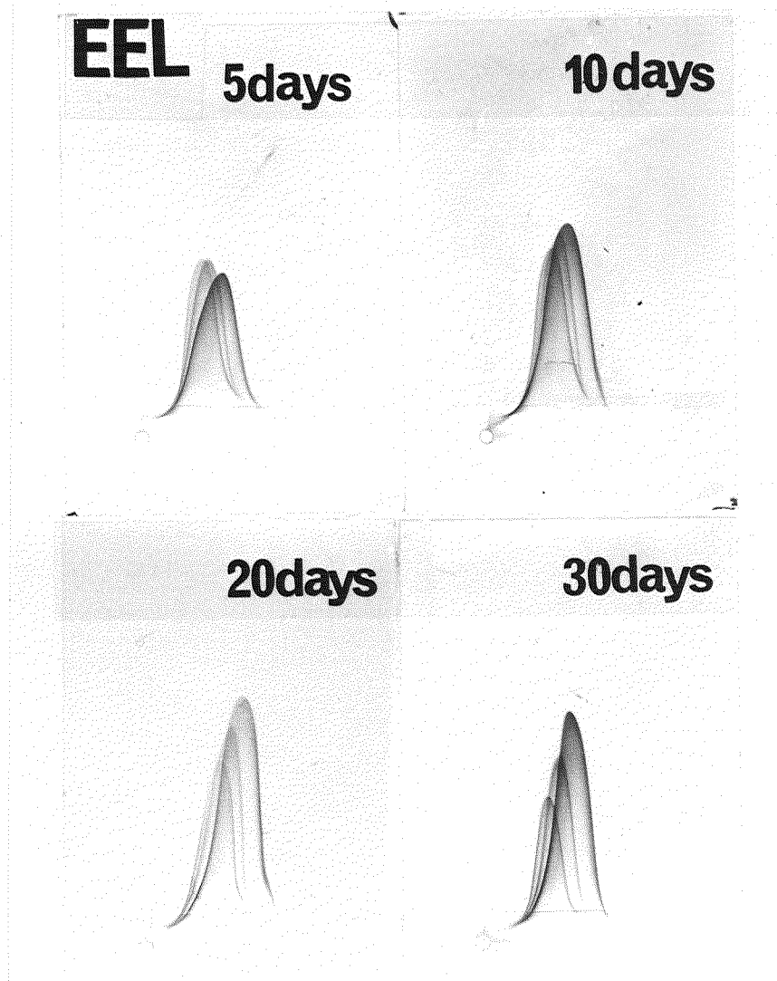
Fig. 67. Crossed immunoelectrophoresis of sera from ethinyl-estradiol-treated medaka.
