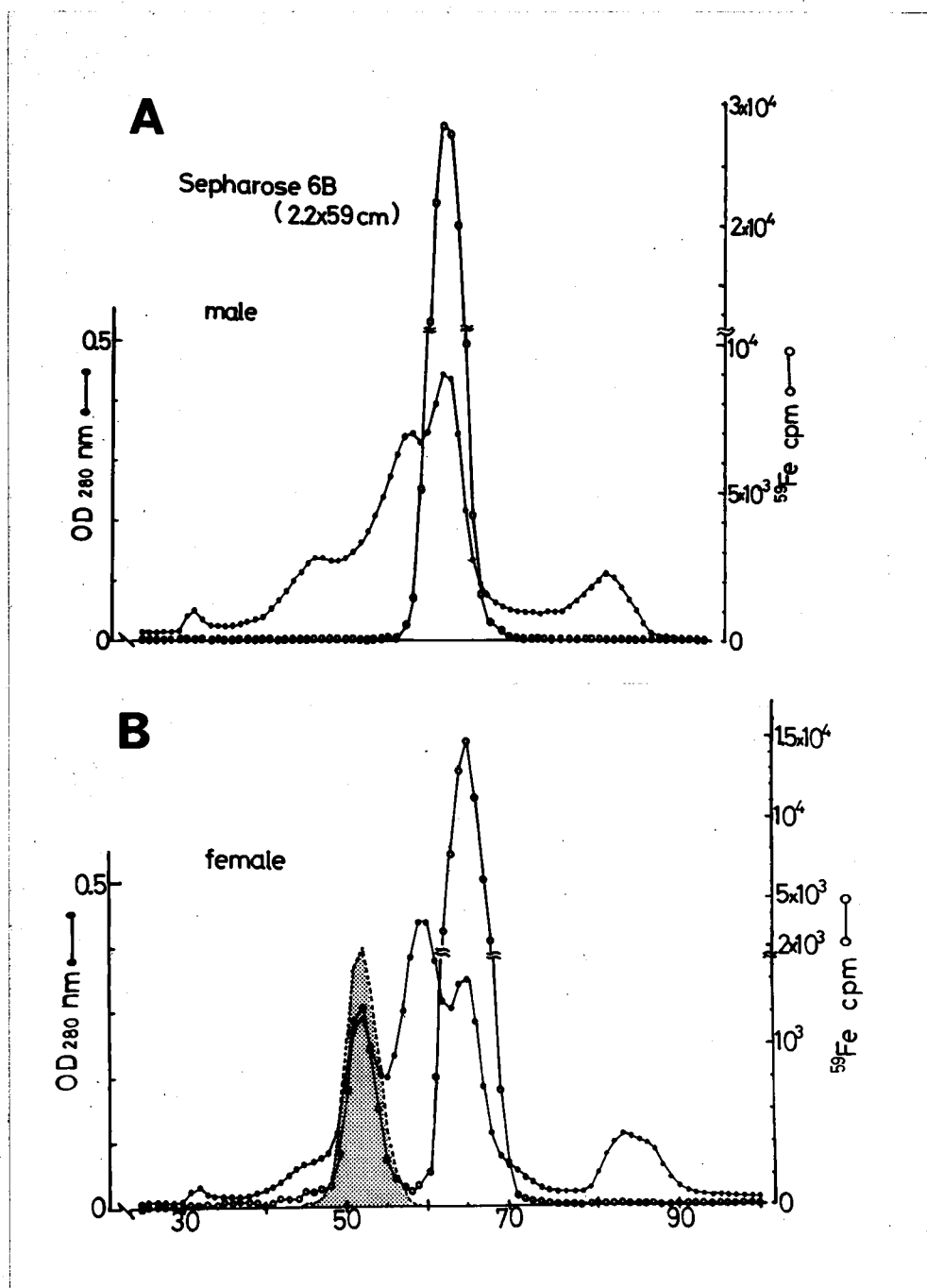
Fig. 5. Gel filtration on Sepharose 6B of sera of ripe male (A) and female (B) rainbow trout. The fractions in shadowed area of female contained female-specific serum protein. One radioactive protein (transferrin) was observed in male, while two radioactive proteins were obtained in female.
