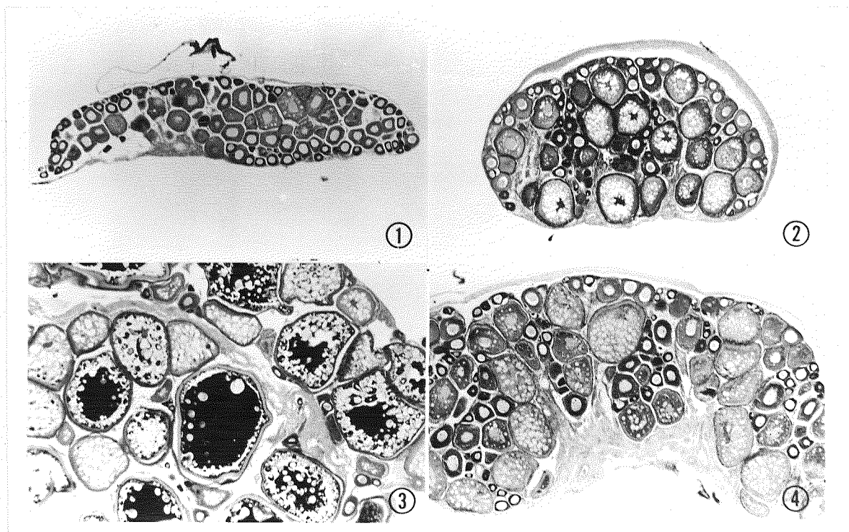
Fig. 60. Histology of the ovary at various stages in medaka. 1,2: "immature", 3: "breeding", 4: "sexually inactive". X 28.
