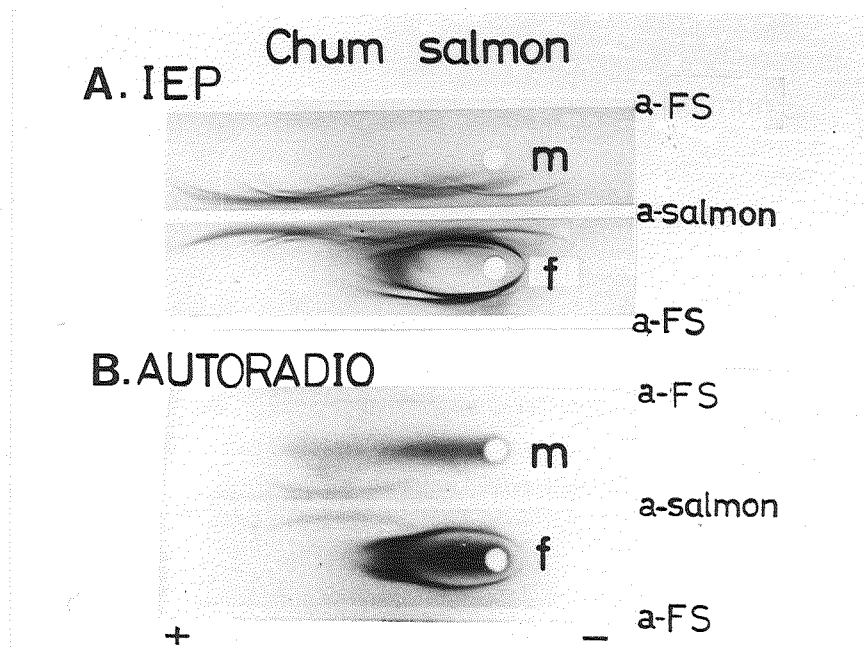
Fig. 36. Immunoelectrophoresis of chum salmon sera. A: protein staining, B: autoradiography with ^{59}\text{Fe} , a-salmon: anti-salmon serum, a-FS: anti-salmon FSSP.
