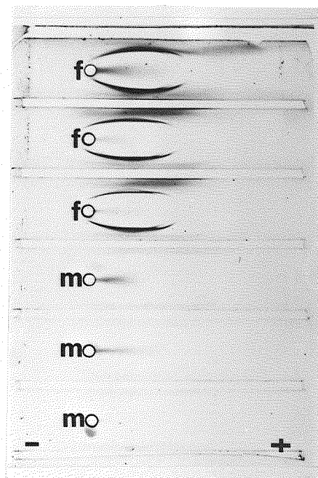
Fig. 56. Immunoelectrophoresis of female and male sera of medaka in breeding season. Each trough was filled with anti-medaka eggs. f: female, m: male
