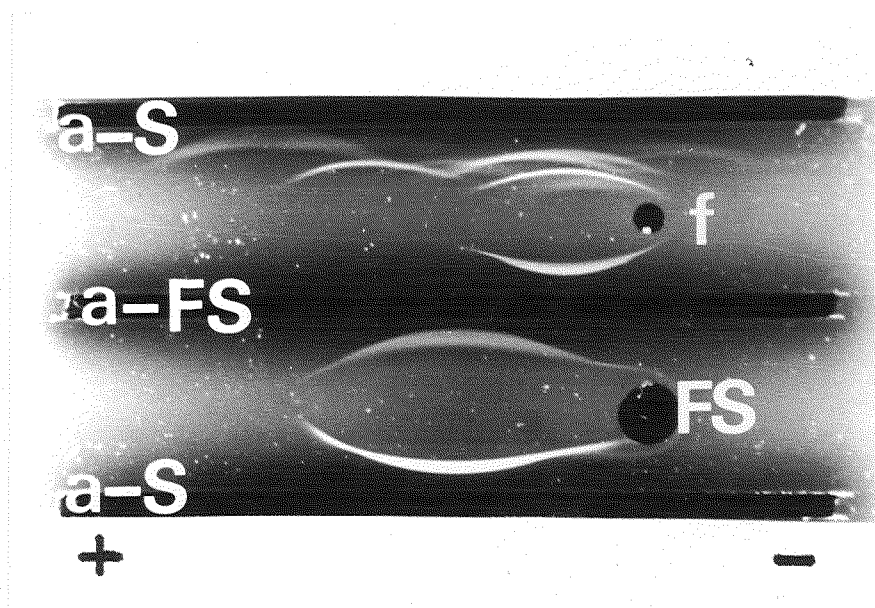
Fig. 41. Immunoelectrophoresis of purified FS of chum salmon. a-S: anti-salmon serum, a-FS: anti-salmon FSSP, f: female serum, FS: purified FS of chum salmon.
