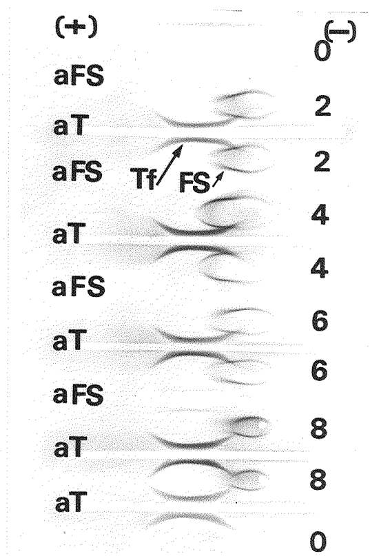
Fig. 27. Autoradiography of immunoelectrophoresis of ^{59}\text{Fe} -binding proteins in estrogen-treated rainbow trout sera. The antigen wells were filled with the serum collected from fish 0 (control), 2, 4, 6 and 8 days after administration of estrogen. Antisera used were anti-trout FSSP (aFS) and anti-trout serum (aT). Tf: transferrin, FS: female-specific iron-binding serum protein.
