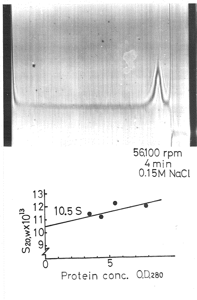
Fig. 19. Ultracentrifugal pattern of purified trout FS and concentration dependency of the sedimentation rate.
