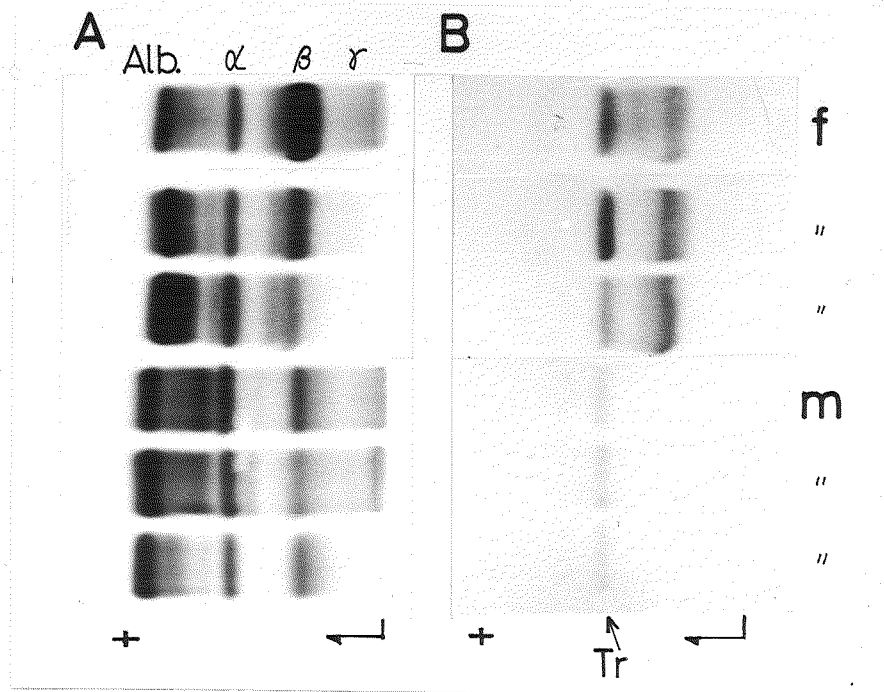
Fig. 34. Electrophoresis of chum salmon sera. A: cellulose acetate electrophoresis (Cellologel), B: autoradiography with ^{59}\text{Fe} ; f: female sera, m: male sera, Tr: transferrin. To 25 \mu\text{l} of the serum was added 10 \mu\text{l} of ^{59}\text{FeCl}_3 solution with an activity of 0.1 \mu\text{Ci} , corresponding to 0.003 \mu\text{g} Fe. After incubation approximately 1 \mu\text{l} of the mixture was subjected to electrophoresis, and the gels were exposed to X-ray films for 2 weeks.
