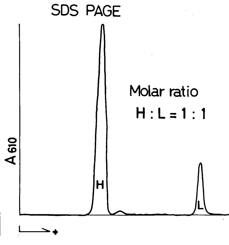
Fig. 18. Spectrophotometric scan of SDS polyacrylamide gel of reduced E1 (R-E1) (Fig. 17). The electrophoretically separated proteins were stained with Coomassie brilliant blue R-250. A molar ratio of 1:1 is obtained for the two subunits (mol. wt. 90,000(H) and 15,000(L)) of E1 of rainbow trout egg yolk.
