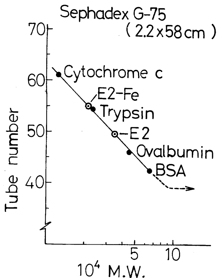
Fig. 10 Estimation of molecular weight from the exclusion volume on Sephadex G-75. Calibration curve of Sephadex G-75 (2.2x58cm). The samples used for calibration are indicated by dark circles. The open circles correspond to the elution volume of trout egg yolk proteins (E2) and radioactive peak of E2 fraction (E2-Fe) (see Fig. 6).
