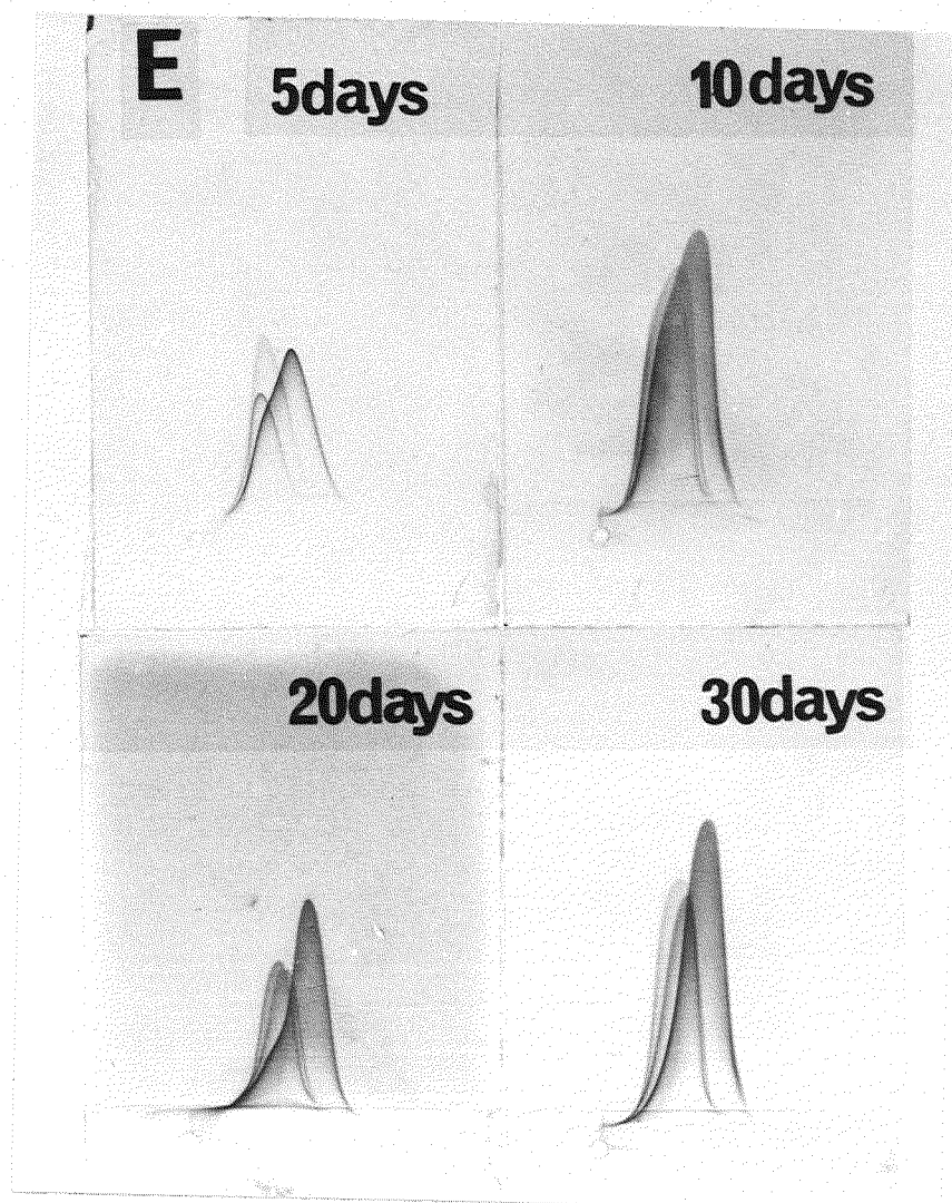
Fig. 68. Crossed immunoelectrophoresis of sera from estradiol-17 \beta -treated medaka.
