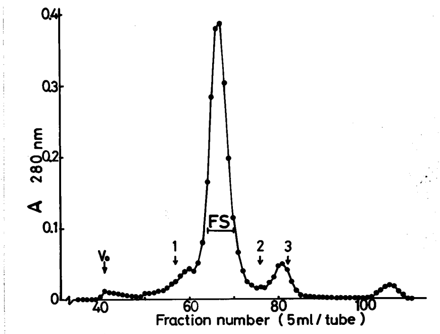
Fig. 7. Chromatography of rainbow trout serum on Sepharose 6B. Material: water-insoluble proteins isolated from pooled ripe female rainbow trout serum. Column: 2.6×90cm, Elution buffer: 0.02 M Tris-HCl, pH 8.0, containing 2% NaCl and 0.1% NaN 3 . FS: fractions eluted in the position indicated by a horizontal bar where collected and designated as FS(see text). Vo: void volume. Marker proteins: (1) IgM, (2) IgG, (3) human serum albumin.
