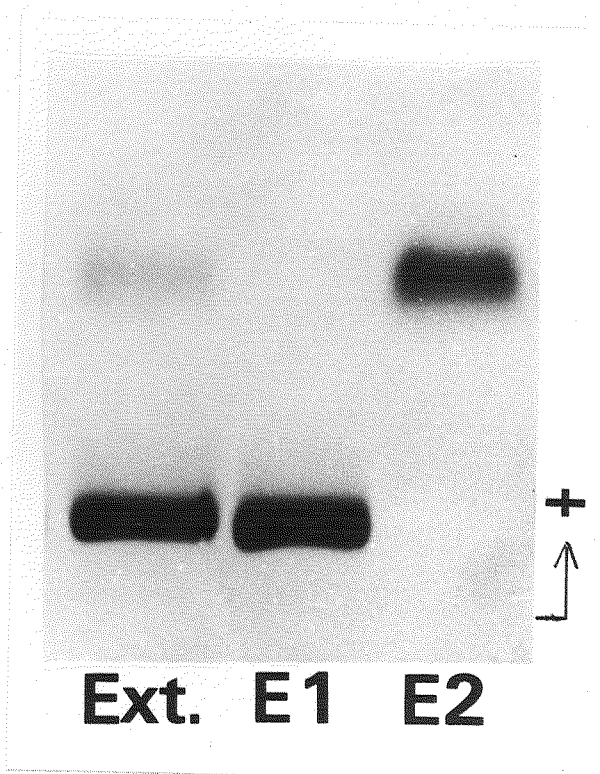
Fig. 43. Cellulose acetate membrane electrophoresis (Cellogel) of egg yolk proteins in chum salmon. Ext.: water insoluble proteins from 0.9% NaCl extraction of chum salmon eggs. E1, E2: two purified egg yolk components isolated by gel filtration.
