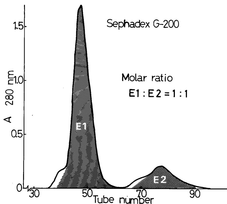
Fig. 11 Elution pattern on Sephadex G-200 of rainbow trout egg yolk proteins (see Fig. 8). Ratios of protein amount between E1 and E2 (shadowed area) were determined planimetrically from charts of gel filtration on Sephadex G-200 monitored by 280 nm absorption. A molar ratio of E1 and E2 can be roughly calculated to be 1 to 1.
