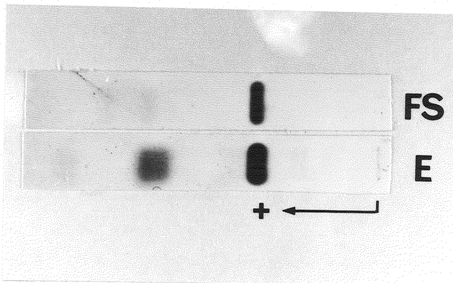
Fig. 52. SDS polyacrylamide gel electrophoresis of purified FS and its related egg yolk protein of Japanese eel. FS, E: same as Fig. 50.
