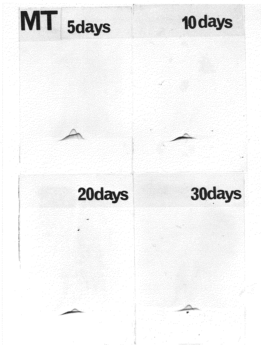
Fig. 65. Crossed immunoelectrophoresis of sera from methyl-testosterone-treated medaka.
