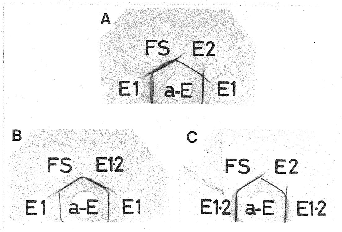
Fig. 16. Precipitin reaction of FS, E1 and E2 from rainbow trout. FS, E1 and E2: same as in Fig. 15. E1·2: E1 plus E2. a-E: anti-trout eggs. After removal of unprecipitated protein by washing and drying, the precipitin arcs were stained with Amido black 10B.
