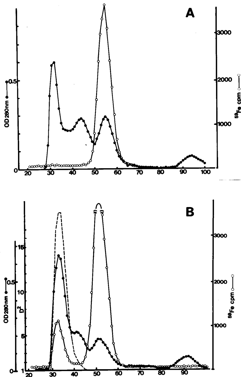
Fig. 28. Gel filtration on Sephadex G-200 of rainbow trout serum collected from non-estrogen treated (A) and estrogen-treated (B) fish. The presence of FS (dotted line) was assessed by the Mancini method using anti-trout FSSP. Column: 2.0×47cm, Elution buffer: 0.02M Tris-HCl, pH 8.0, containing 2% NaCl and 0.1% NaN 3 . Each serum was 0.5 ml and was mixed with 10 \mu\text{l} of ^{59}\text{Fe} (0.25 \mu\text{Ci} ).
