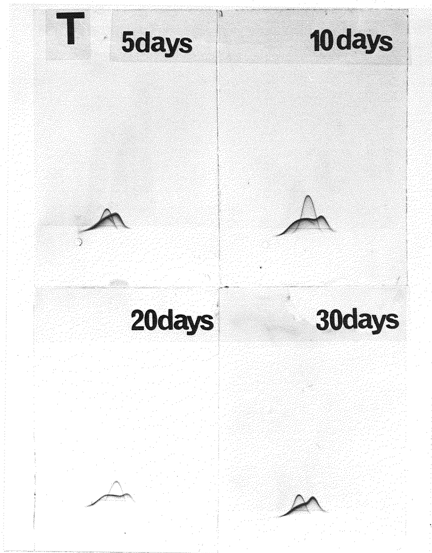
Fig. 66. Crossed immunoelectrophoresis of sera from testosterone-treated medaka.
