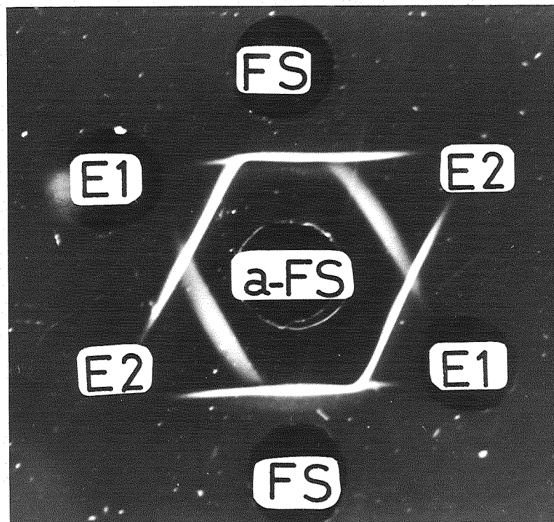
Fig. 15. Precipitin reaction of FS, E1 and E2 from rainbow trout. FS: female-specific iron-binding serum protein. E1 and E2: fractions of egg yolk proteins. a-FS: anti-trout FSSP.
