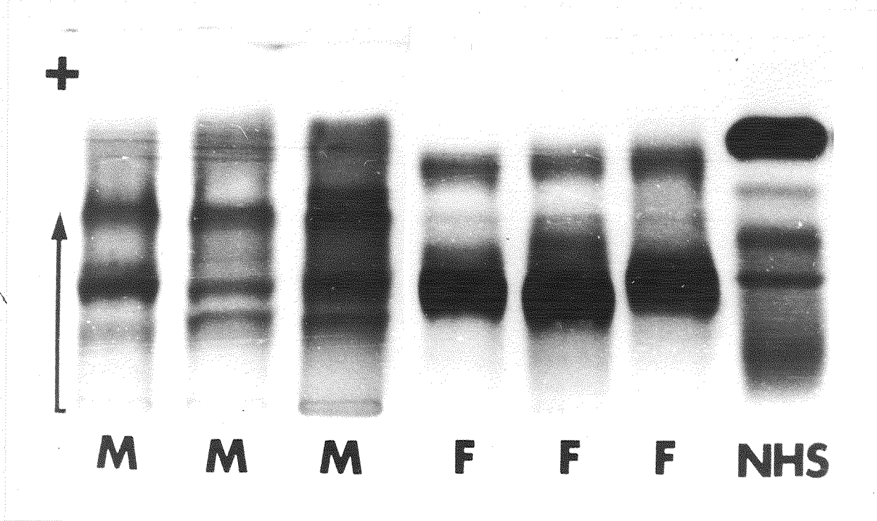
Fig. 47. Typical electrophoretic patterns of serum of silver migrated forms of male Japanese eel (M) and of female Japanese eel (F) treated with salmon pituitary glands. NHS: normal human serum.
