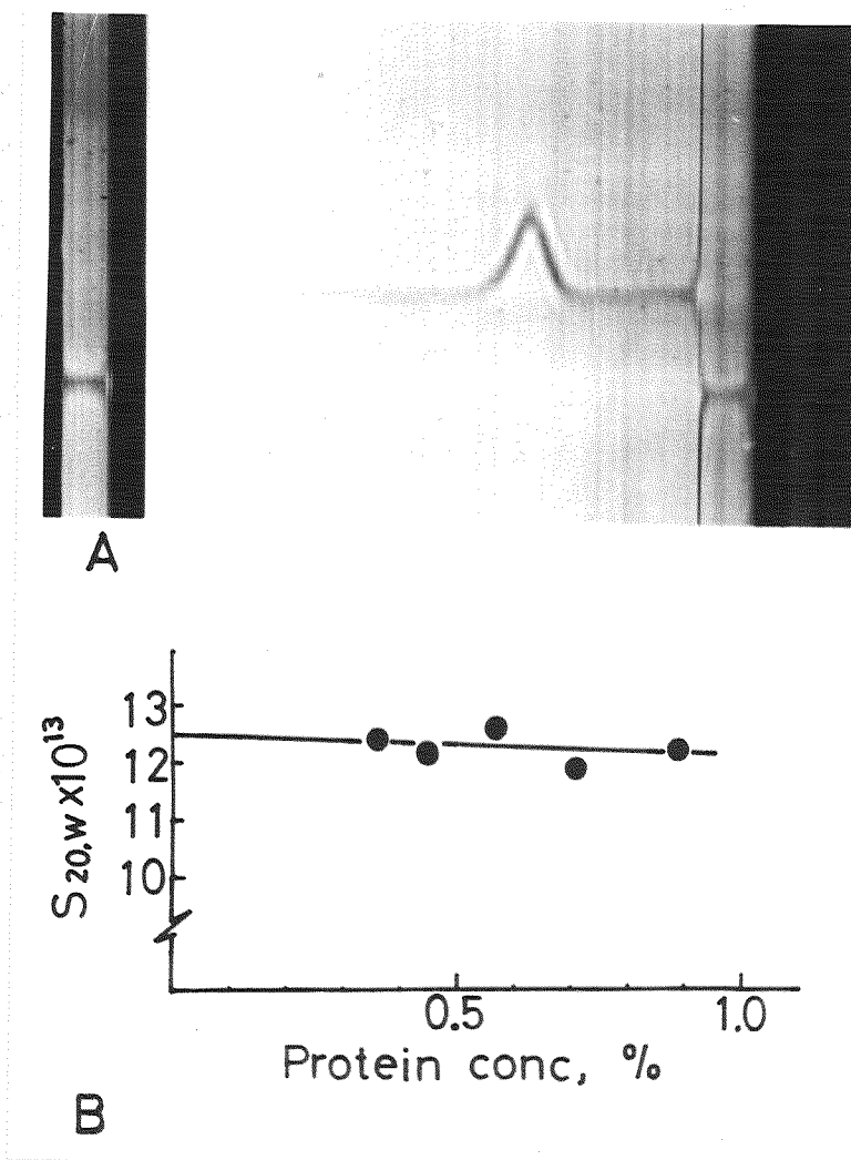
Fig. 46. Ultracentrifugation of purified FS of chum salmon. (A) Schlieren pattern of the purified FS at concentration of 0.9% in 0.15 M NaCl. Photograph was taken 24 min after reaching to 56,100 rpm. (B) Concentration dependency of the sedimentation rate.
