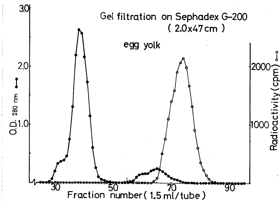
Fig. 6. Gel filtration on Sephadex G-200 of egg yolk extracts from rainbow trout. One radioactive peak was observed at the very small molecular weight fraction.
