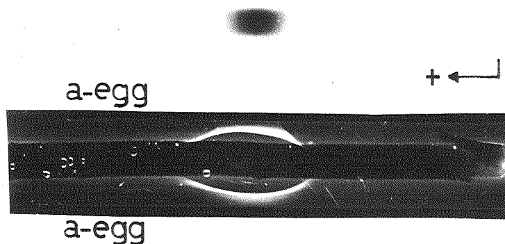
Fig. 14. Disc immunoelectrophoresis of purified E1 (A) and E2 (B) isolated from egg yolk proteins of rainbow trout. The samples were subjected first to disc electrophoresis in 5% or 7.5% polyacrylamide gel, followed by immunodiffusion in 1.2% agarose gel. a-egg: antiserum to trout eggs (anti-trout eggs).
