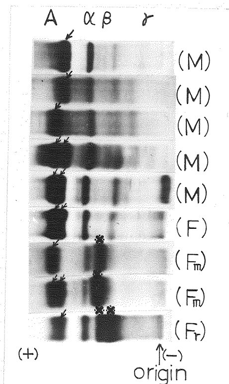
Fig. 1. Typical cellulose acetate membrane (Cello-gel) electrophoretic patterns of serum of male (M) and female (F) rainbow trout. The electrophoregrams show one (↘) or two bands (↘↘) in the albumin fraction. All specimens of maturing (Fm) and ripe (Fr) females have one or two components (*) in the \beta -globulin region.
