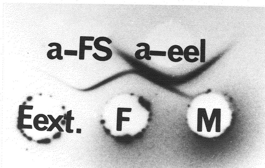
Fig. 49. Autoradiography of a gel diffusion reaction between the ^{59}\text{Fe} -binding proteins in serum or egg yolk proteins of Japanese eel, and rabbit antisera. a-eel: anti-eel serum. M, F, Eext., a-FS: same as in Fig. 48.
