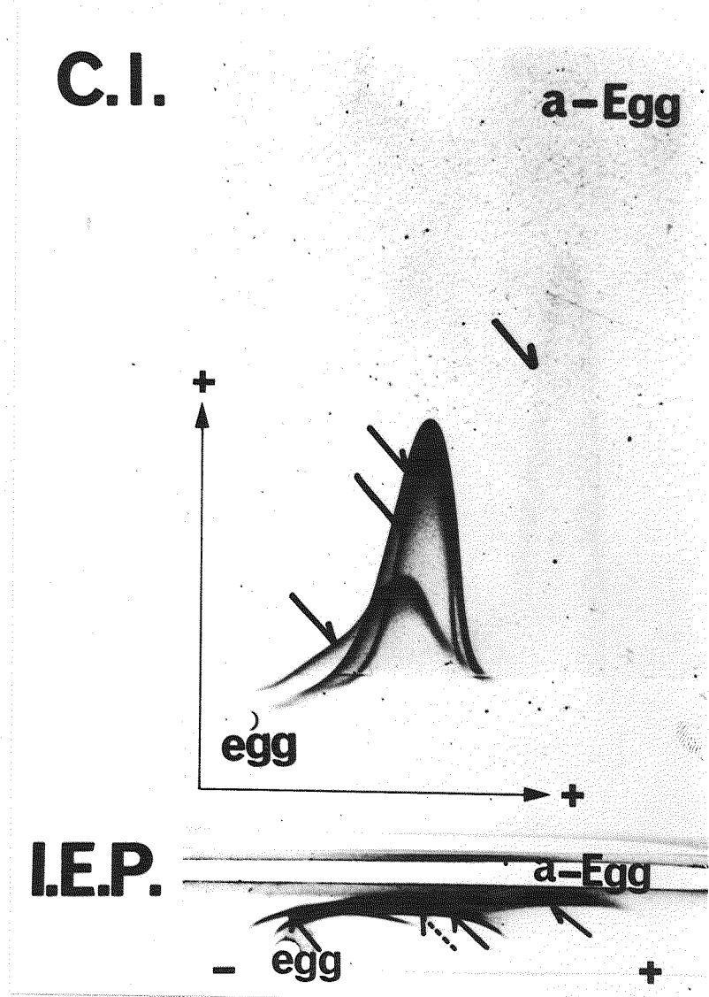
Fig. 54. Immunoelectrophoresis (I.E.P.) and crossed immunoelectrophoresis (C.I.) of egg yolk proteins of medaka. Antigen: 4 \mu l of 0.9% NaCl extracts of ovulated eggs of medaka. The antiserum used was the polyvalent antiserum to medaka egg yolk extracts (a-Egg) in both electrophoresis. First dimension (C.I.): 90 minutes, 10 V per cm. Anode to the right. Antibodies: 0.4 ml antiserum plus 6 ml agarose. Second dimension: overnight (20 hours), 3 V per cm, anode at the top. Staining: Commassie brilliant blue R-250.
