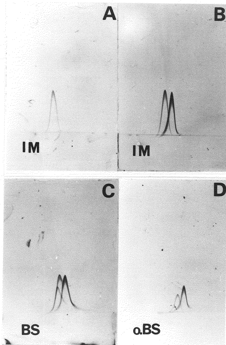
Fig. 58. Crossed immunoelectrophoresis of female medaka serum of various maturations. IM: "immature" (A.B), BS: "breeding", o.BS: "sexually inactive". Details in test.
