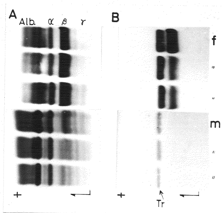
Fig. 3. Cellulose acetate membrane (Cellogel) electrophoresis of ripe rainbow trout sera (A) and its autoradiography with ^{59}\text{Fe} (B). f: female serum, m: male serum, Tr: transferrin. To 25 \mu\text{l} of the serum was added 10 \mu\text{l} of ^{59}\text{FeCl}_3 solution with an activity of 0.1 \mu\text{Ci} , corresponding to 0.003 \mu\text{g} Fe. After incubation the mixture was subjected to electrophoresis, and the gels were exposed to X-ray films for 2 weeks.
