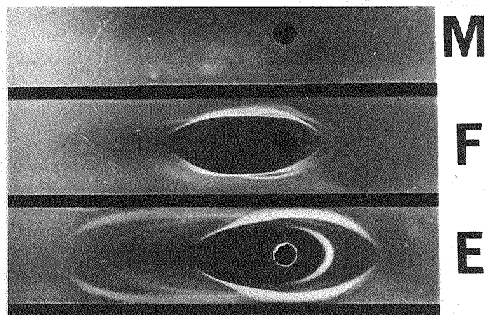
Fig. 2. Immunoelectrophoresis of serum of ripe male (M) and female (F) rainbow trout, and egg yolk extracts (E) with rabbit anti-trout FSSP.
