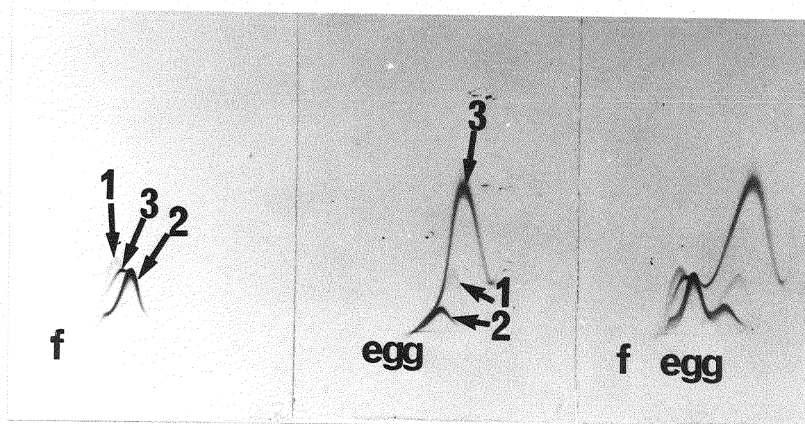
Fig. 63. Tandem-crossed immunoelectrophoretic comparison of serum and egg in medaka. Antigen: female medaka serum in breeding season (f), egg yolk extracts of medaka (egg).
