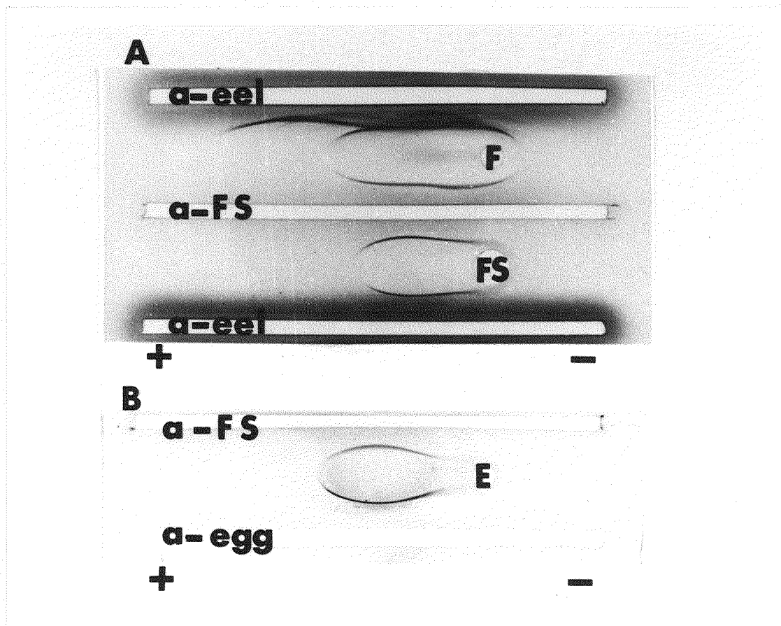
Fig. 50. Immunoelectrophoresis of purified FS (A) and egg yolk protein (B) of Japanese eel. FS: female-specific iron-binding serum protein, E: FS related egg yolk protein, \alpha -egg: rabbit antiserum against egg yolk proteins extracted with 0.9% NaCl (anti-eel eggs), F, \alpha -eel, \alpha -FS: same as in Fig. 49.
