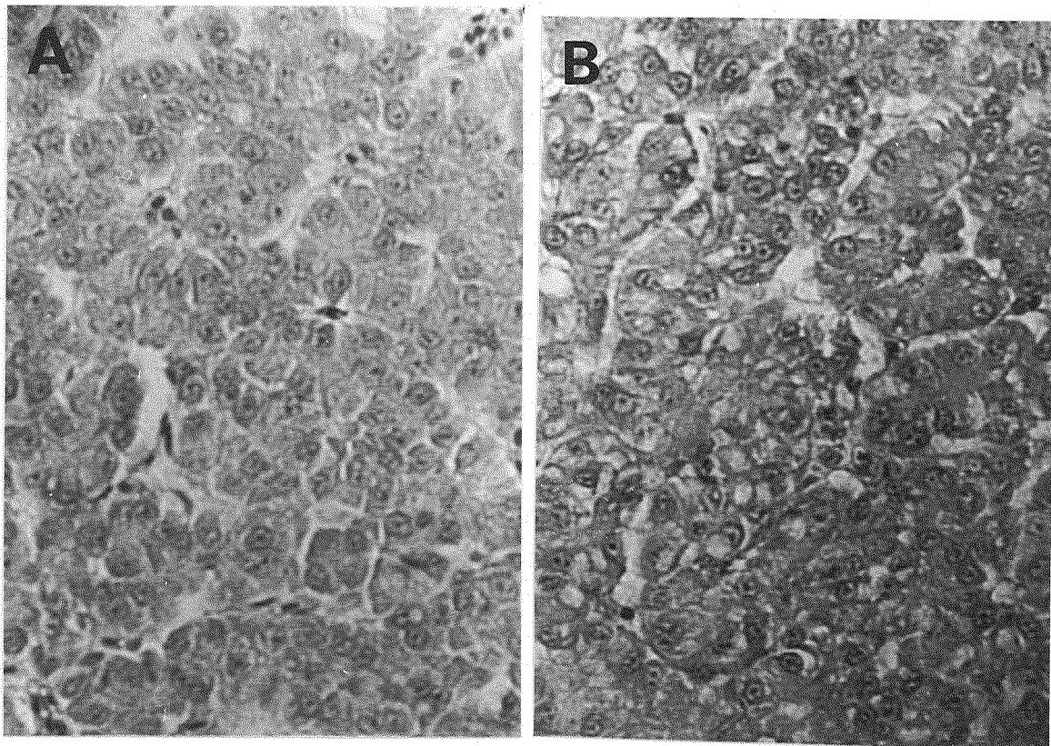
Fig. 31. Liver cells of immature rainbow trout (A) and of estradiol-17 \beta -treated immature fish (B).
