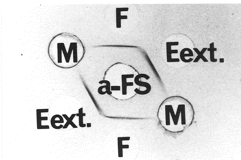
Fig. 48. Precipitin reaction of serum and egg yolk proteins of Japanese eel against anti-eel FSSP. M: male serum, F: female serum, Eext.: egg yolk proteins extracted with 0.9% NaCl, a-FS: anti-eel FSSP (see Table 1).
