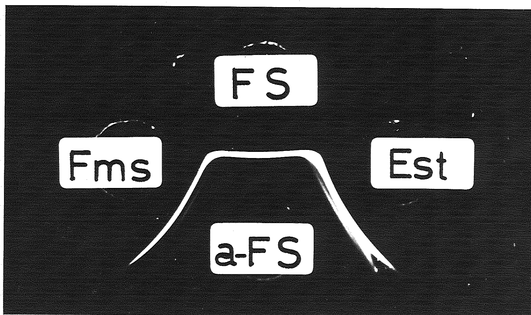
Fig. 26. Precipitin reaction of FS, sera of maturing female and estrogen-treated male rainbow trout. Fms: serum of maturing female fish. Est: serum of estrogen-treated fish (6 days after injection). FS: female-specific iron-binding serum protein of rainbow trout, a-FS: anti-trout FSSP.
