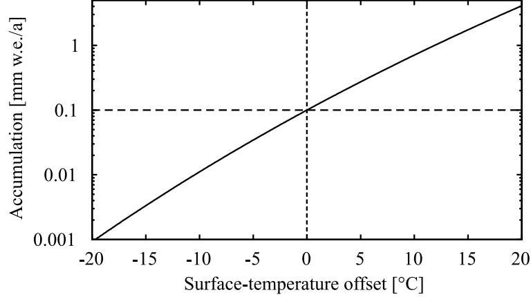
Figure 4: Accumulation rate a_{\text{sat}}^+ as a function of surface-temperature offset \Delta T_s , for present value a_{\text{sat},0}^+ = 0.1 \text{ mm w.e. a}^{-1} .
