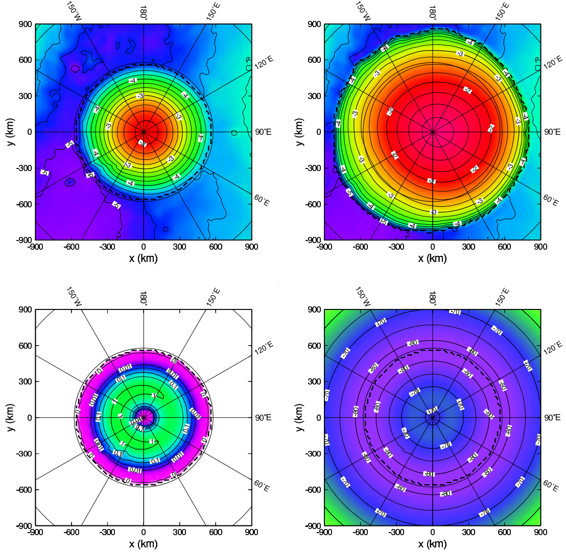
Figure 7: Standard steady-state simulation. Top left: Surface topography for t_{\text{build}} = 29.66 Ma (in km relative to the reference geoid). Top right: Surface topography for t_{\text{final}} = 500 Ma (in km relative to the reference geoid). Bottom left: Surface velocity for t_{\text{build}} = 29.66 Ma (in \text{mm a}^{-1} ). Bottom right: Basal temperature relative to pressure melting for t_{\text{build}} = 29.66 Ma (in ^{\circ}\text{C} ). In all panels, heavy-dashed lines indicates the ice margin.
