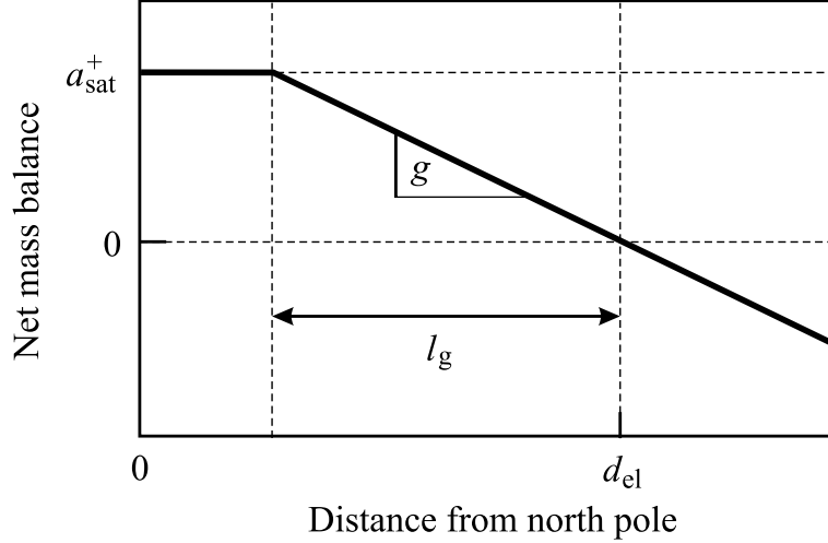
Figure 5: Distance-dependent parametrization of the net mass balance (accumulation-ablation rate).
