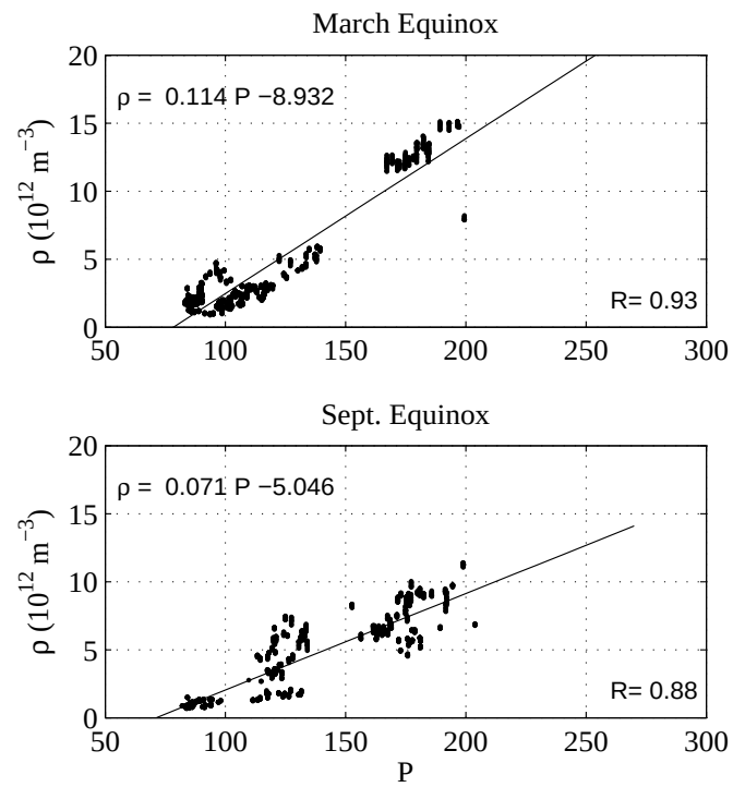
Figure 10. Solar activity dependence of the noontime neutral density at the dip equator.
