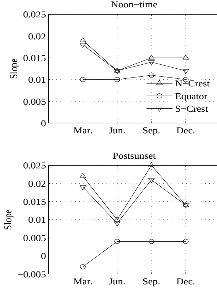
Figure 9. Slopes of the solar activity dependence of Ne in different seasons in the EIA trough and crest regions for noon and post-sunset local time sectors. Slopes are obtained by least-square fitting of data points for P \leq 200 shown in Figures 7 and 8.
