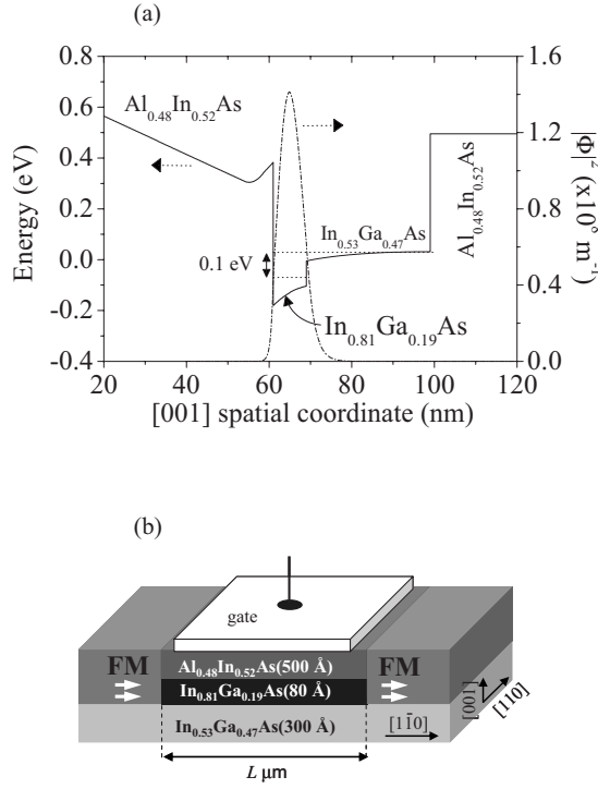
FIG. 1. (a) Calculated spatial profiles of conduction band (left vertical axis) and square of wave function (right vertical axis) at V_g=0 . (b) Schematic picture of the present spin-FET structure.
