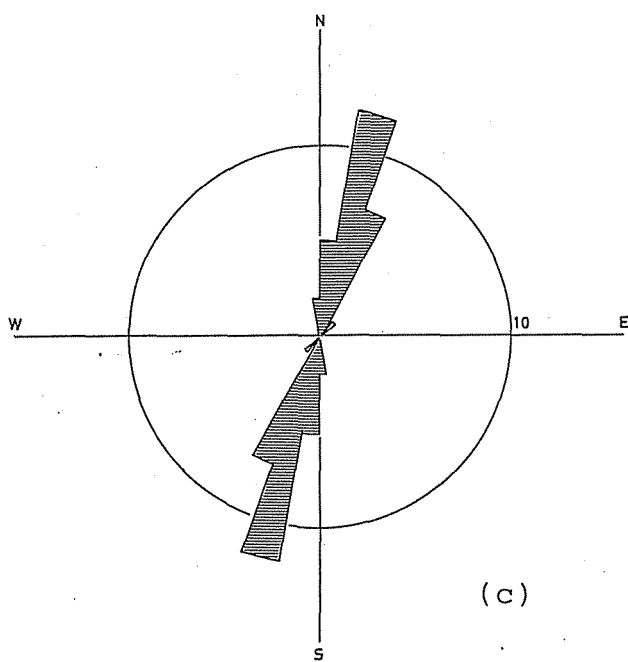
CUYA DIKE SWARM
