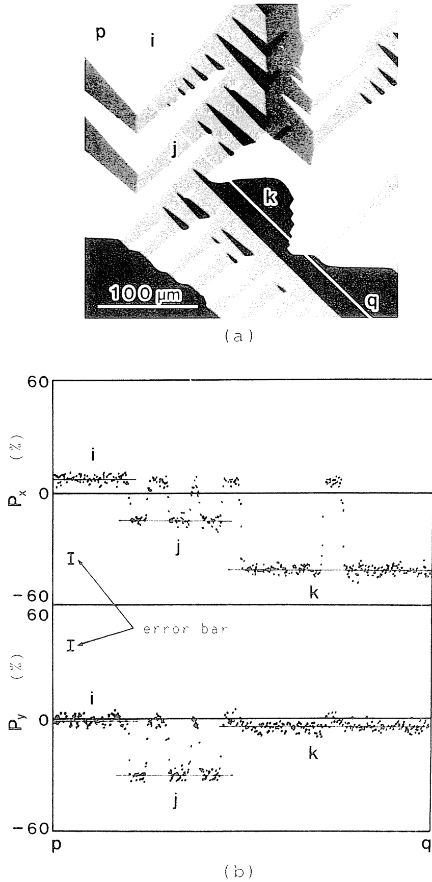
Fig. 4.9. Domain image (a) of an Fe (001) surface and polarization components P_x and P_y (b) on a straight line pq. 8
