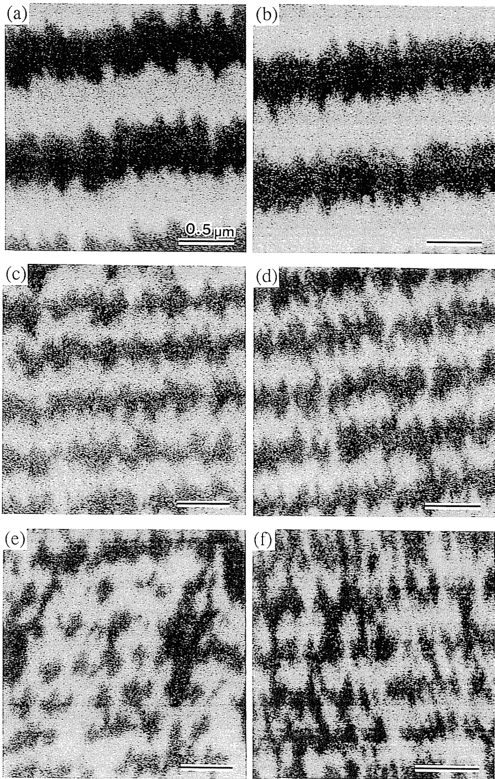
Fig. 7.2. Bit images are of the magnetization component along the track direction. Images (a), (c), and (e) are obtained from 10 at% Cr-CoCrTa, and correspond to 50, 100, and 140 kFCl. Images (b), (d), and (f) are from 16 at% Cr-CoCrTa and correspond to the same densities as the previous images. 4
