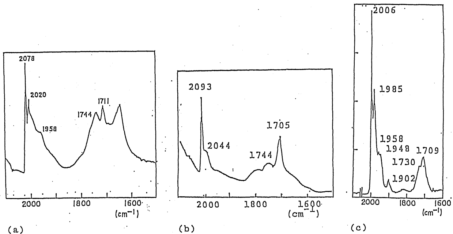
Figure 3. FTIR spectra of \text{Rh}_x\text{Fe}_y(\text{CO})_z/\text{NaY} (a), [\text{NMe}_3(\text{CH}_2\text{Ph})]_2[\text{Fe}_2\text{Rh}_4(\text{CO})_{18}] deposited on NaY (b), and [\text{NMe}_3(\text{CH}_2\text{Ph})]_2[\text{Fe}_2\text{Rh}_4(\text{CO})_{18}] in acetonitrile (c).
