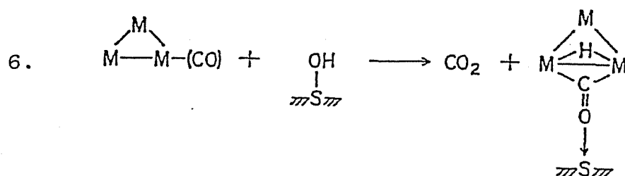
Figure 8. Reactions of organometallic compounds with oxide surfaces. 3
