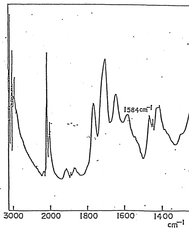
Figure 5. In situ FTIR spectrum of \text{Rh}_x\text{Fe}_y/\text{NaY} under the conditions of ethylene hydroformylation: 150 °C; \text{C}_2\text{H}_4+\text{CO}+\text{H}_2 (1:1:1) gas, flow rate = 60 ml/min, 1 atm.
