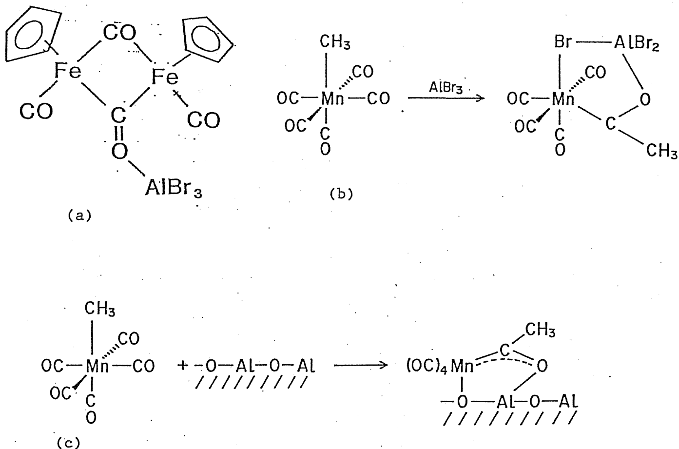
Figure 10. Adduct formation between metal carbonyls and Lewis acids: (a) \text{Cp}_2\text{Fe}_2(\text{CO})_4 with \text{AlBr}_3 , (b) \text{Mn}(\text{CH}_3)(\text{CO})_5 with \text{AlBr}_3 , and (c) \text{Mn}(\text{CH}_3)(\text{CO})_5 with \text{Al}_2\text{O}_3 . In (b) and (c), Lewis acids greatly enhance the methyl migration (CO insertion).
