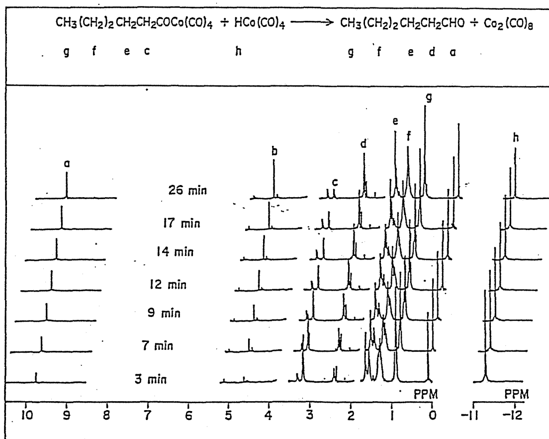
Figure 2. Stacked plot of ^1\text{H} NMR spectra during the reaction of hexanoylcobalt tetracarbonyl with \text{HCo}(\text{CO})_4 at 20^\circ\text{C} (Table 1, Run 1). The peak b is uncharacterized.
