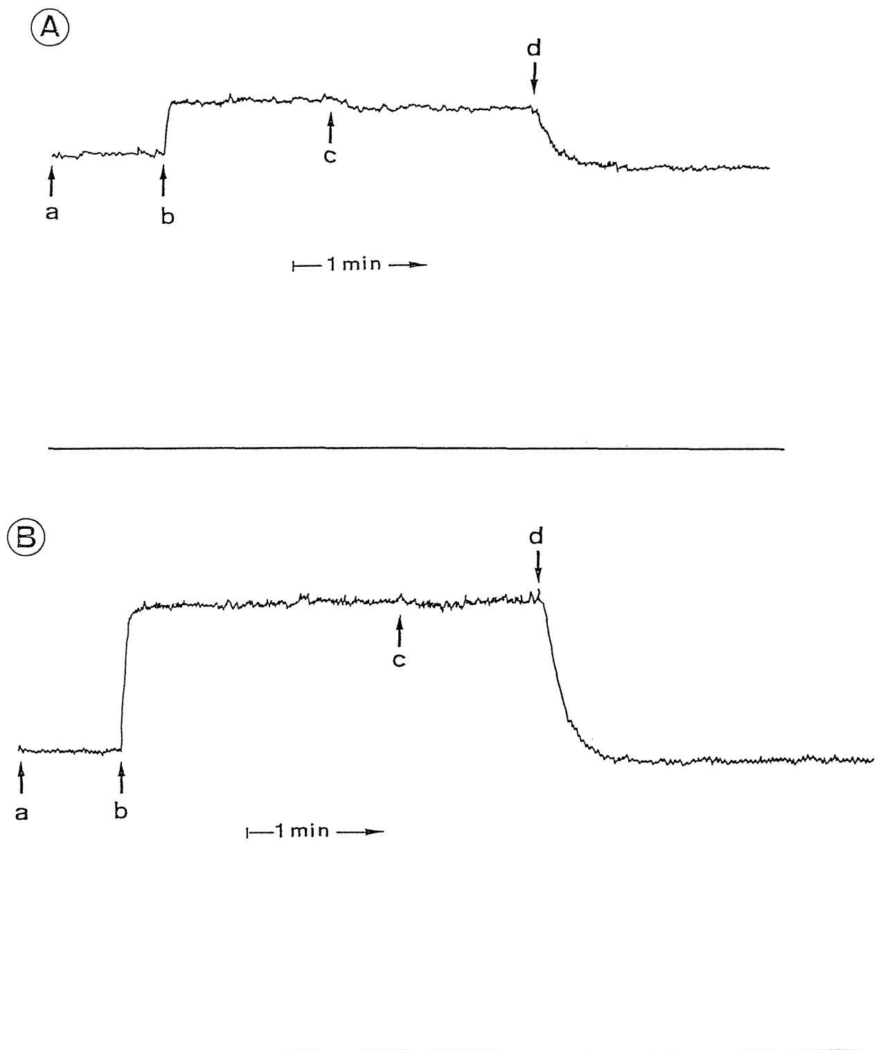
Fig. 8. Time course of fluorescence intensity change of DNS-ATP in the presence of \alpha subunit. (A) To a reaction mixture containing 0.8 \mu M \alpha subunit in a buffer solution (2 mM EDTA, 0.1 M NaCl and 50 mM Tris-acetate at pH 7.0 and 30°C), the following additions were made at the time indicated by arrows (a-d); a, 1.1 \mu M DNS-ATP; b, 5 mM MgCl_2 ; c, 2 mM K-P_i ; d, 2 mM ATP. (B) To a reaction mixture containing 4 \mu M \alpha subunit in the buffer solution, the following additions were made at the time indicated by arrows (a-d); a, 1.1 \mu M DNS-ATP; b, 5 mM MgCl_2 ; c, 0.2 mM AMP; d, 0.2 mM ATP.
