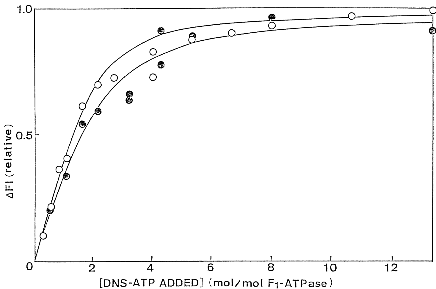
Fig. 5. Fluorometric titration of F_1 by DNS-ATP in the presence of MgCl_2 . The extent of fluorescence enhancement 2 min after addition of 5 mM MgCl_2 was plotted against the amount of DNS-ATP added. The reaction mixture contained 0.75 (●) or 1.5 \mu M (○) F_1 in 2 mM EDTA, 50 mM Tris-HCl at pH 8.0. The solid lines are the theoretical curves (see text). The upper is for 1.5 \mu M F_1 , and the lower for 0.75 \mu M F_1 .
