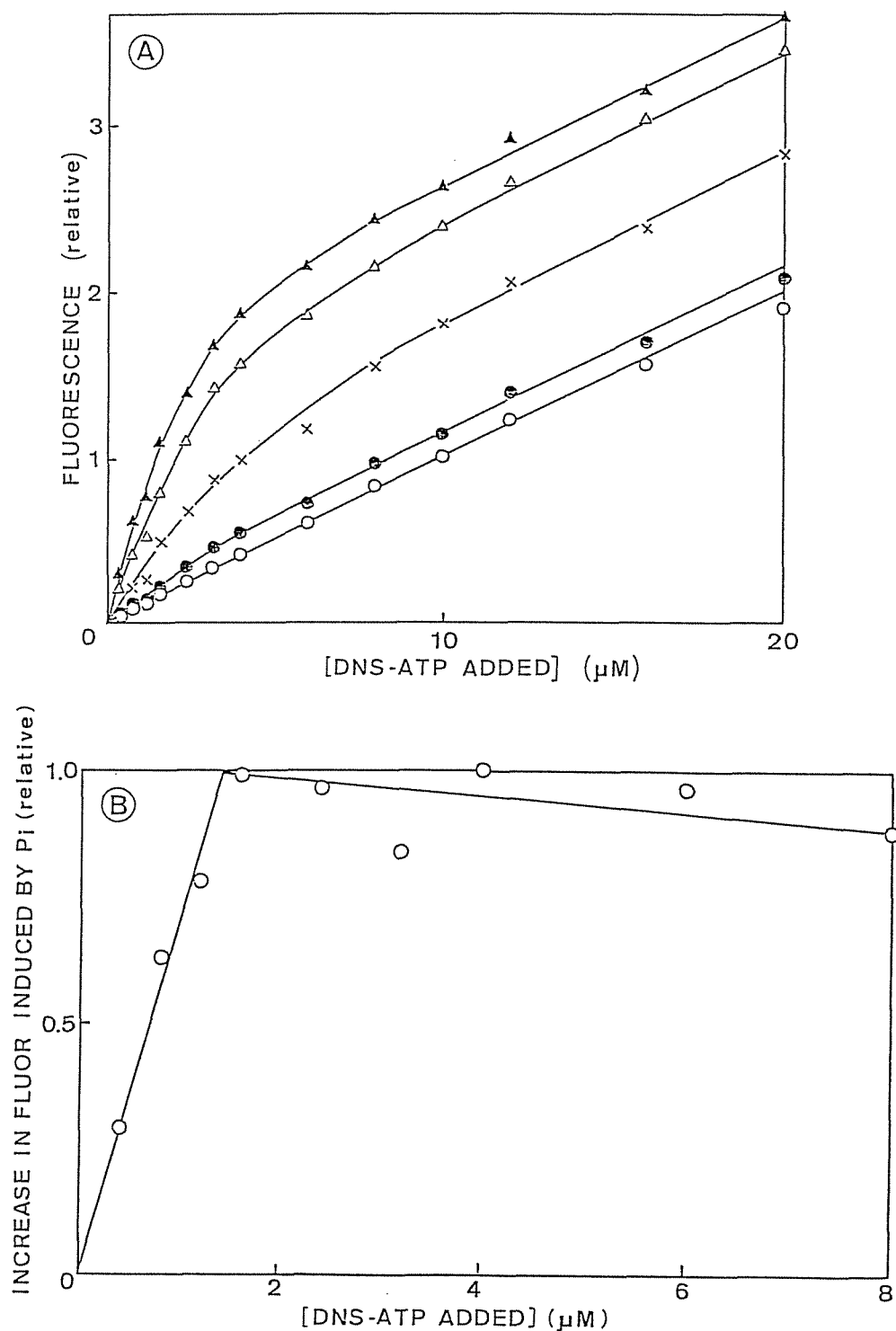
Fig. 27. Fluorometric titration of F_1 by DNS-ATP in the presence of \text{P}_i . A: The fluorescence intensity was measured sequentially as follows; DNS-ATP alone (O); 1 min after addition of 1.5 \mu\text{M} F_1 ( \odot ); 2 min after addition of 5 \text{ mM} \text{MgCl}_2 ( \Delta ); 2 min after addition of 8 \text{ mM} \text{K-P}_i ( \blacktriangle ); the level decreased rapidly on addition of 0.2 \text{ mM} ATP ( \times ). B: The extent of fluorescence enhancement after addition of 8 \text{ mM} \text{K-P}_i ( \blacktriangle minus \Delta ) was plotted against the concentration of DNS-ATP added.
