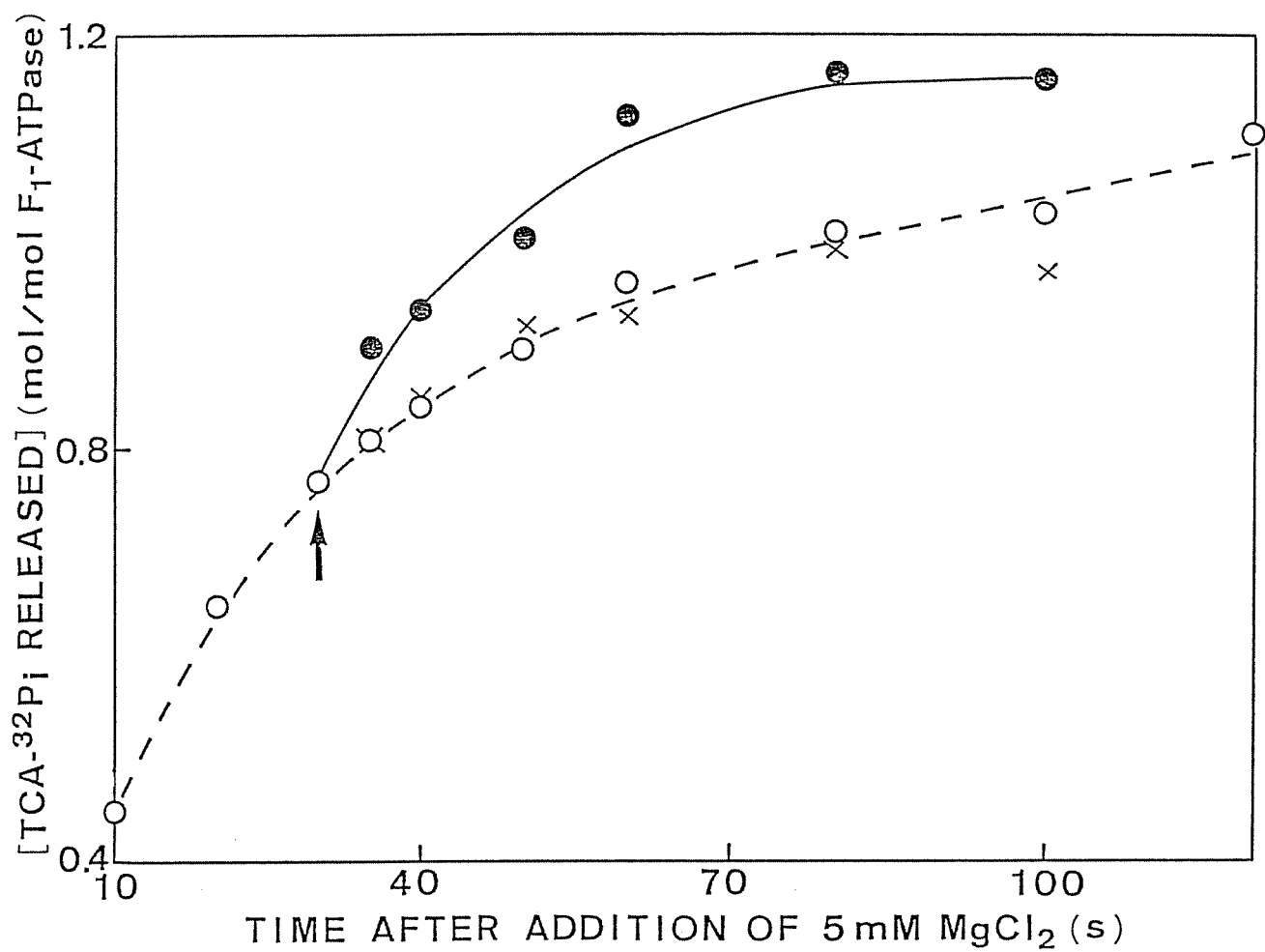
Fig. 19. Effect of CTP and AMP on TCA- 32 P i liberation from the F 1 -DNS-AT 32 P system. The reaction mixture contained 1.8 \mu M DNS-AT 32 P and 1.2 \mu M F 1 in 2 mM EDTA, 50 mM Tris-HCl at pH 8.0. The reaction was started by addition of 5 mM MgCl 2 . At the arrow (30 s), 0.2 mM CTP (●) or 0.2 mM AMP (X) was added. The control (O) is also indicated.
