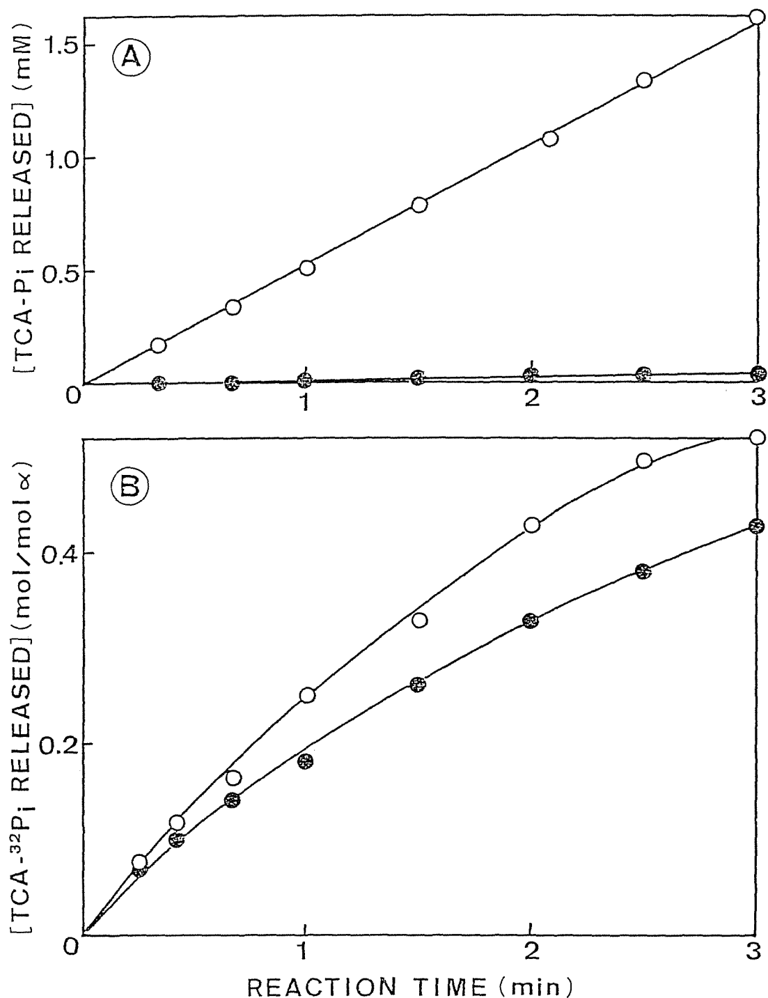
Fig. 7. Effects of DCCD-treatment of EF_1 on its steady-state ATPase and single turnover of DNS-ATP hydrolysis. (A) EF_1 at 0.87 \mu\text{M} was preincubated with (●) or without (○) 0.2 \text{ mM} DCCD in 2 \text{ mM} EDTA and 50 \text{ mM} Tris-acetate at pH 7.0 and 30^\circ\text{C} for 20 min. Then, EF_1 solution was diluted to 0.087 \mu\text{M} in 5 \text{ mM} phosphoenolpyruvate, 0.11 \text{ mg/ml} pyruvate kinase, 2.5 \text{ mM} \text{MgCl}_2 , 0.2 \text{ mM} EDTA and 50 \text{ mM} Tris-HCl at pH 8.0 and 30^\circ\text{C} . The reaction was started by addition of 5 \text{ mM} ATP. (B) EF_1 at 1.6 \mu\text{M} was preincubated with (●) or without (○) 0.2 \text{ mM} DCCD under the same conditions as A, then allowed to react with 2.8 \mu\text{M} DNS-AT 32 P for 1 min. The reaction was started by addition of 3 \text{ mM} \text{Mg}^{2+} .
