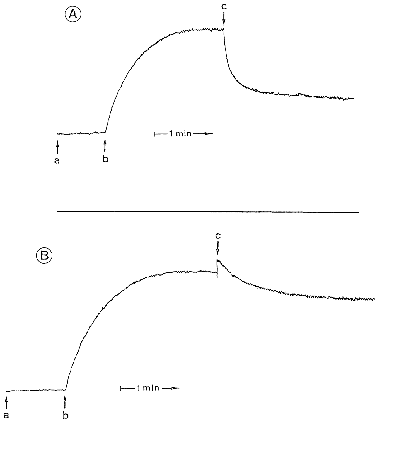
Fig. 6. Inhibition by DCCD-treatment of decrease in the fluorescence intensity of \text{EF}_1 -DNS-nucleotide upon addition of ATP. After incubation of 0.98 \mu\text{M} \text{EF}_1 without (A) or with (B) 0.2 mM DCCD in 2 mM EDTA, 100 mM NaCl and 50 mM Tris-acetate at pH 7.0 and 30°C for 20 min, the following additions were made at the time indicated by arrows (a-c) a, 1.1 \mu\text{M} DNS-ATP; b, 5 mM \text{MgCl}_2 ; c, 2 mM ATP.
