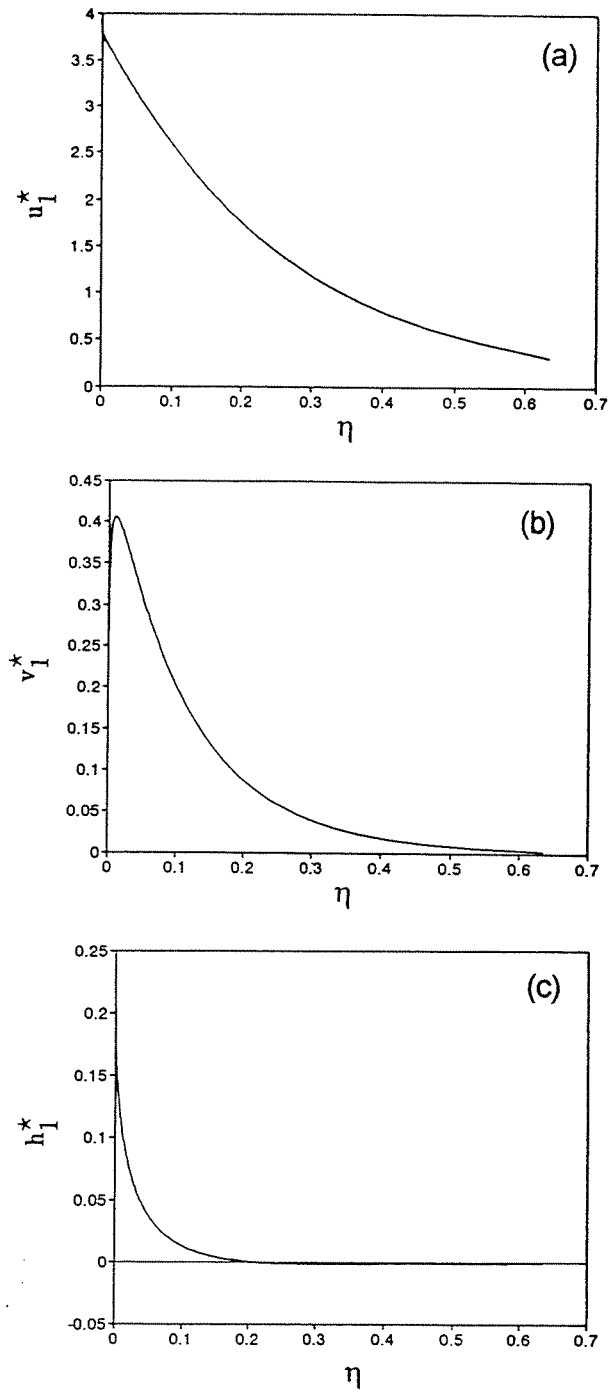
Figure 3-5. Velocity and depth profiles for the case F = 0.5 and k = 4 .
