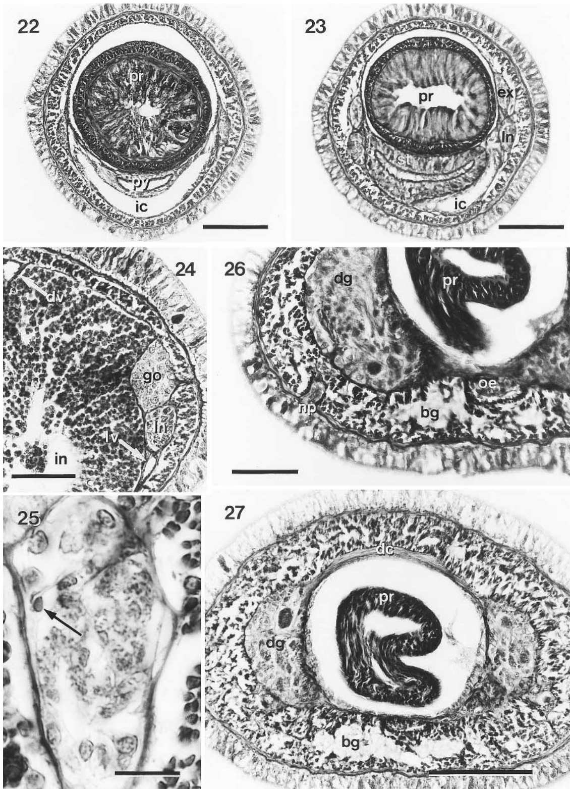
Figs 22–27. Nemertellina yamaokai sp. nov. 22. Transverse section through the pyloric portion (py) of the foregut. 23. Transverse section through the intestinal caecum (ic). 24. Transverse section through the intestine (in) of the holotype to show the distribution of the immature gonads (go). Mid-dorsal (dv) and lateral (lv) blood vessels are indicated by arrows. 25. Transverse section through a lateral nerve cord in the intestinal region; the arrow indicates a myofibrilla. 26. Transverse section through the posterior brain region to show a ventrolateral nephridiopore (np). 27. Transverse section through the brain region at the level of the dorsal cerebral commissure (dc). bg=basophilic cephalic glands; dg=dorsal cerebral ganglion; ln=lateral nerve cord; oe=oesophagus; pr=proboscis. Scale bars: 22, 23, 27=100 µm; 24, 26=50 µm; 25=10 µm.
