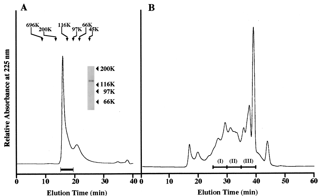
Fig. 1. Gel filtration profiles. (A) H. pulcherrimus sperm mGC (200 \mu g) obtained from the Prep-Cell was applied to a TSK-Gel G6000PW column equilibrated with 50 mM ammonium bicarbonate (pH 8.5) and eluted with the equilibration solution at a flow rate of 0.5 ml/min at 30°C. Fractions of 0.5 ml were collected and the peak fraction (20 \mu l) was analyzed by SDS-PAGE with a 7.5% gel (insert). (B) The tryptic digest of the cyclase was applied to a Superdex Peptide HR10/30 column equilibrated with 50 mM Tris-HCl (pH 7.5) containing 200 mM NaCl and eluted with equilibration solution at a flow rate of 0.5 ml/min at 30°C. Fractions of 0.5 ml were collected and fractions 26 - 30 (I), 31 - 35 (II), and 36 - 40 (III) were pooled, separately. The column effluent was monitored by the absorbance at 225 nm.
