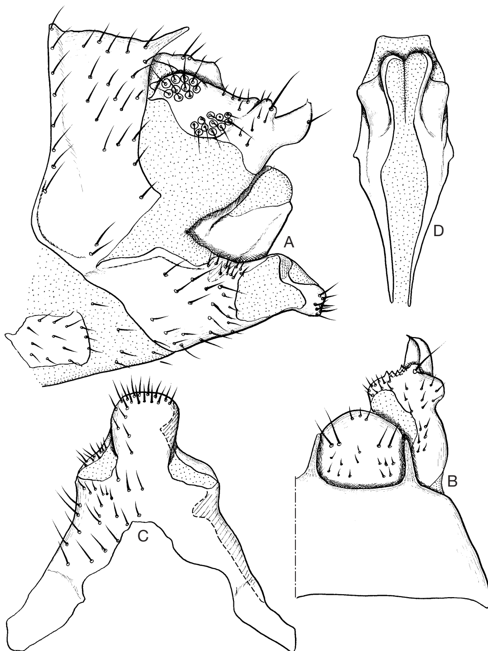
Fig. 4. Male terminalia of Psocidus pellucidus . A, terminalia, lateral view. B, terminalia, dorsal view (hairs on clunium and trichobothrial field not drawn). C, hypandrium, ventral view (hairs not drawn on right side). D, phallosome, ventral view.
