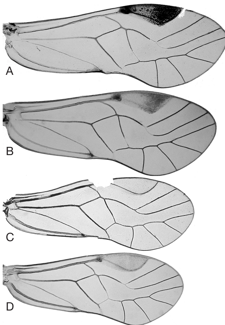
Fig. 1. Forewings of psocids examined in this study. A, Psocidus pellucidus , syntype female. B, P. pellucidus , male. C, Neoblaste tateokana , syntype female. D, N. tateokana , male.
