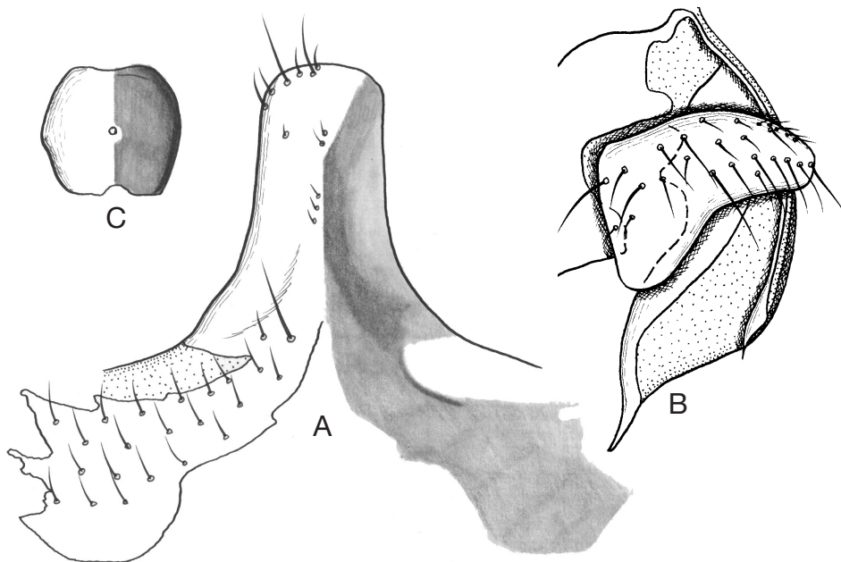
Fig. 3. Genitalia of Psocidus pellucidus , syntype female, ventral view. A, subgenital plate. B, gonapophyses. C, internal plate. A and C show structure (left) and color pattern (right).
