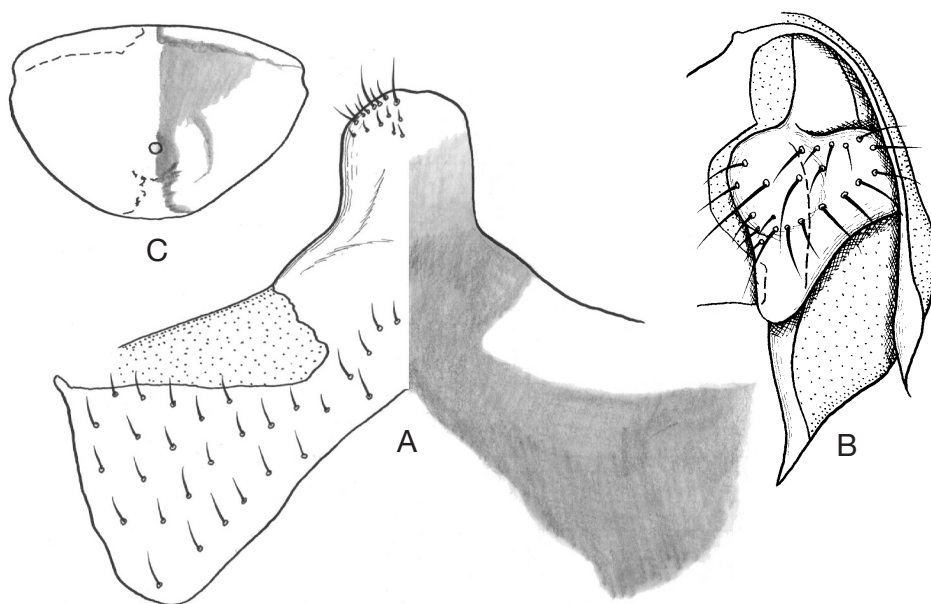
Fig. 5. Genitalia of Neoblaste tateokana , syntype female, ventral view. A, subgenital plate. B, gonapophyses. C, internal plate. A and C show structure (left) and color pattern (right).
