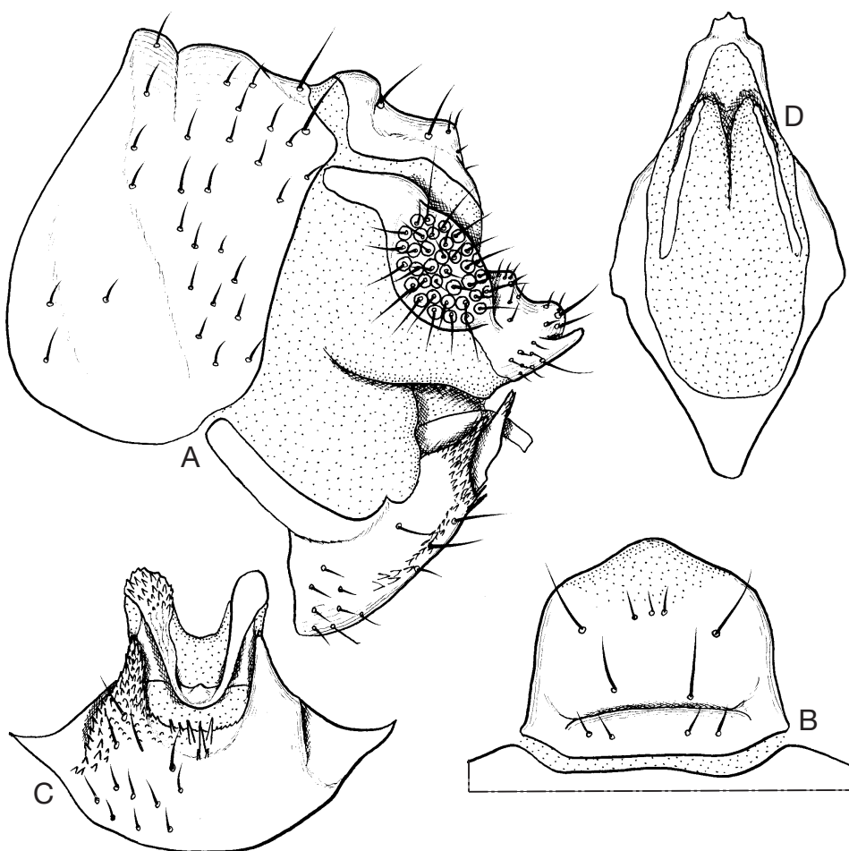
Fig. 2. Terminalia of Symbiopsocus formosanus , syntype male. A, terminalia, lateral view. B, posterior margin of clunium and epiproct, dorsal view. C, hypandrium, posterior view (sculptures, spines and hairs not drawn for right side). D, phallosome, ventral view.
