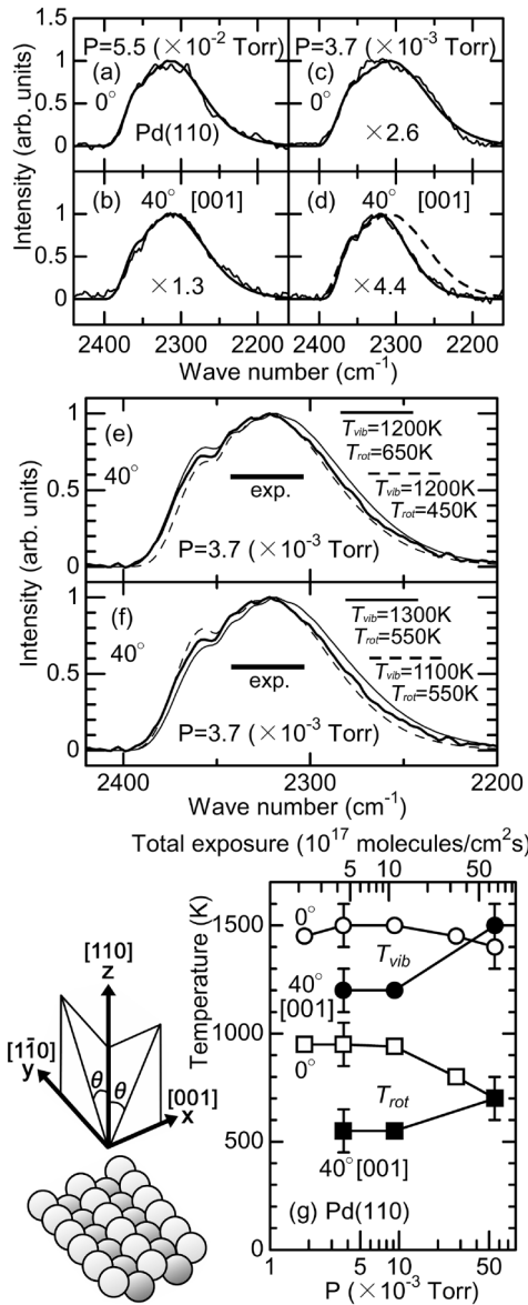
FIG. 1. Chemiluminescence measurements on Pd(110). (a)–(d) Infrared emission spectra at \text{O}_2/\text{CO} = 1/2 and T_{\text{surf}} = 600 K. The resolution of the wave number is 4 \text{ cm}^{-1} . Intensities were normalized so that the maxima of peaks become unity. The thin lines show the emission spectra from AR product \text{CO}_2 at \theta = 0^\circ and P = 5.5 \times 10^{-2} Torr (a), \theta = 40^\circ in [001] and P = 5.5 \times 10^{-2} Torr (b), \theta = 0^\circ and P = 3.7 \times 10^{-3} Torr (c), and \theta = 40^\circ in [001] and P = 3.7 \times 10^{-3} Torr (d). The thick solid lines show the best results of simulation. These were obtained with T_{\text{rot}} = 700 K and T_{\text{vib}} = 1400 K (a), T_{\text{rot}} = 700 K and T_{\text{vib}} = 1450 K (b), T_{\text{rot}} = 950 K and T_{\text{vib}} = 1500 K (c), and T_{\text{rot}} = 550 K and T_{\text{vib}} = 1200 K (d). For comparison, the best simulation at 0^\circ and P = 3.7 \times 10^{-3} Torr is shown by the broken line in (d). (e), (f) Comparison of experimental spectrum (smoothed) and some simulated curves. (g) Dependence on the reactant pressure on Pd(110): T_{\text{vib}} at \theta = 0^\circ (open circles), T_{\text{vib}} at \theta = 40^\circ ([001]) (closed circles), T_{\text{rot}} at \theta = 0^\circ (open squares), and T_{\text{rot}} at \theta = 40^\circ ([001]) (closed squares). Total exposure indicates the sum of \text{O}_2 exposure and \text{CO} exposure and is proportional to P . Schematic illustration of Pd(110), polar angle \theta , and azimuthal directions is shown at the bottom of the left side.
