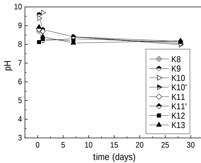
Fig. 2(b) pH changes of the leachate from altered igneous rock samples of K8 to K13
