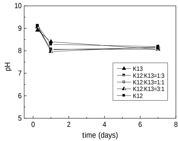
Fig. 12 pH change of the leachate from K12 and K13 mixture
