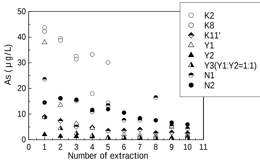
Fig. 16 As concentration changes of the leachate with the number of extractions
