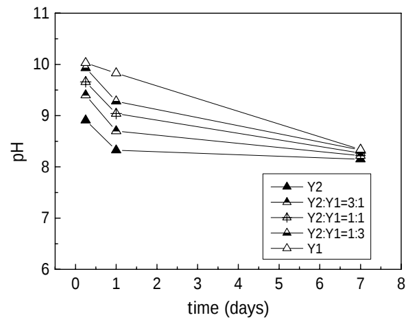
Fig. 13 pH change of the leachate from Y1 and Y2 mixture
