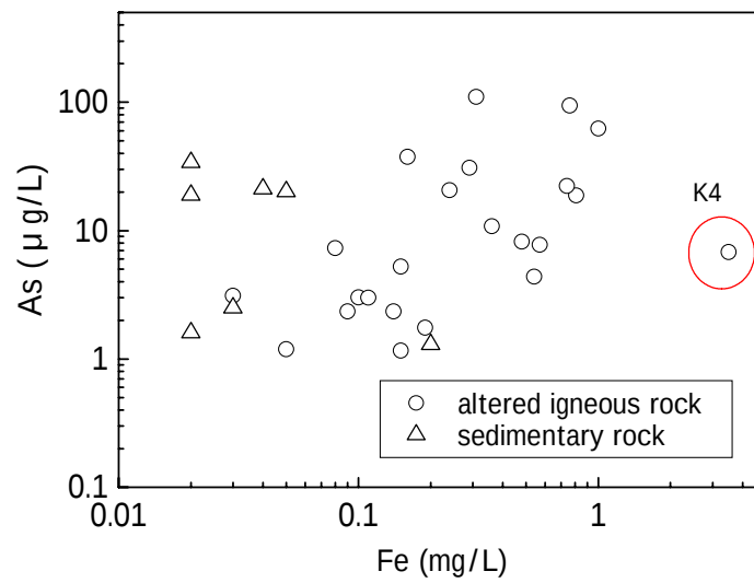
Fig. 6 As concentration in leachate vs Fe concentration in leachate
