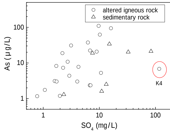
Fig. 5 As concentration in leachate vs \text{SO}_4 concentration in leachate
