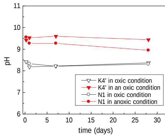
Fig. 15 Comparison of leachate pH in oxic and anoxic conditions
