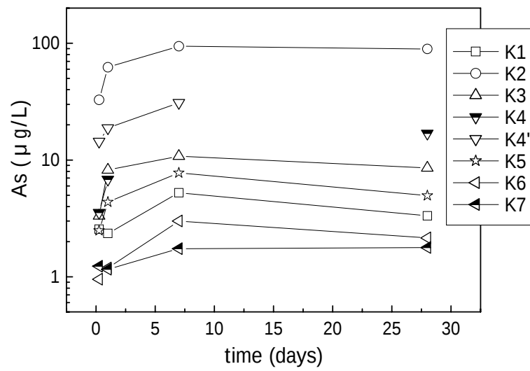
Fig. 1(a) As concentration changes of the leachate from altered igneous rock samples of K1 to K7
