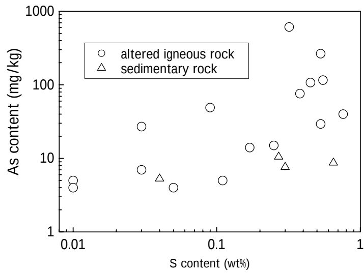
Fig. 9 As content vs S content in rock samples
