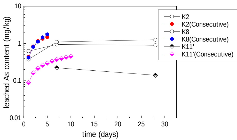
Fig. 18(a) Cumulative leached As content from altered igneous rock samples
