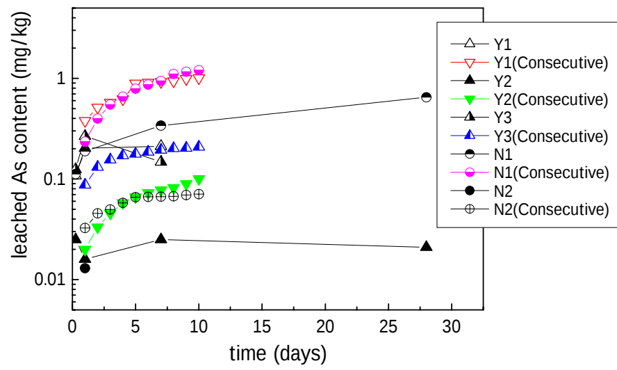
Fig. 18(b) Cumulative leached As content from sedimentary rock samples
