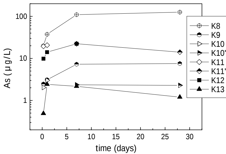
Fig. 1(b) As concentration changes of the leachate from altered igneous rock samples of K8 to K13
