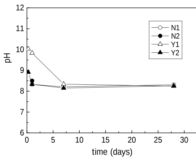
Fig. 4 pH changes of the leachate from sedimentary rock samples
