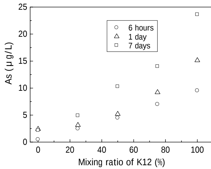
Fig. 10 As concentration in leachate as a function of mixing ratio of K12 sample
