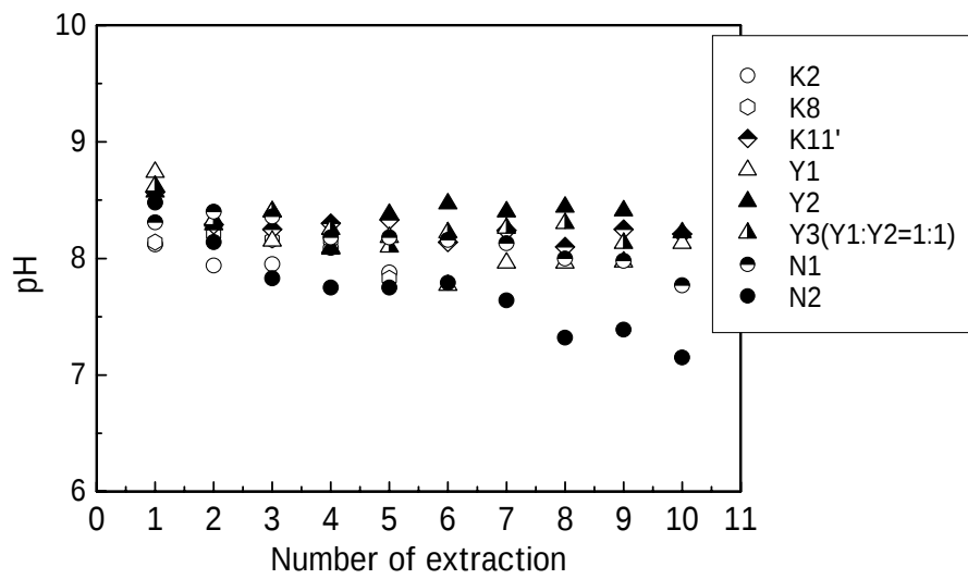
Fig. 17 pH changes of the leachate with the number of extractions
