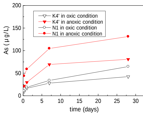
Fig. 14 Comparison of As leaching in oxic and anoxic conditions
