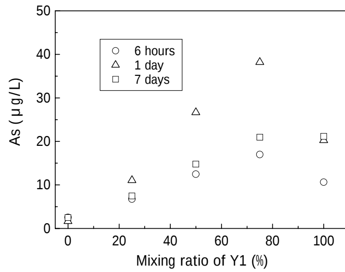
Fig. 11 As concentration in leachate as a function of mixing ratio of Y1 sample
