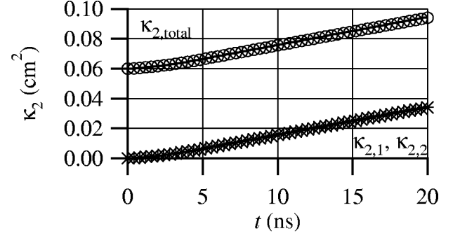
Fig. 10. Second-order cumulants of component and composite electron swarms: +, \kappa_{2,1} (MC); ×, \kappa_{2,2} (MC); o, \kappa_{2,\text{total}} (MC); —, \kappa_{2,1} , \kappa_{2,2} and \kappa_{2,\text{total}} (PM).
