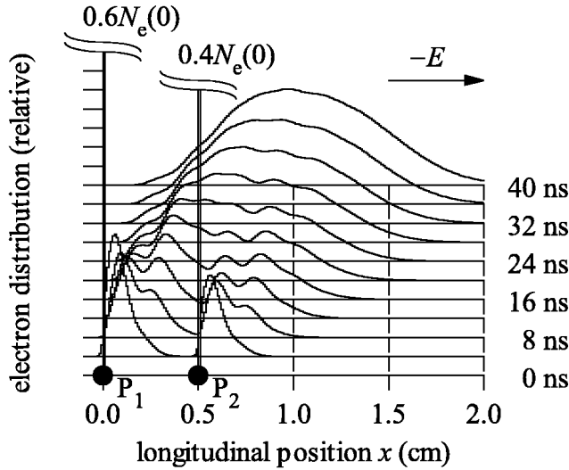
Fig. 12. Spatiotemporal development of electron swarm in \text{CF}_4 calculated by MC at E/N = 283 \text{ Td} . Sixty percent of the initial electrons has been released from electron source P_1 at x = 0 \text{ cm} , and forty percent from electron source P_2 at x = 0.5 \text{ cm} .
