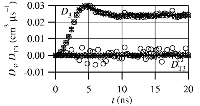
Fig. 14. Third-order longitudinal and transverse diffusion coefficients of component and composite electron swarms calculated by MC: +, D_{3,1} and D_{T3,1} ; x, D_{3,2} and D_{T3,2} ; and o, D_{3,\text{total}} and D_{T3,\text{total}} .
