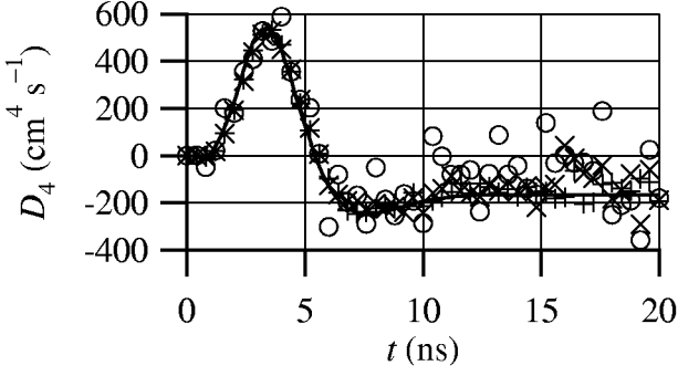
Fig. 7. Fourth-order diffusion coefficients of component and composite electron swarms: +, D_{4,1} (MC); ×, D_{4,2} (MC); o, D_{4,\text{total}} (MC); —, D_{4,1} , D_{4,2} and D_{4,\text{total}} (PM, overlapping).
