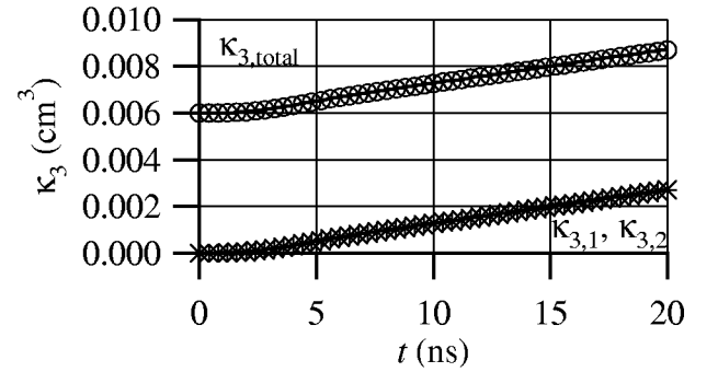
Fig. 11. Third-order cumulants of component and composite electron swarms: +, \kappa_{3,1} (MC); ×, \kappa_{3,2} (MC); o, \kappa_{3,\text{total}} (MC); —, \kappa_{3,1} , \kappa_{3,2} and \kappa_{3,\text{total}} (PM).
