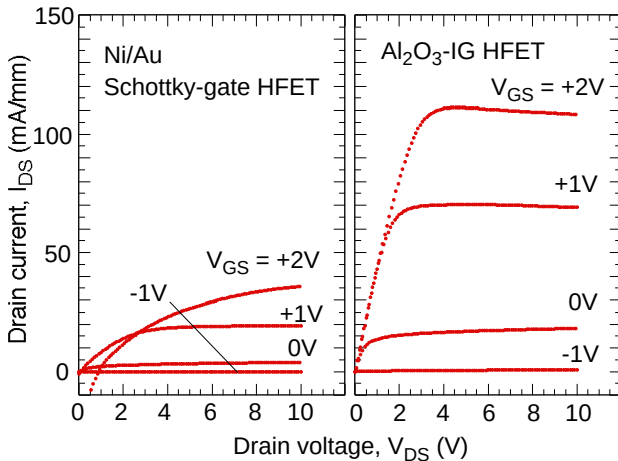
Fig.2 Drain I-V characteristics of the Ni/Au Schottky-gate and Al 2 O 3 IG HFETs with device size of 1 mm x 60 mm.
